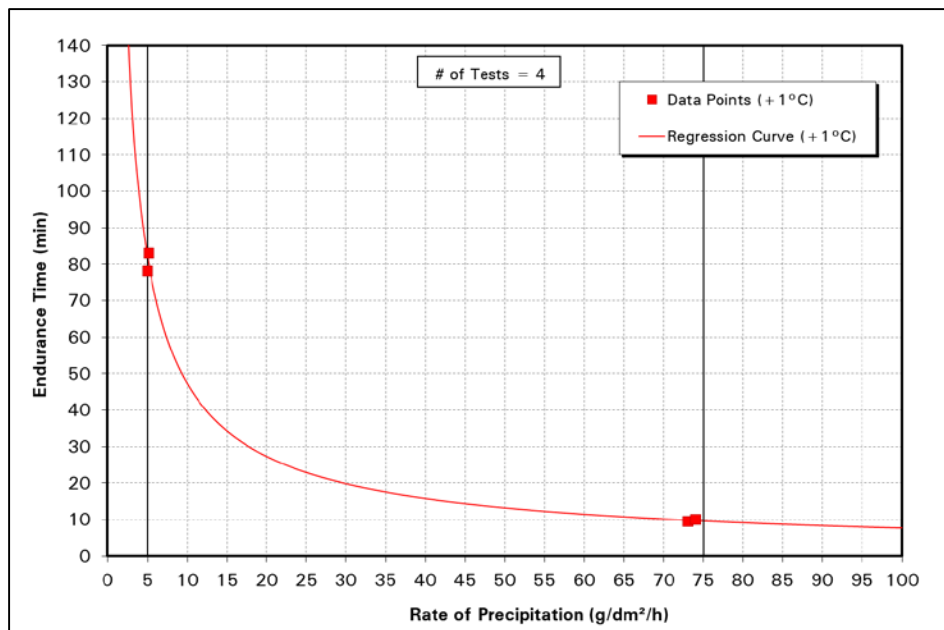
Figure 5.1: Sample Regression Curve – Cold-Soaked Wing
