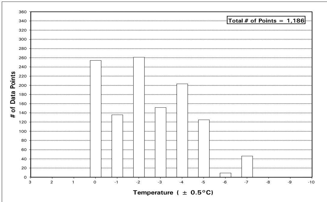
Figure 5.10: Distribution of Freezing Rain/Drizzle Mixed with Ice Pellets Data Points by Temperature for Winters 2006-07 to 2012-13
