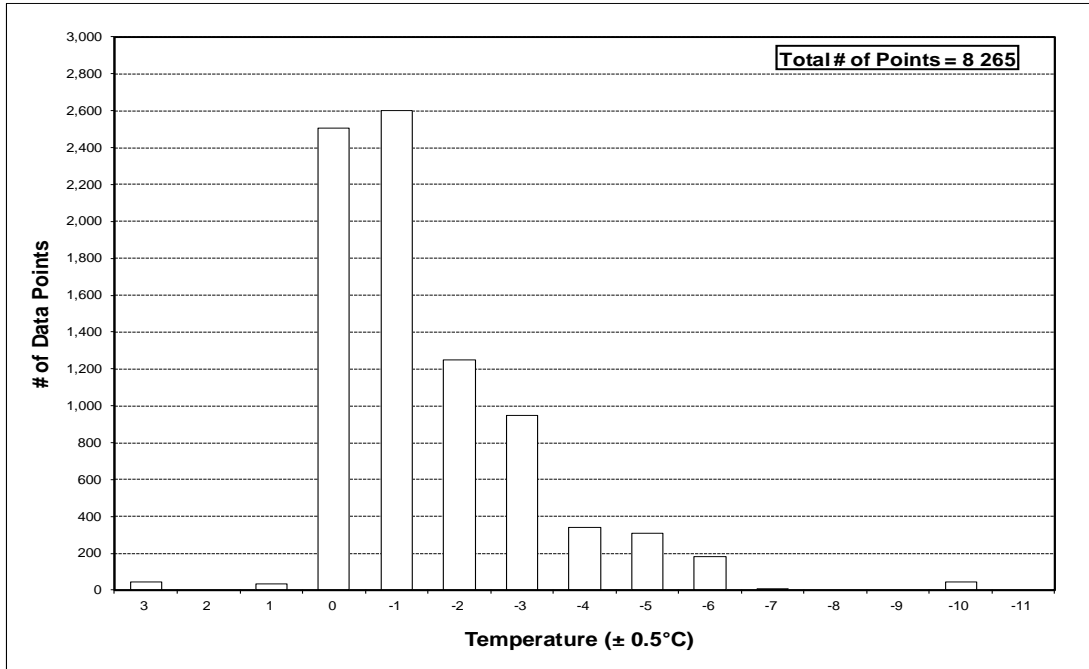
Figure 5.1: Distribution of Pure Freezing Rain/Drizzle Data Points by Temperature for Winters 2007-08 to 2012-13
