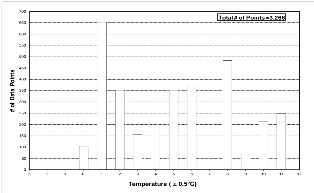
Figure 5.4: Distribution of Freezing Rain/Drizzle Mixed with Snow Data Points by Temperature for Winters 2007-08 to 2012-13
