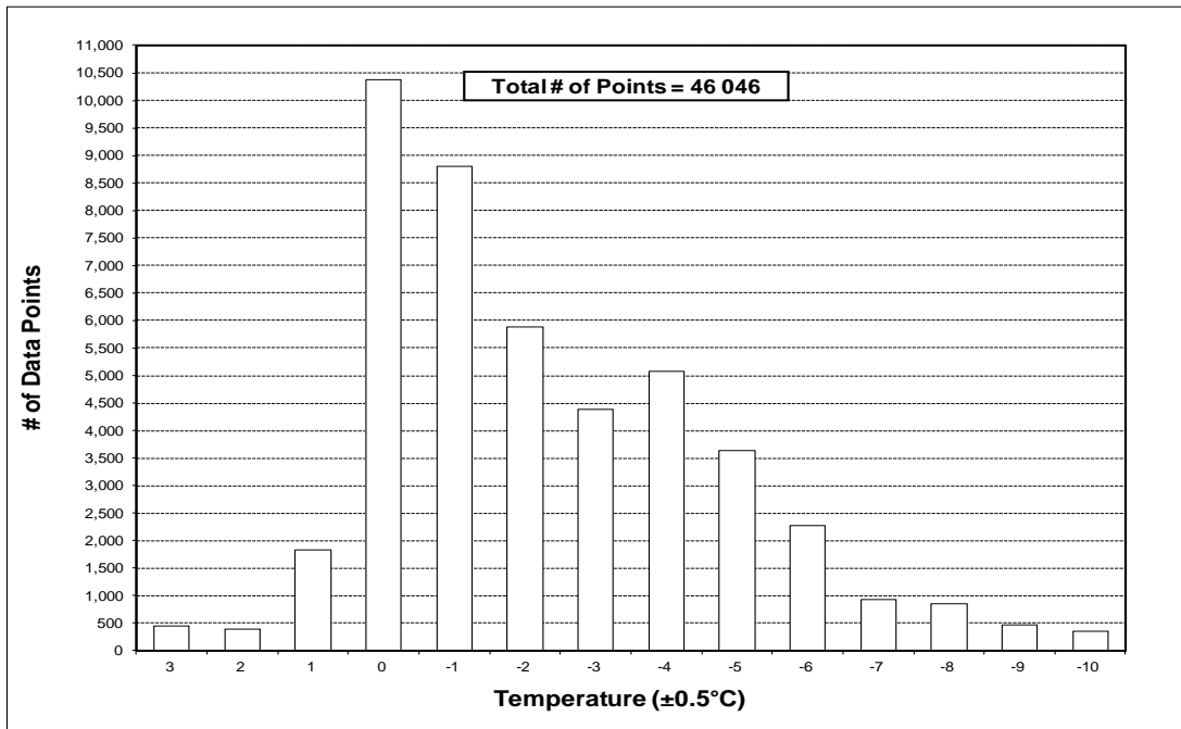
Figure 4.1: Distribution of 1996-97 to 2012-13 Freezing Rain/Drizzle Data Points by Temperature
