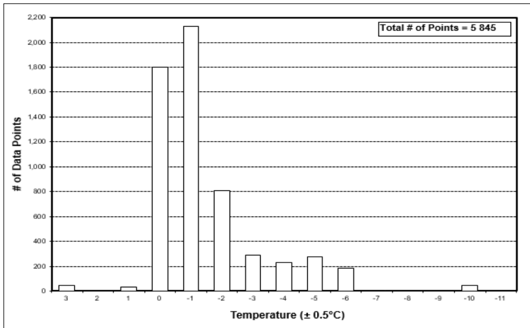
Figure 5.1: Distribution of Pure Freezing Rain/Drizzle Data Points by Temperature for Winters 2007-08 to 2010-11
