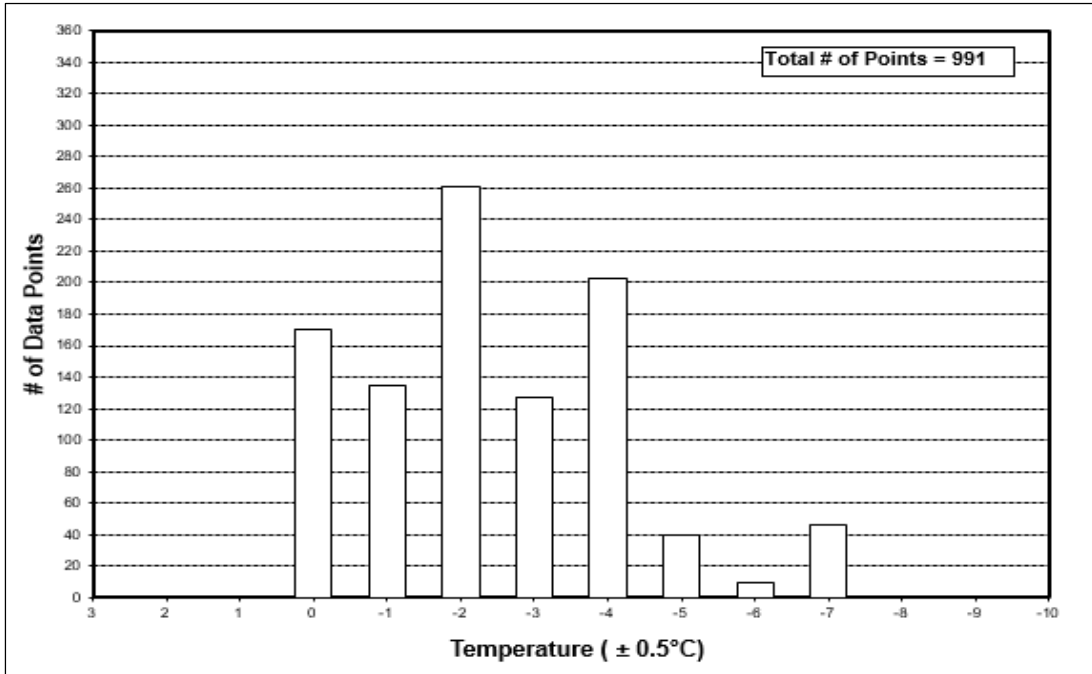
Figure 5.10: Distribution of Freezing Rain/Drizzle Mixed with Ice Pellets Data Points by Temperature for Winters 2006-07 to 2010-11
