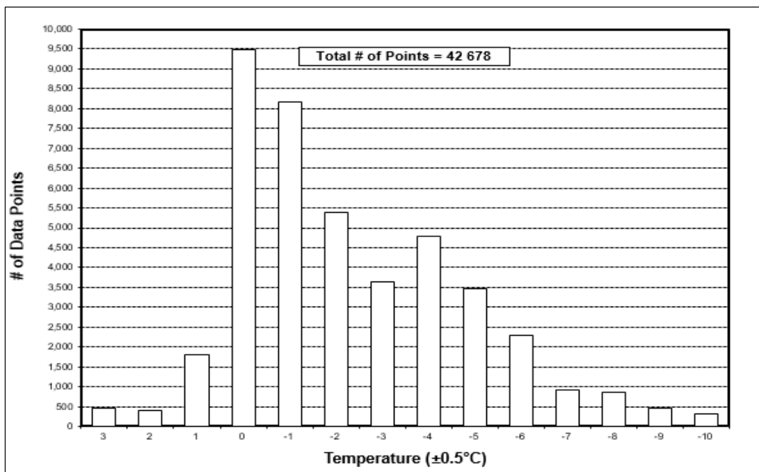
Figure 4.1: Distribution of 1996-97 to 2010-11 Freezing Rain/Drizzle Data Points by Temperature
