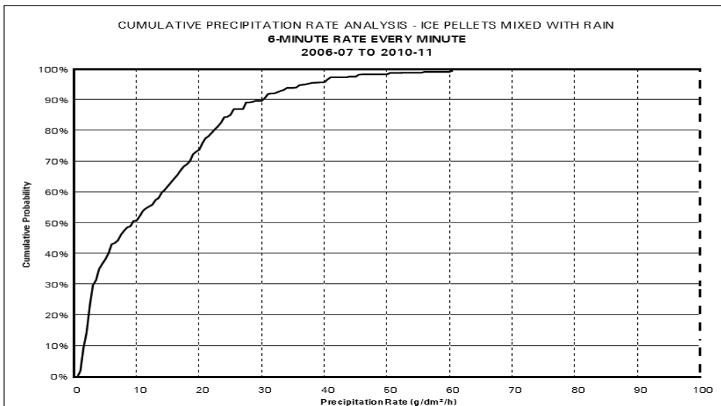
Figure 6.6: Cumulative Precipitation Rate Analysis for the Ice Pellets Mixed with Rain
