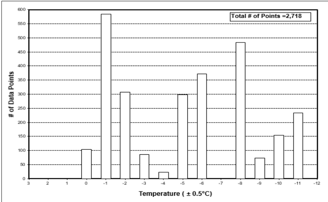
Figure 5.4: Distribution of Freezing Rain/Drizzle Mixed with Snow Data Points by Temperature for Winters 2007-08 to 2010-11
