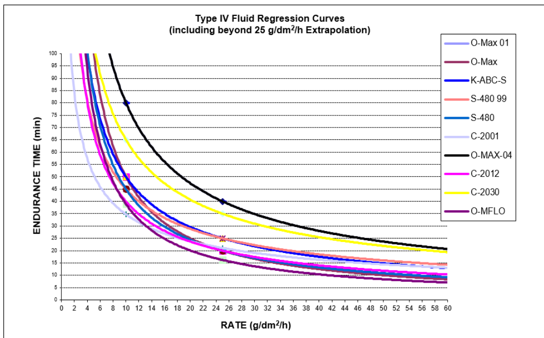
Figure 8.1: Type IV Fluid Regression Curves in Snow (Neat Fluid, -3°C to -14°C) including 25 g/dm 2 /h
