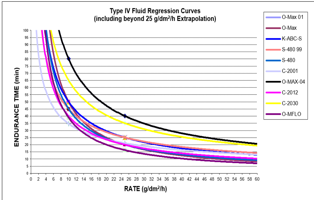
Figure 9.1: Type IV Fluid Regression Curves in Snow (Neat Fluid, -3°C to -14°C) including 25 g/dm 2 /h
