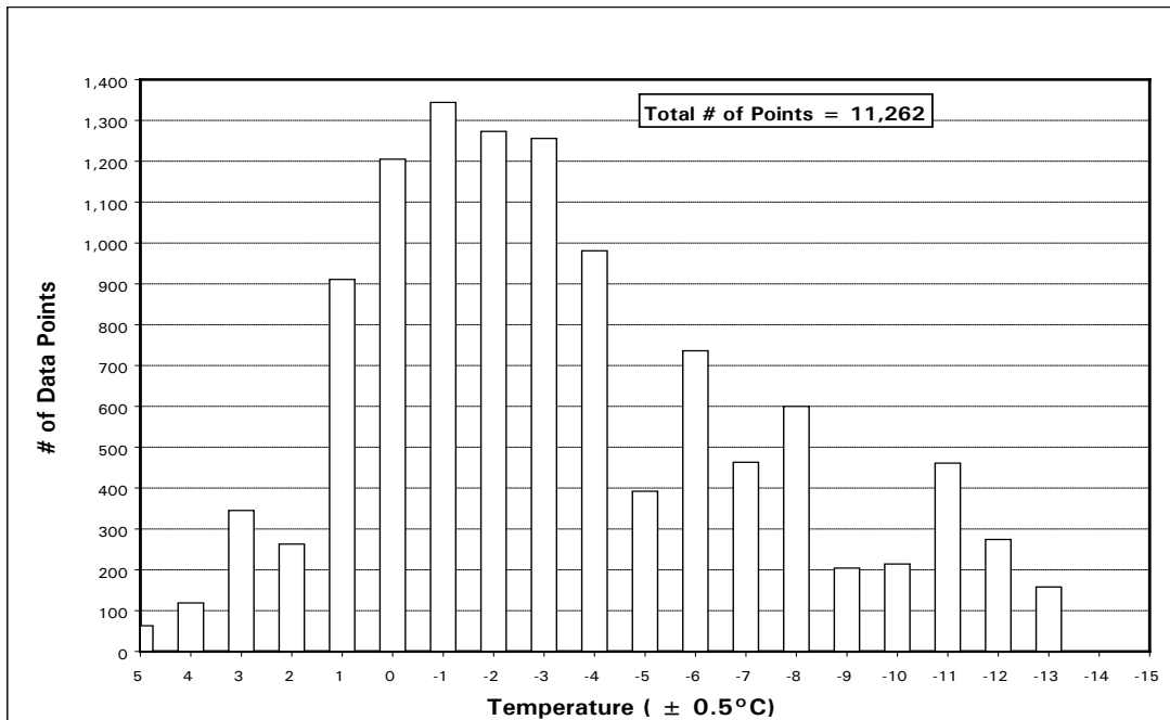
Figure 6.1: Distribution of Mixed Ice Pellets Data Points by Temperature for Winters 2004-05 to 2009-10
