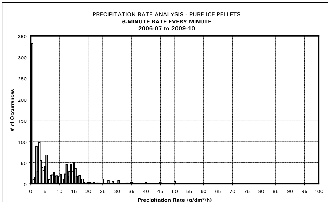
Figure 7.1: Distribution of Pure Ice Pellets Data Points by Precipitation Rate
