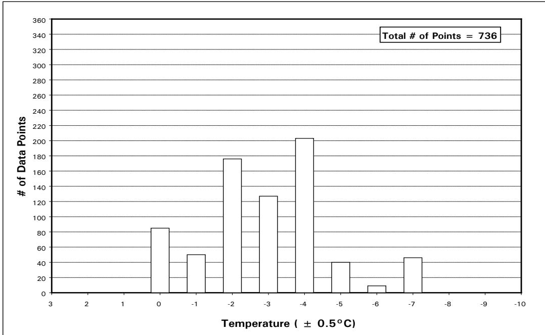
Figure 5.10: Distribution of Freezing Rain/Drizzle Mixed with Ice Pellets Data Points by Temperature for Winters 2006-07 to 2009-10
