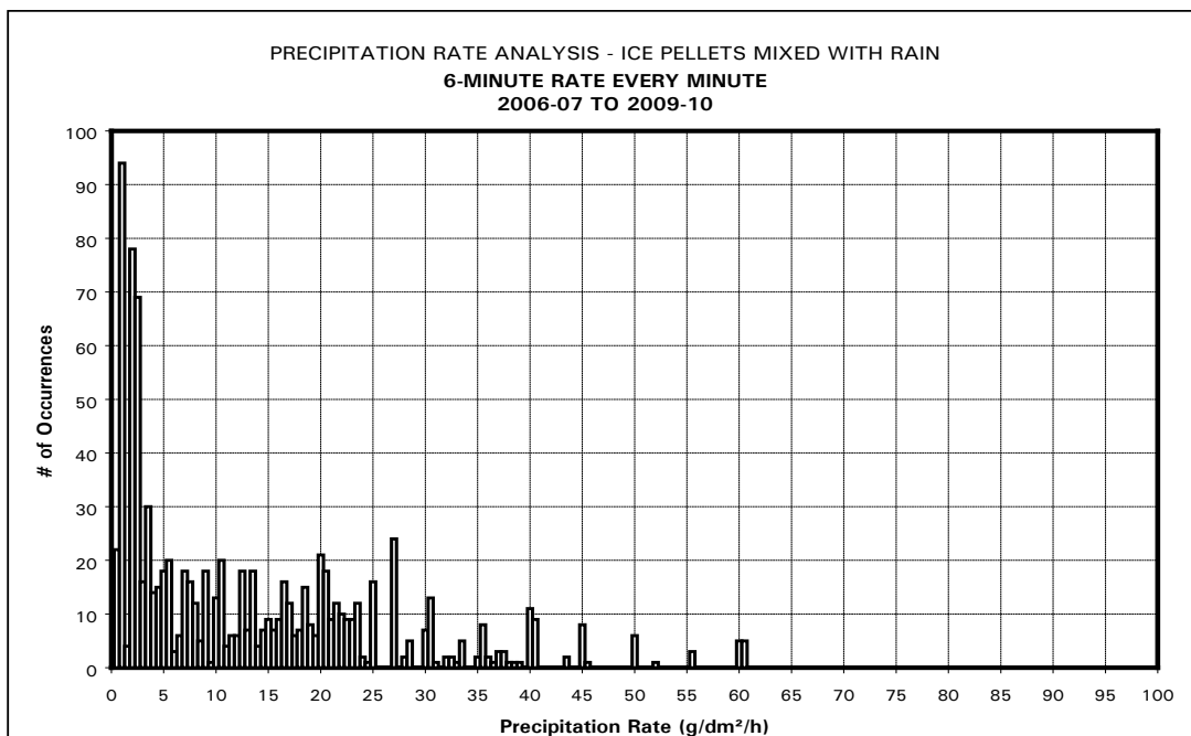
Figure 7.5: Distribution of Ice Pellets Mixed with Rain Data Points by Precipitation Rate
