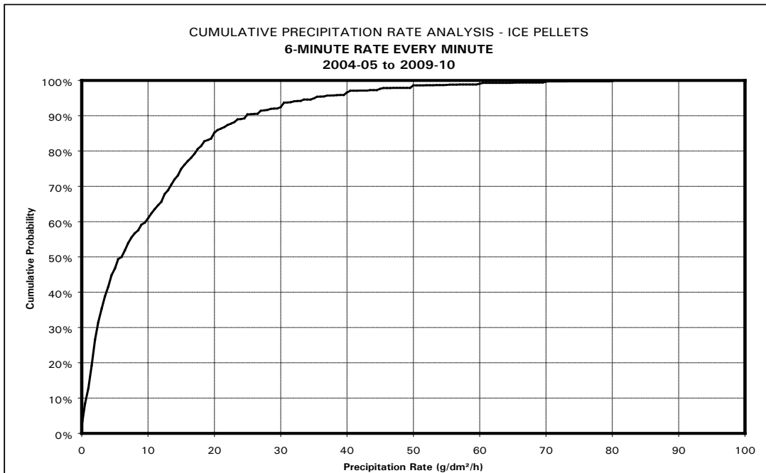
Figure 6.3: Cumulative Precipitation Rate Analysis for Mixed Ice Pellets
