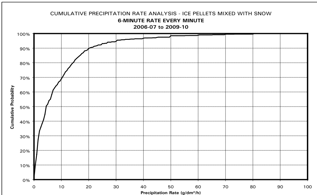
Figure 7.4: Cumulative Precipitation Rate Analysis for Ice Pellets Mixed with Snow
