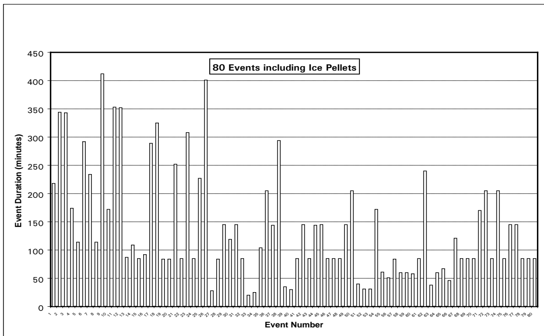
Figure 6.4: Distribution of Ice Pellet Event Duration
