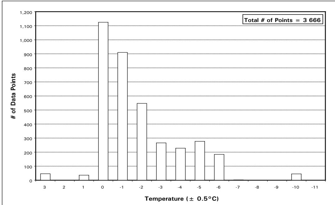
Figure 5.1: Distribution of Pure Freezing Rain/Drizzle Data Points by Temperature for Winters 2007-08 to 2009-10
