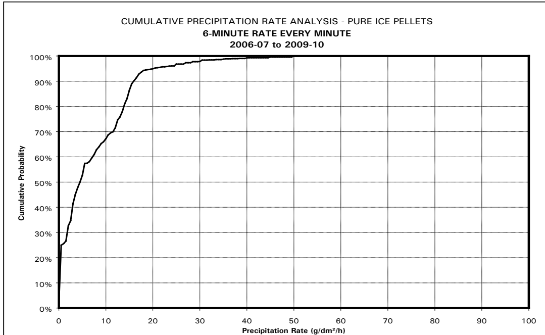
Figure 7.2: Cumulative Precipitation Rate Analysis for Pure Ice Pellets
