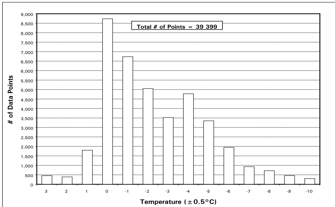
Figure 4.1: Distribution of 1996-97 to 2009-10 Freezing Rain/Drizzle Data Points by Temperature
