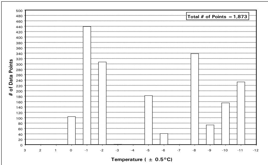
Figure 5.4: Distribution of Freezing Rain/Drizzle Mixed with Snow Data Points by Temperature for Winters 2007-08 to 2009-10
