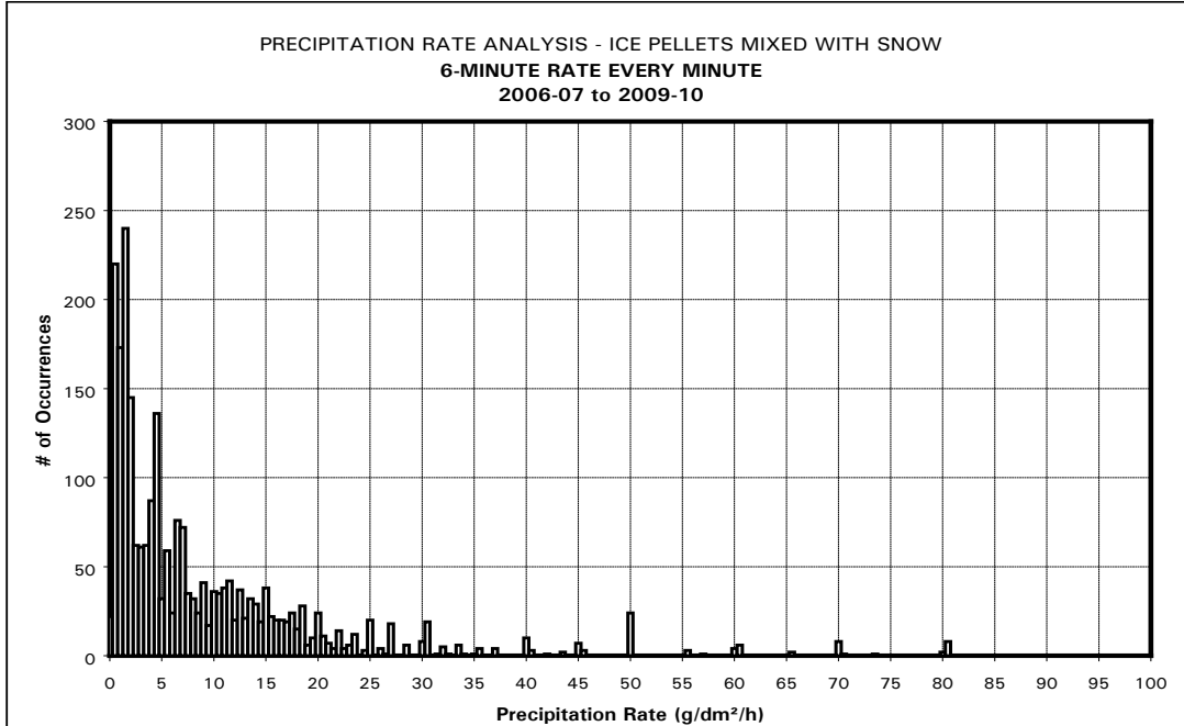
Figure 7.3: Distribution of Ice Pellets Mixed with Snow Data Points by Precipitation Rate
