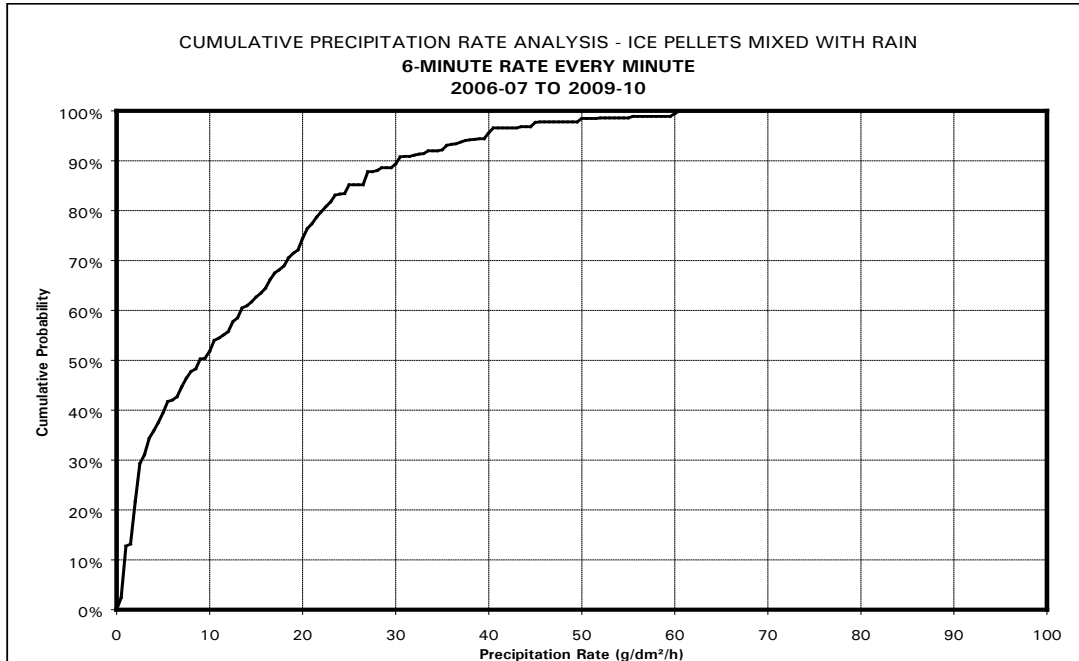
Figure 7.6: Cumulative Precipitation Rate Analysis for Ice Pellets Mixed with Rain
