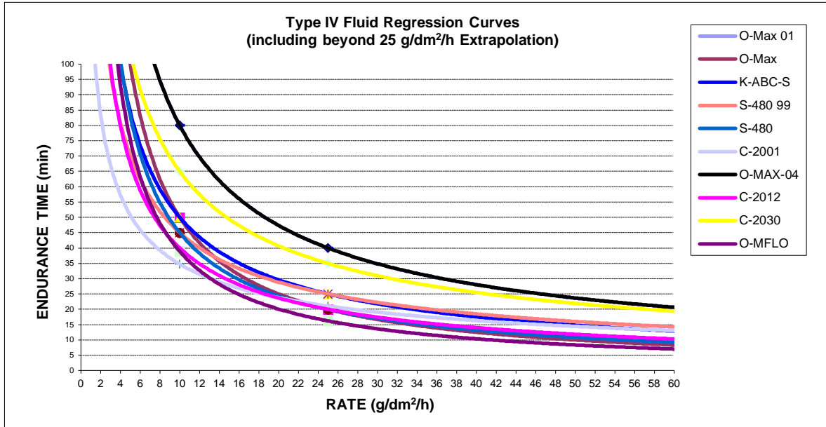
Figure 9.1: Type IV Fluid Regression Curves in Snow (Neat Fluid, -3°C to -14°C) including 25 g/dm 2 /h
