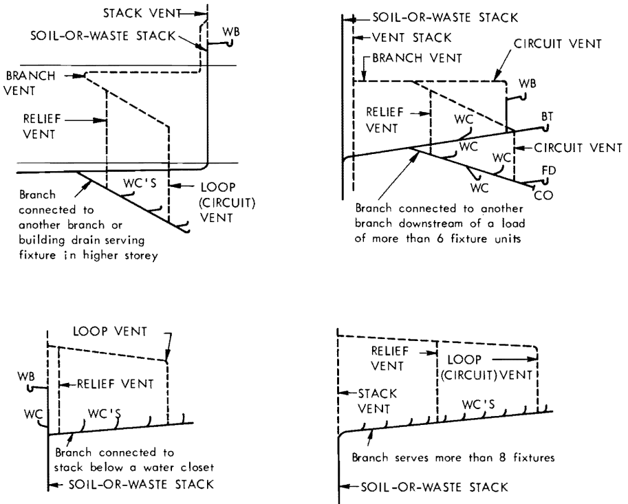
Figure 61 Relief venting
