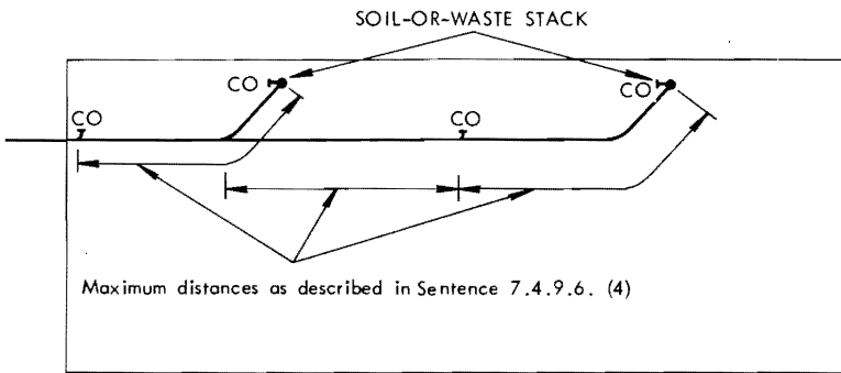
Figure 41 Spacing of cleanouts
