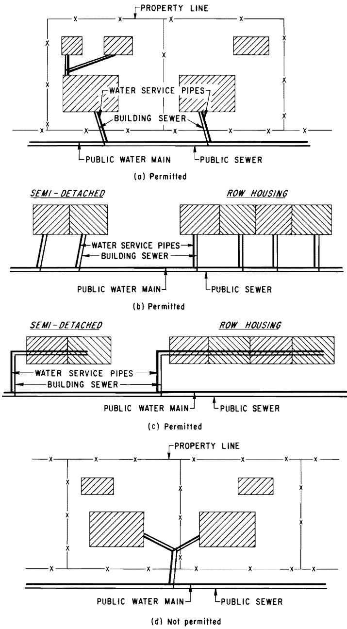
Figure 25 Service piping
