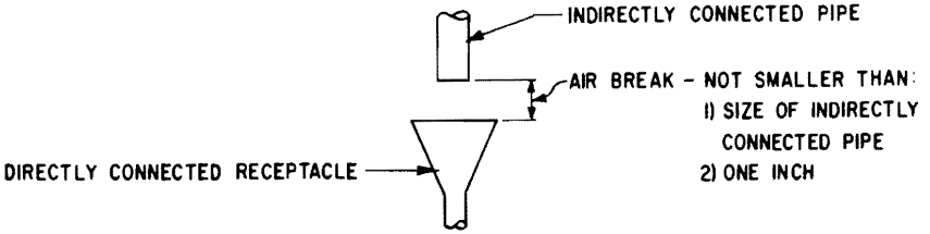
Figure 32 Air break
