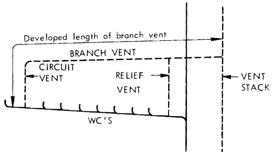
Figure 70 Developed length of branch vent
