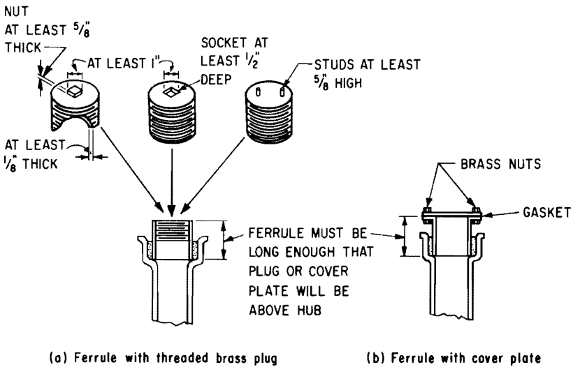
Figure 24 Cleanout ferrules
