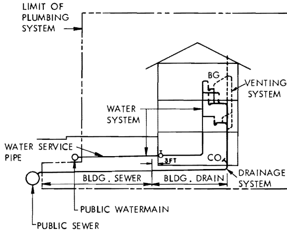
Figure 12 Plumbing system
