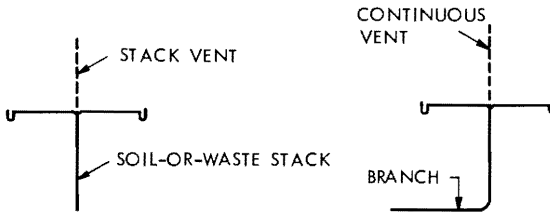
Figure 57 Dual venting
