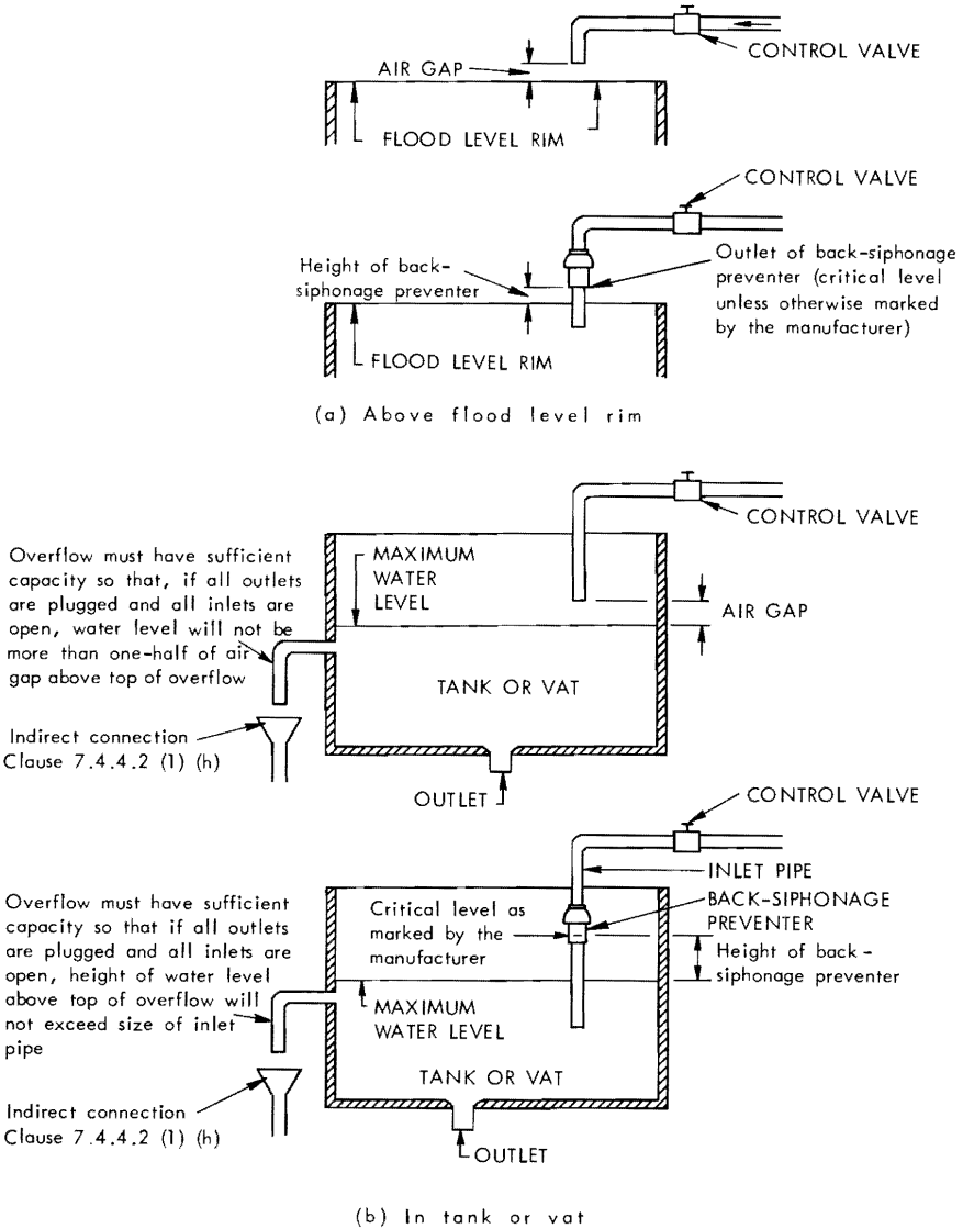
Figure 76 Installation of air gaps and back-siphonage preventers
