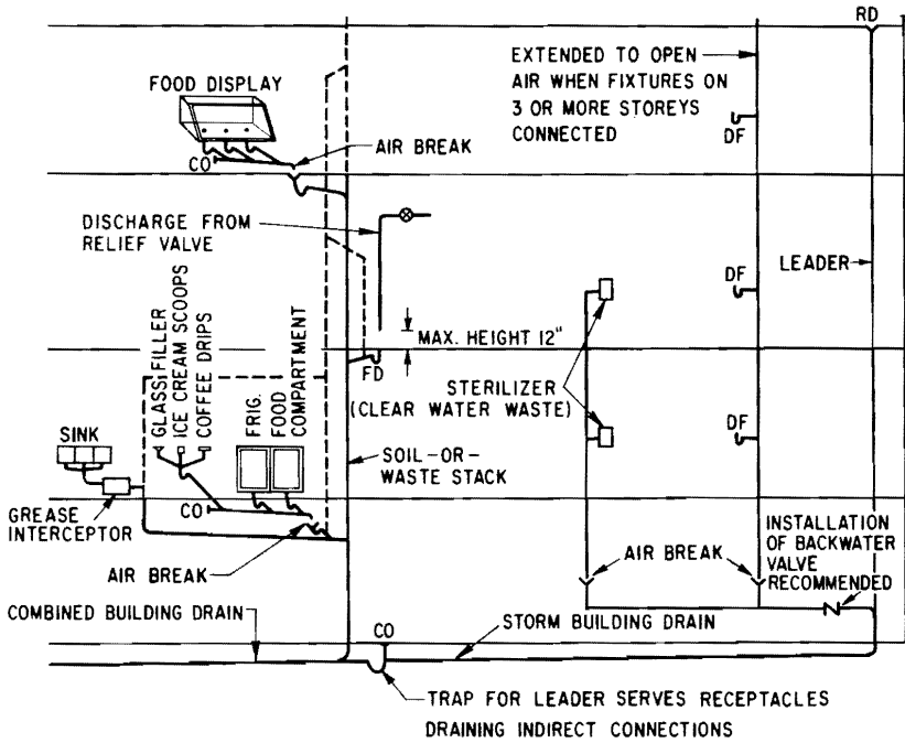
Figure 31 Indirect connections
