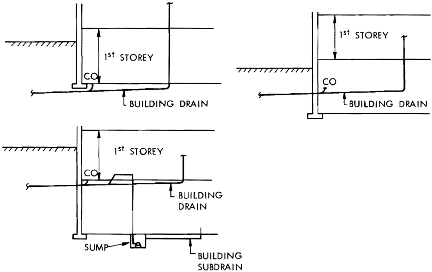
Figure 13 First storey
