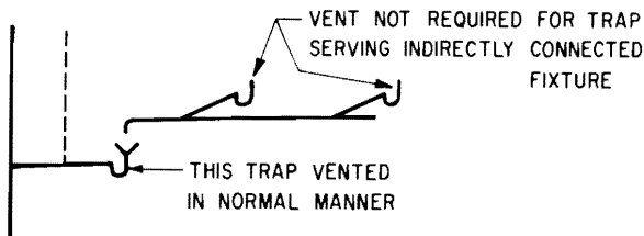
Figure 54 Trapping indirectly connected fixtures
