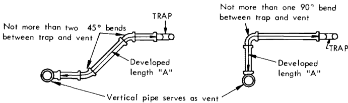
Figure 56 Vent connections
