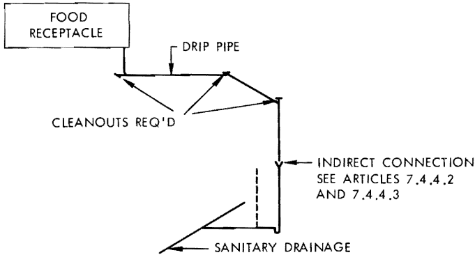
Figure 42 Cleanouts for food receptacle drip pipe
