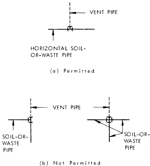
Figure 20 T fittings in drainage systems
