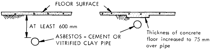
(a) Concrete floors less than 75 mm thick
