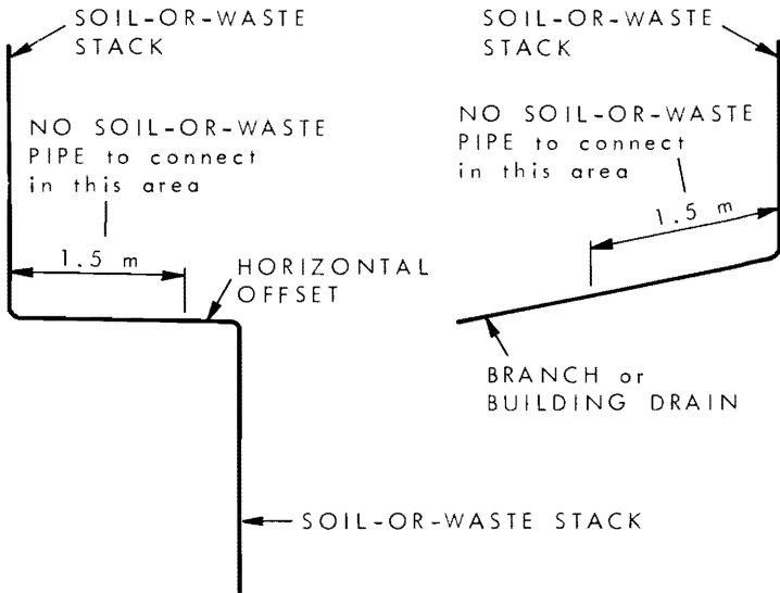
(a) Connection to nominally horizontal offset
