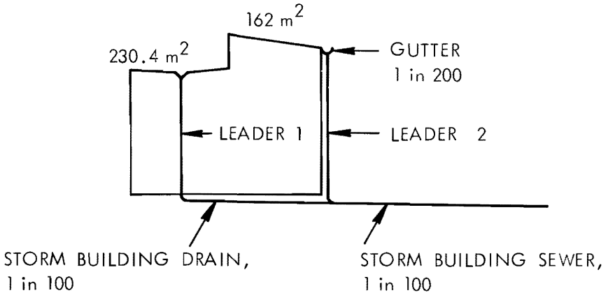
Storm Drainage Components (Example I) (Elevation View)
