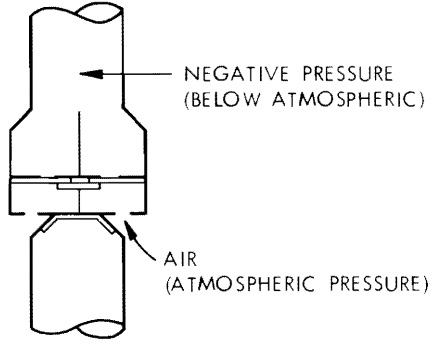
(b) No backflow - valve closed by atmospheric pressure
