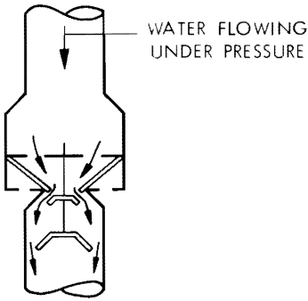
(a) Normal operation with valve open
