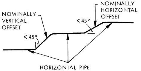
(c) Elevation view of horizontal pipe
