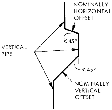
(a) Elevation view of vertical pipe
