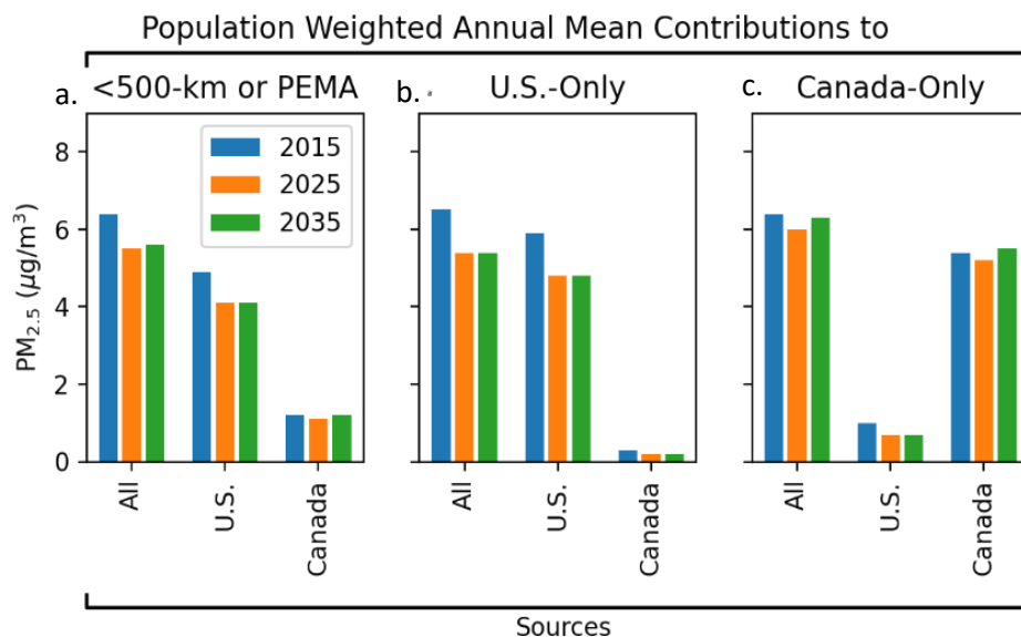
Figure 4-13. ECCC modeled population weighted annual mean PM 2.5 contributions (µg/m 3 ) from sources (All, Canada, U.S.) to populations within 500-km or PEMA states, the U.S. portion, or the Canadian portion.
