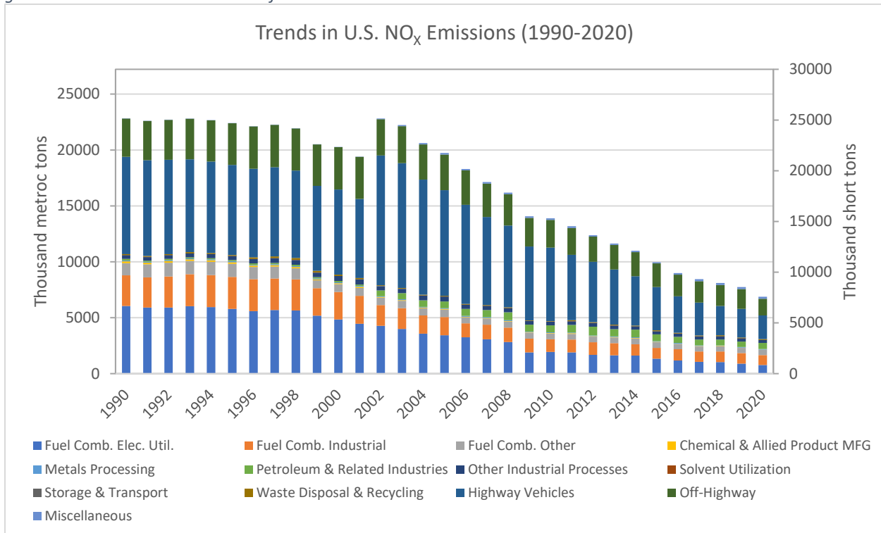
Figure 2-4. U.S. NO x emission trends for 1990-2020.
