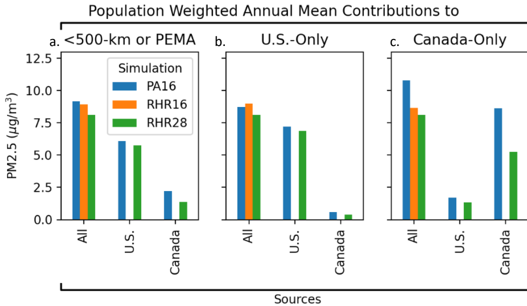
Figure 4-14. U.S. EPA modeled population weighted annual mean PM 2.5 contributions (µg/m 3 ) from sources (All, Canada, U.S.) to populations within 500-km or PEMA states, the U.S. portion, or the Canadian portion.
