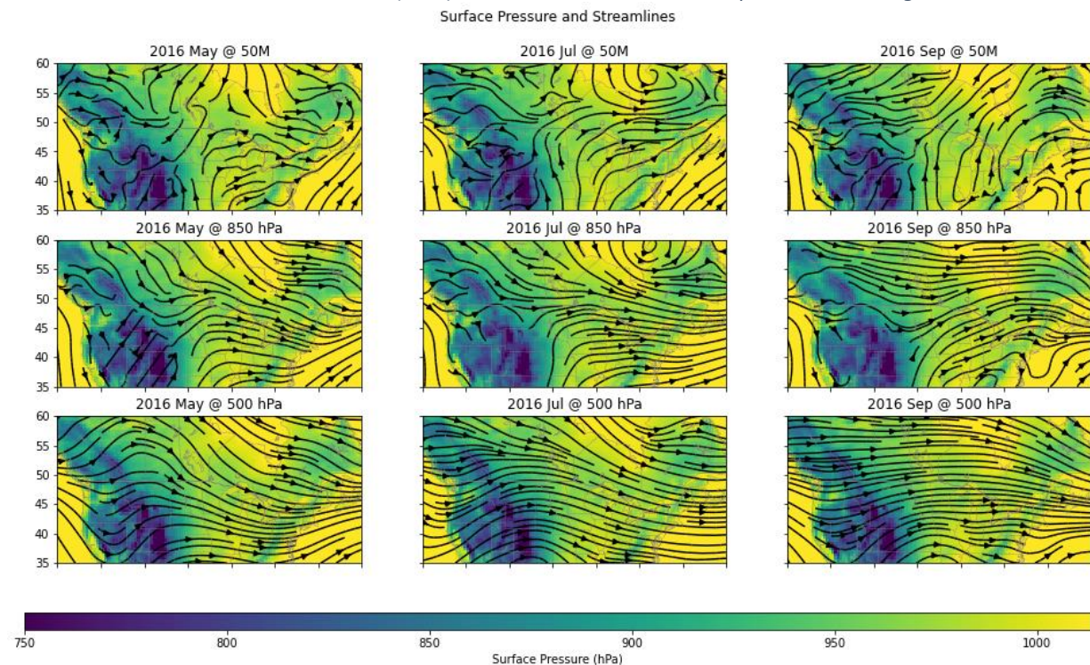
Figure B-1. MERRA-2 monthly average surface pressures and wind fields are shown for May, July, and September of 2016. The winds are shown at 50-meters (50M), 850 hPa and 500 hPa that represent increasing altitude.
