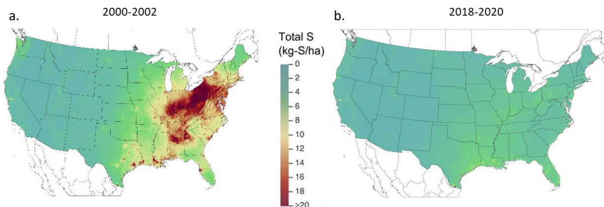
Figure 2-7. Three-year average of total sulfur deposition in the U.S. for (a) 2000-2002 and (b) 2018-2020 7 .
