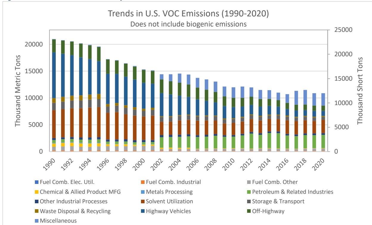
Figure 3-3. U.S. VOC emission trends for 1990-2020.
