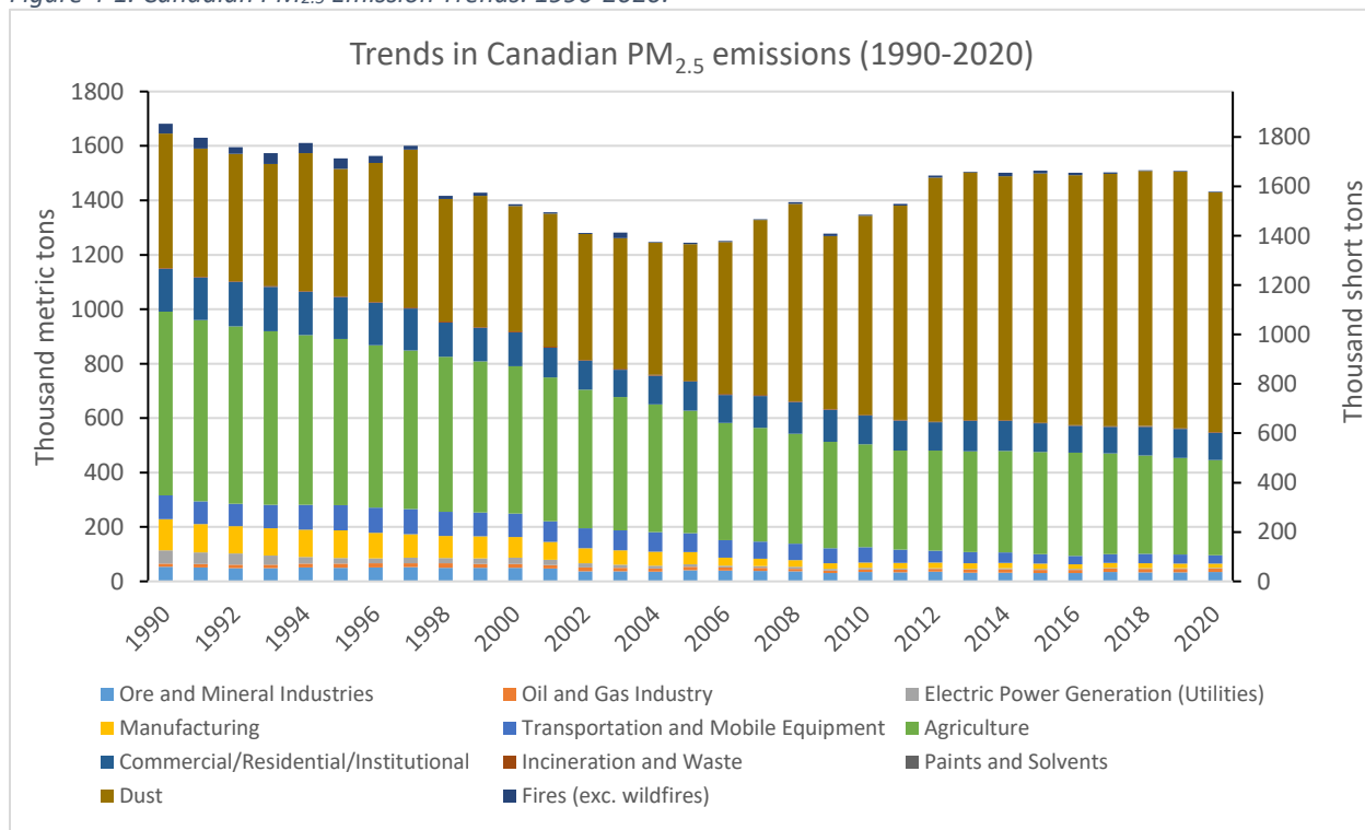
Figure 4-1. Canadian PM 2.5 Emission Trends. 1990-2020.
