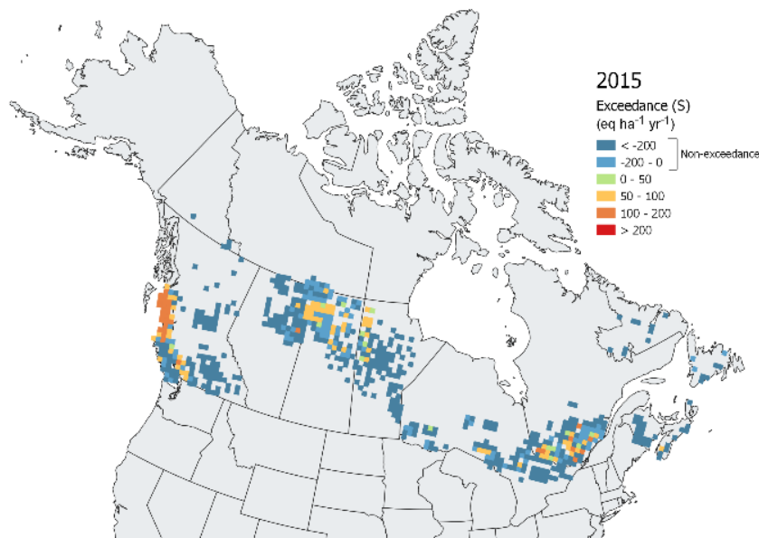
Figure 2-12. Mapped lake exceedance under GEM-MACH modeled deposition for (a) baseline 2015 and (b) BAU 2035, with changes to the exceedance shown in (c). Lake critical loads of acidity were estimated with the SSWC model using sulfur deposition only. Values above 0 are considered in exceedance of their critical loads. Critical loads were summed to the 5 th percentile, to provide protection for 95% of the ecosystems in each 42 km grid (Jeffries et al., 2010).
