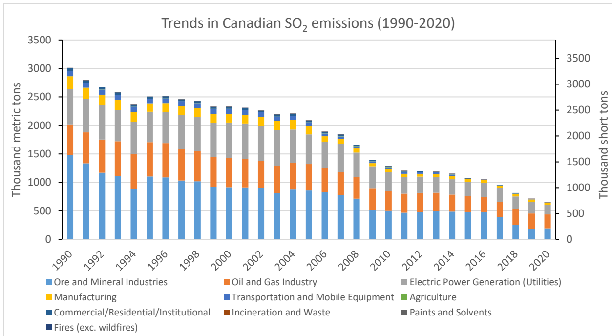
Figure 2-1. Canadian SO 2 emission trends for 1990-2020.
