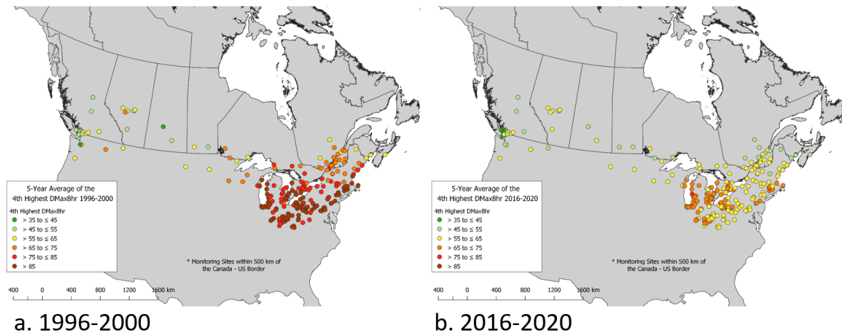
Figure 3-5. Ozone concentrations (five-year average of the annual 4 th highest MDA8 ozone concentration) along the Canada-U.S. border for (a) 1996-2000 and (b) 2016-2020.
