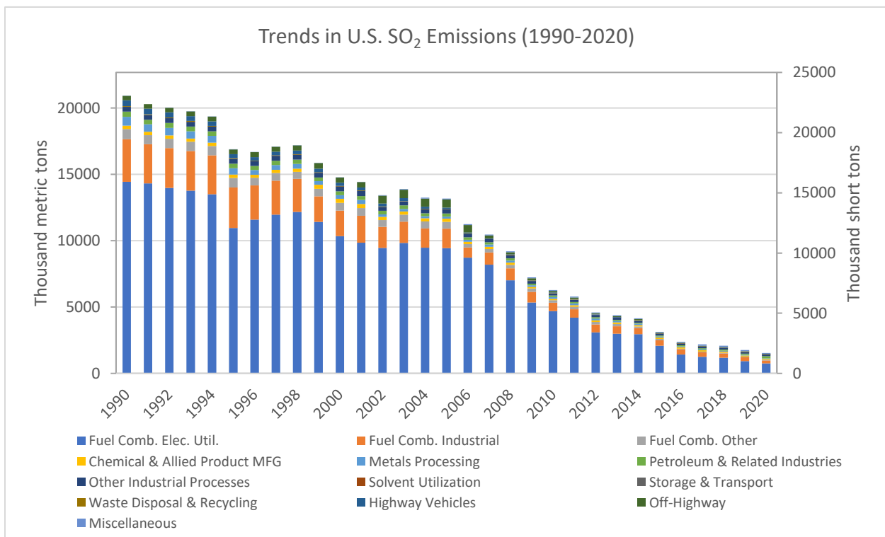
Figure 2-3. U.S. SO 2 emission trends for 1990-2020.
