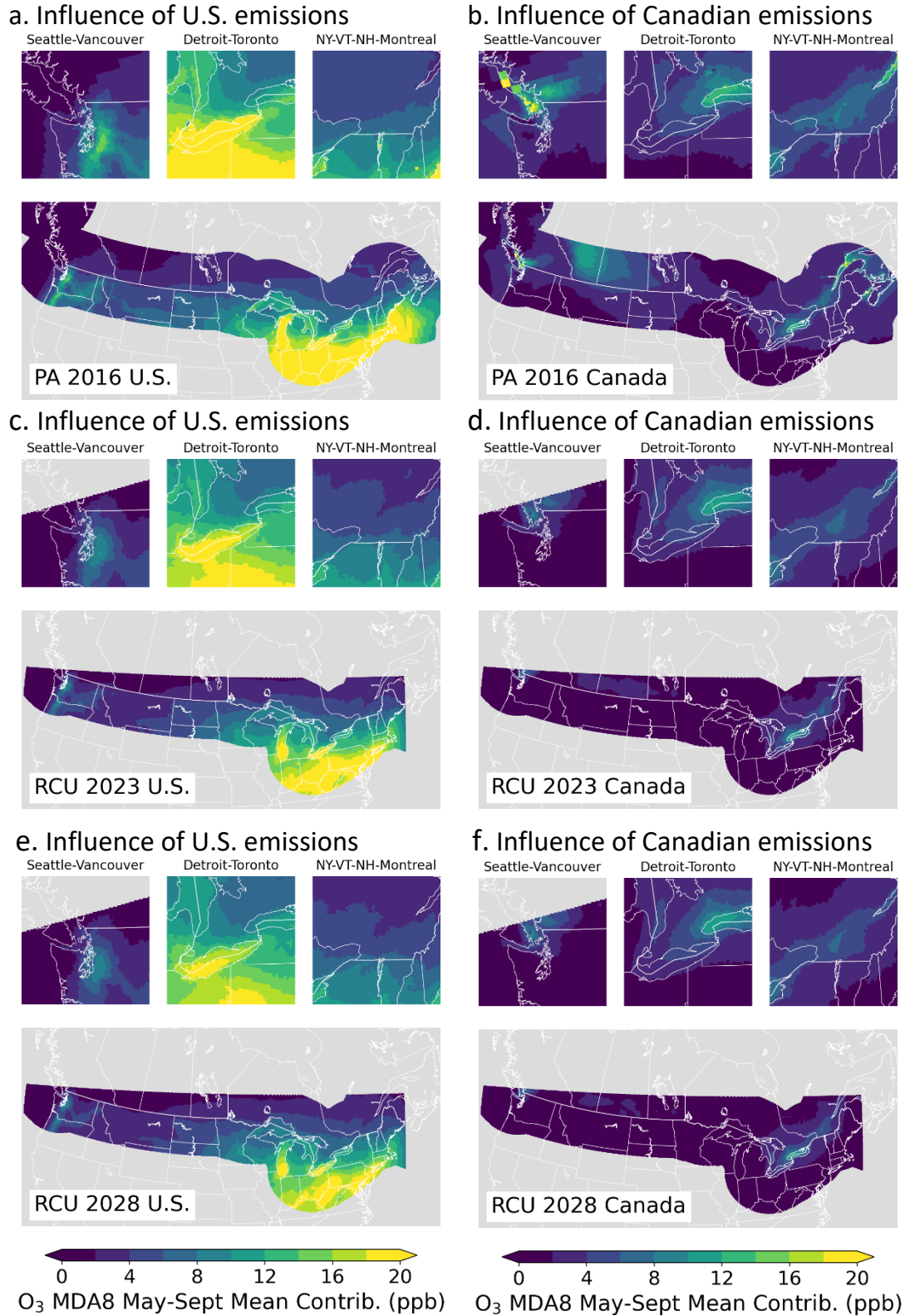
Figure 3-10. Attribution of ozone for PA16 from (a) U.S. emissions and (b) Canadian emissions; for RCU23 from (c) U.S. emissions and (d) Canadian emissions; and for RCU28 from (e) U.S. emissions and (f) Canadian emissions. All results are MDA8 ozone concentrations averaged from May-Sept.
