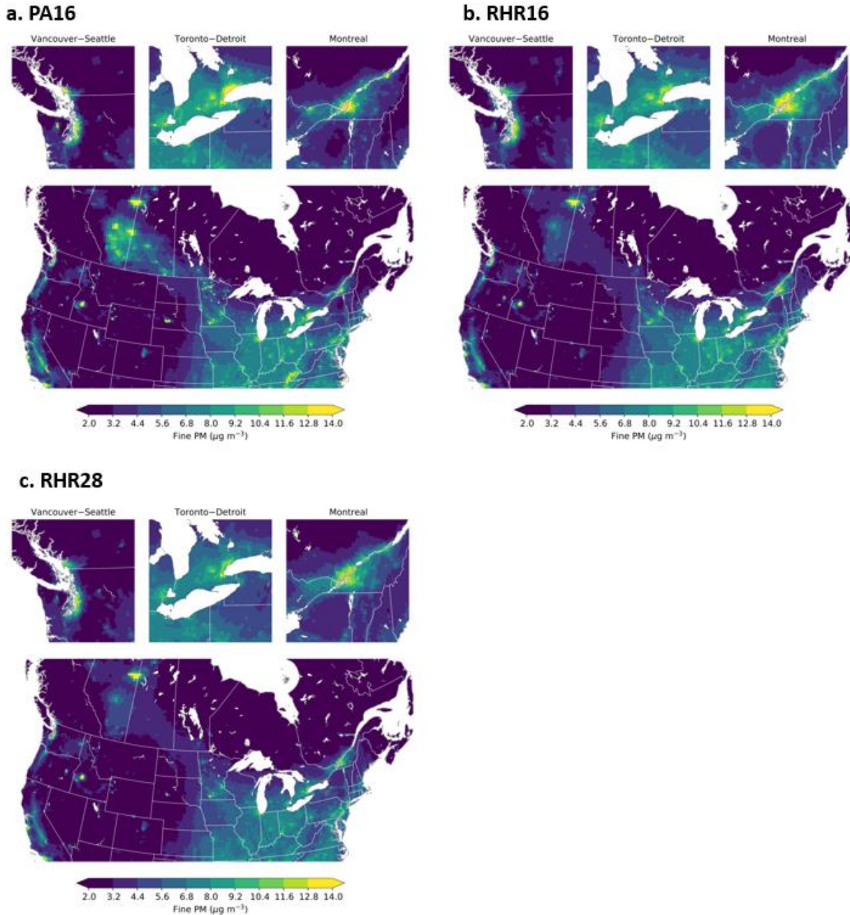
Figure 4-8. Annual average PM_{2.5} concentrations from U.S. EPA modeling scenarios for the base year (a) PA16 and (b) RHR16, and for future projections (c) RHR28.
