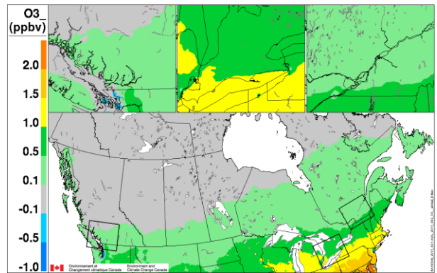
d. BASE – U.S. 20% reduc. 2015
