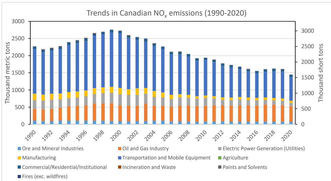
Figure 2-2. Canadian NO x emission trends for 1990-2020.
