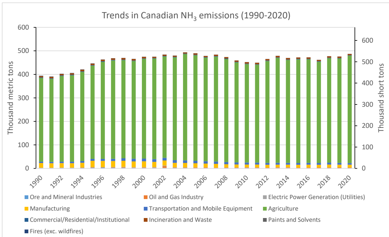
Figure 4-2. Canadian NH 3 Emission Trends. 1990-2020.
