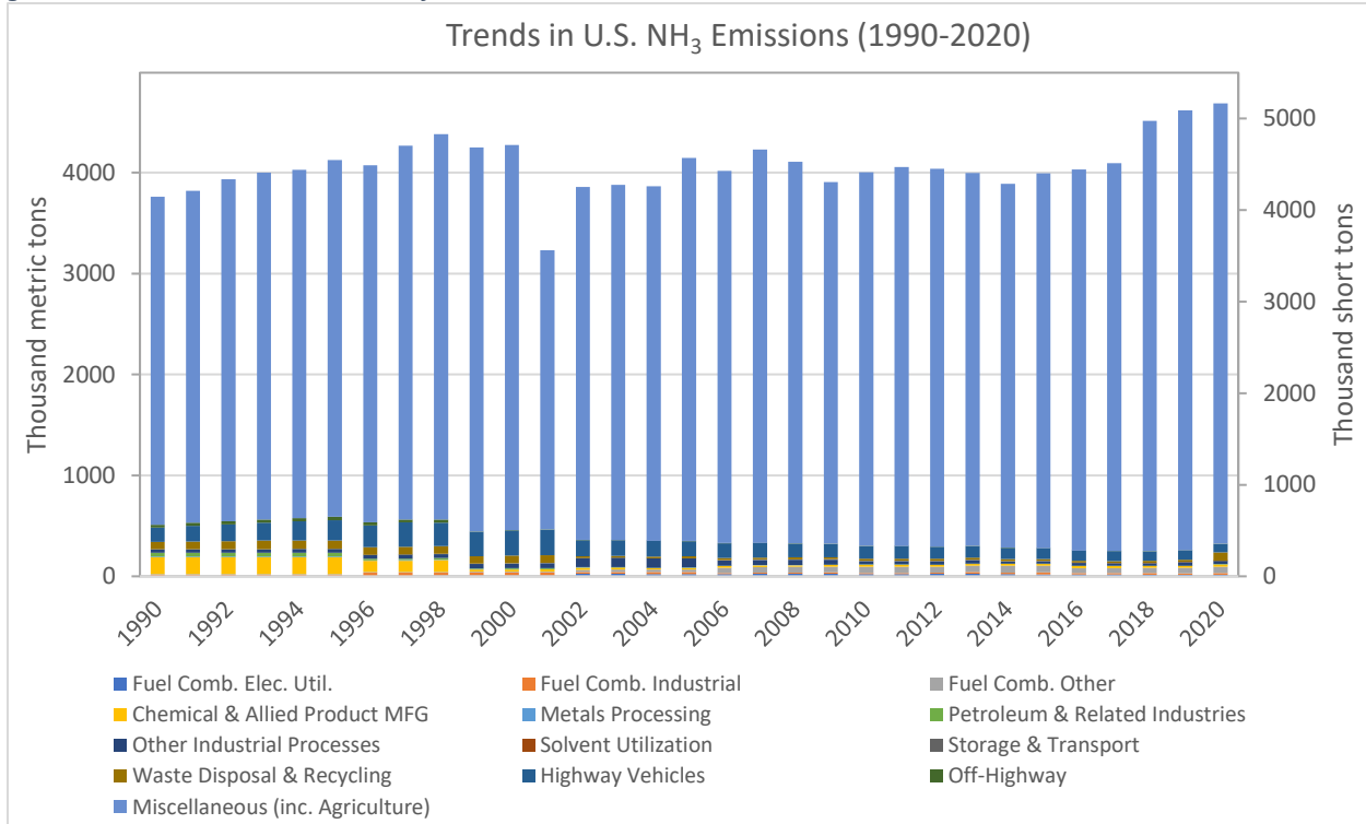
Figure 4-4. U.S. NH 3 emission trends from 1990-2020.
