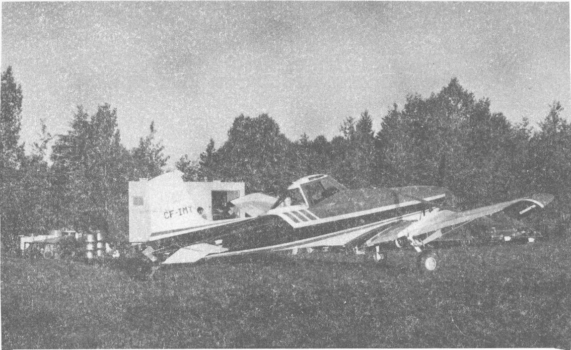
Figure 2. Cessna Agtruck with Micronair AU3000 spray atomizers.
