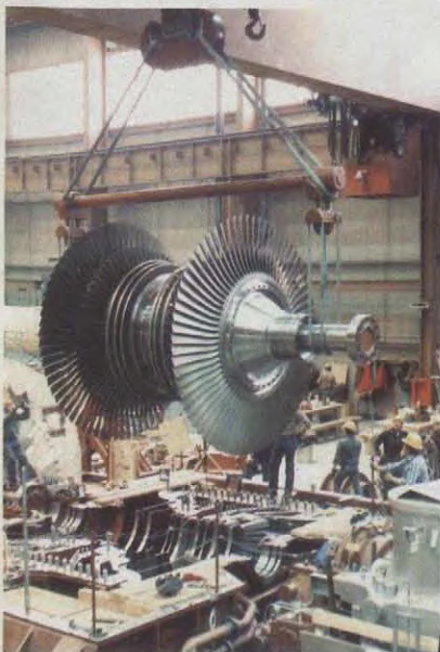
L.P. Spindle during erection at Atikokan Generating Station – Ontario Hydro
