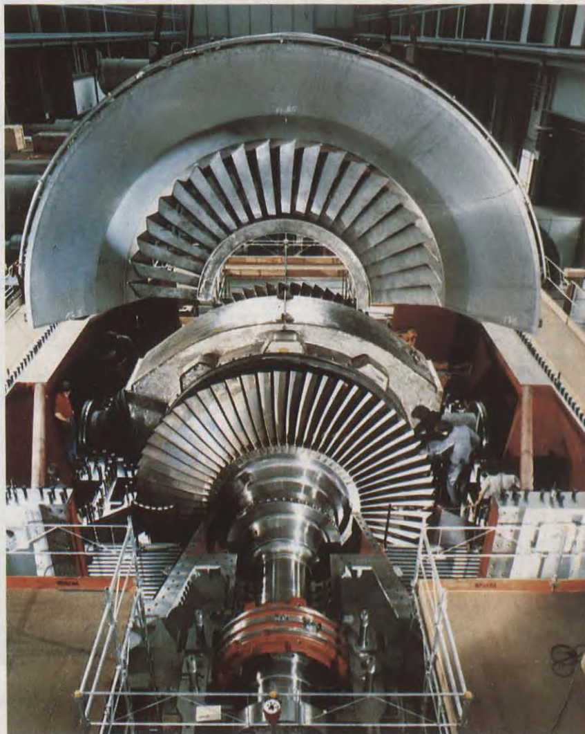
Assembly of L.P. Turbine
