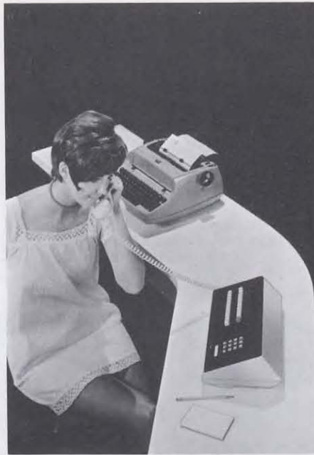
Canadian-developed electronic private automatic branch exchange (PABX) uses pulse amplitude modulation method of time-division multiplexing and has solid-state reliability and complete flexibility of services in the up-to-80 line class.
