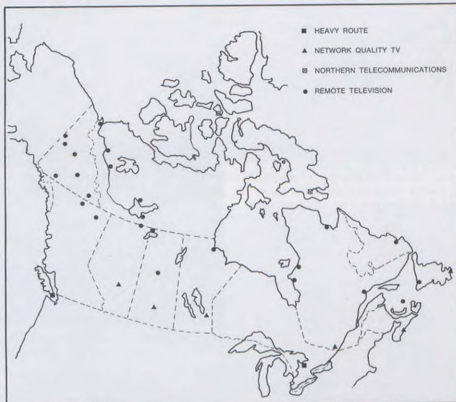
Map of Canada shows locations of the initial ground relay stations for the Canadian domestic satellite communications network — the world's first (a total of 37 stations were operating by December, 1973).
