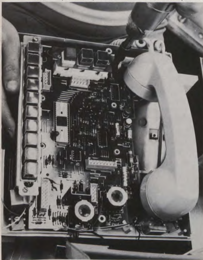
Final assembly on a telephone terminal for business systems.
