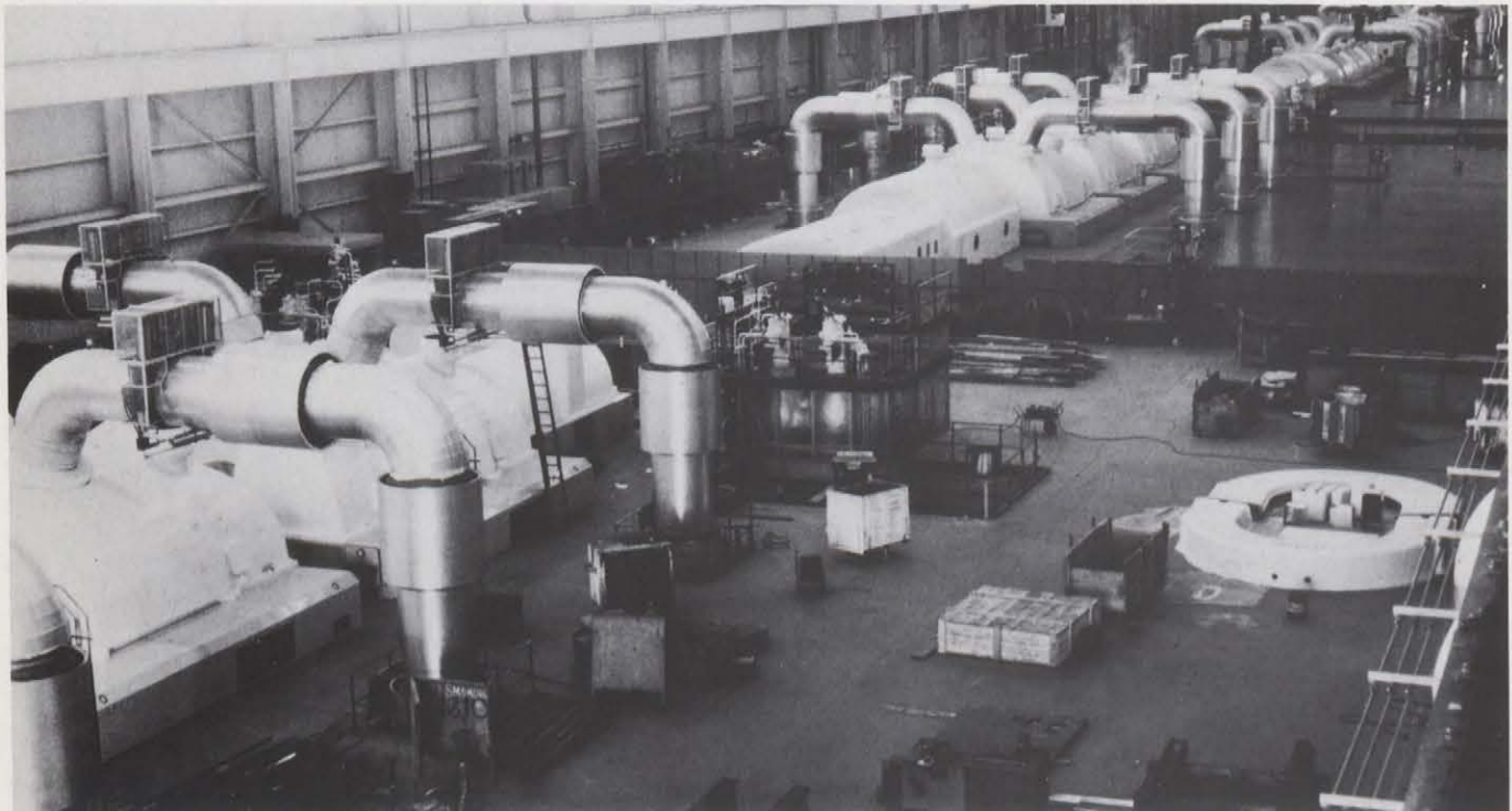
Turbogenerator hall, Pickering nuclear station. Unit in foreground is in final stages of erection.
