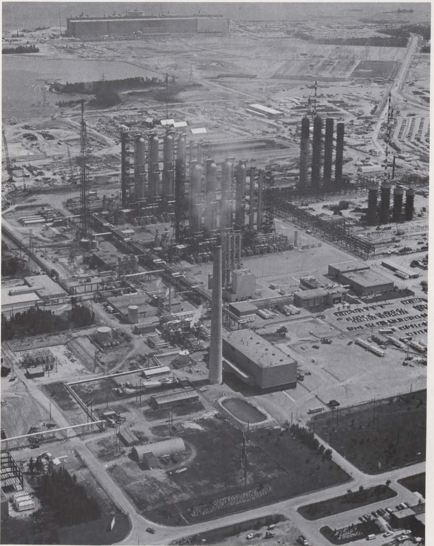
In left foreground is the 200 MW Douglas Point Nuclear Station. Center is a heavy water extraction plant. In the background can be seen the 3200 MW Bruce Nuclear Generating Station currently under construction on the shore of Lake Huron, Canada.
