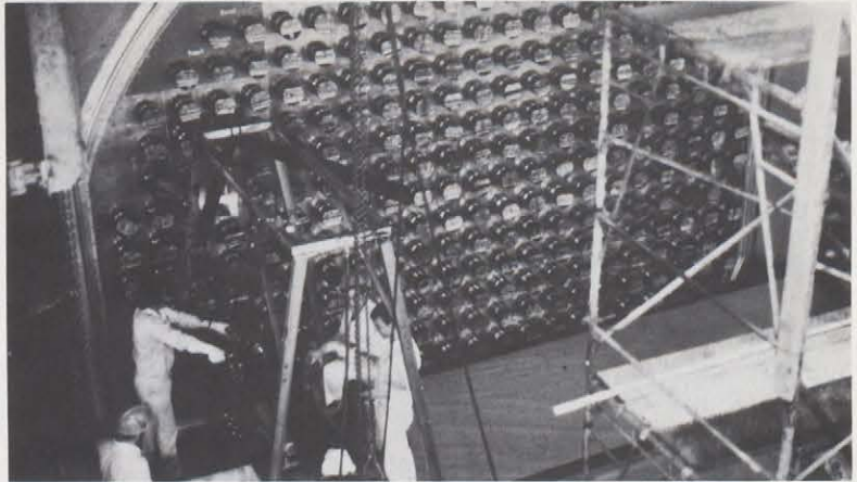
Hand loading of initial fuel charge into a nuclear reactor vessel at the nuclear power generating station, Pickering, Ontario, Canada.
