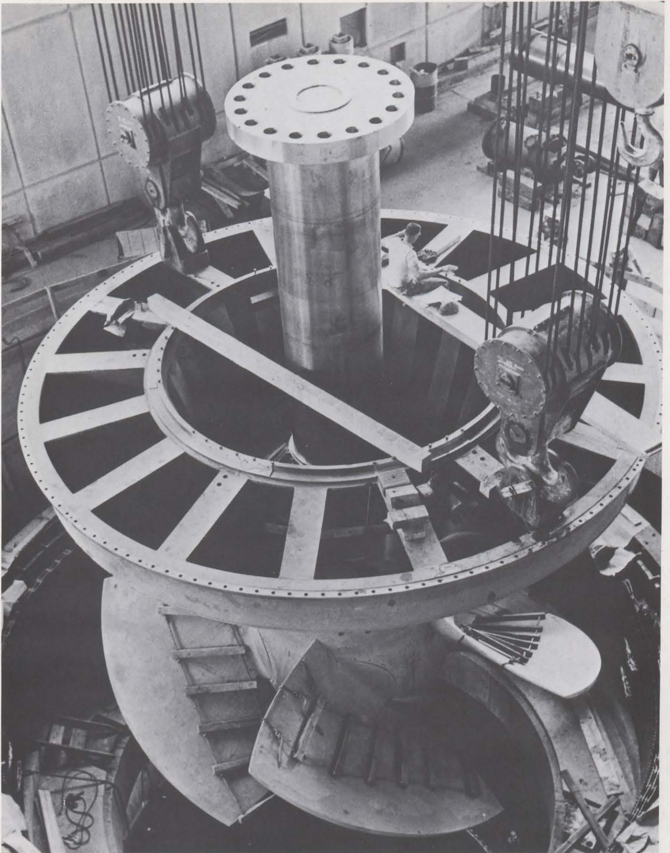
A Canadian-designed and fabricated turbine runner, typical of those supplied throughout the world, is lowered into its working position.
