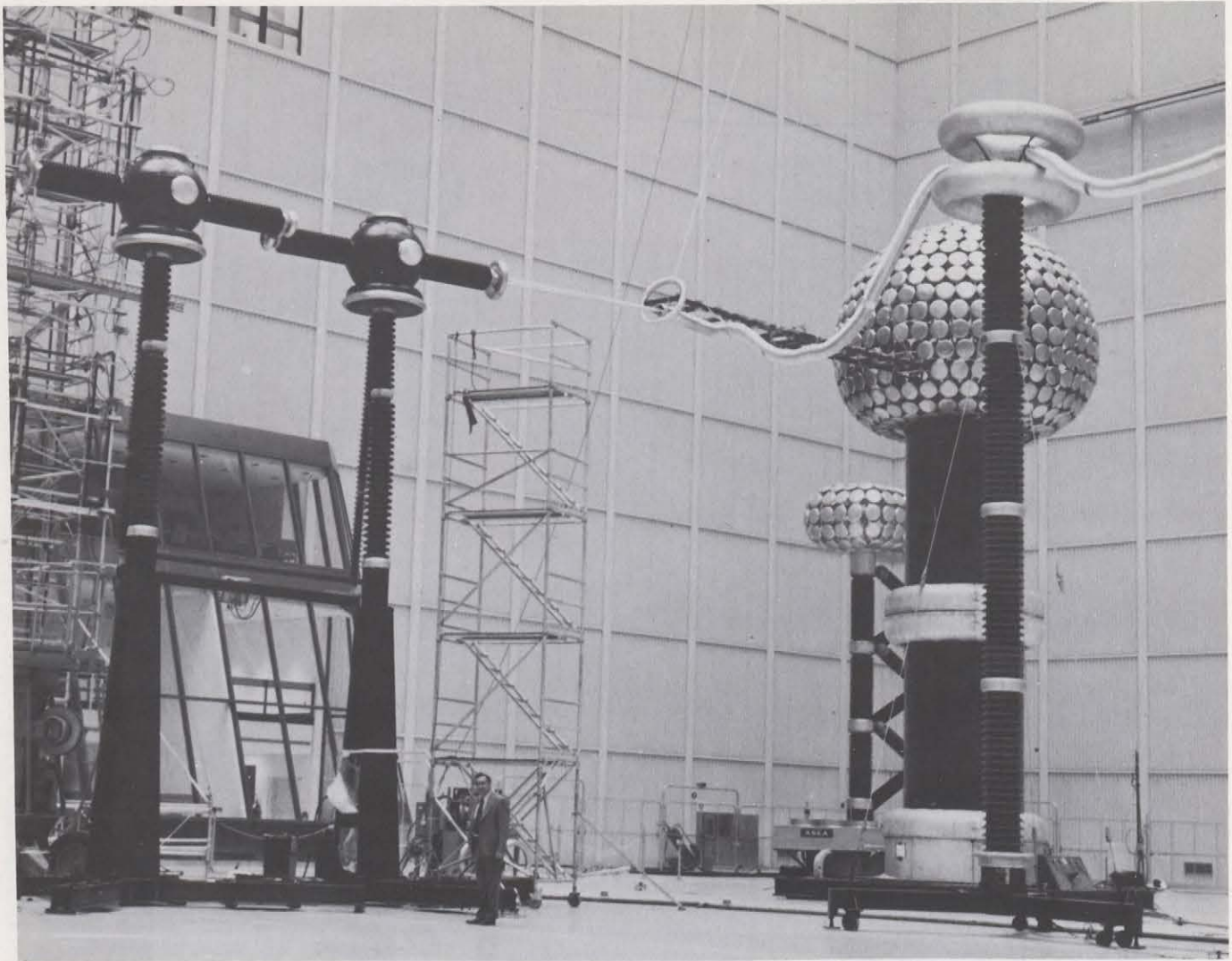
Canadian-developed EHV airblast circuit breakers being tested at the Hydro Quebec Research Centre.
