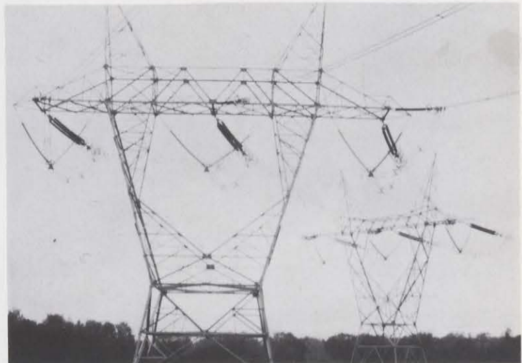
Canada has accumulated several years of successful 735 kV transmission experience on lines such as these.
