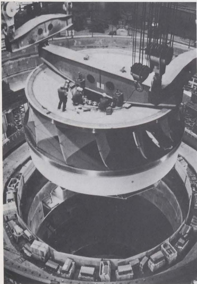
Francis type runner being lowered into position in a Canadian-designed turbine with a demonstrated capacity in excess of one million horsepower. The unit is located at the Grand Coulee Project on the Columbia River in the United States.
