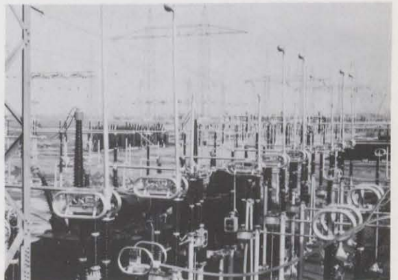
735 kV switching yard at Hydro Quebec Research Centre.
