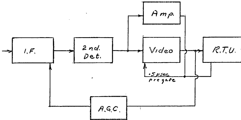
Figure 1 - Pre-gating Circuit.
