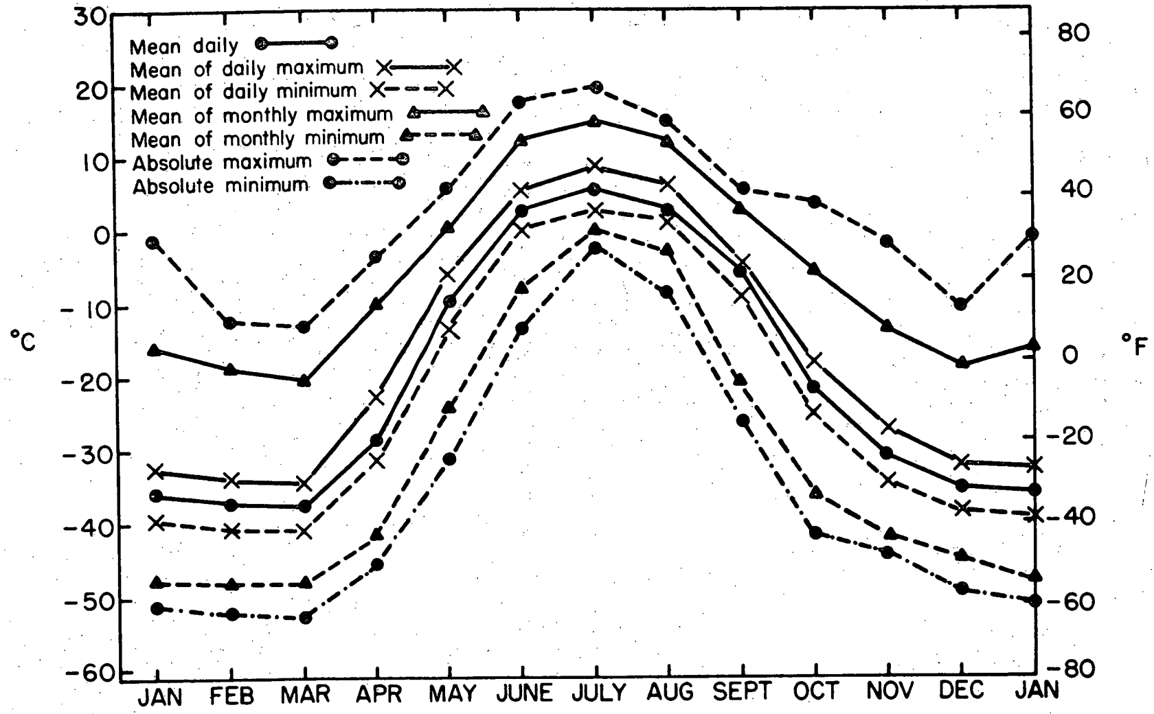
Fig. 2: Temperature Variations for Alert 1931-60.
