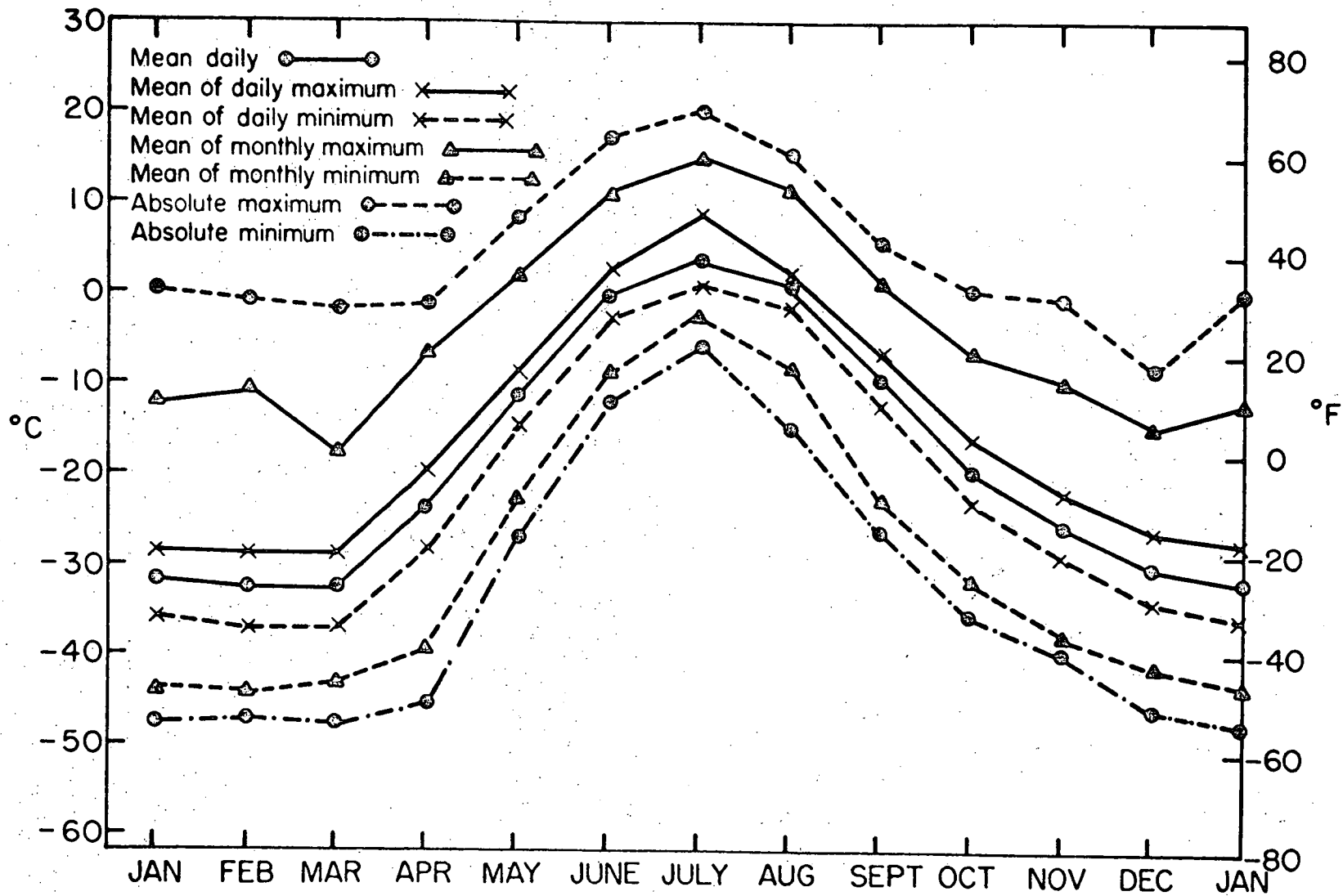
Fig. 1: Temperature Variations for Eureka 1931-60.
