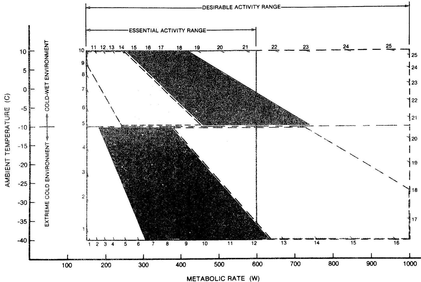
Figure 2. Predicted prototype clothing capabilities. The densely-shaded regions indicated the range of metabolic rates and ambient temperatures for which the prototype clothing system can provide appropriate and easily changed levels of thermal insulation. The lightly-shaded regions indicate levels of thermal resistance which the clothing can provide although changes in the clothing configuration are less convenient. These results assume no ventilation or sweating.
