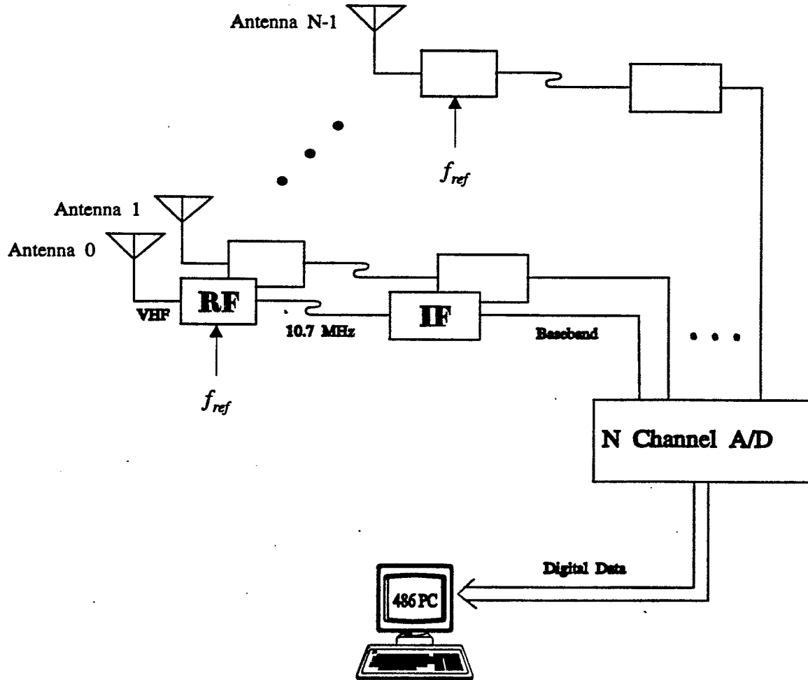
Figure 1: Experimental N channel DF system block diagram.
