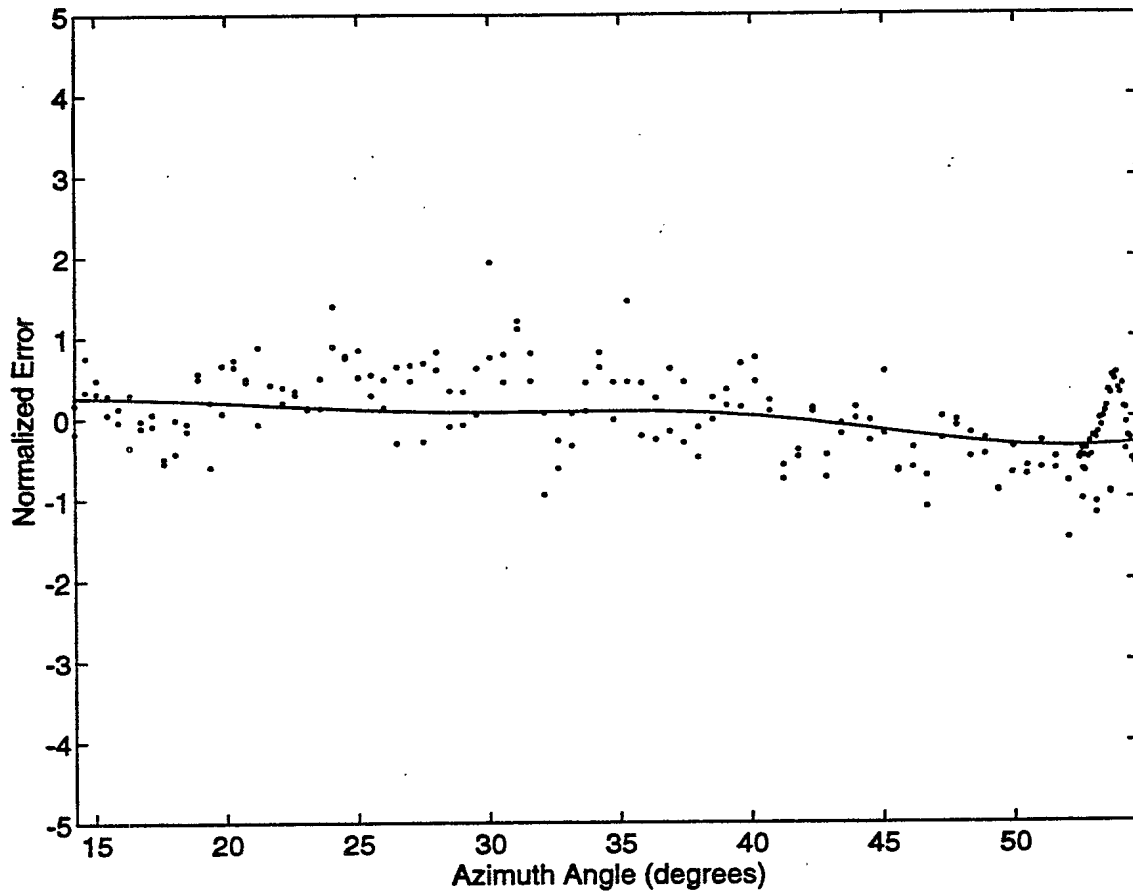
Figure 34: Revised error results for November 6, 1992. The dots represent actual error and the solid line represents predicted error due to mutual coupling.
