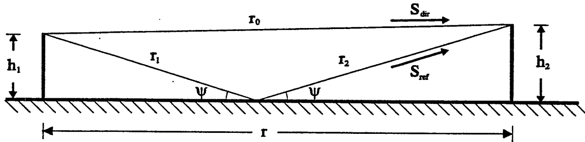
Figure 13: Plane Earth propagation model.
