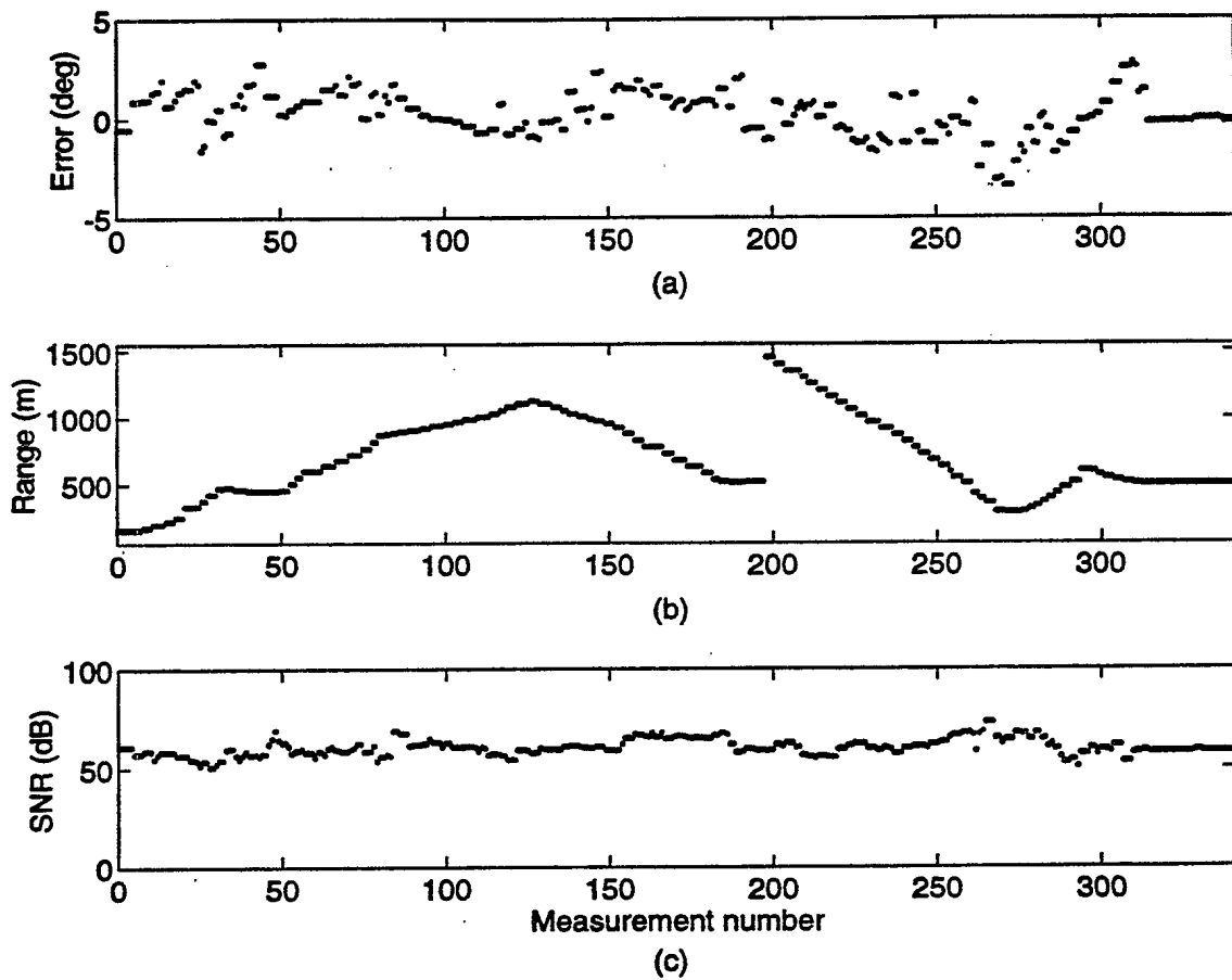
Figure 31: Field trial parameters for March 25, 1993: (a) broadside normalized error, (b) range, and (c) signal to noise ratio.
