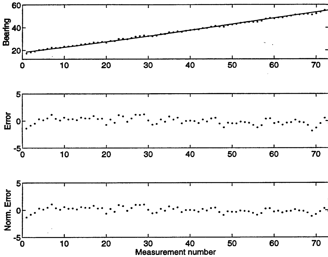
Figure 24: Field trial results for November 5, 1992
