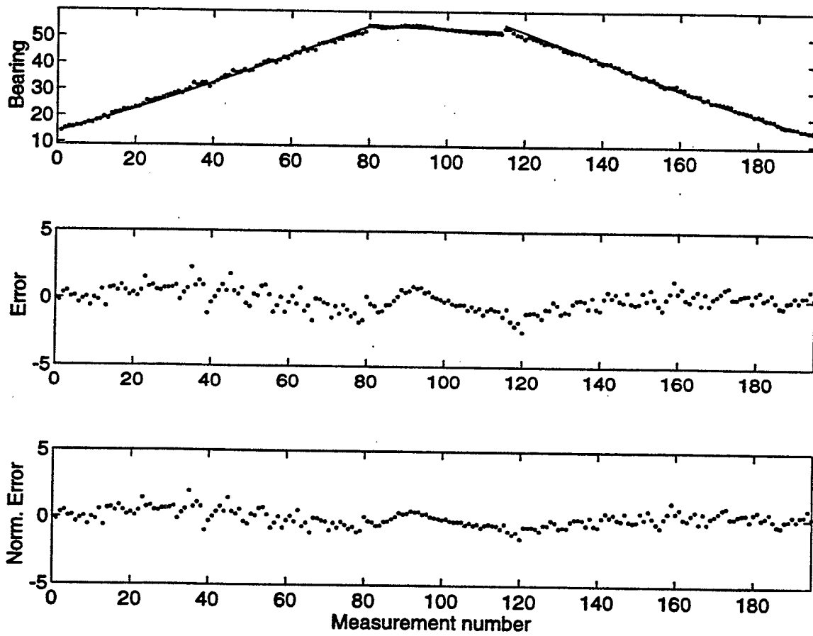
Figure 25: Field trial results for November 6, 1992
