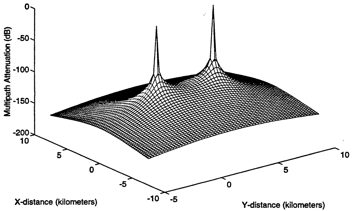
Figure 18: Excess path loss for an isotropic scatterer.
