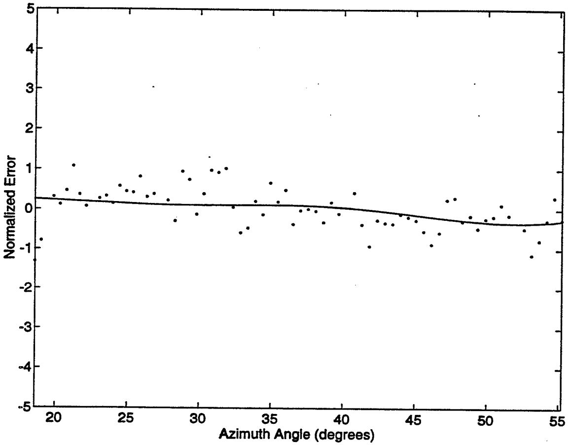
Figure 33: Revised error results for November 5, 1992. The dots represent actual error and the solid line represents predicted error due to mutual coupling.
