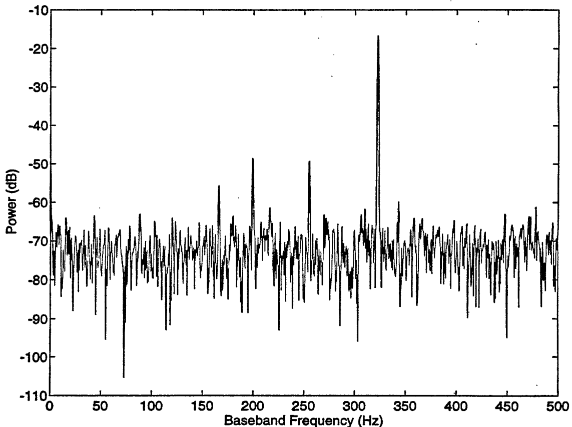
Figure 7: FFT spectrum of raw baseband data from channel 0
