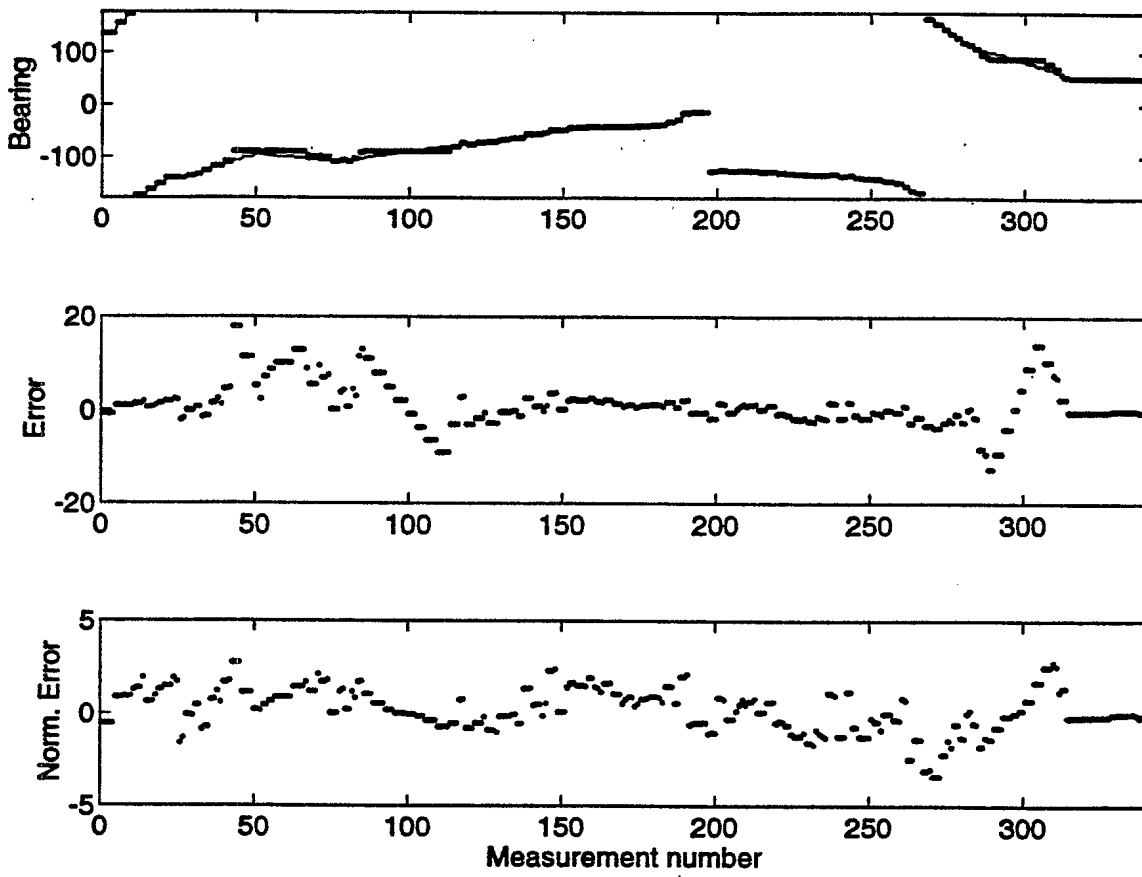
Figure 27: Field trial results for March 25, 1993
