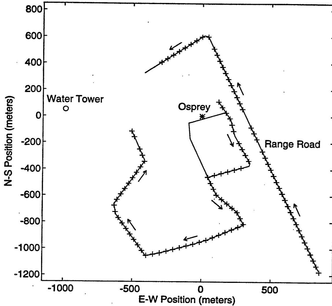
Figure 6: Transmitter locations (marked by +) on March 25, 1993 relative to Osprey system. Arrows show vehicle direction. Start position was (x_{E-W}, y_{N-S}) = (118, 110)
