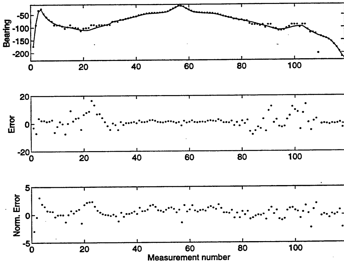
Figure 26: Field trial results for March 24, 1993
