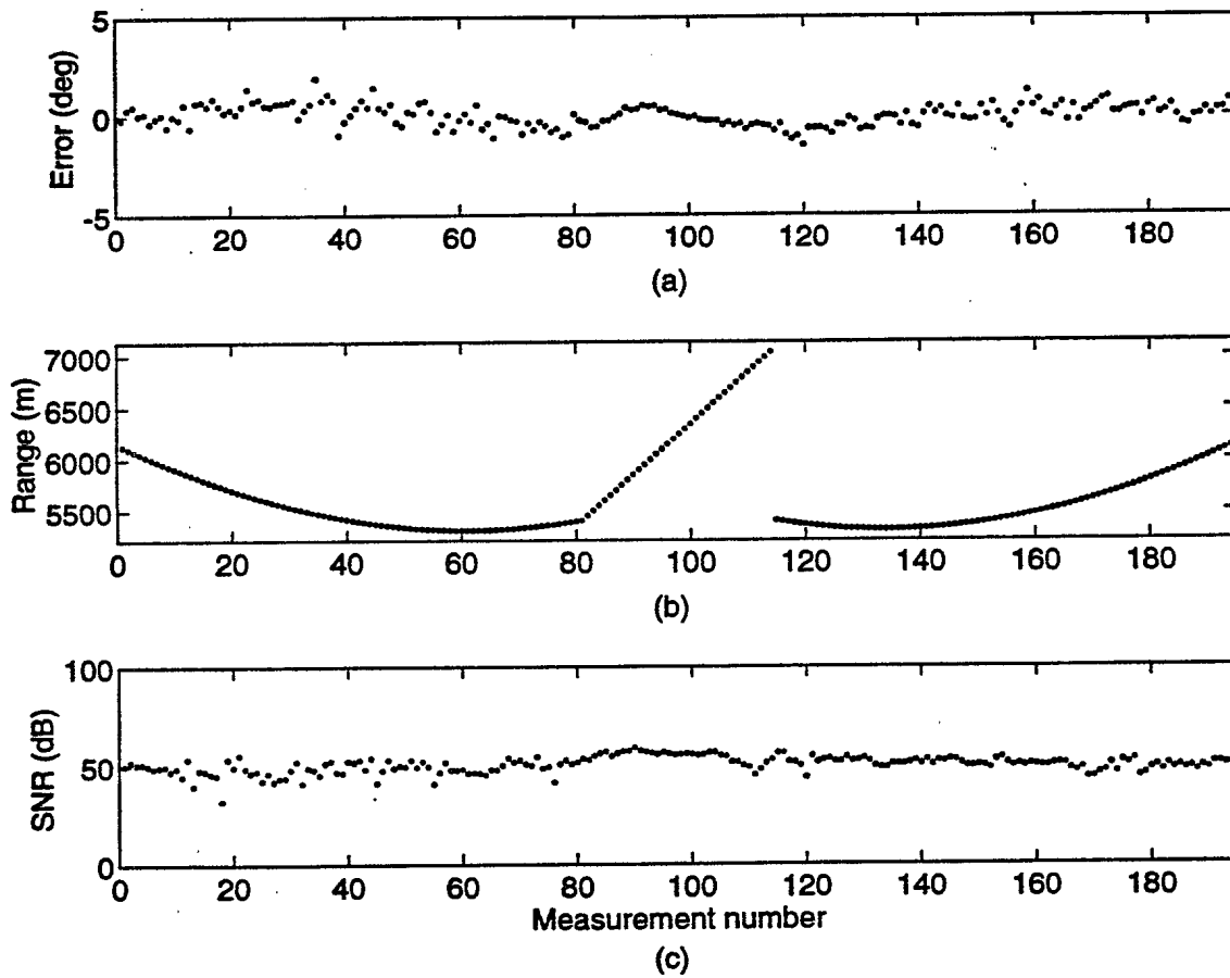
Figure 29: Field trial parameters for November 6, 1992: (a) broadside normalized error, (b) range, and (c) signal to noise ratio.
