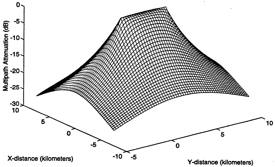
Figure 16: Excess path loss for a perfect reflector.
