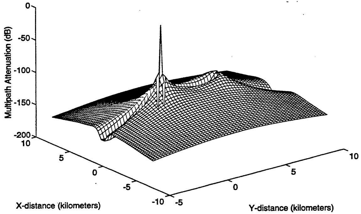
Figure 21: Combined effect of excess path loss and directional loss for an isotropic scatterer.
