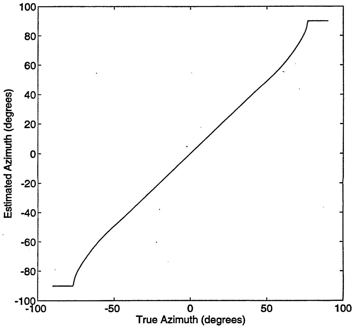
Figure 10: Estimated bearing versus true bearings with mutual coupling.
