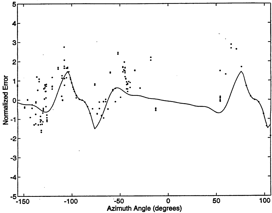
Figure 36: Revised error results for March 25, 1993. The dots represent actual error and the solid line represents predicted error due to mutual coupling.
