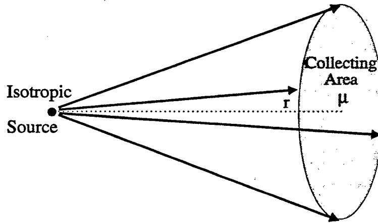
Figure 12: Effective collecting area of an isotropic antenna.
