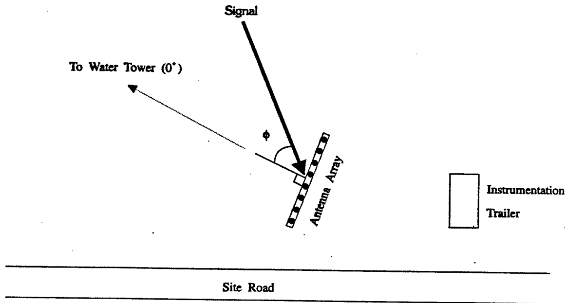
Figure 2: Physical layout of field trial DF site.
