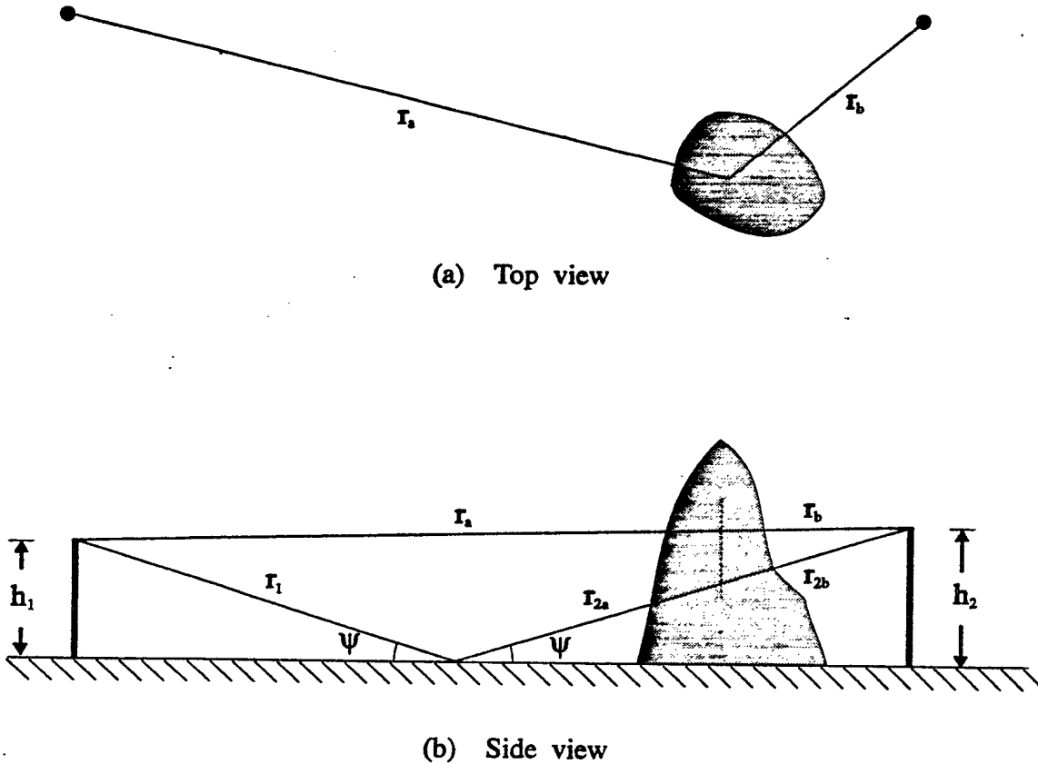
Figure 15: Plane Earth propagation model for a perfect reflector.
