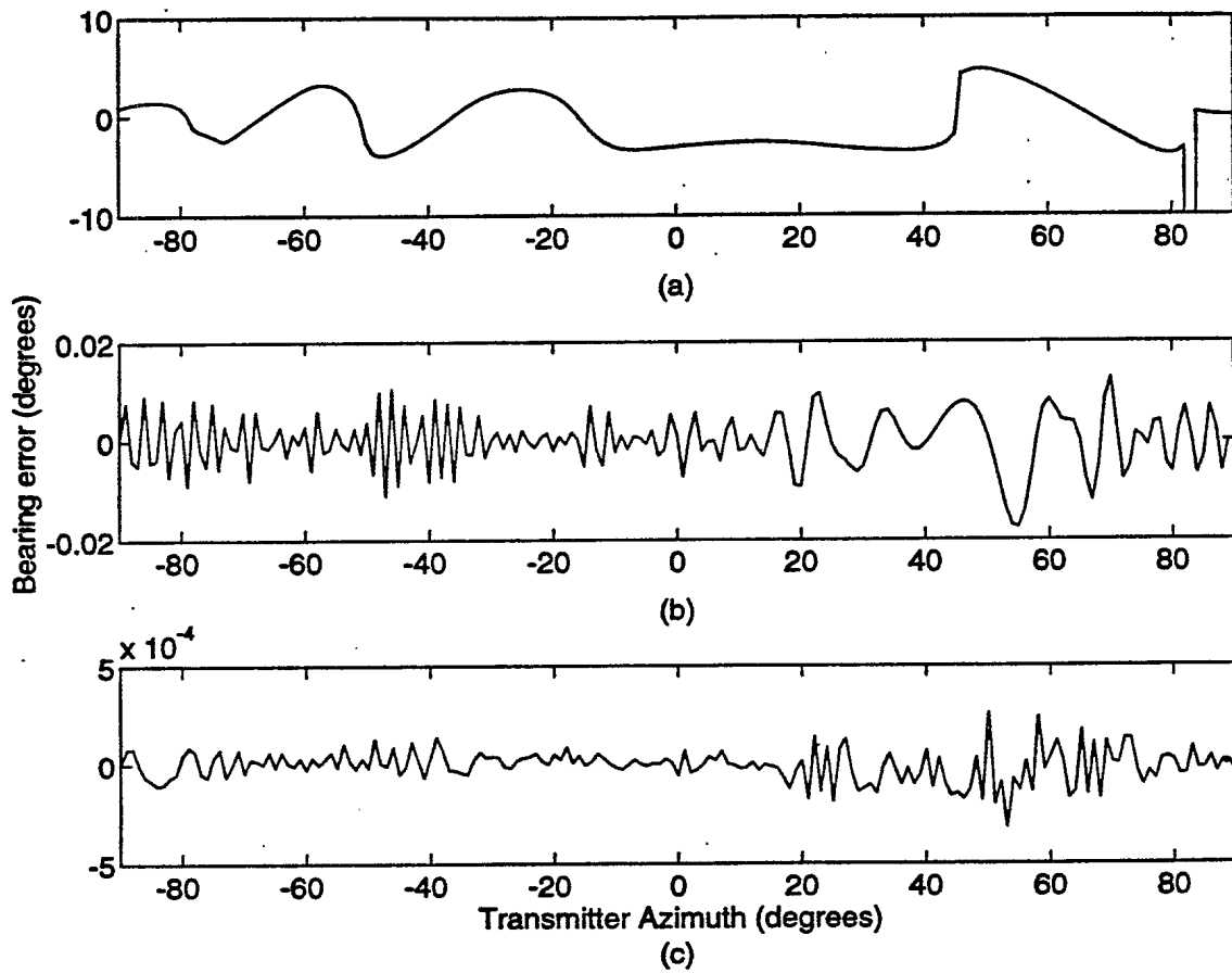
Figure 23: Simulated DF error response for 3 multipath scatterers at bearings of -60, 40, and 90 degrees, and ranges of (a) 10 m (b) 100 m, and (c) 1000 m.
