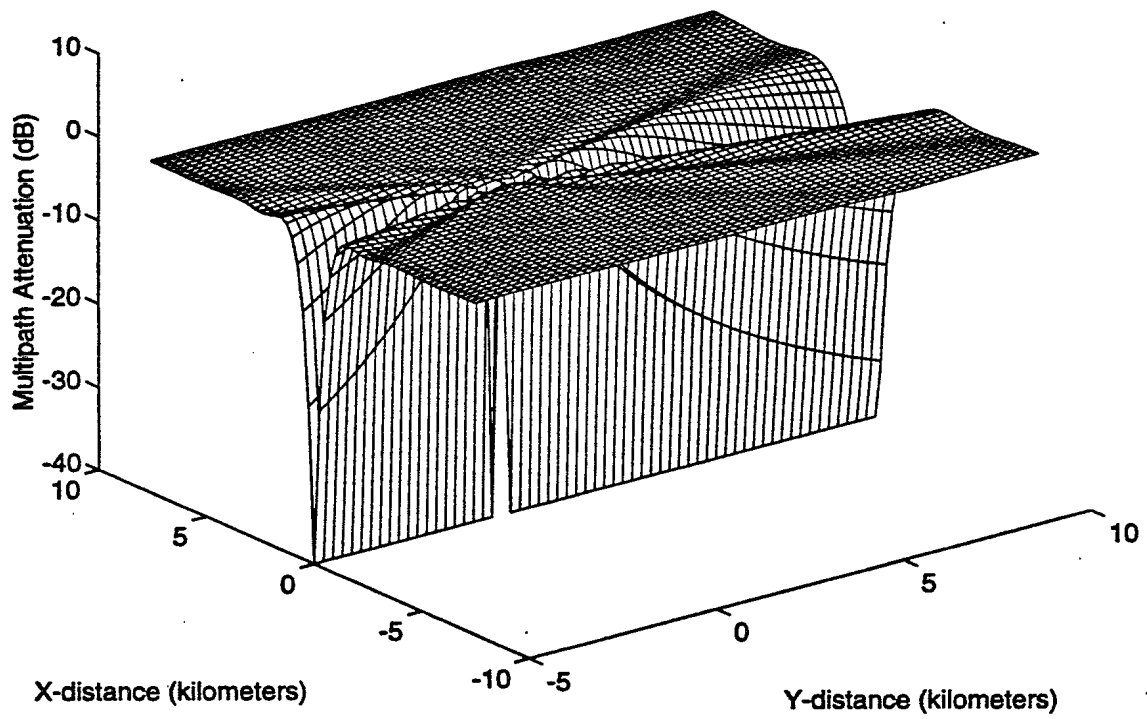
Figure 19: Directional multipath power loss l_{\varphi} .
