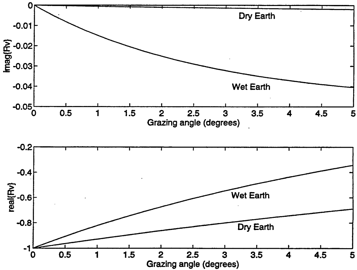
Figure 14: Reflection coefficient versus grazing angle.
