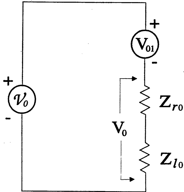
Figure 9: Equivalent electrical circuit for antenna 0.
