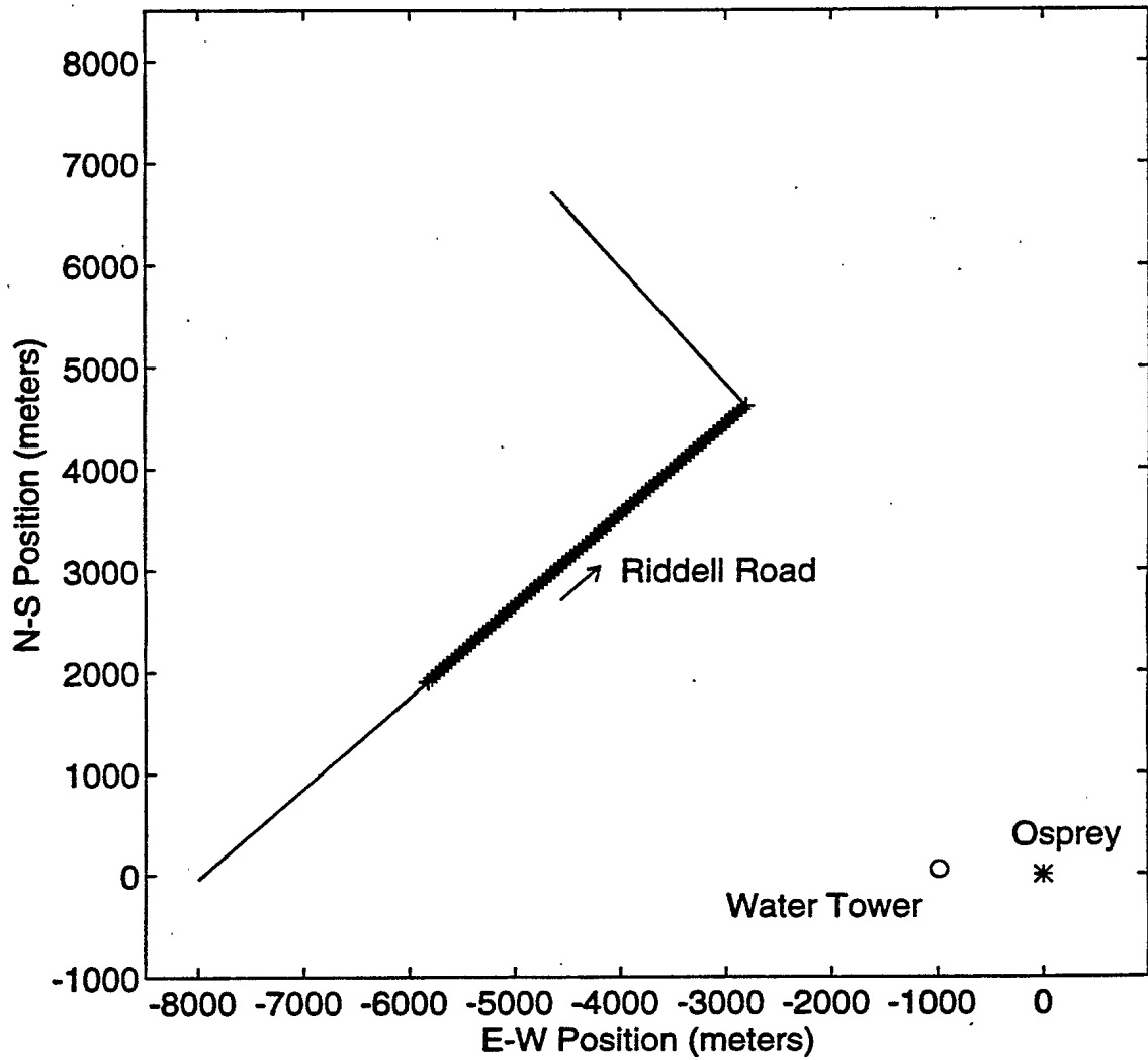
Figure 3: Transmitter locations (marked by +) on November 5, 1992 relative to Osprey system at (0,0). Arrows show vehicle direction. Start position was (x_{E-W}, y_{N-S}) = (-5825, 1909)
