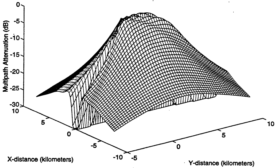
Figure 20: Combined effect of excess path loss and directional loss for a perfect reflector.
