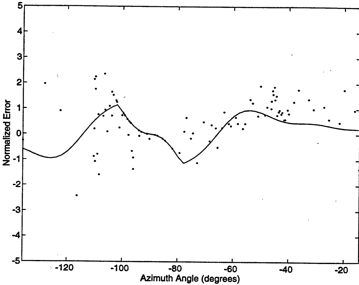
Figure 35: Revised error results for March 24, 1993. The dots represent actual error and the solid line represents predicted error due to mutual coupling.
