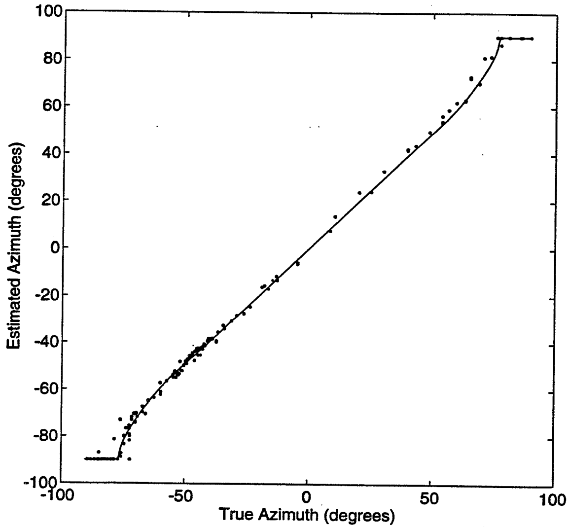
Figure 32: Theoretical mutual coupling effects (solid line) compared to results from March 25, 1993 (dots)
