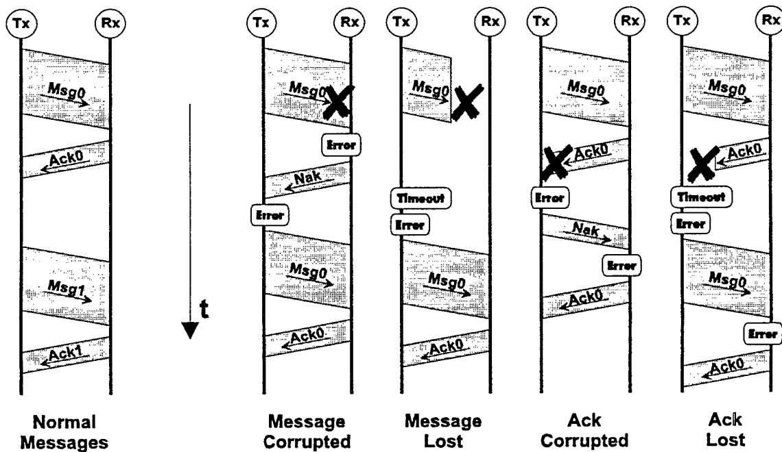
Fig. 2. Normal and single-error cases for stop-and-wait ARQ.
