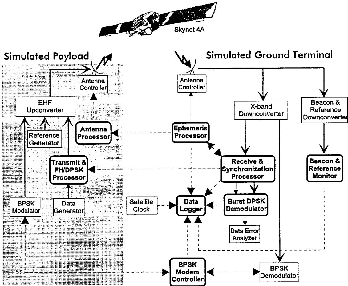
Fig. 1. Skynet EHF trials block diagram.
