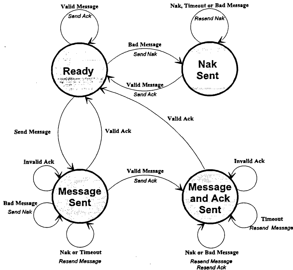
Fig. 3. High-level protocol receiver state diagram.
