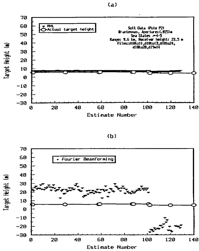
Figure 14: RML and Fourier beamforming tracking over sea states 4 and 5.
