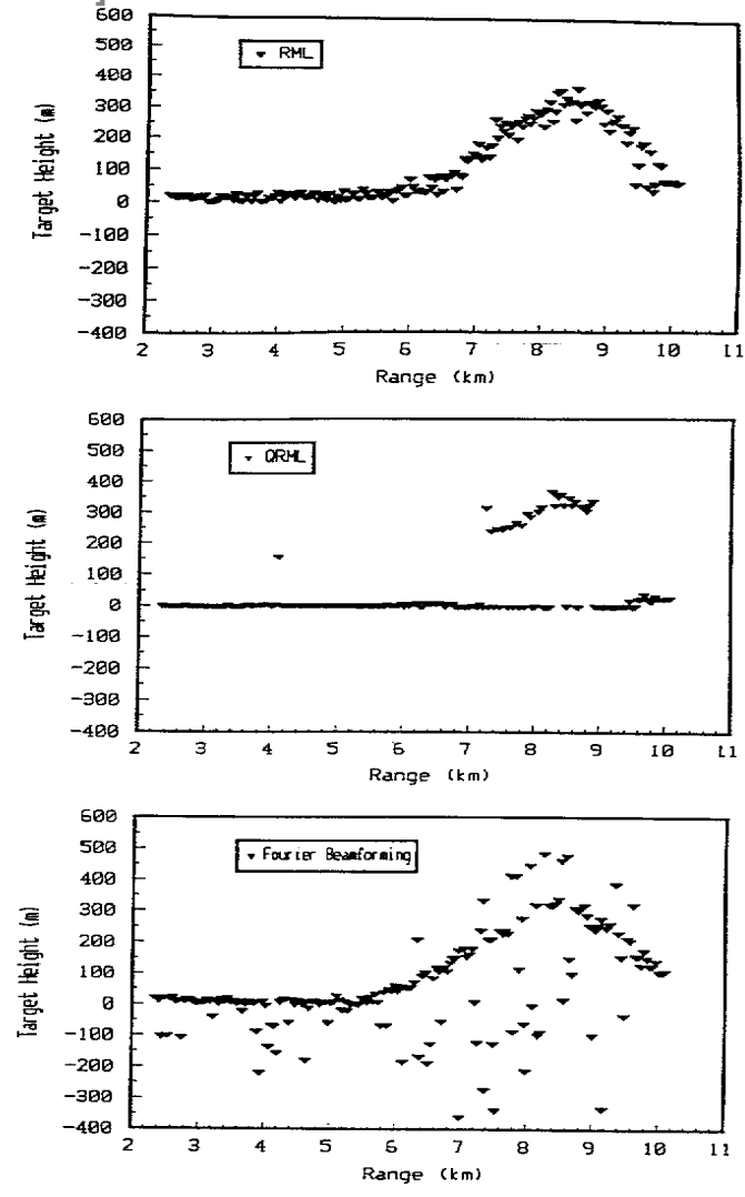
Figure 15: Tracking of a Sea King Helicopter over SS3 sea conditions.
