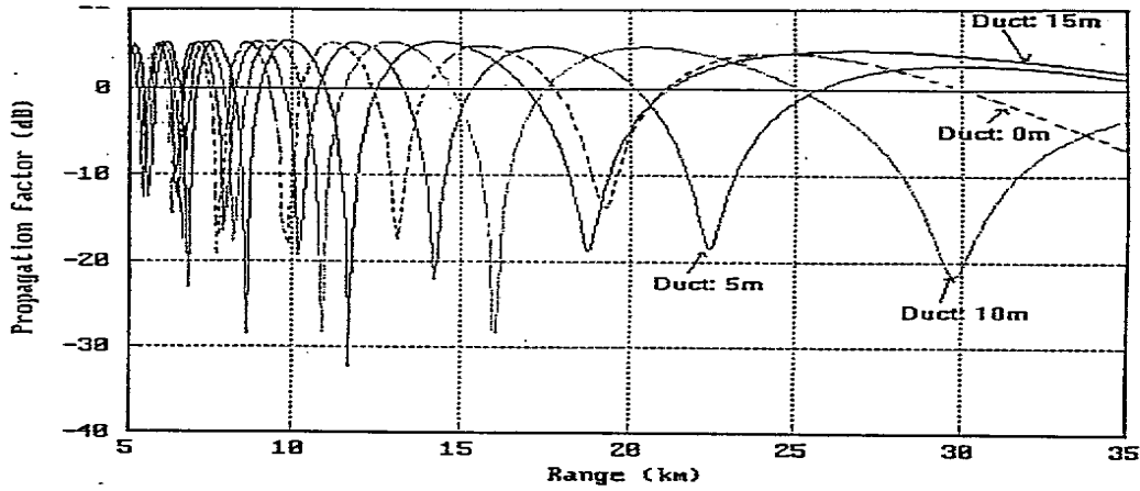
Figure 6: Propagation factor versus range for various duct heights: Freq.=10GHz, antenna height=25 m, pol.=H, BW=1.4 deg., height of the source=20 m.
