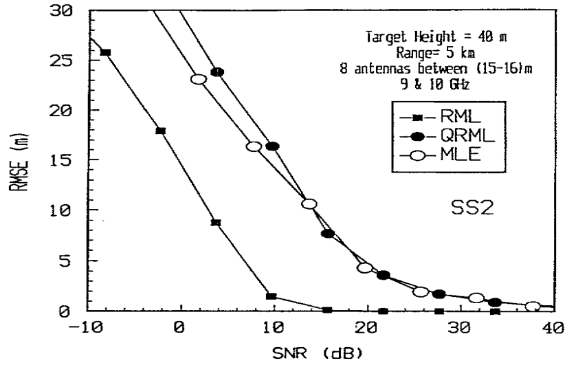
Figure 7: Performance of QRML, RML and MLE when no incoherent multipath is present.
