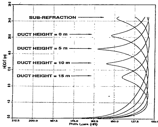
Figure 5: Low-level vertical interference pattern for various duct heights and a subrefractive condition (10 GHz).
