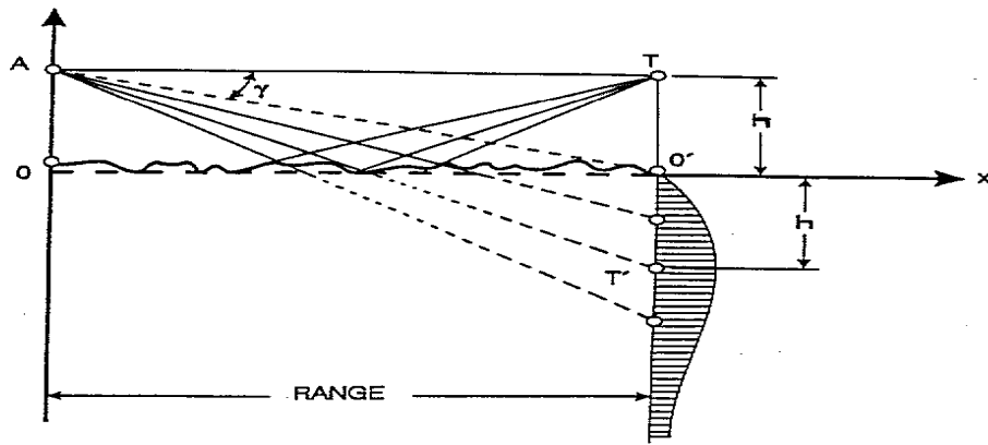
Figure 3: Extension in apparent height of the target due to multiple reflections from a rough surface.
