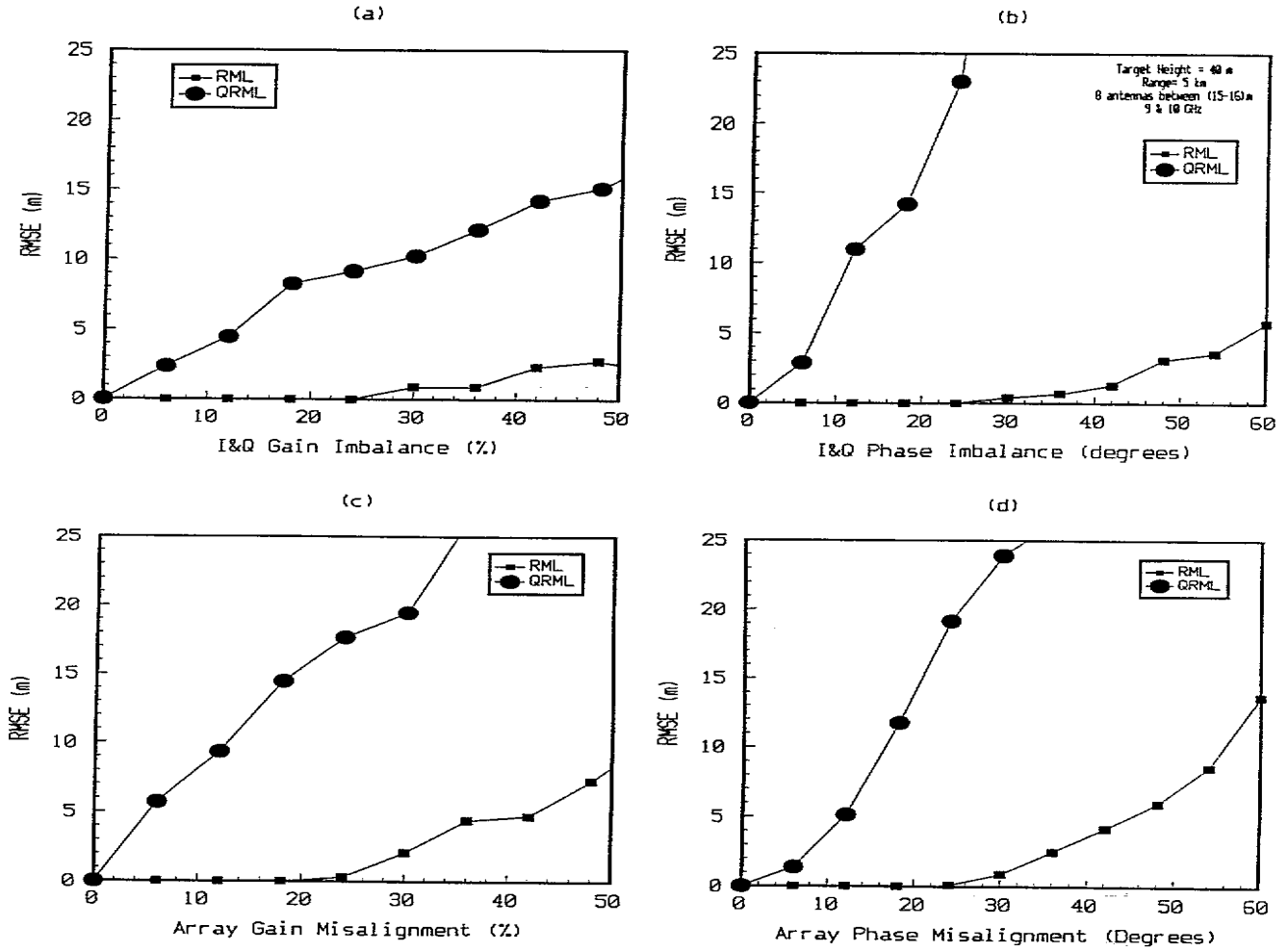
Figure 10: Effects of calibration errors on the performance of QRML, RML and MLE.
