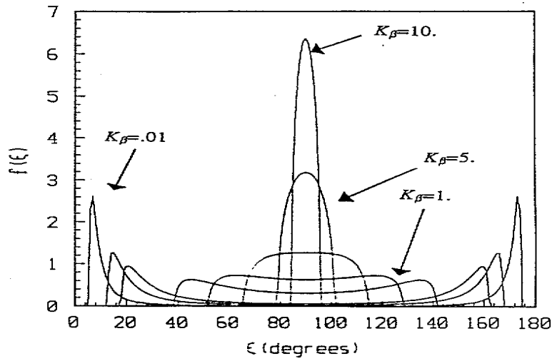
Figure 2: The function f(\xi)
