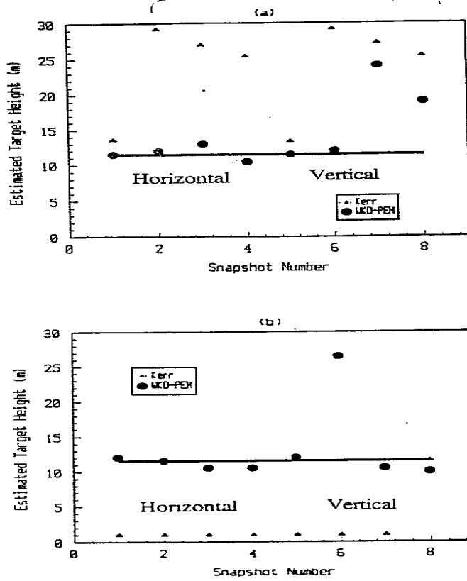
Figure 20: Target height estimations derived from HGP measurements: (a) Condition 1, (b) Condition 2.
