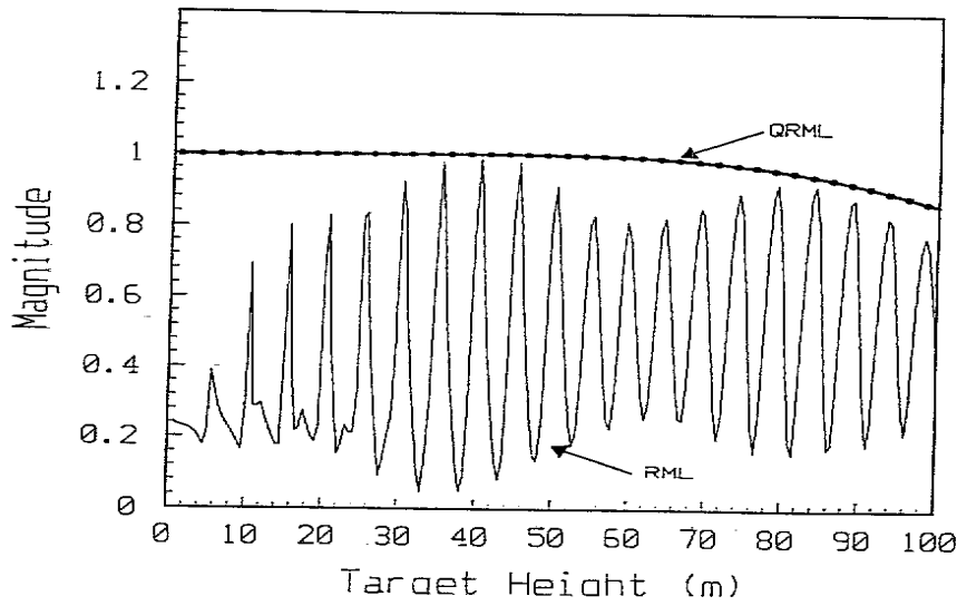
Figure 4: An example of RML and QRML versus height.
