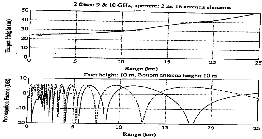
Figure 12: RML target height estimations versus range under a 10-m duct condition and the corresponding propagation factor for a target height of 25 m.
