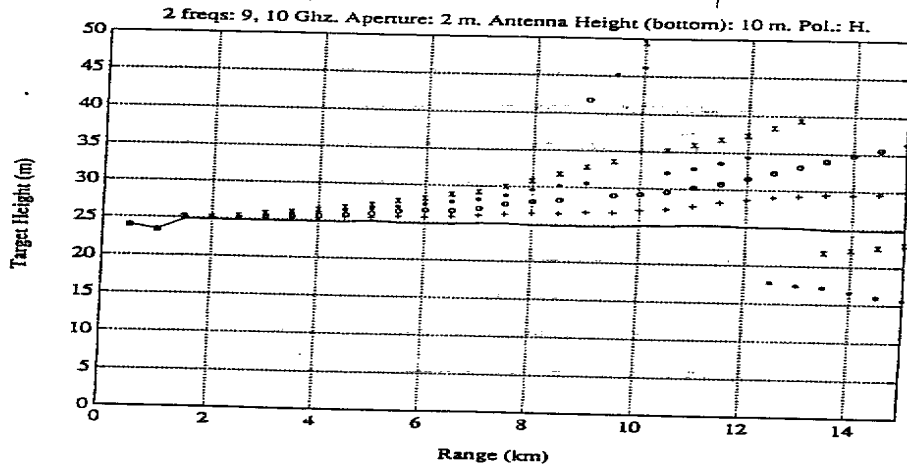
Figure 13: RML target height estimations for duct heights of 0 m (solid line), 5 m (+), 10 m (o), 15 m (*) and 20 m (x) and for a target height of 25 m.
