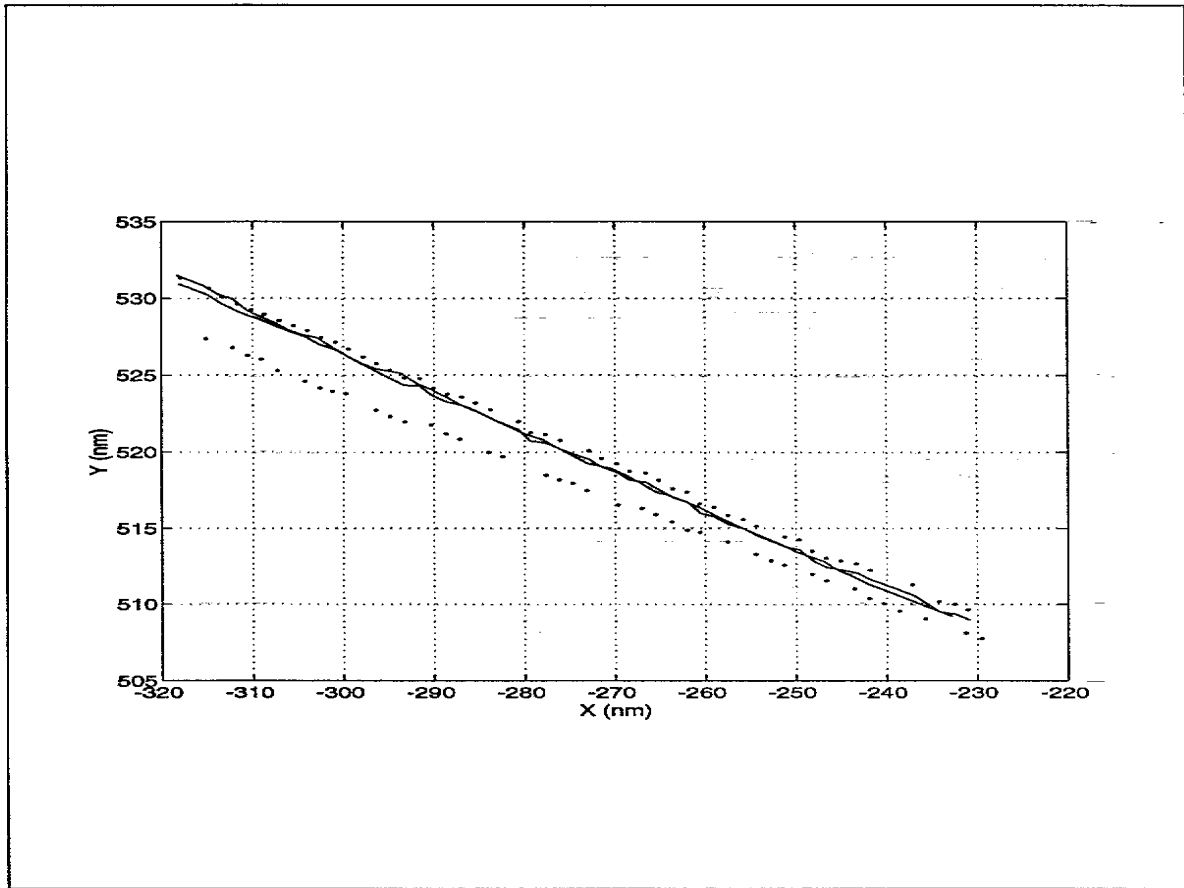
Figure 5 Tracks from two radars in CW before and after the LS-RTQC algorithm
