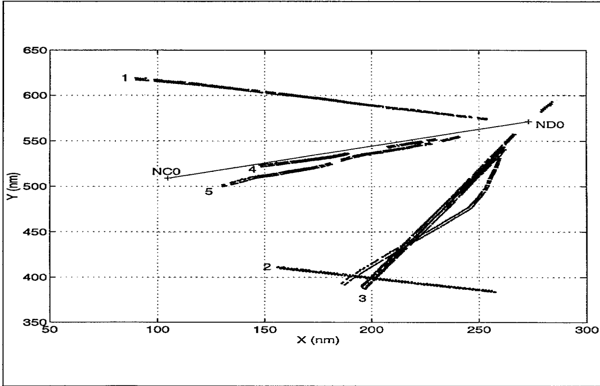
Figure 6 Common tracks of radar NC0 and ND0 (DREO1)
