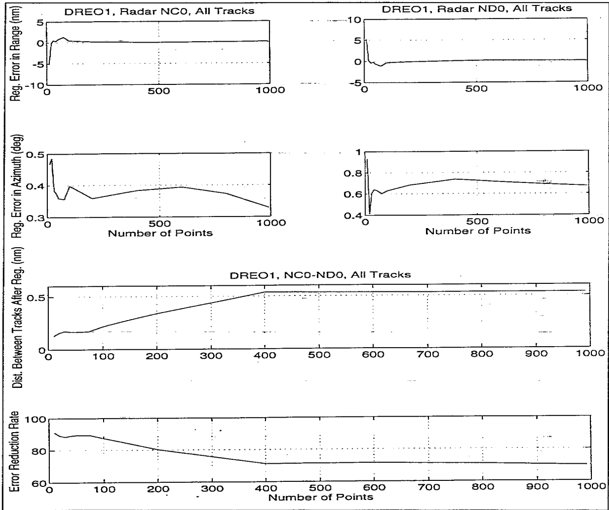
Figure 8 Convergence analysis of bias and registration error of DREO1CD
