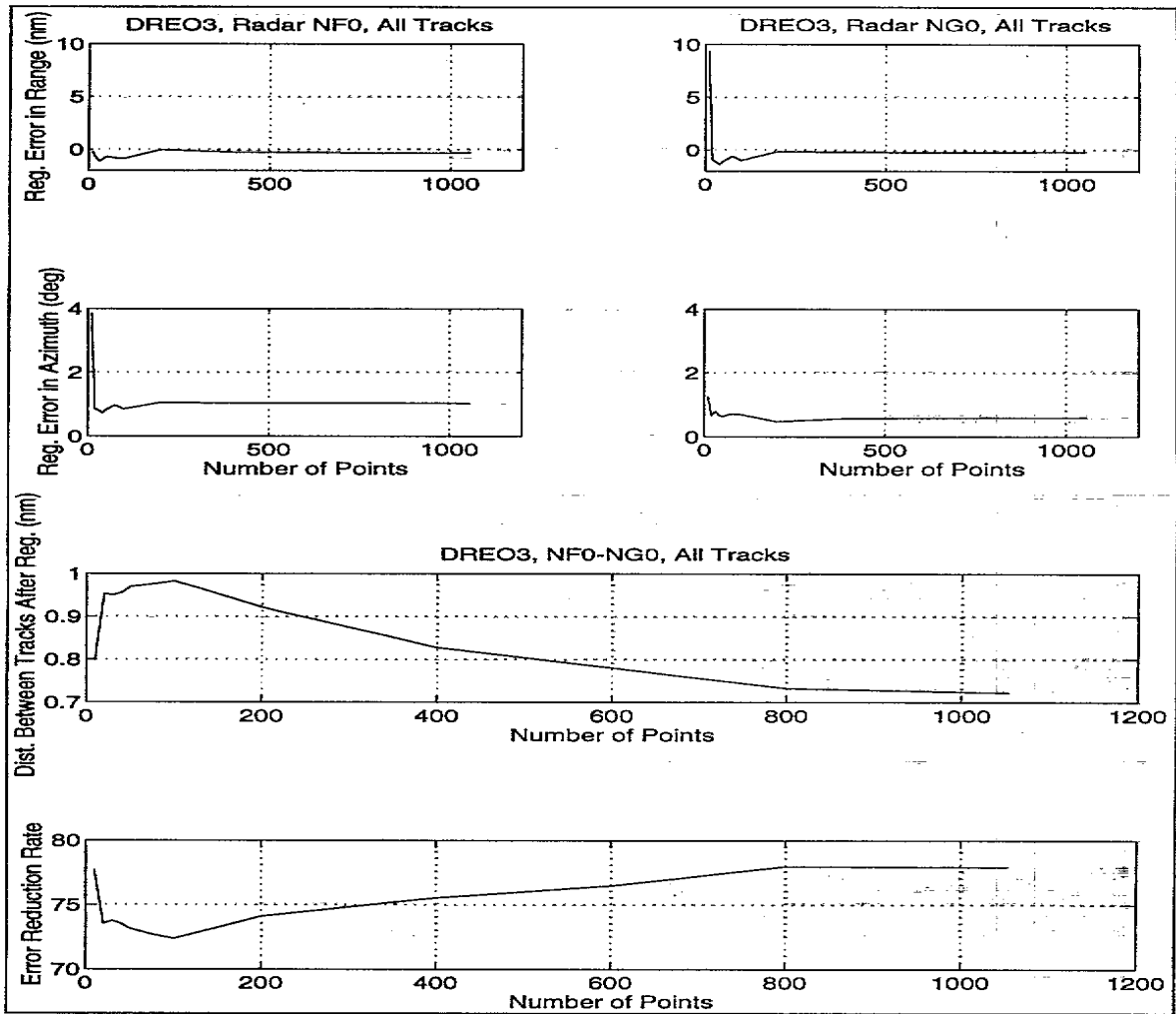
Figure 9 Convergence analysis of bias and registration error of DREO3FG
