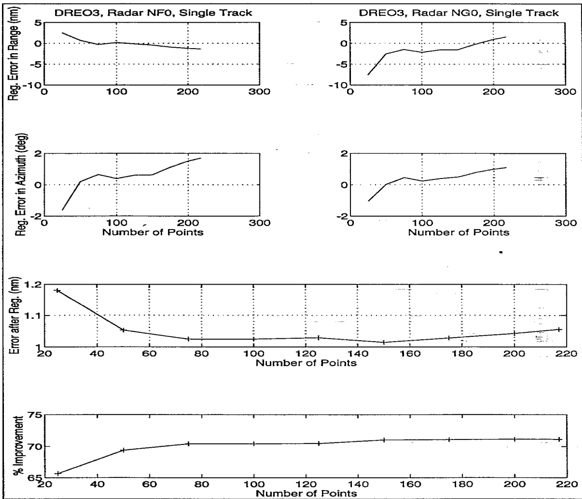
Figure 11 Convergence analysis of bias and registration error of DREO3 using a single track
