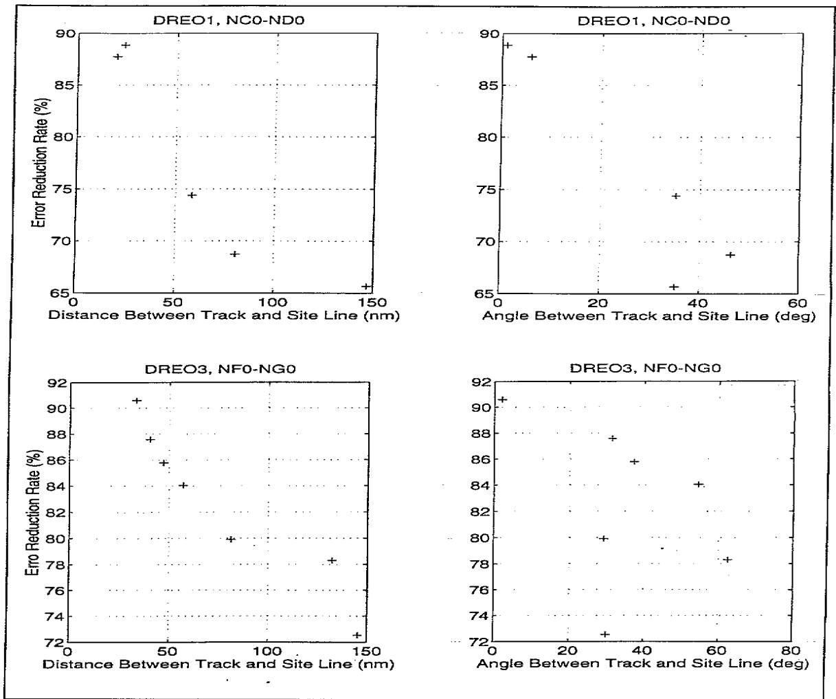
Figure 13 Relationship between the error reduction rate and the track location
