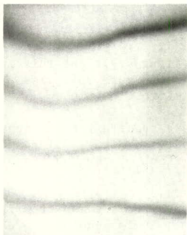
Figure 34. Beam Shearing Interferogram after the collimator.
