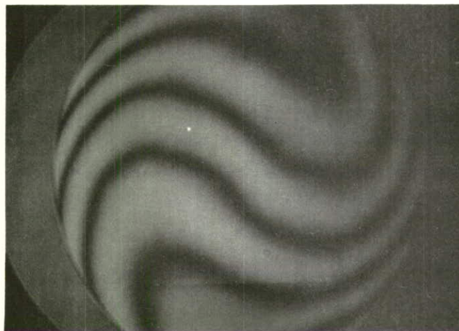
Figure 39. Beam Shearing Interferogram after the spherical telescope mounted with two good quality mirrors.
