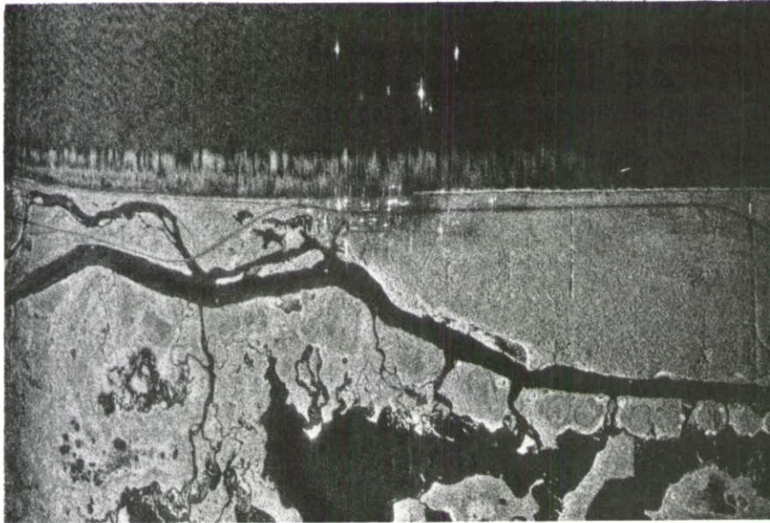
Figure 51. Image produced by the ERIM Correlator from the Interferogram used to produce the image shown in figure 50.
