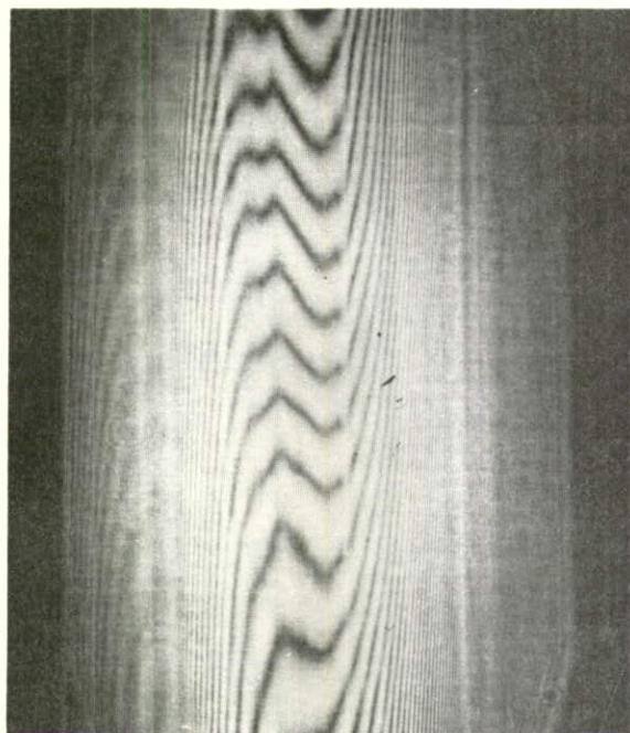
Figure 27. Beam Shearing interferogram after the cylindrical telescope ( K=4 )
