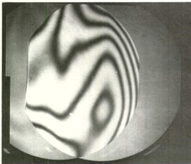
Figure 40. Beam Shearing interferograms after the spherical telescope mounted with two poor quality mirrors.
