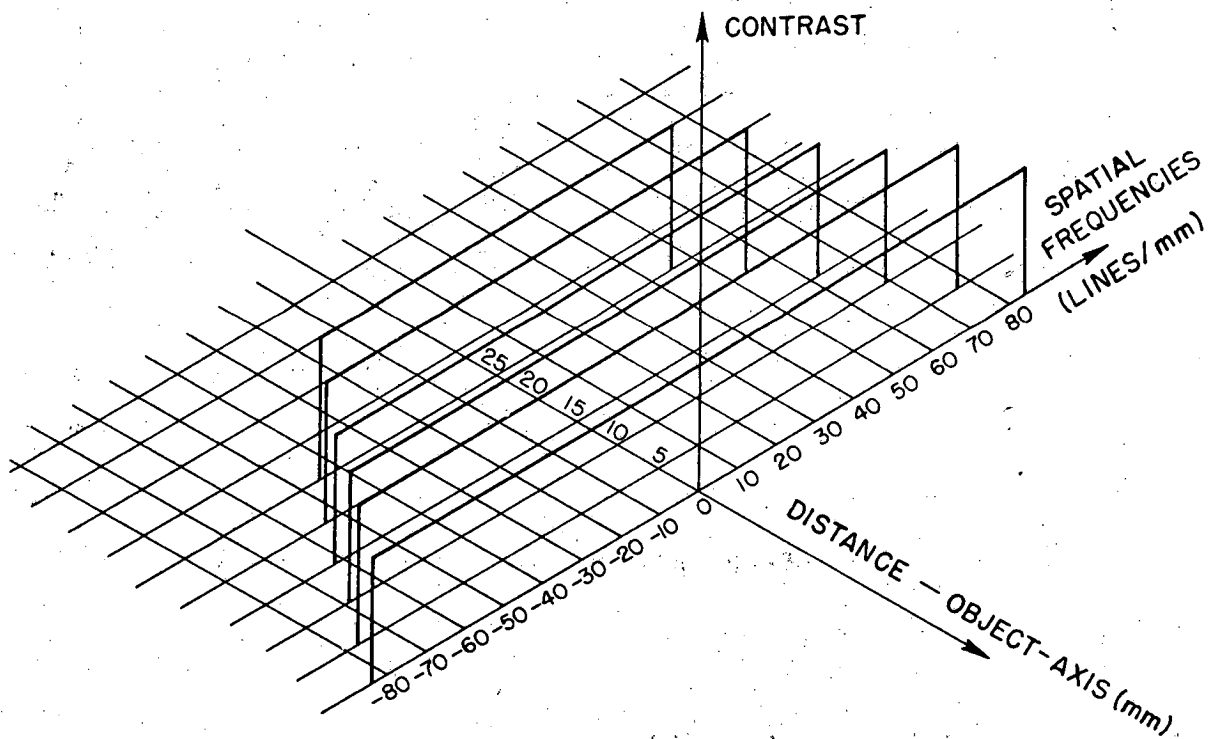
Figure 15. Theoretical transfer function of the spherical telescope
