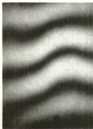
Figure 37. Beam Shearing Interferogram after reflection on two good mirrors
