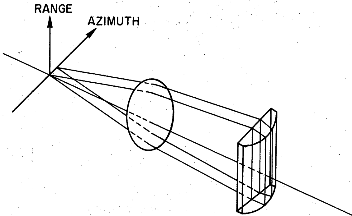
Figure 44. Azimuthal curvature of the image field
