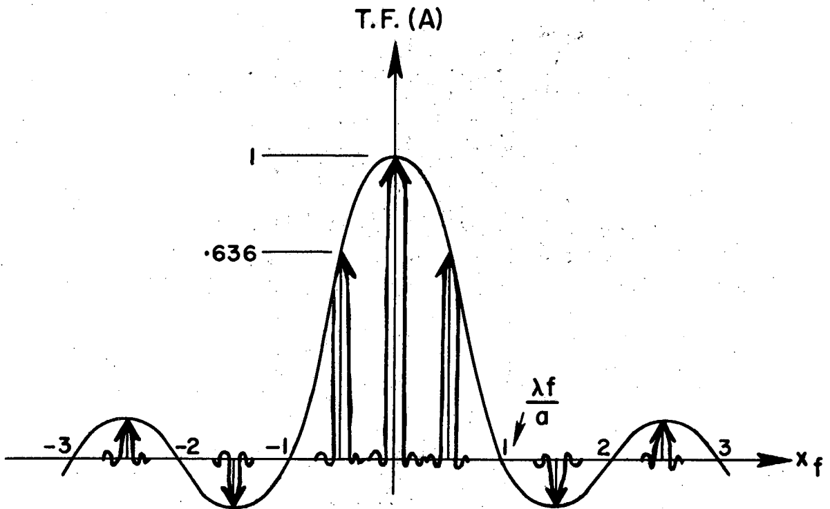
Figure 22. Fourier transform of a Ronchi grating
