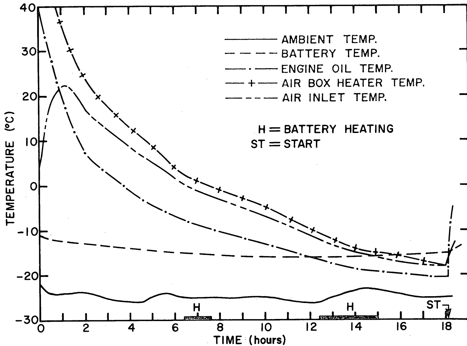
Fig. 15: Cooling Curves Test #10.
