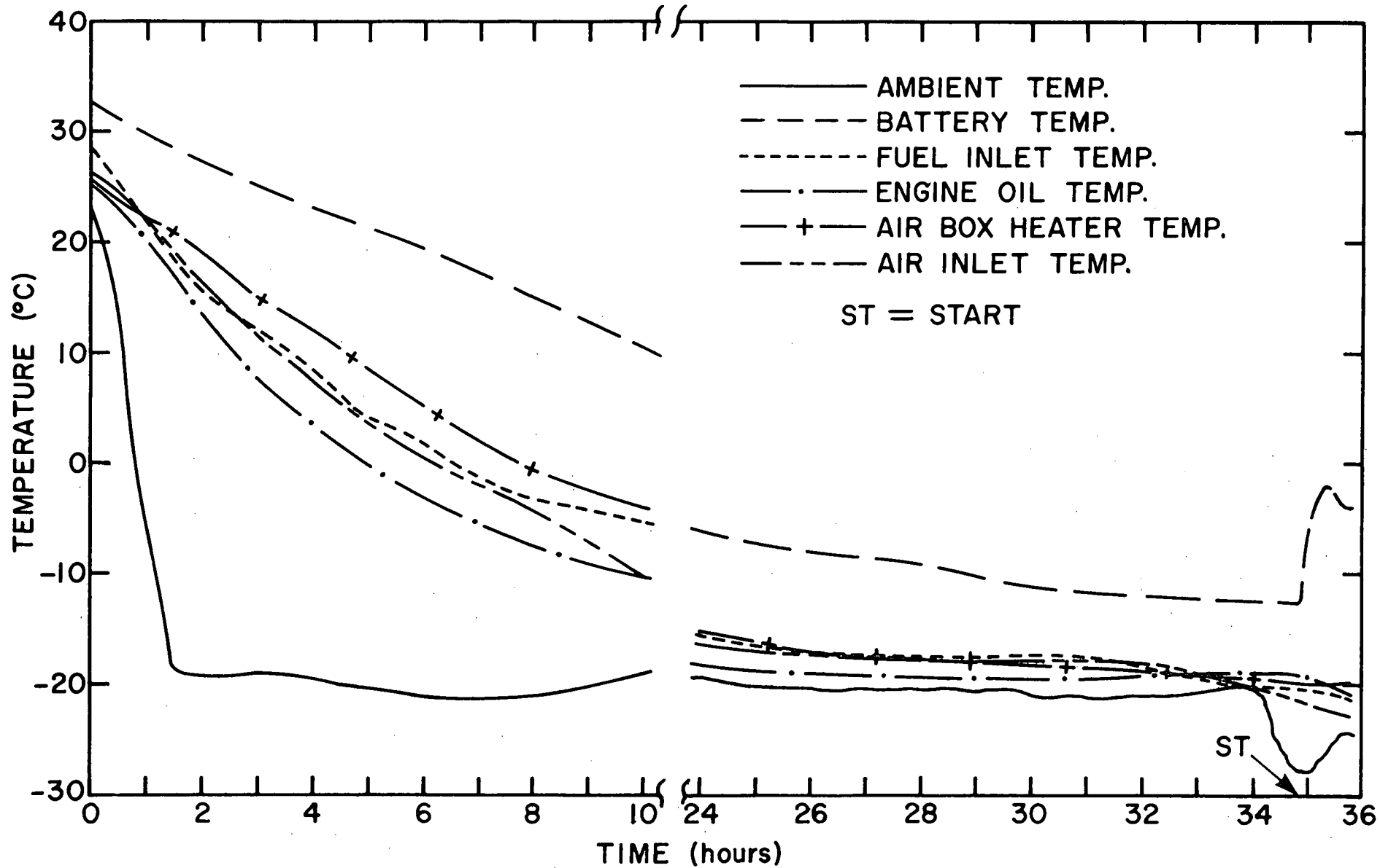
Fig. 6: Cooling Curves Test #1.
