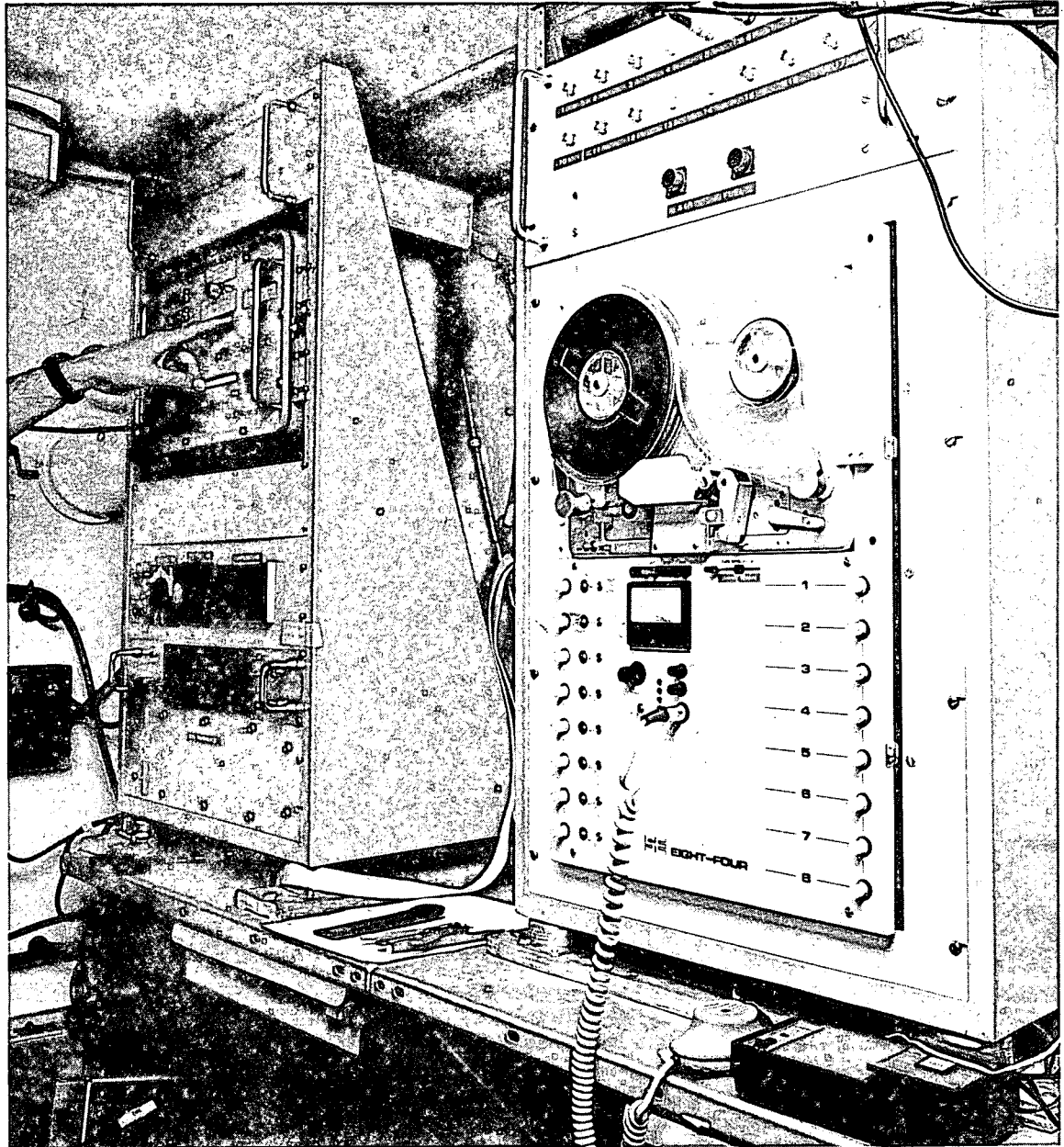
Fig. 3: Instrumentation Racks Inside Instrumentation Vehicle.
