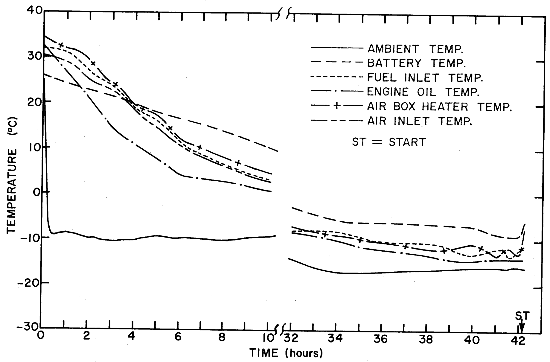
Fig. 10: Cooling Curves Test #5.
