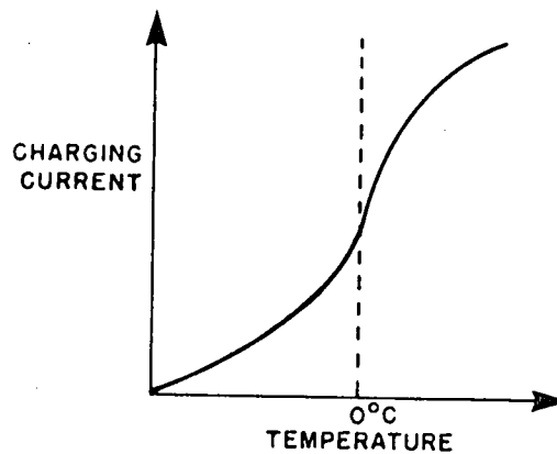
Fig. 2-VII: Charging current as a function of temperature. Voltage is constant. From [1].
