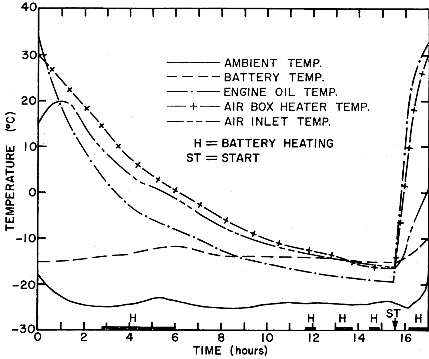
Fig. 14: Cooling Curves Test #9.
