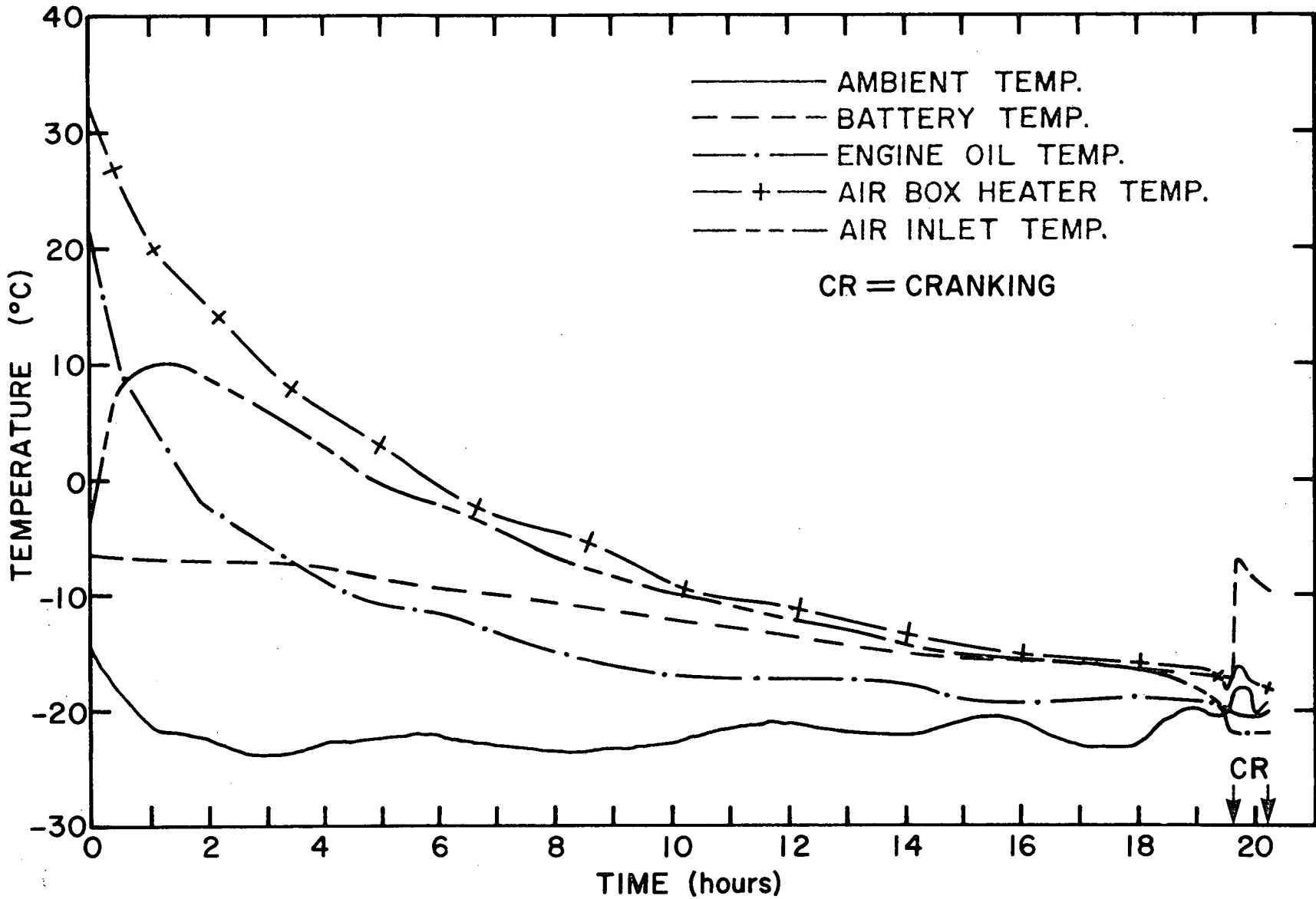
Fig. 11: Cooling Curves Test #6.
