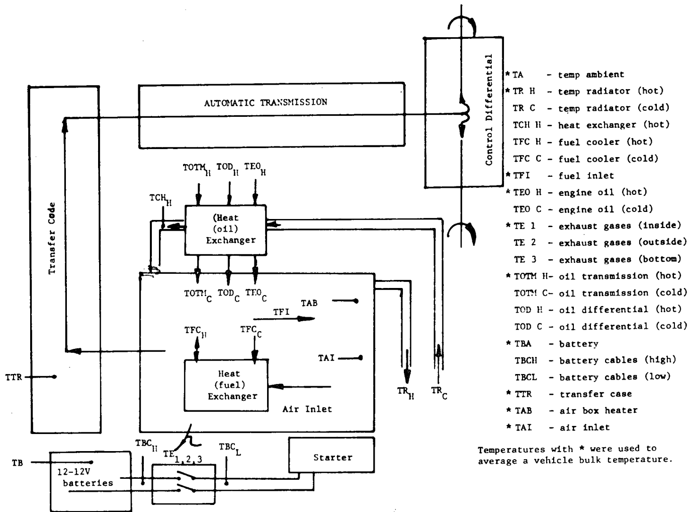
Figure 3-IV - System Temperature
