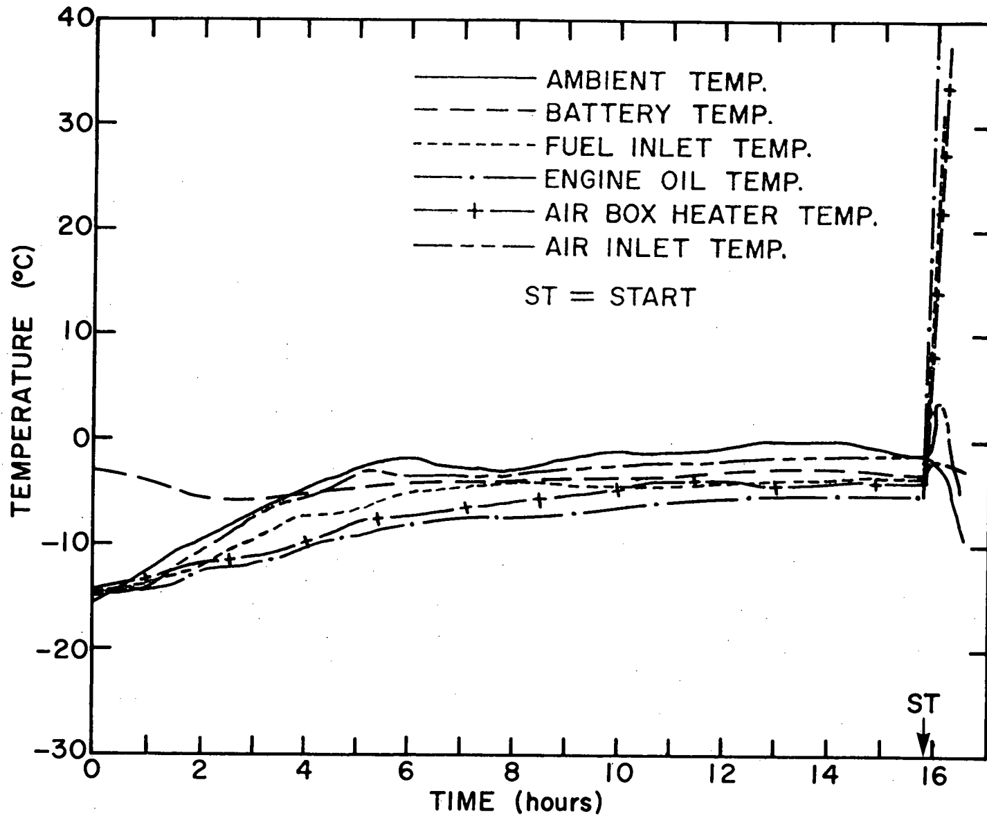
Fig. 8: Cooling Curves Test #3.
