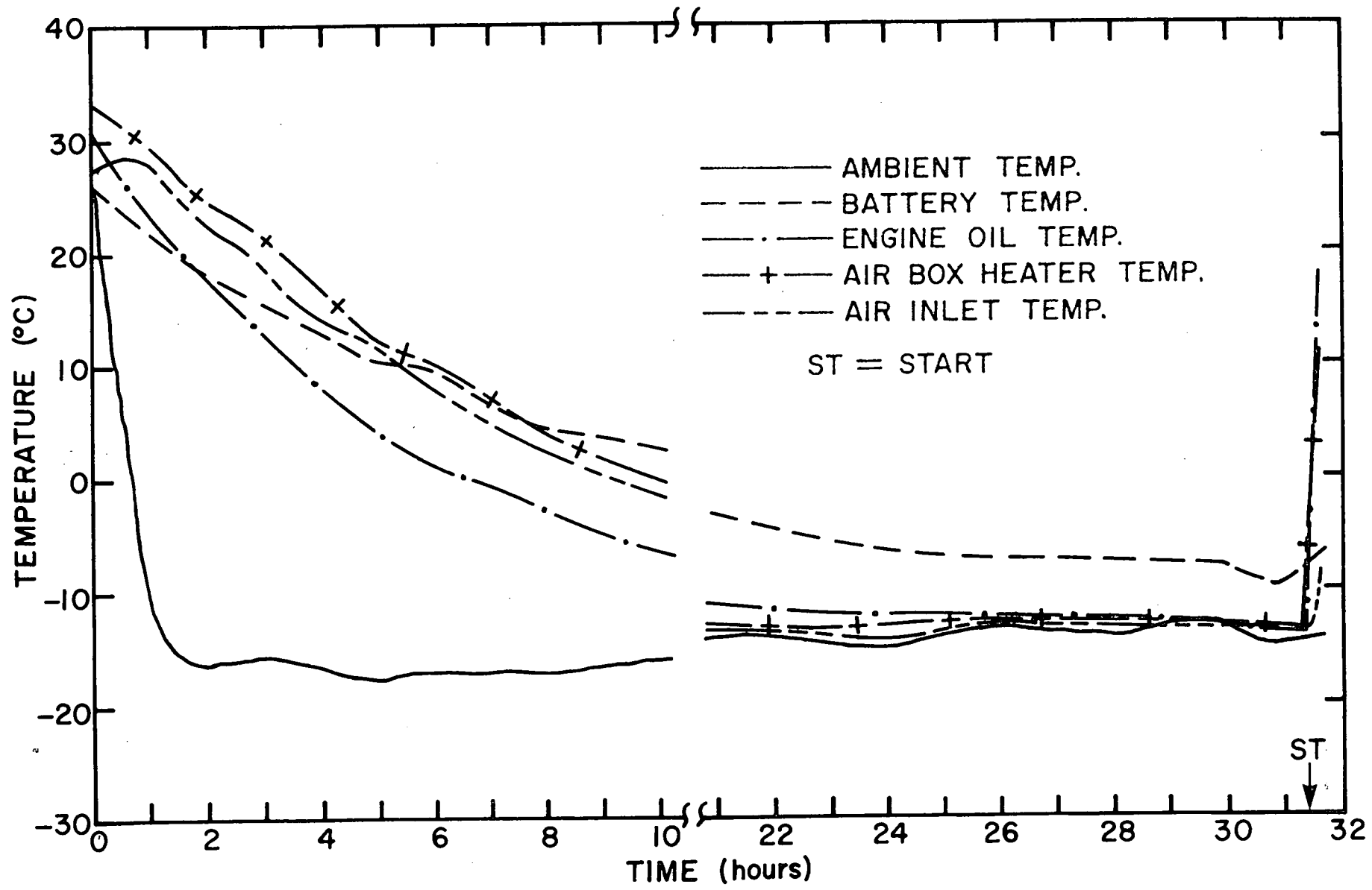
Fig. 12: Cooling Curves Test #7.
