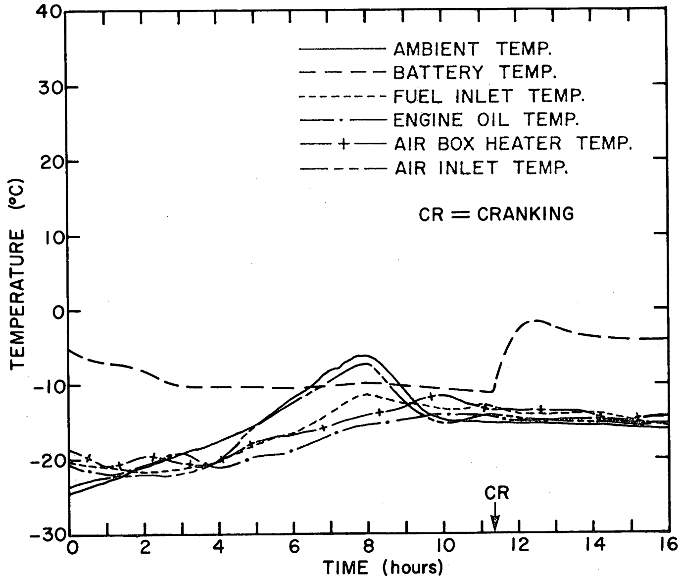
Fig. 7: Cooling Curves Test #2.
