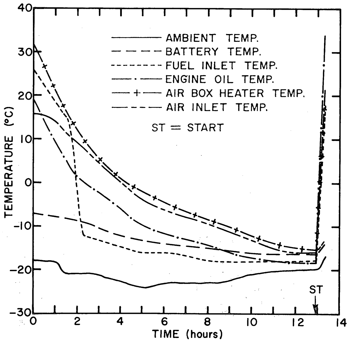
Fig. 13: Cooling Curves Test #8.
