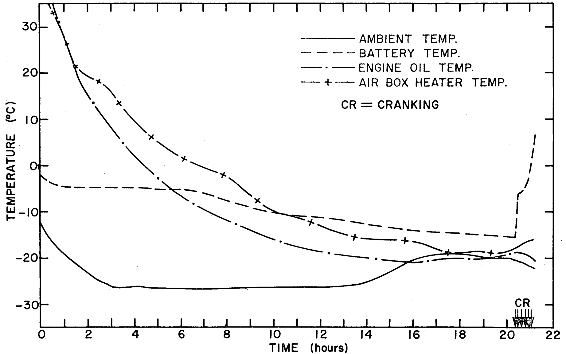
Fig. 9: Cooling Curves Test #4.
