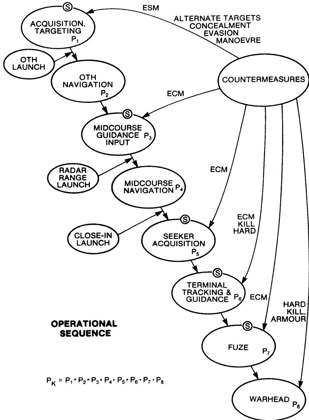
FIGURE 1 SEQUENCE OF OPERATIONS INVOLVED IN THE AIR LAUNCH OF AN ANTI-SHIP MISSILE
