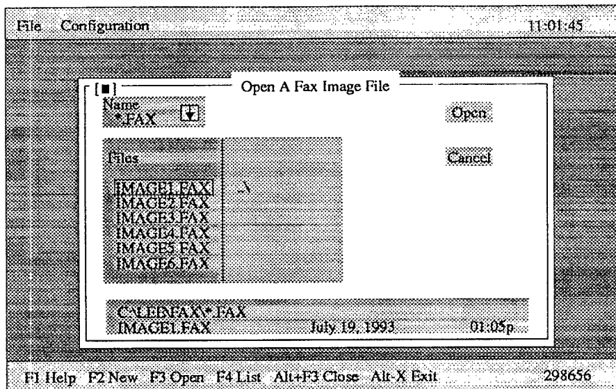
Figure 2: Defaxer File Manager Dialogue Box
