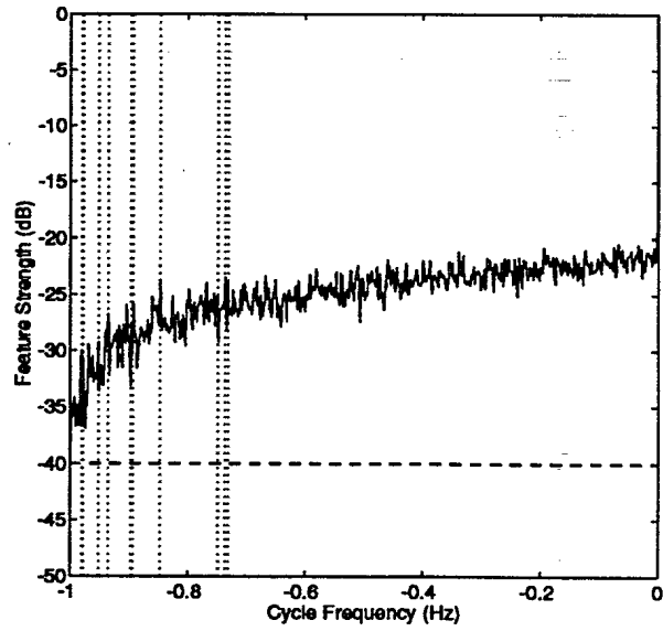
(b) N0 ( N=4096 , Np=64 )
