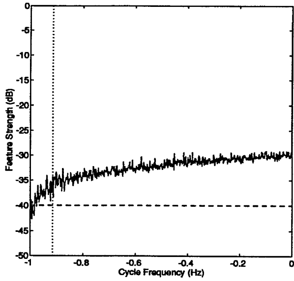
(a) N0 ( N=32768 , Np=64 )
