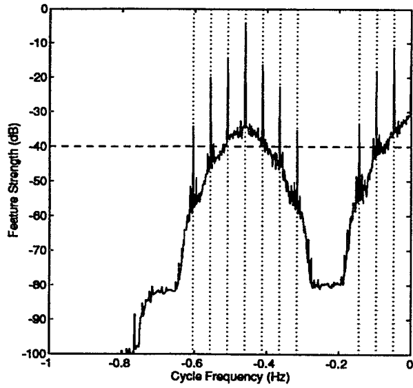
(a) A(N=32768, Np=64)
