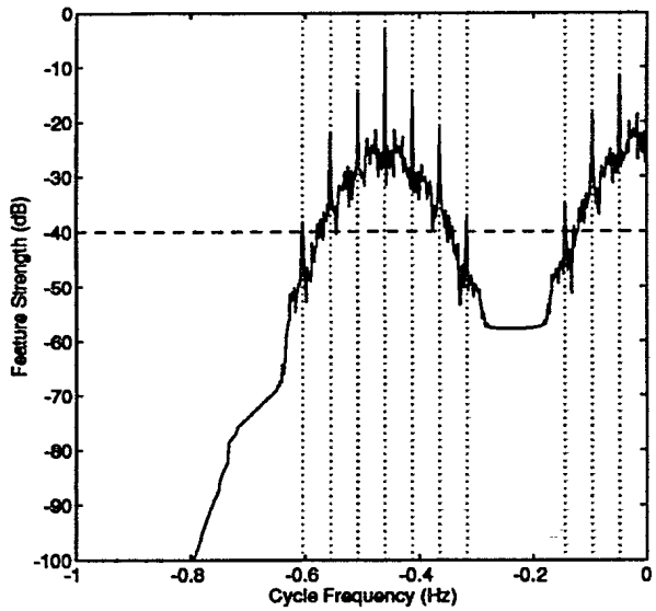
(a) A ( N=1024, Np=64 )
