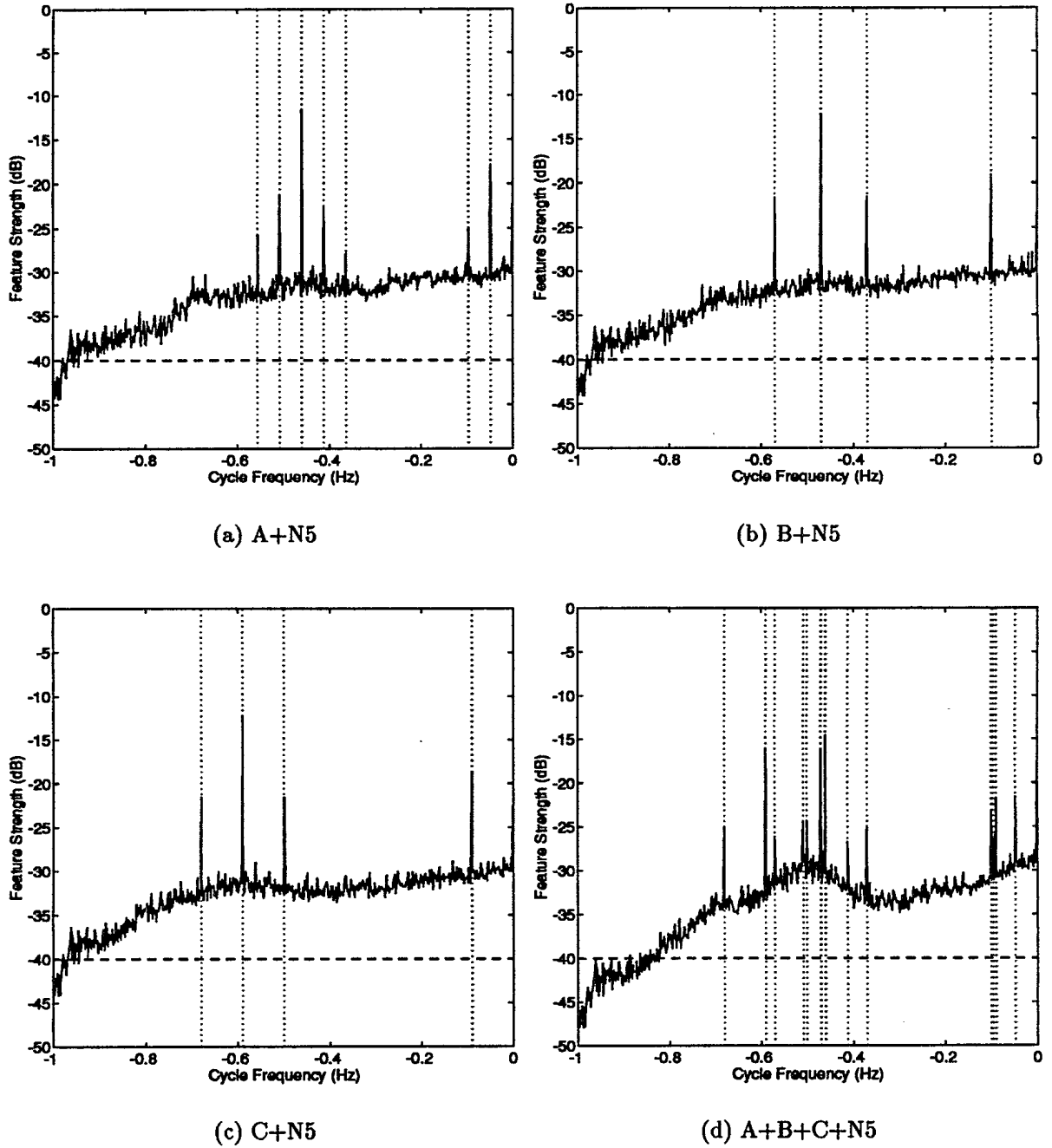
Figure 18: CFF of Various BPSK Signals in Noise N5 Using N=32768 , N_p=64 .
