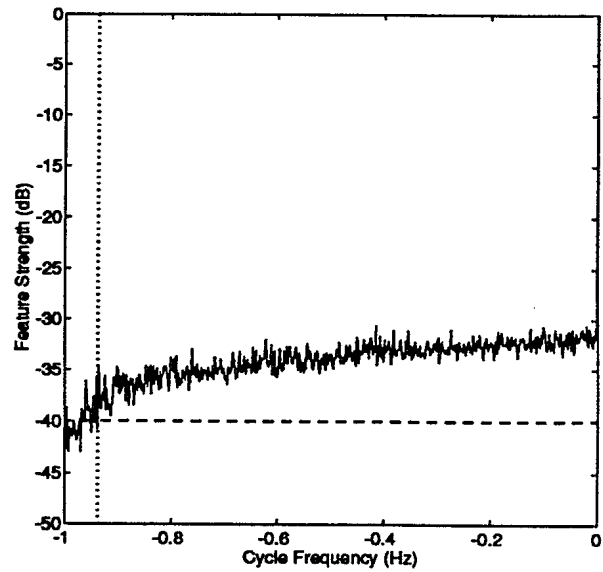
(b) N0 ( N=32768 , Np=32 )
