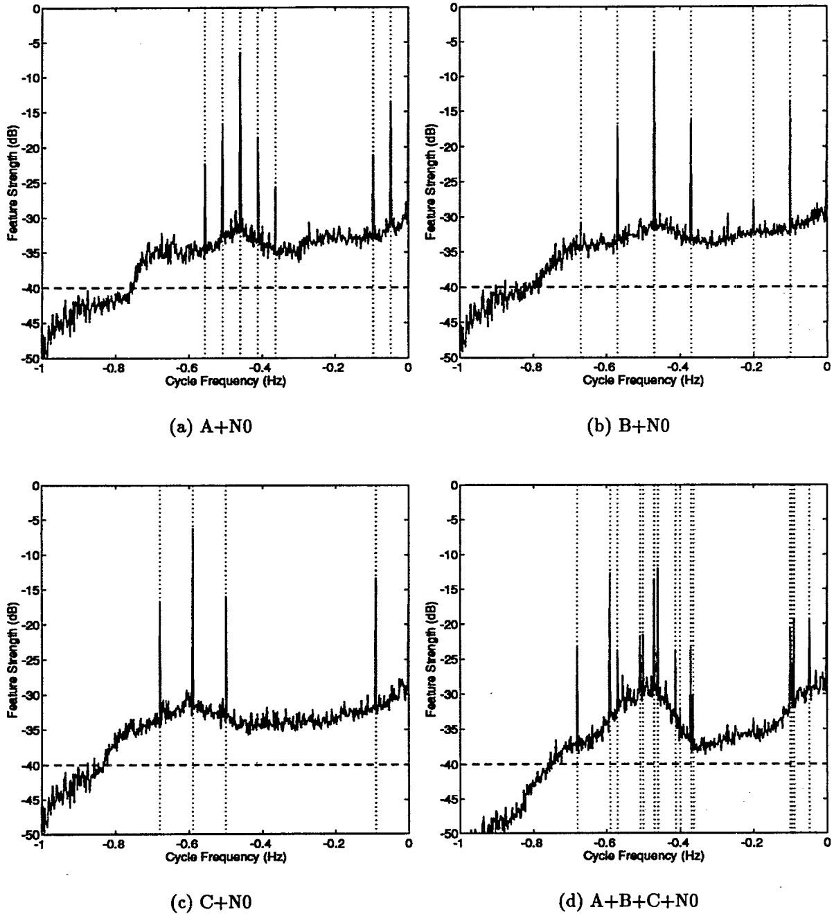
Figure 16: CFF of Various BPSK Signals in Noise N0 Using N=32768 , N_p=64 .
