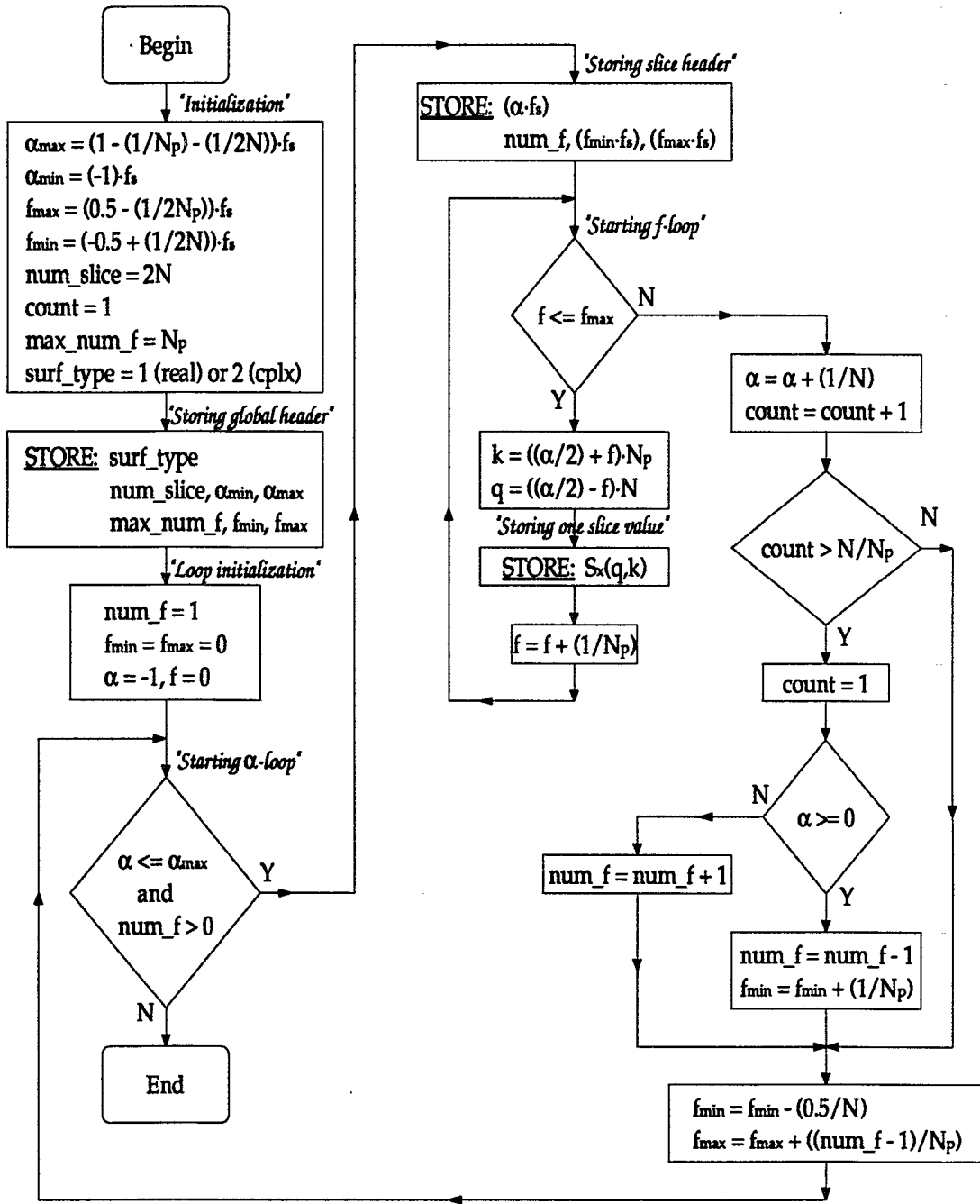
Figure 3: SSCA Mapping Algorithm.
