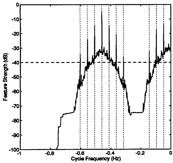
(c) A ( N=16384, Np=64 )
