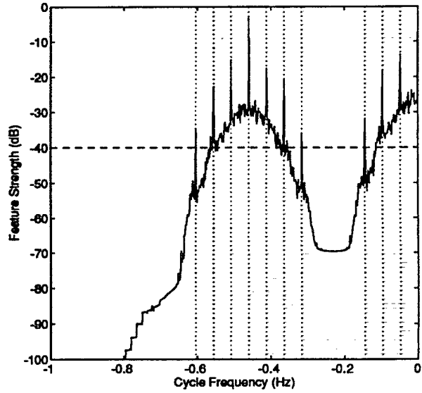
(b) A ( N=4096, Np=64 )
