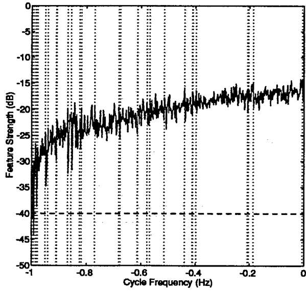
(a) N0 ( N=1024 , Np=64 )
