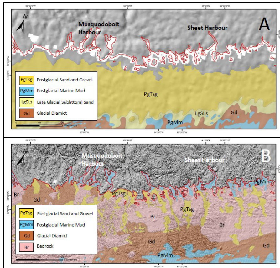
Figure 9: A) Base map (Fader et al. , 2004) and B) updates to the base map using King (2018) along the eastern shore of Nova Scotia between Jeddore and Moser River as well as multibeam sonar, LiDAR, Olex single beam sonar and DFO non-navigational bathymetric data (NONNA).
