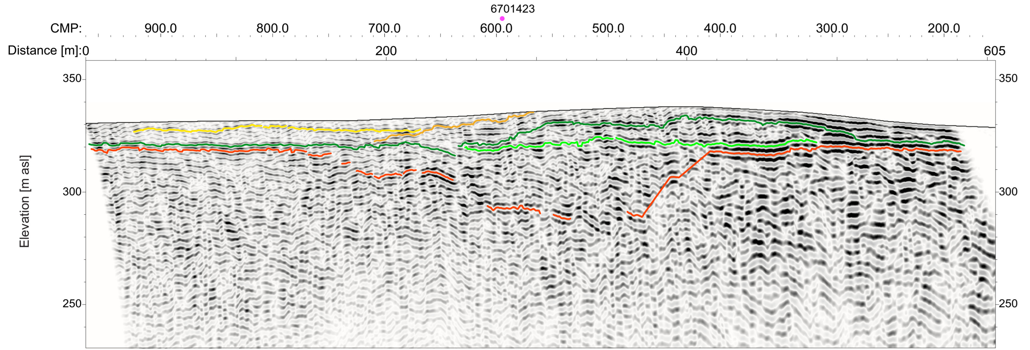
S-velocity (depth):
