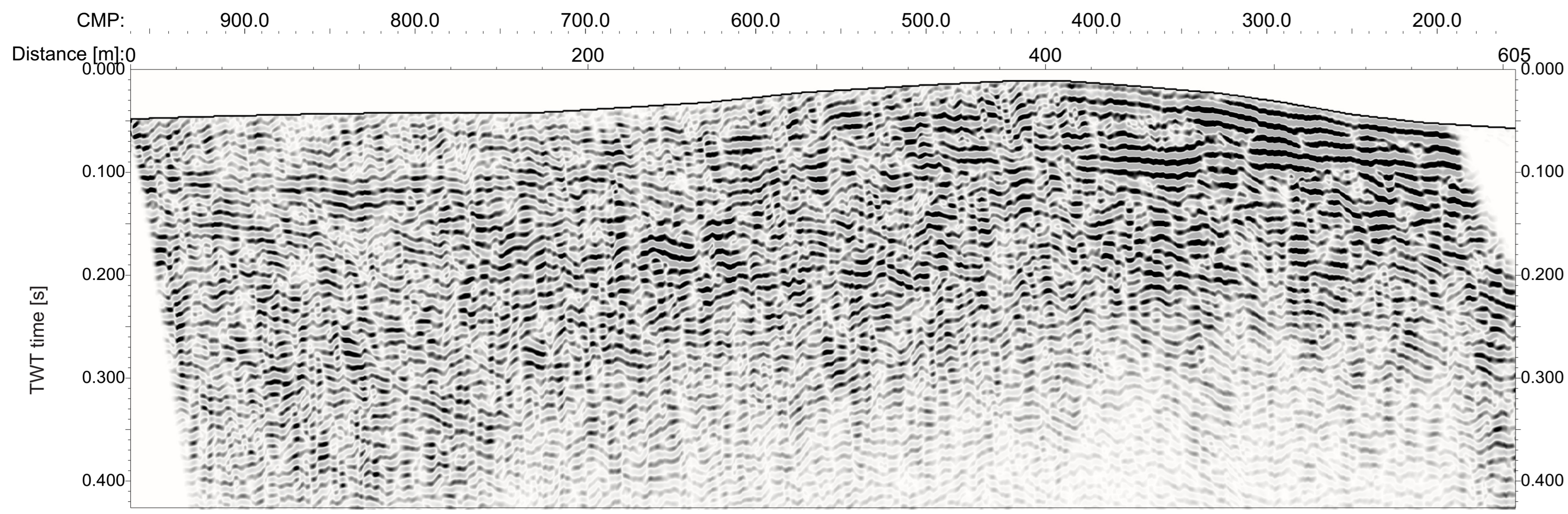
S-wave (depth):
