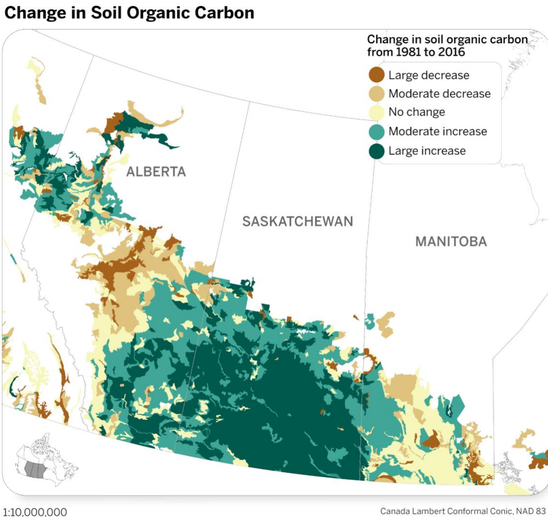
Figure 14 – Change in Soil Organic Carbon: Prairies (1981 to 2016)
