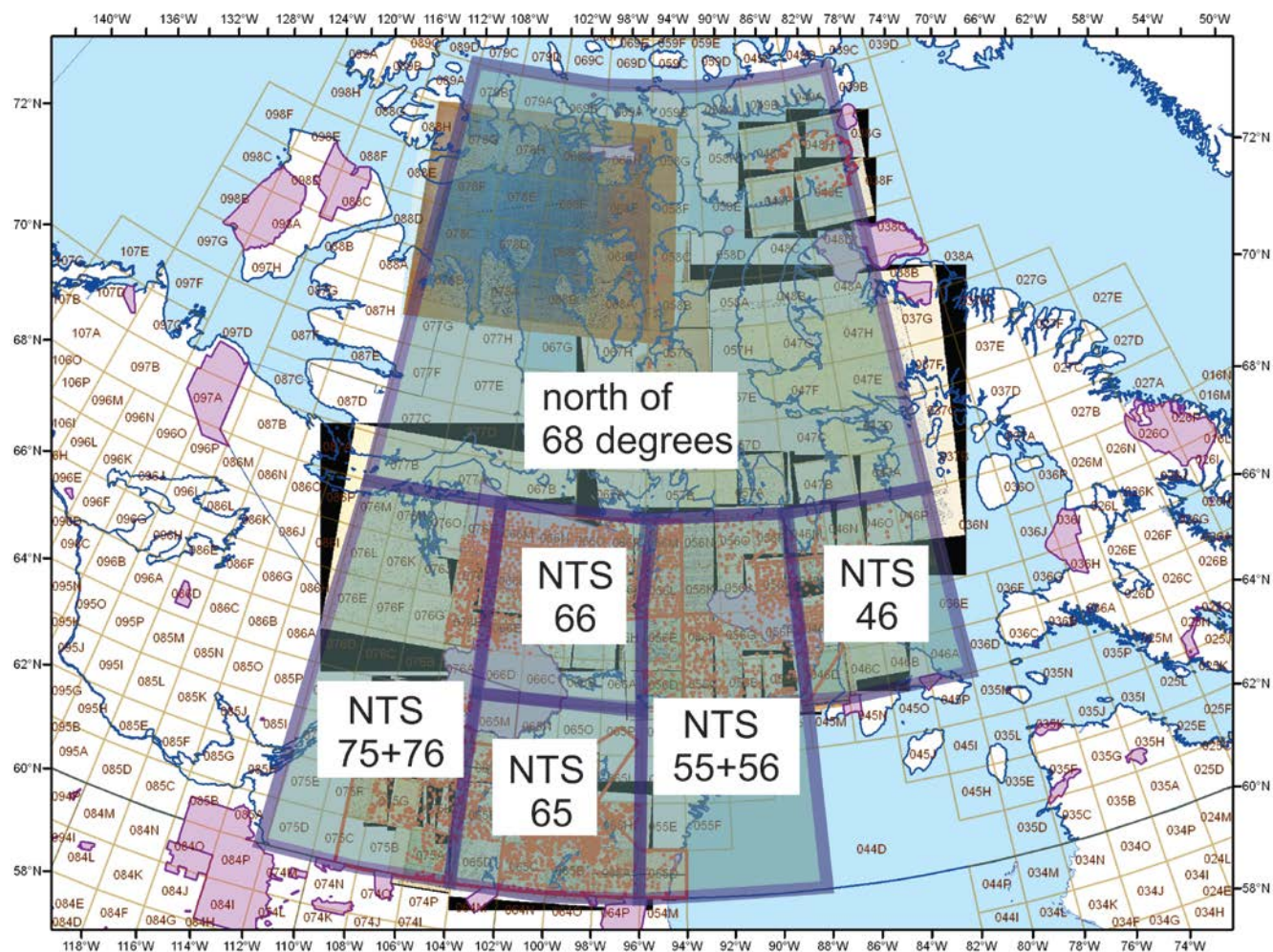
Figure 4. Distribution of the scanned traverse maps in Open Files 06 to XX11. Red dots are field stations digitized from these maps. Irregular purple polygons are protected areas.
