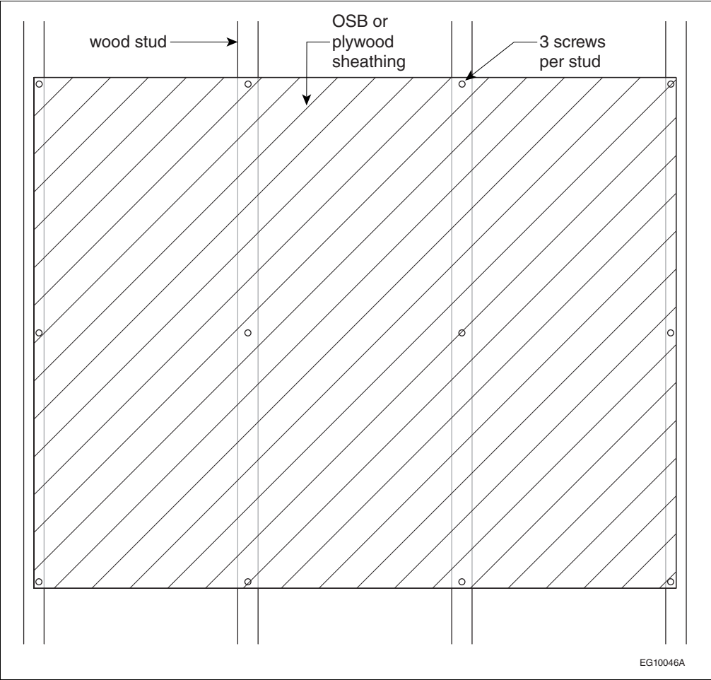
Figure A-9.31.2.3.(5) Example of an acceptable configuration for the attachment of OSB or plywood sheathing to span wood studs
