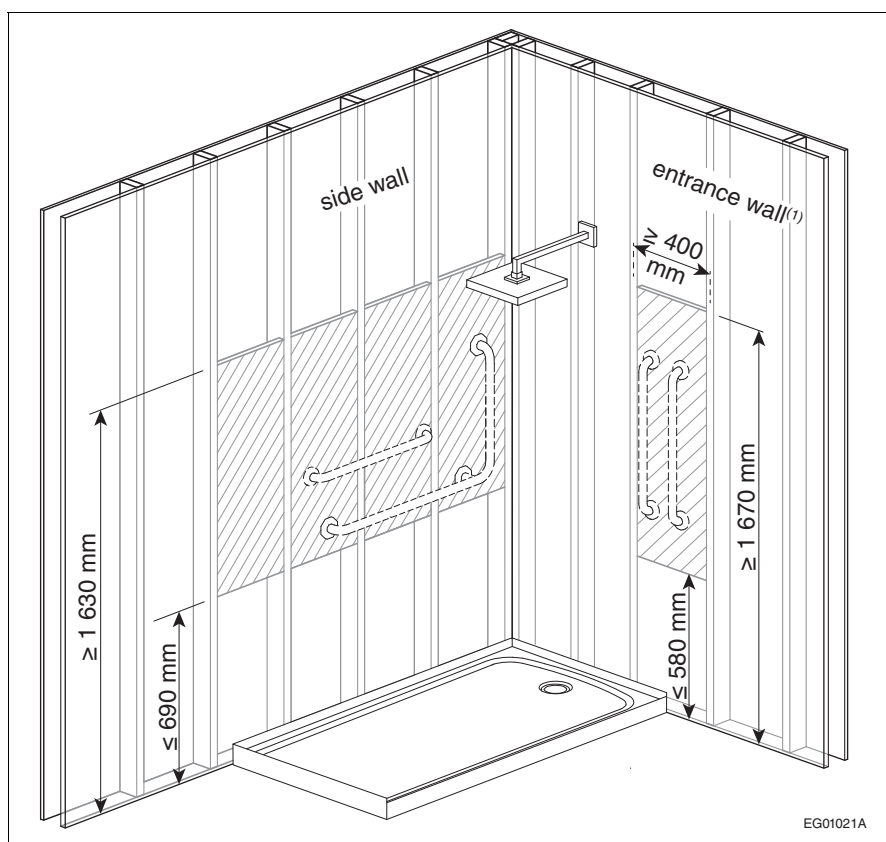
Figure A-3.8.4.4.(2) and (4)-A
