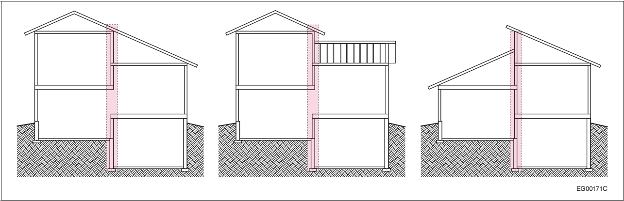
Figure A-9.23.13.4-C Braced wall bands at changes in floor level in split-level buildings (Sentence 9.23.13.4.(2))
