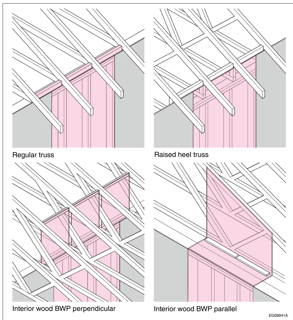
Figure A-9.23.13.5.(3) and (4)
