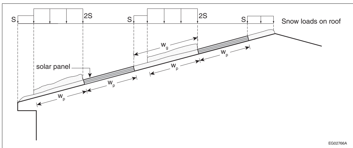
Figure A-4.1.6.16.(4)(b)
