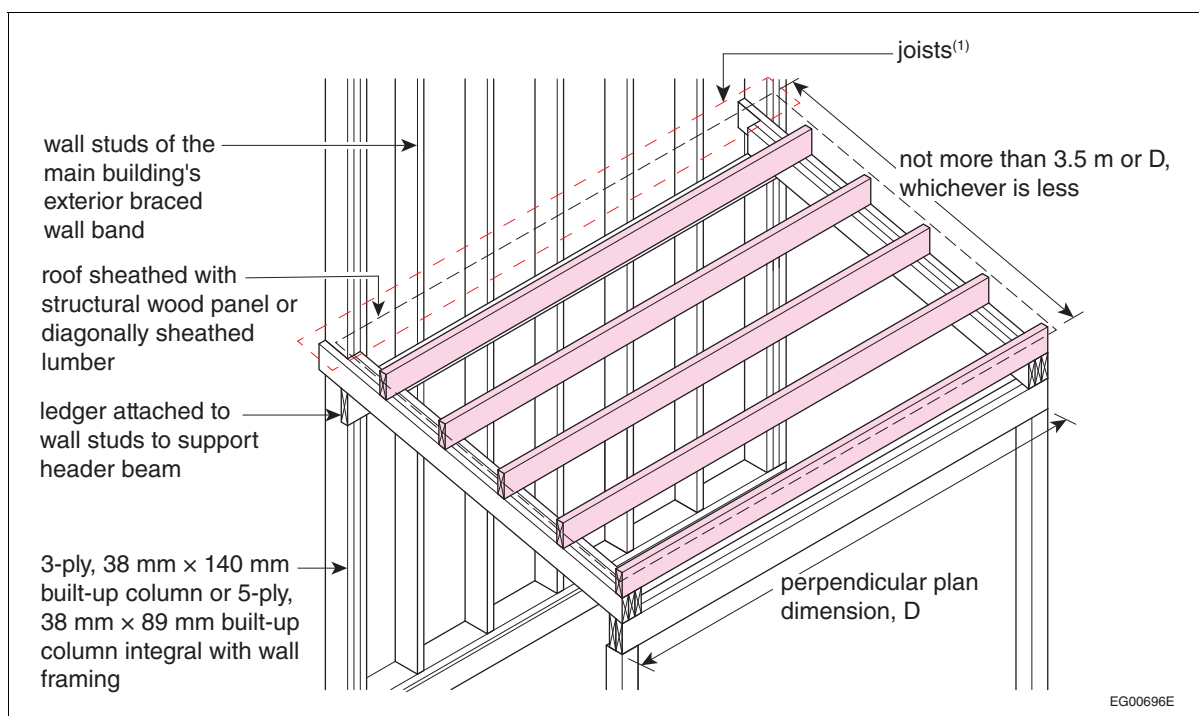
Figure A-9.23.13.12.(2)-B
