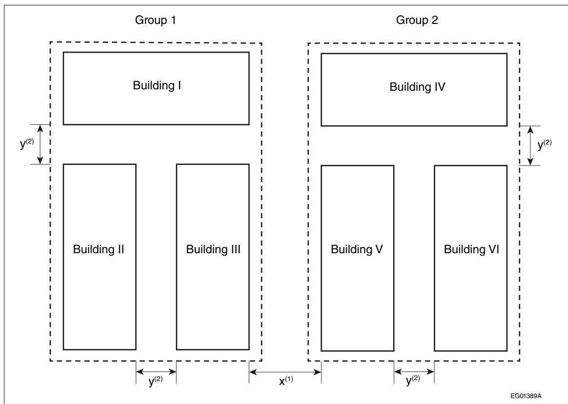
Figure A-3.9.2.2.
