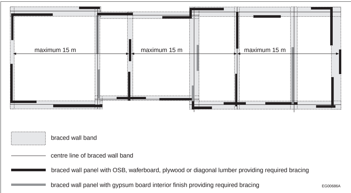
Figure A-9.23.13.6.(3) Braced wall panels constructed of wood-based sheathing in basements and crawl spaces
