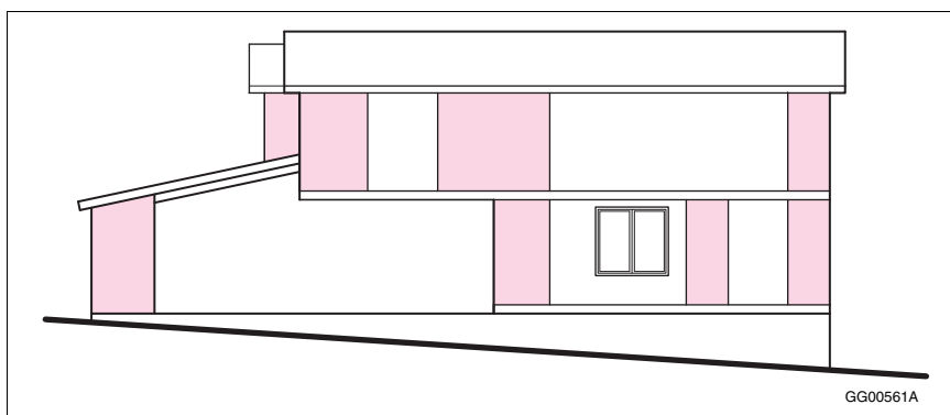
Figure A-9.23.13.9.(2) and (3)-G Intermittent braced wall panels in braced wall bands
