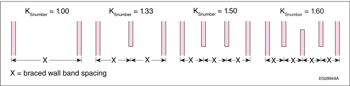
Figure A-9.23.13.9.(2) and (3)-F Adjustment for number of braced wall bands for resistance to seismic forces
