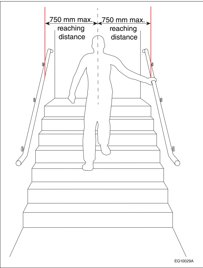
Figure A-3.4.6.5.(3)-A Stair where an intermediate handrail is not required by Clause 3.4.6.5.(3)(a)
