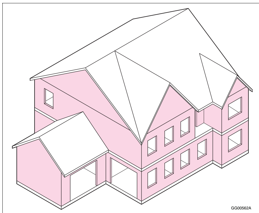
Figure A-9.23.13.9.(2) and (3)-H Continuously sheathed braced wall bands
