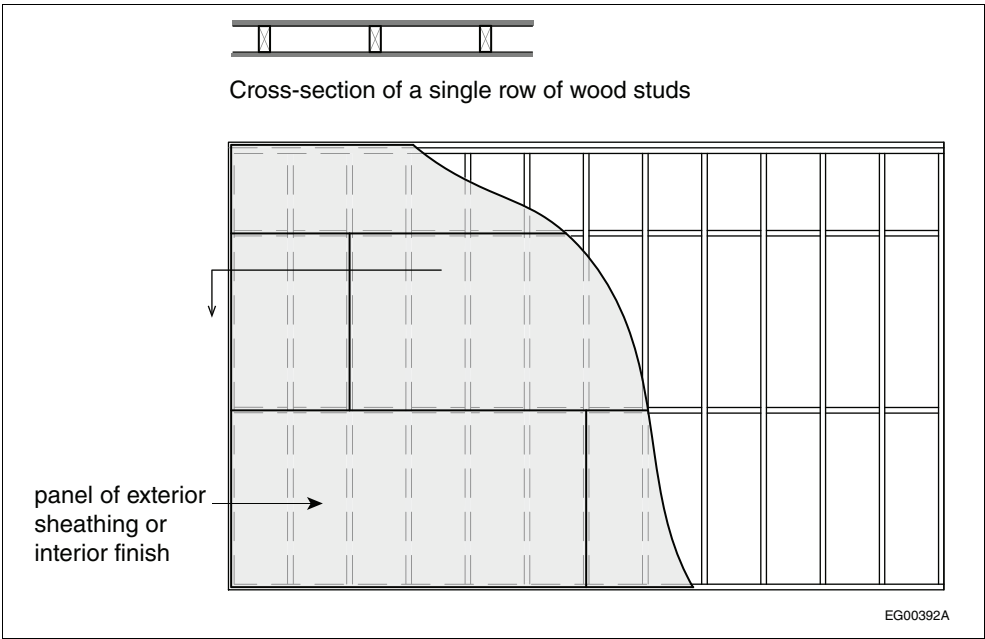
Figure A-9.10.3.1.-G Horizontal application of exterior wall sheathing or interior wall finish with all joints backed with lumber having the same dimensions as the framing members Note to Figure A-9.10.3.1.-G: (1) Figure is for illustrative purposes only and is not to scale.
