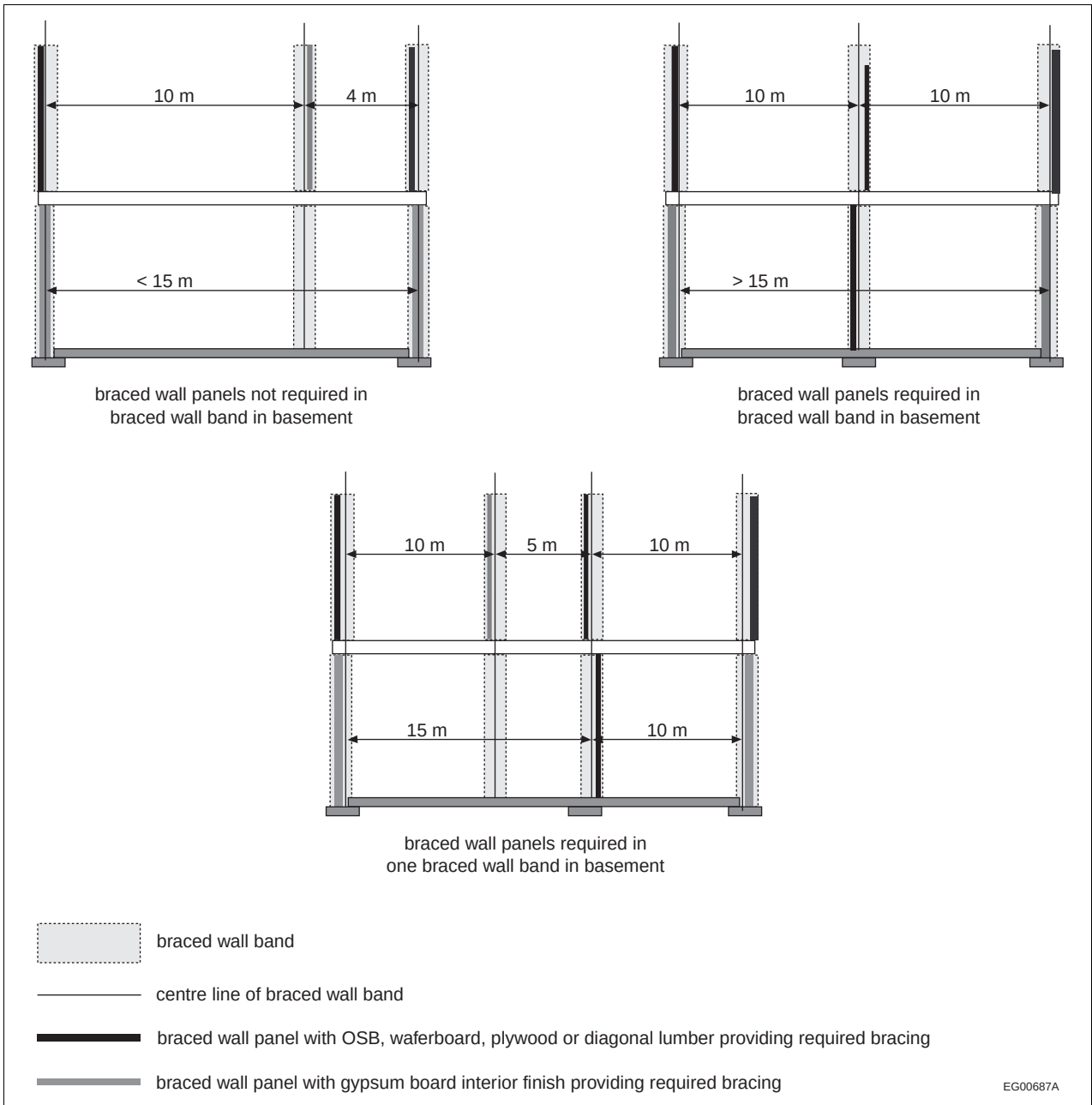
Figure A-9.23.13.5.(2)
