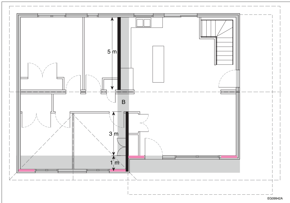
Figure A-9.23.13.6.(5)-A
