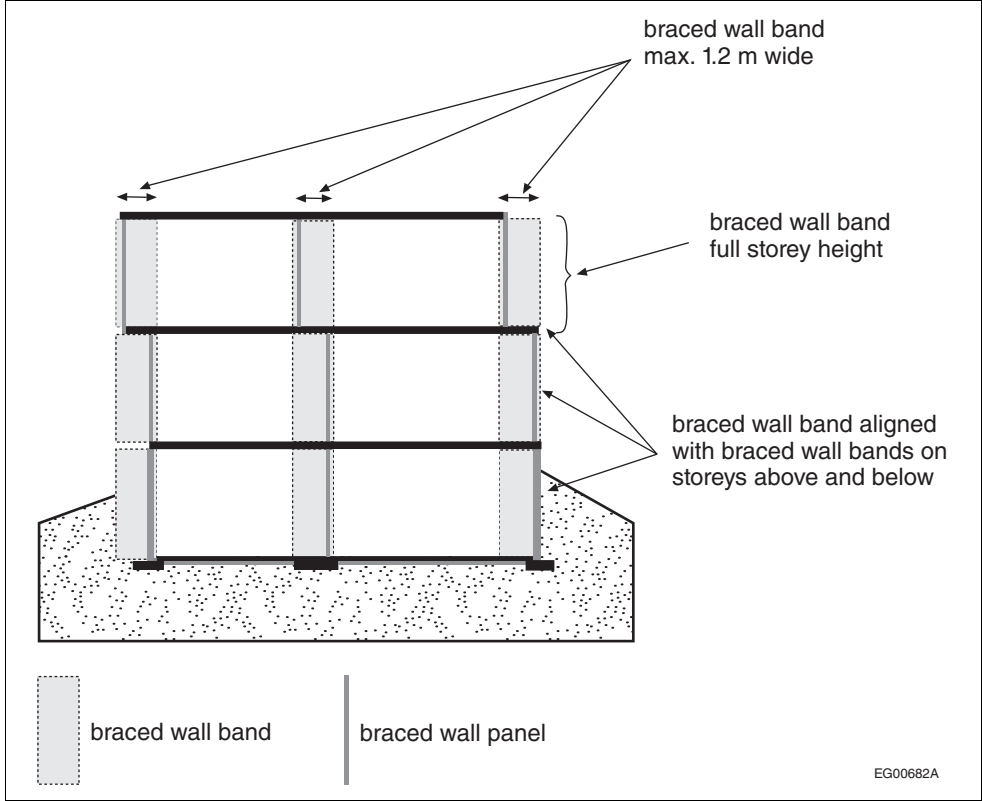
Figure A-9.23.13.4.-A Braced wall bands in an example building section (Clauses 9.23.13.4.(1)(b), (c) and (e))
