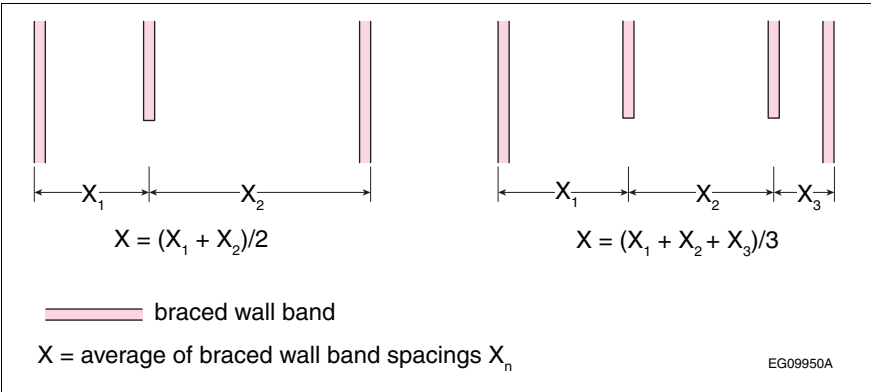
Figure A-9.23.13.9.(2) and (3)-E Calculation of average braced wall band spacing
