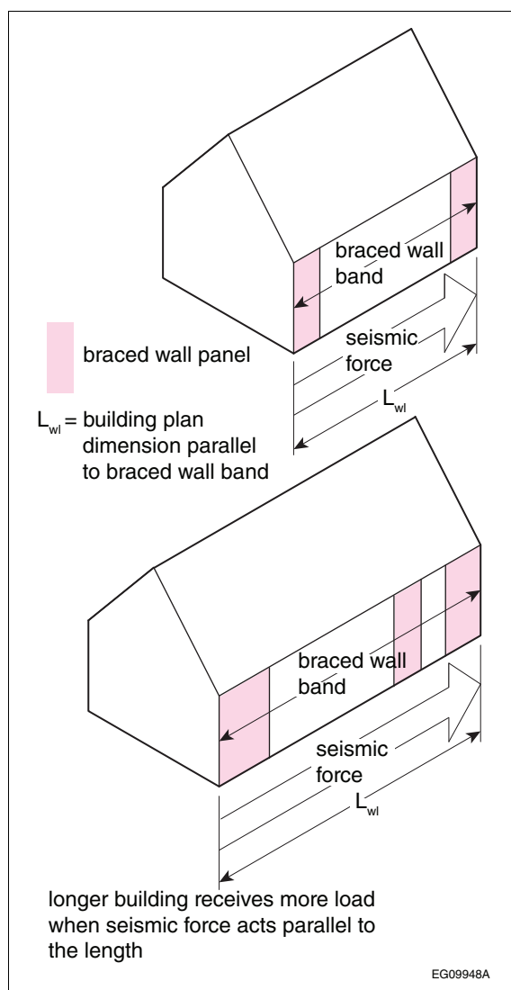
Figure A-9.23.13.9.(2) and (3)-B Seismic force on buildings with different lengths
