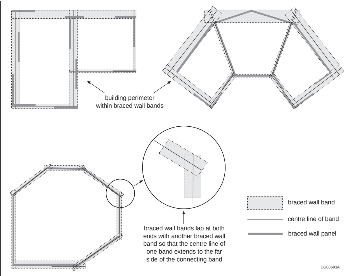
Figure A-9.23.13.4-B Lapping bands and building perimeter within braced wall bands (Clauses 9.23.13.4.(1)(a) and (d))
