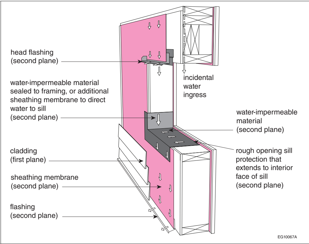
Figure A-9.27.2-A Second plane of protection maintained at the rough opening sill
