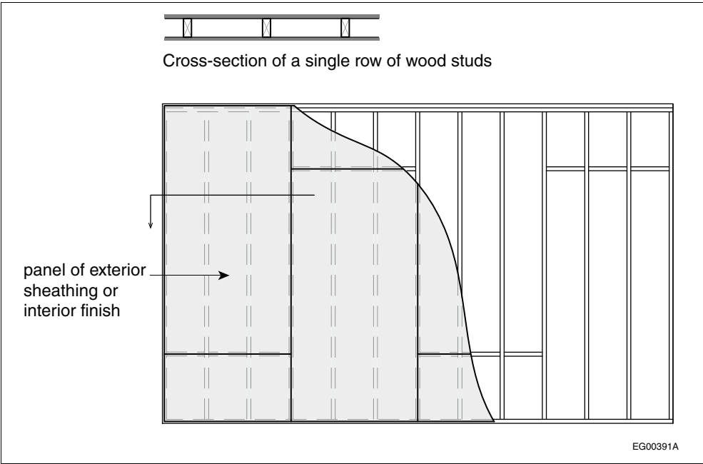
Figure A-9.10.3.1.-F Vertical application of exterior wall sheathing or interior wall finish with all joints backed with lumber having the same dimensions as the framing members Note to Figure A-9.10.3.1.-F: (1) Figure is for illustrative purposes only and is not to scale.
