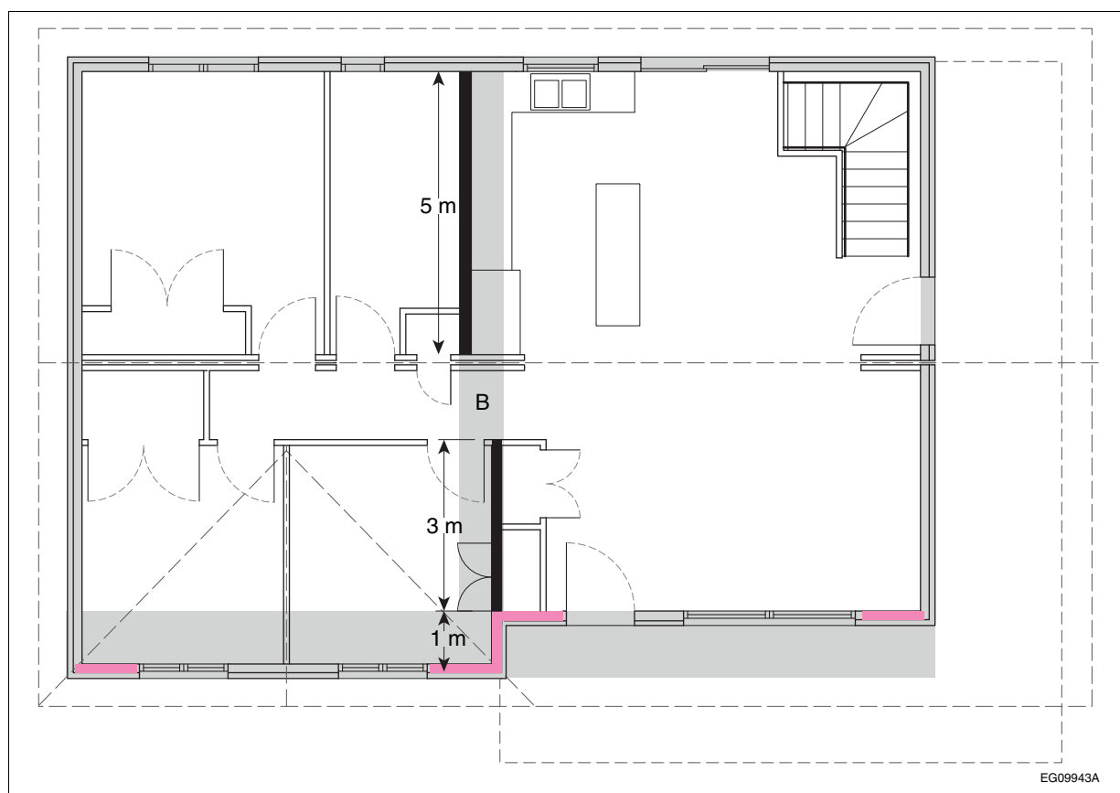
Figure A-9.23.13.6.(5)-B
