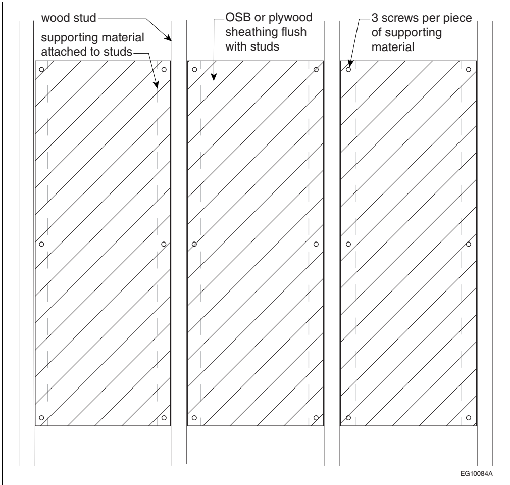
Figure A-9.31.2.3.(6) Example of an acceptable configuration for the attachment of OSB or plywood sheathing inset between wood studs
