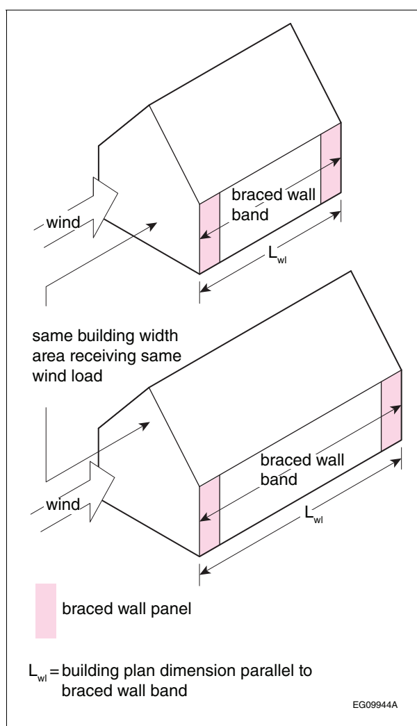
Figure A-9.23.13.9.(2) and (3)-A Wind force on buildings with different lengths
