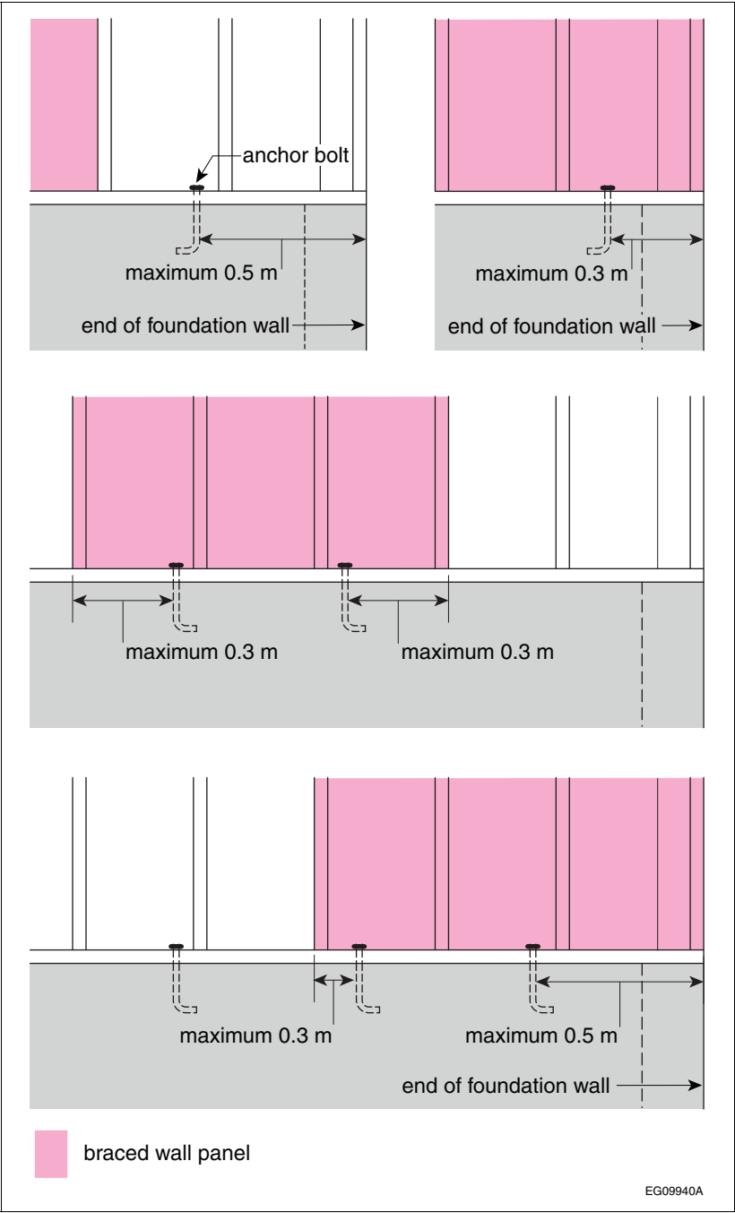
Figure A-9.23.6.1.(3) Anchorage of braced wall panels
