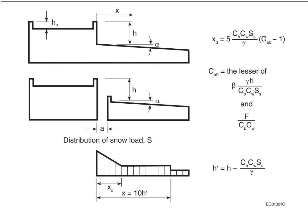
Figure 4.1.6.5.-A Snow load factors for lower level roofs Forming Part of Sentences 4.1.6.5.(1) and (3), Table 4.1.6.5.-A and Sentence 4.1.6.6.(1)
