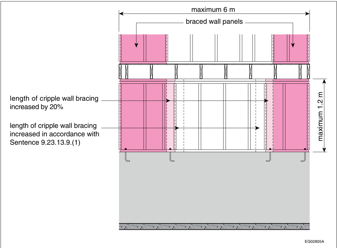
Figure A-9.23.13.10.(2) Foundation cripple wall where S_{max} \leq 0.60
