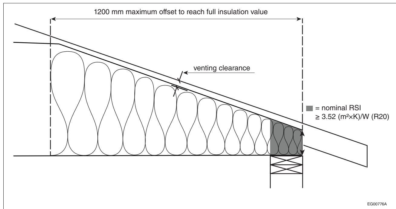
Figure A-9.36.2.6.(3)
