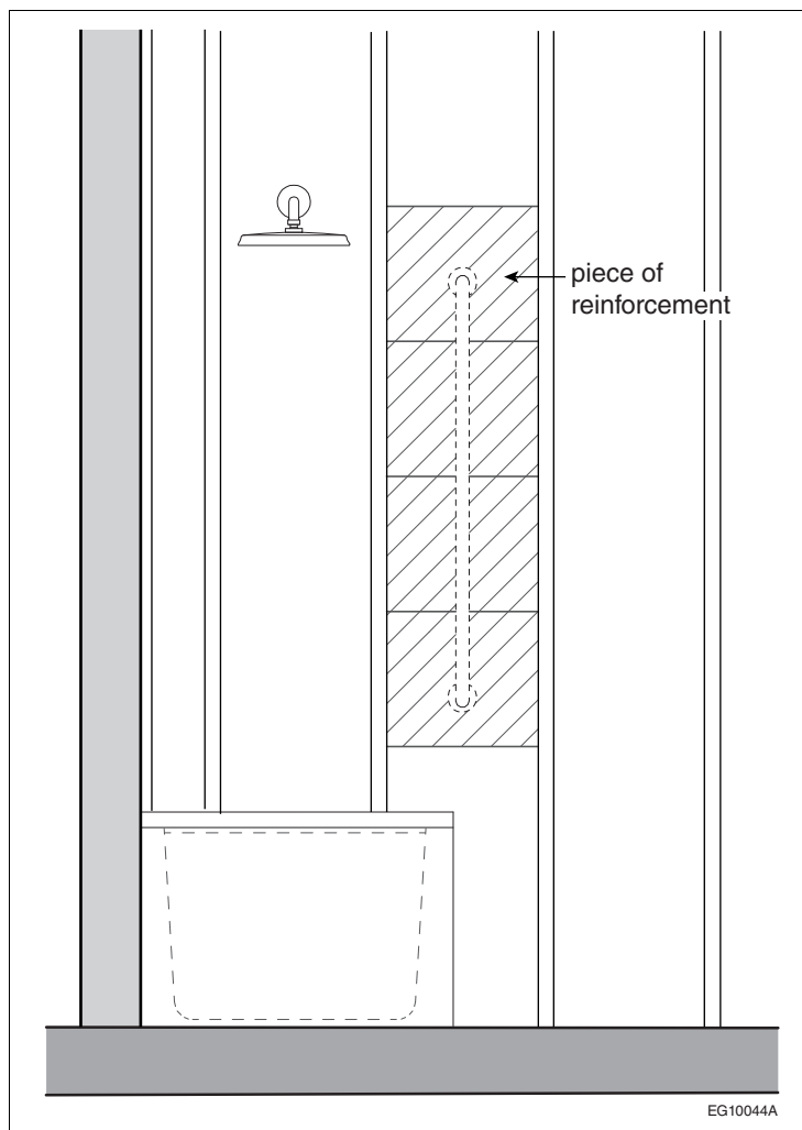
Figure A-9.31.2.3.(3) Multiple pieces of lumber or OSB or plywood sheathing used as reinforcement
