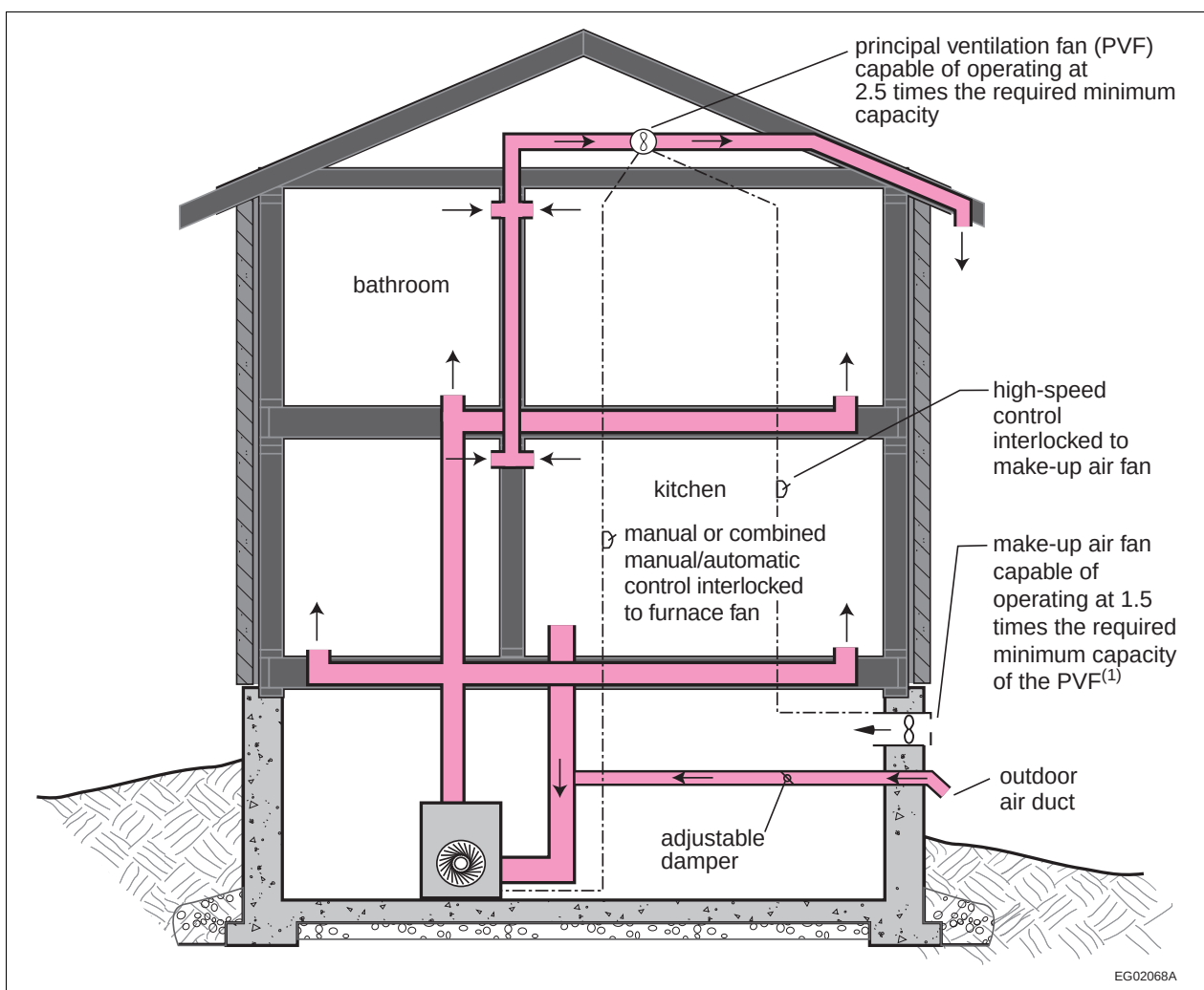
Figure A-9.32.3.3-E
