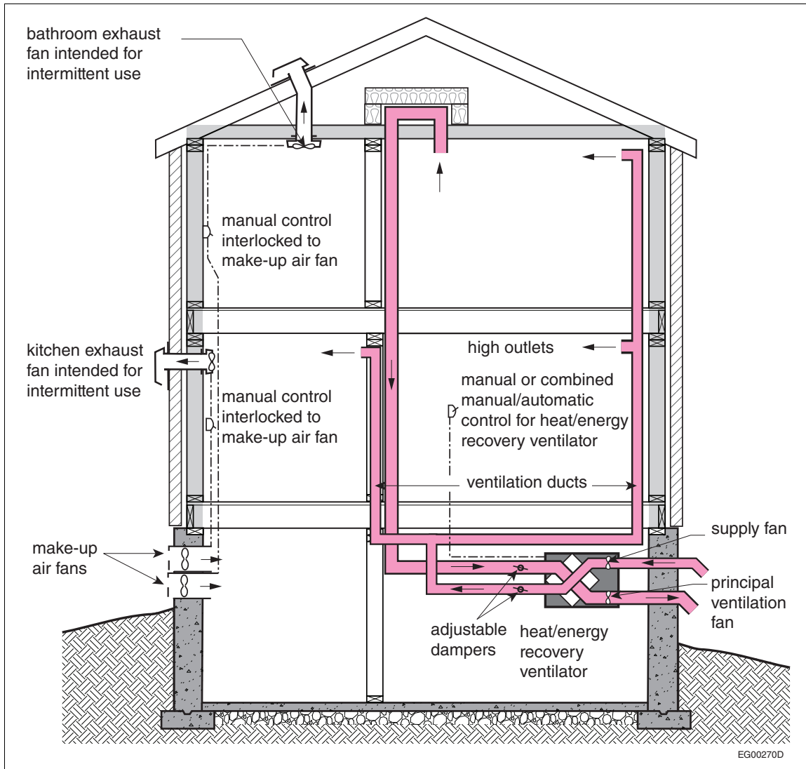
Figure A-9.32.3.3.-D
