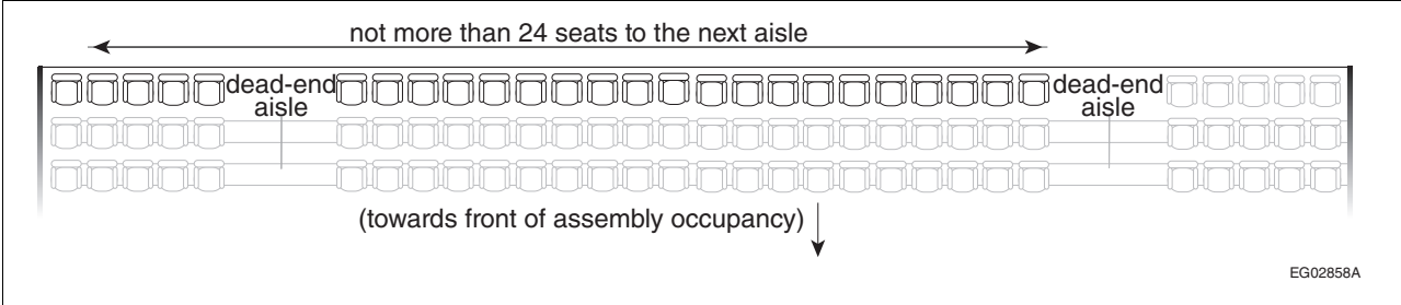
Figure A-3.3.2.5.(5) Twenty-four seat count to another aisle
