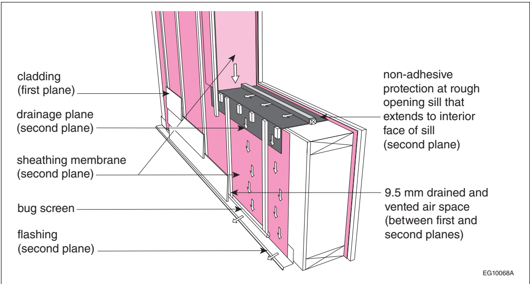
Figure A-9.27.2-B Rain control assembly with second plane of protection composed of a drained and vented air space system
