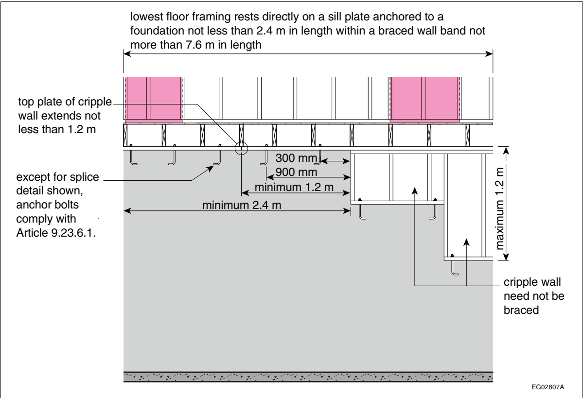
Figure A-9.23.13.11.(1) Cripple wall in a stepped foundation
