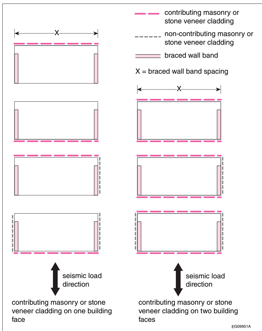
Figure A-9.23.13.9.(2) and (3)-D Contribution of masonry or stone veneer cladding to seismic loading
