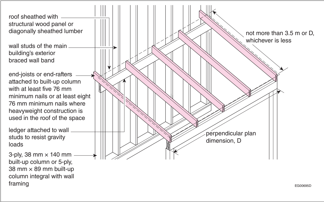
Figure A-9.23.13.12.(2)-A Porch roof framing perpendicular to wall framing between floors
