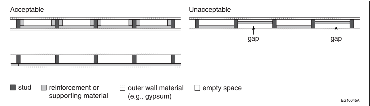
Figure A-9.31.2.3.(7) Top view of examples of wall assemblies with acceptable and unacceptable configurations of the reinforcement material with respect to the outer wall material
