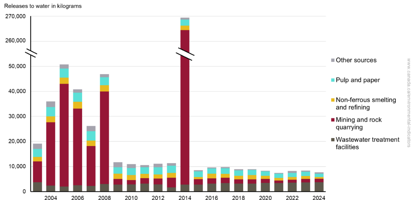
Figure 11. Facility-based arsenic releases to water by source, Canada, 2003 to 2024
