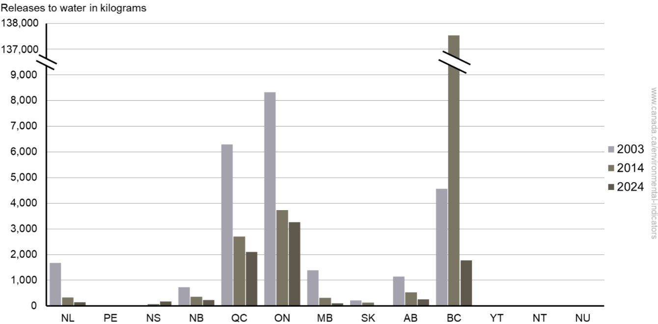
Figure 6. Facility-based lead releases to water by province and territory, Canada, 2003, 2014 and 2024
