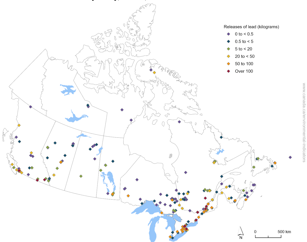
Figure 7. Releases of lead to water by facility, Canada, 2024
