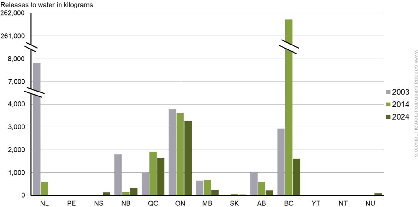
Figure 12. Facility-based arsenic releases to water by province and territory, Canada, 2003, 2014 and 2024
