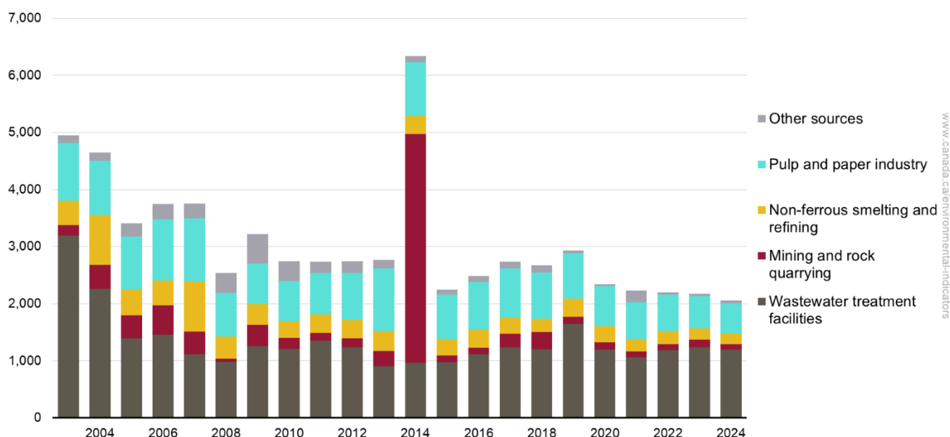
Figure 8. Facility-based cadmium releases to water by source, Canada, 2003 to 2024
