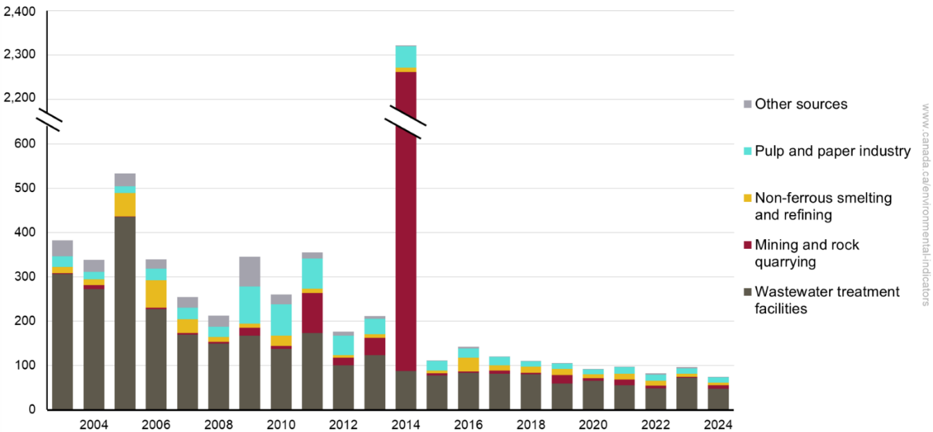
Figure 2. Facility-based mercury releases to water by source, Canada, 2003 to 2024
