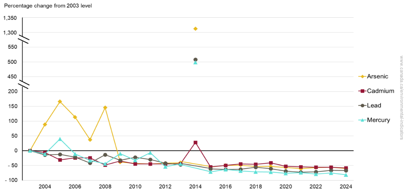
Figure 1. Facility-based releases of mercury, lead, cadmium and arsenic to water, Canada, 2003 to 2024
