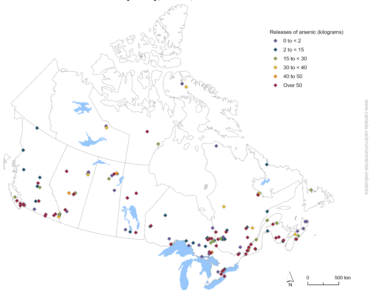
Figure 13. Releases of arsenic to water by facility, Canada, 2024
