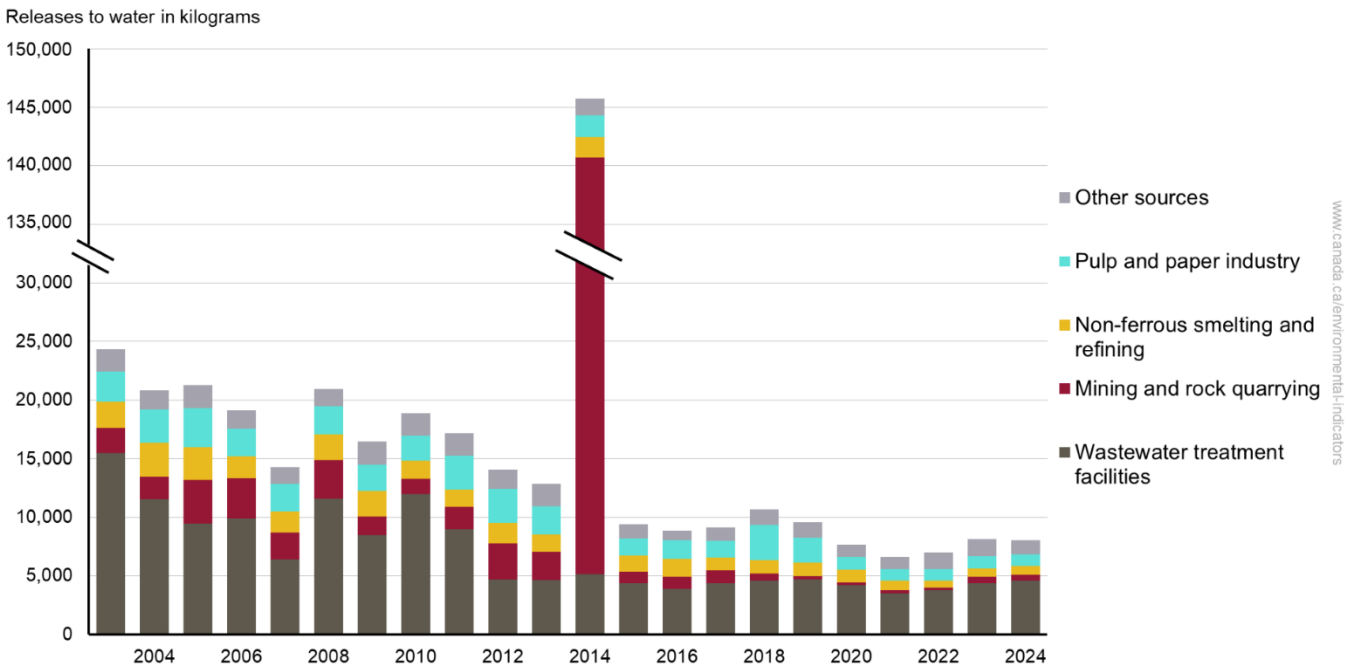
Figure 5. Facility-based lead releases to water by source, Canada, 2003 to 2024
