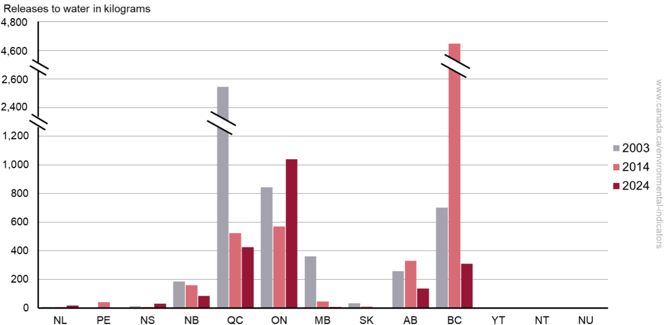
Figure 9. Facility-based cadmium releases to water by province and territory, Canada, 2003, 2014 and 2024
