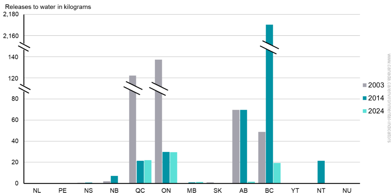
Figure 3. Facility-based mercury releases to water by province and territory, Canada, 2003, 2014 and 2024
