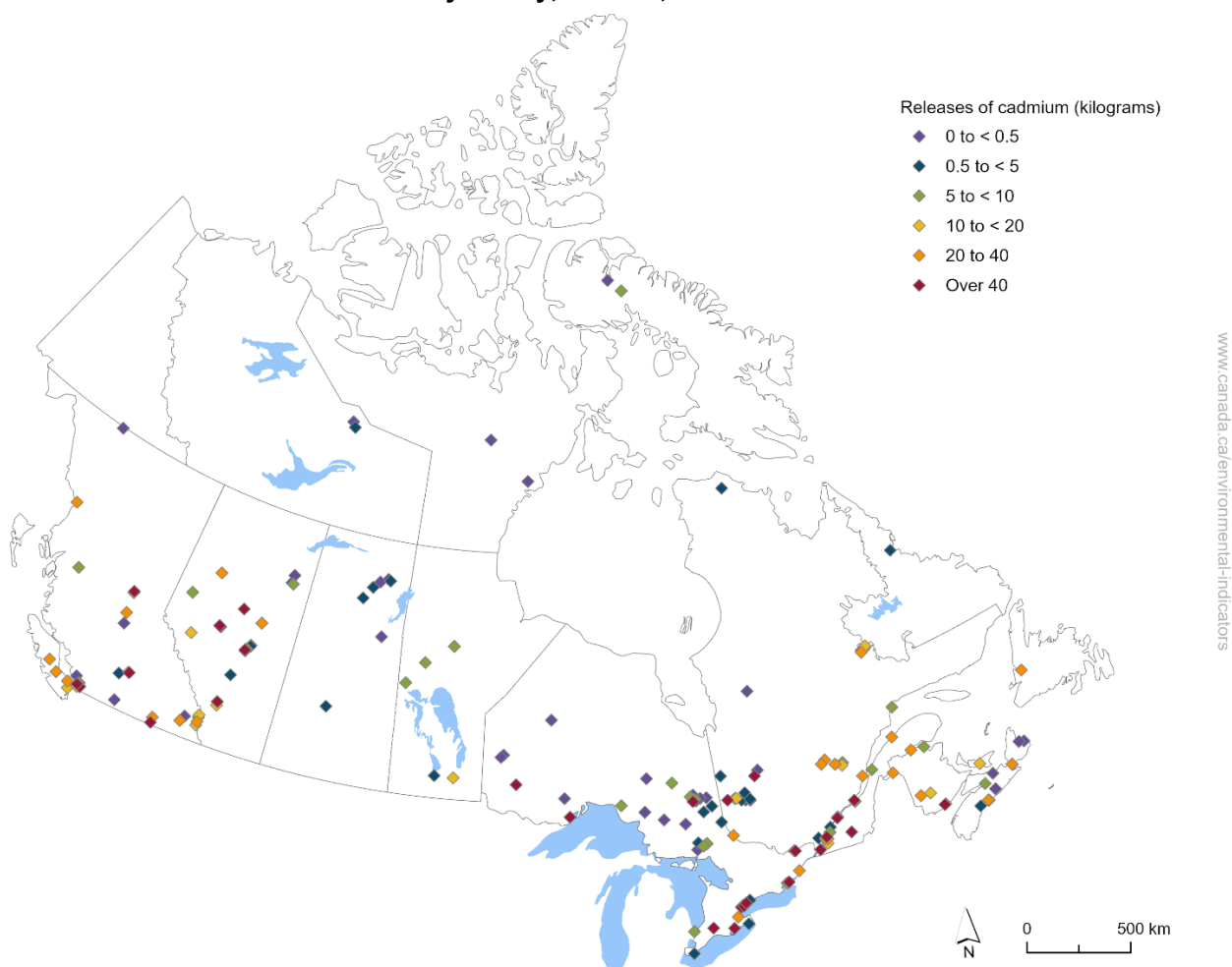
Figure 10. Releases of cadmium to water by facility, Canada, 2024
