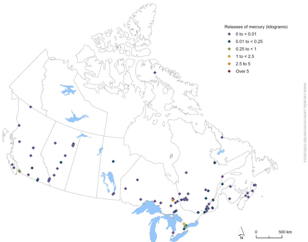
Figure 4. Releases of mercury to water by facility, Canada, 2024
