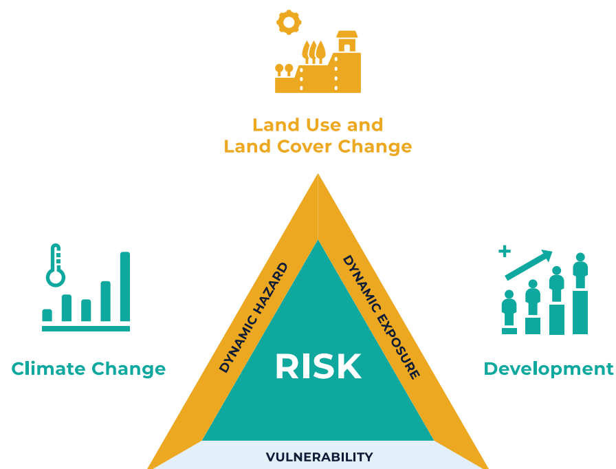
Figure 1-5: Simple model of risk showing changing hazard and exposure with land use and land cover change.
