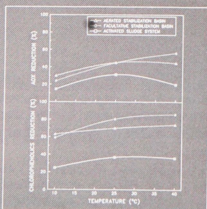
Figure 1. Relationship Between Organochlorine Removal Efficiency and Temperature
