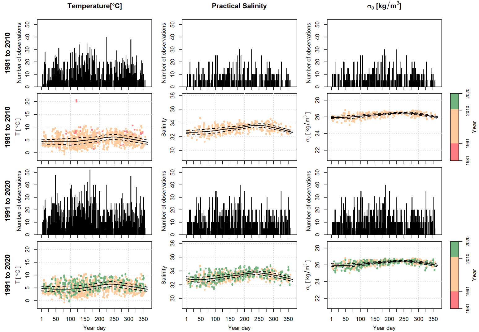
Figure 25. The 112.5m to 117.5m depth bin total number of observations per year day for the 1981 to 2010 (top row) and the 1991 to 2020 (third row) reference period and the scatter plot of data, color coded by year, with the mean (thick black line) and \pm 1 SD (dashed black line) local polynomial regression fits for the 1981 to 2010 (second row) and the 1991 to 2020 (bottom row) reference period for temperature (left column), salinity (middle column), and density (right column).
