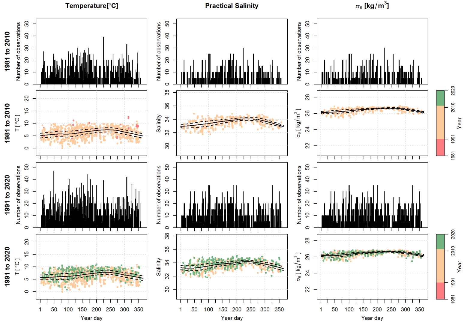
Figure 29. The 132.5m to 137.5m depth bin total number of observations per year day for the 1981 to 2010 (top row) and the 1991 to 2020 (third row) reference period and the scatter plot of data, color coded by year, with the mean (thick black line) and \pm 1 SD (dashed black line) local polynomial regression fits for the 1981 to 2010 (second row) and the 1991 to 2020 (bottom row) reference period for temperature (left column), salinity (middle column), and density (right column).
