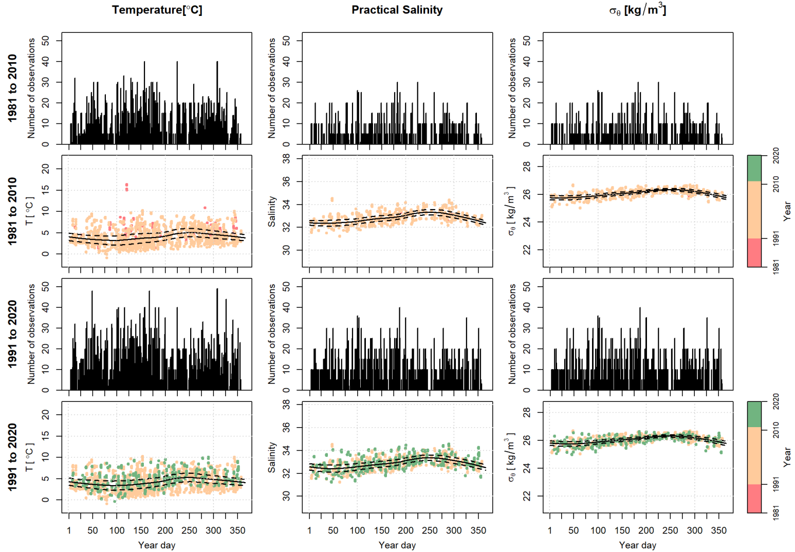
Figure 22. The 97.5m to 102.5m depth bin total number of observations per year day for the 1981 to 2010 (top row) and the 1991 to 2020 (third row) reference period and the scatter plot of data, color coded by year, with the mean (thick black line) and \pm 1 SD (dashed black line) local polynomial regression fits for the 1981 to 2010 (second row) and the 1991 to 2020 (bottom row) reference period for temperature (left column), salinity (middle column), and density (right column).
