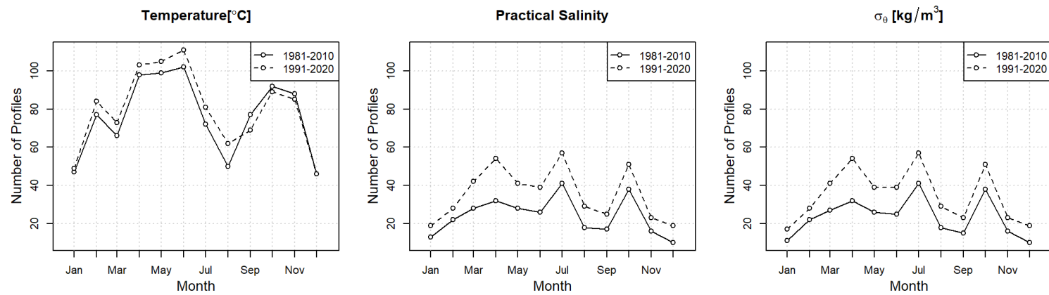
Figure 34. Monthly number of occupations for both climatology reference periods for temperature (left), salinity (middle), and density (right).
