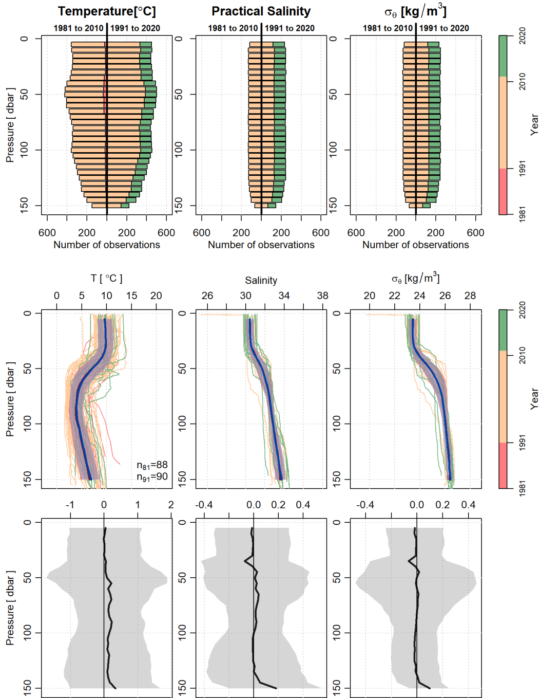
Figure 45. The November number of observations for each climatology reference period, as indicated by the label on the top axis, color coded by year (top row). Mean profiles (thick line) and the \pm 0.5\text{SD} (indicated by shading) for the 1981 to 2010 reference period (red) and 1991 to 2020 reference period (blue) (middle row). Thin lines, color coded by year, are the profile observations that were used in the mean and standard deviation calculations. The difference, 1991 to 2020 minus 1981 to 2010, of the two mean profiles and \pm 0.5\text{SD} for temperature (bottom left), salinity (bottom middle), and density (bottom right). Vertical thin black line denotes a difference of zero.
