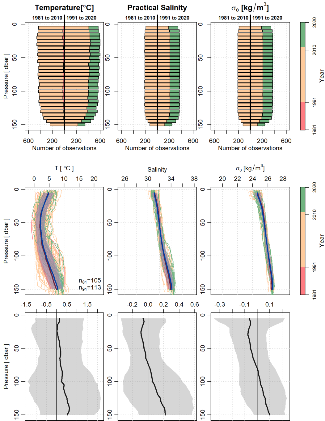
Figure 39. The May number of observations for each climatology reference period, as indicated by the label on the top axis, color coded by year (top row). Mean profiles (thick line) and the \pm 0.5SD (indicated by shading) for the 1981 to 2010 reference period (red) and 1991 to 2020 reference period (blue) (middle row). Thin lines, color coded by year, are the profile observations that were used in the mean and standard deviation calculations. The difference, 1991 to 2020 minus 1981 to 2010, of the two mean profiles and \pm 0.5SD for temperature (bottom left), salinity (bottom middle), and density (bottom right). Vertical thin black line denotes a difference of zero.
