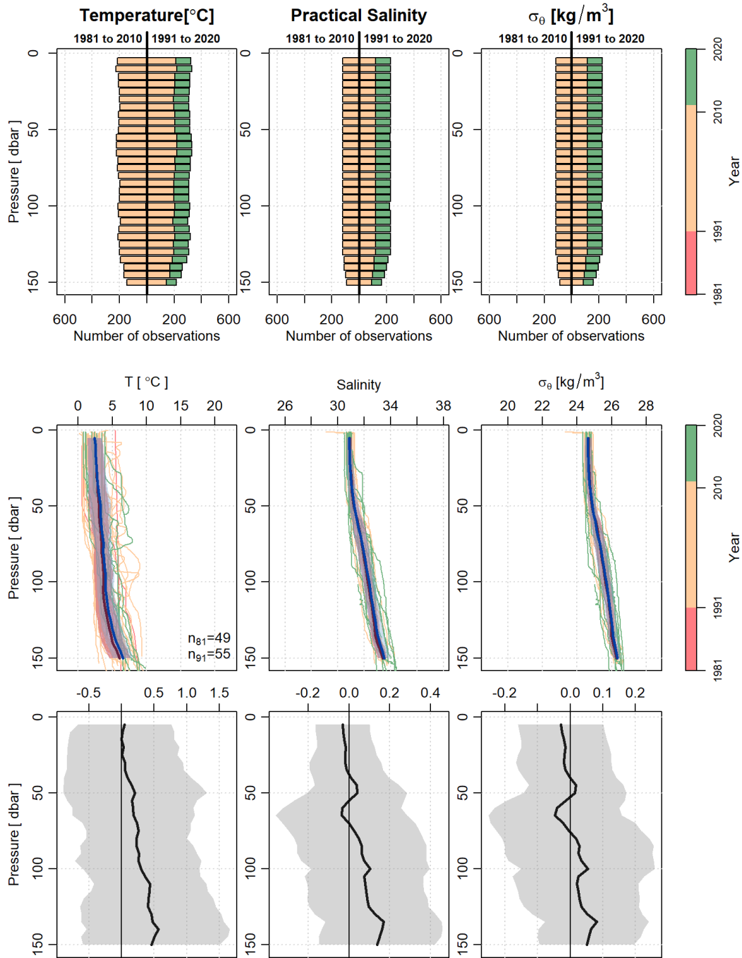
Figure 35. The January number of observations for each climatology reference period, as indicated by the label on the top axis, color coded by year (top row). Mean profiles (thick line) and the \pm 0.5SD (indicated by shading) for the 1981 to 2010 reference period (red) and 1991 to 2020 reference period (blue) (middle row). Thin lines, color coded by year, are the profile observations that were used in the mean and standard deviation calculations. The difference, 1991 to 2020 minus 1981 to 2010, of the two mean profiles and \pm 0.5SD for temperature (bottom left), salinity (bottom middle), and density (bottom right). Vertical thin black line denotes a difference of zero.
