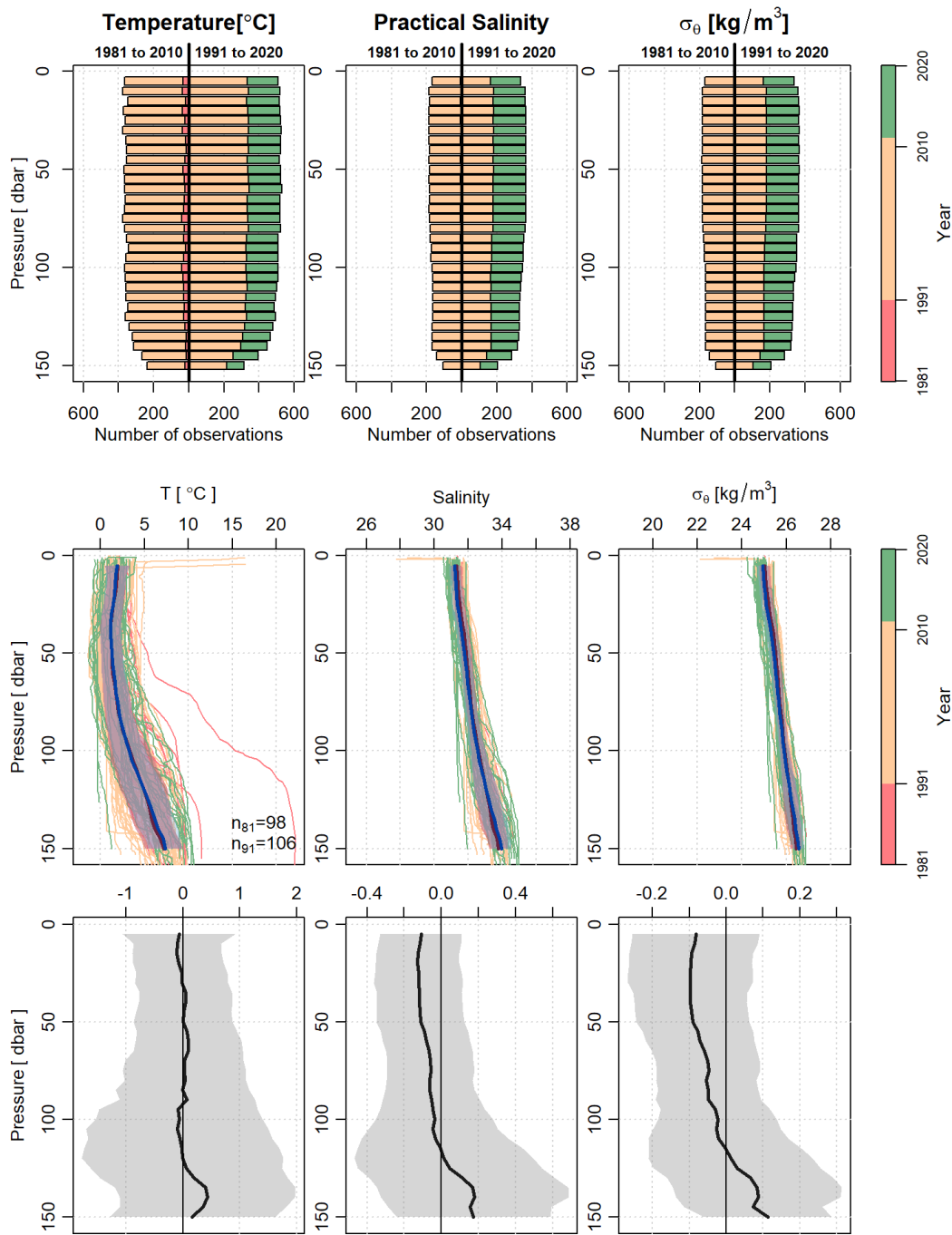
Figure 38. The April number of observations for each climatology reference period, as indicated by the label on the top axis, color coded by year (top row). Mean profiles (thick line) and the \pm 0.5\text{SD} (indicated by shading) for the 1981 to 2010 reference period (red) and 1991 to 2020 reference period (blue) (middle row). Thin lines, color coded by year, are the profile observations that were used in the mean and standard deviation calculations. The difference, 1991 to 2020 minus 1981 to 2010, of the two mean profiles and \pm 0.5\text{SD} for temperature (bottom left), salinity (bottom middle), and density (bottom right). Vertical thin black line denotes a difference of zero.
