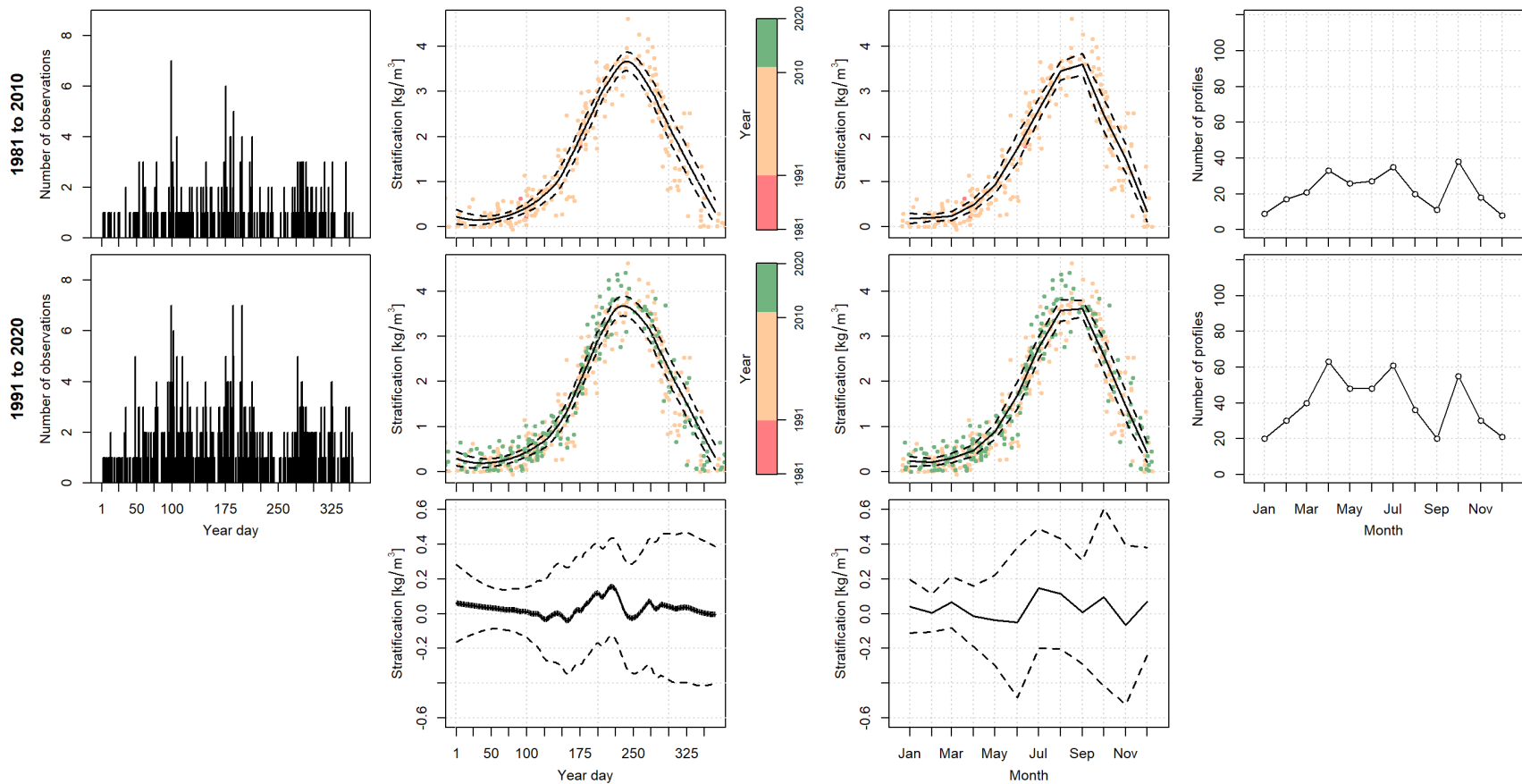
Figure 50. The stratification calculated between depths 5 to 50m, from left to right, the total number of calculated values per year day, the daily mean local polynomial regression fits (thick black line) and \pm 0.5 SD (dashed black lines) with a scatter plot of the calculated values colour coded by year, the monthly mean (thick black line) and \pm 0.5 SD (dashed black lines) with a scatter plot of the calculated values colour coded by year, and the total number of observations per month for the 1981 to 2010 (top row) and 1991 to 2020 (middle row) climatology reference periods. The difference (1991 to 2020 minus the 1981 to 2010) of the climatology reference periods mean (thick black line) and the propagated uncertainty (dashed black lines) for the daily and monthly fits (bottom row).
