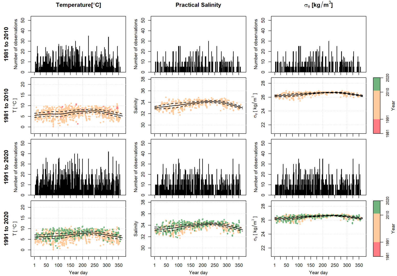
Figure 30. The 137.5m to 142.5m depth bin total number of observations per year day for the 1981 to 2010 (top row) and the 1991 to 2020 (third row) reference period and the scatter plot of data, color coded by year, with the mean (thick black line) and \pm 1 SD (dashed black line) local polynomial regression fits for the 1981 to 2010 (second row) and the 1991 to 2020 (bottom row) reference period for temperature (left column), salinity (middle column), and density (right column).
