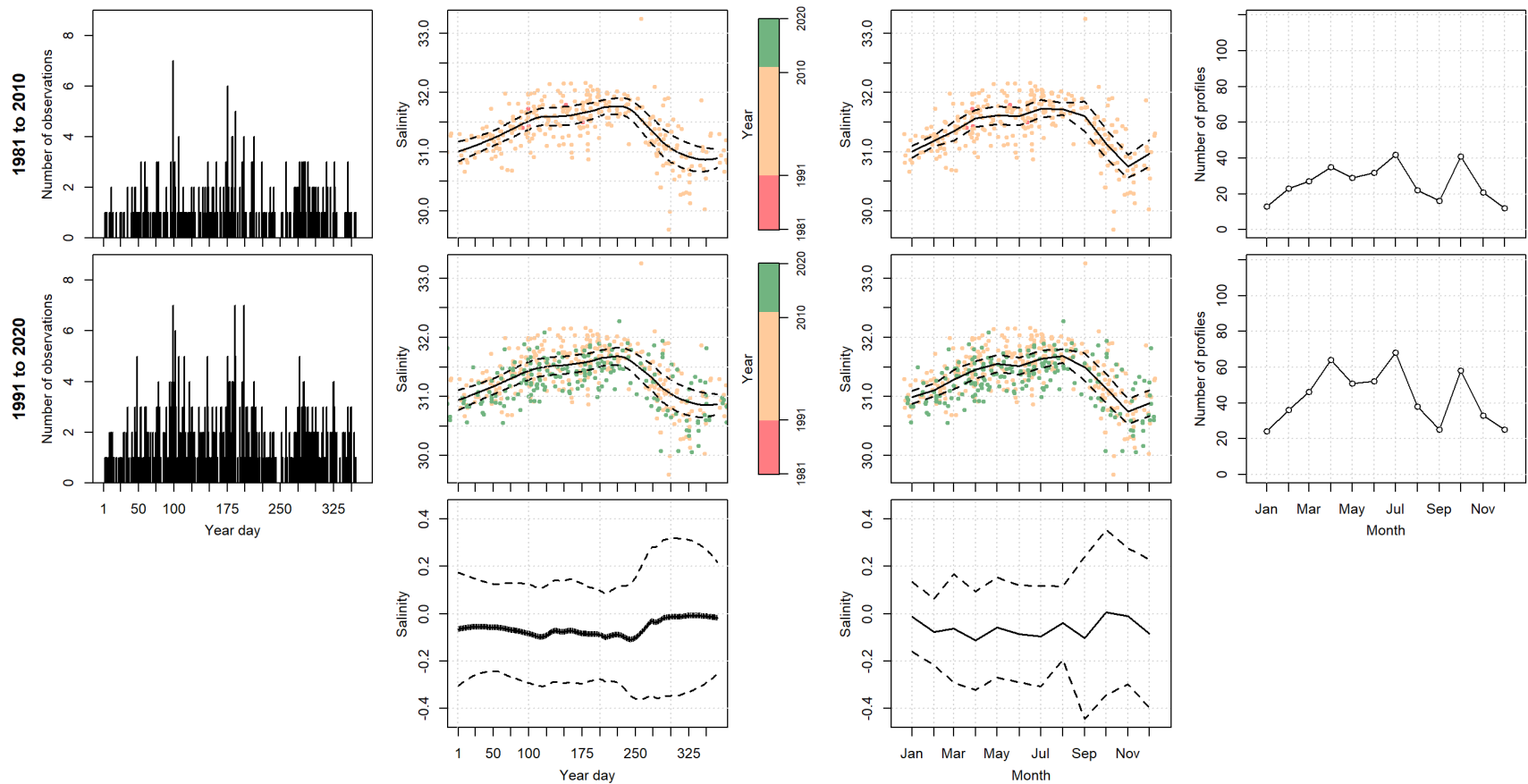
Figure 49. The integrated salinity over depths 5 to 50m, from left to right, the total number of calculated values per year day, the daily mean local polynomial regression fits (thick black line) and \pm 0.5SD (dashed black lines) with a scatter plot of the calculated values colour coded by year, the monthly mean (thick black line) and \pm 0.5SD (dashed black lines) with a scatter plot of the calculated values colour coded by year, and the total number of observations per month for the 1981 to 2010 (top row) and 1991 to 2020 (middle row) climatology reference periods. The difference (1991 to 2020 minus the 1981 to 2010) of the climatology reference periods mean (thick black line) and the propagated uncertainty (dashed black lines) for the daily and monthly fits (bottom row).
