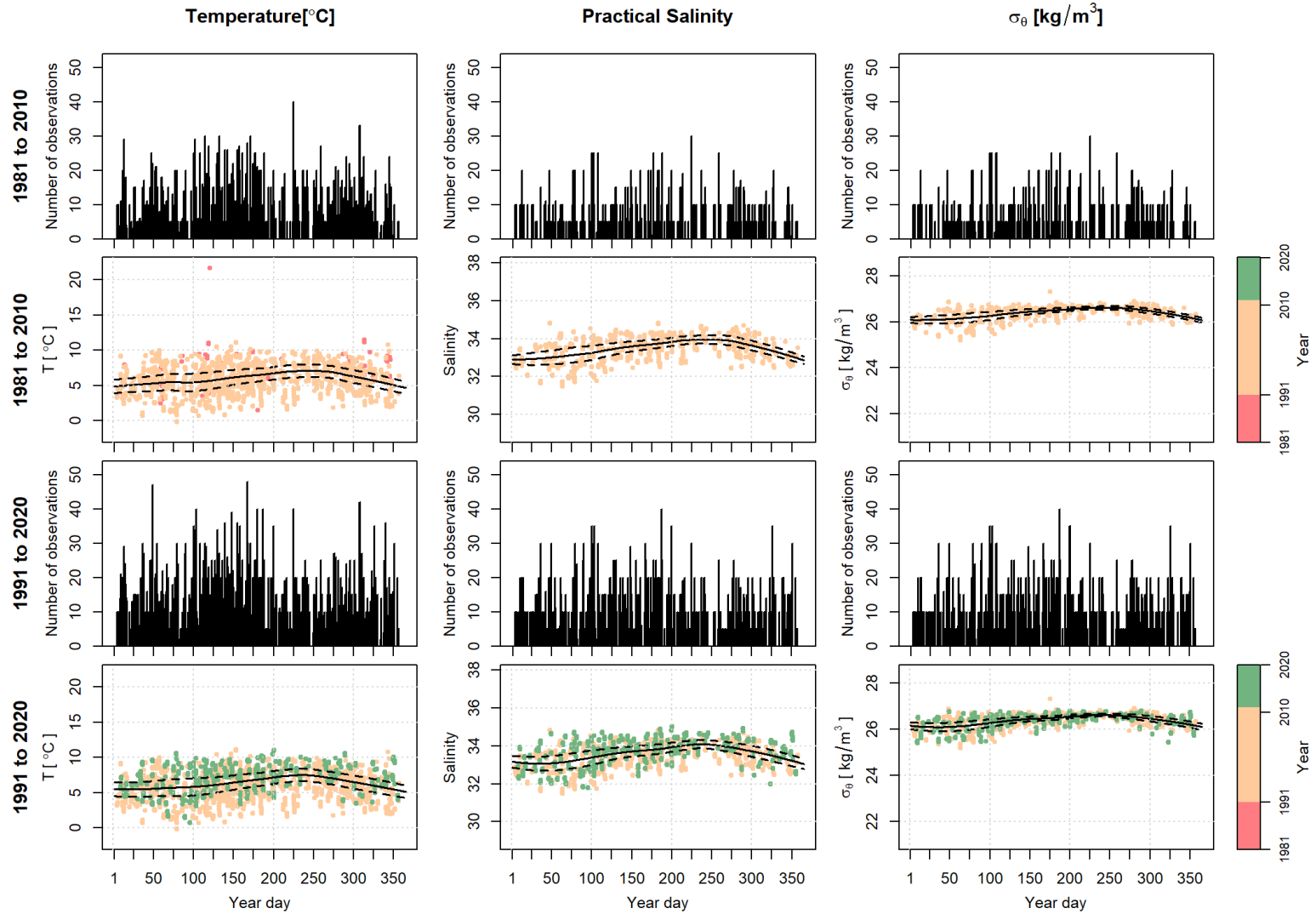
Figure 28. The 127.5m to 132.5m depth bin total number of observations per year day for the 1981 to 2010 (top row) and the 1991 to 2020 (third row) reference period and the scatter plot of data, color coded by year, with the mean (thick black line) and \pm 1 SD (dashed black line) local polynomial regression fits for the 1981 to 2010 (second row) and the 1991 to 2020 (bottom row) reference period for temperature (left column), salinity (middle column), and density (right column).
