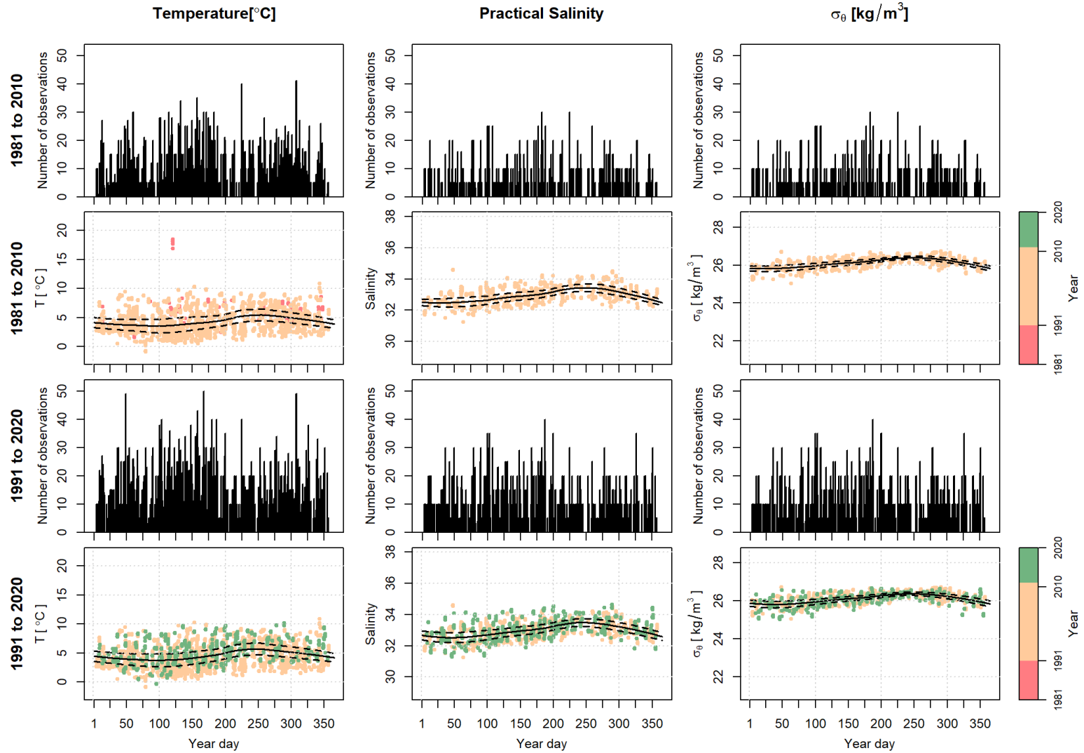
Figure 23. The 102.5m to 107.5m depth bin total number of observations per year day for the 1981 to 2010 (top row) and the 1991 to 2020 (third row) reference period and the scatter plot of data, color coded by year, with the mean (thick black line) and \pm 1 SD (dashed black line) local polynomial regression fits for the 1981 to 2010 (second row) and the 1991 to 2020 (bottom row) reference period for temperature (left column), salinity (middle column), and density (right column).
