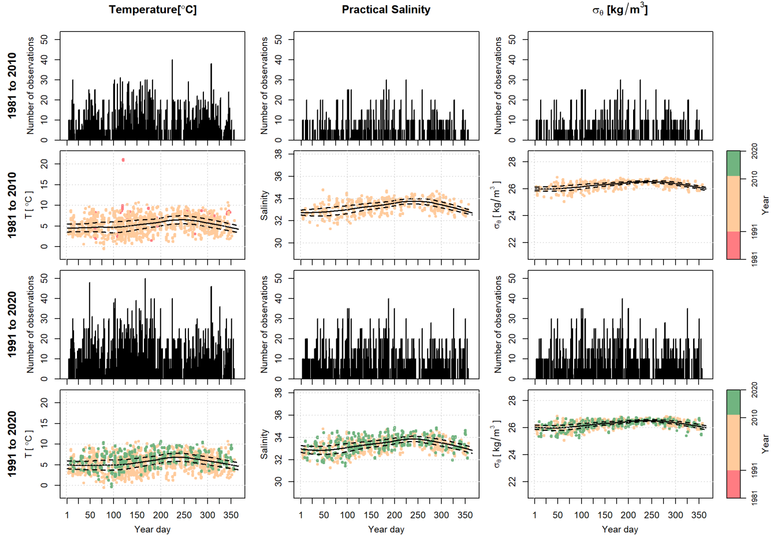
Figure 26. The 117.5m to 122.5m depth bin total number of observations per year day for the 1981 to 2010 (top row) and the 1991 to 2020 (third row) reference period and the scatter plot of data, color coded by year, with the mean (thick black line) and \pm 1 SD (dashed black line) local polynomial regression fits for the 1981 to 2010 (second row) and the 1991 to 2020 (bottom row) reference period for temperature (left column), salinity (middle column), and density (right column).
