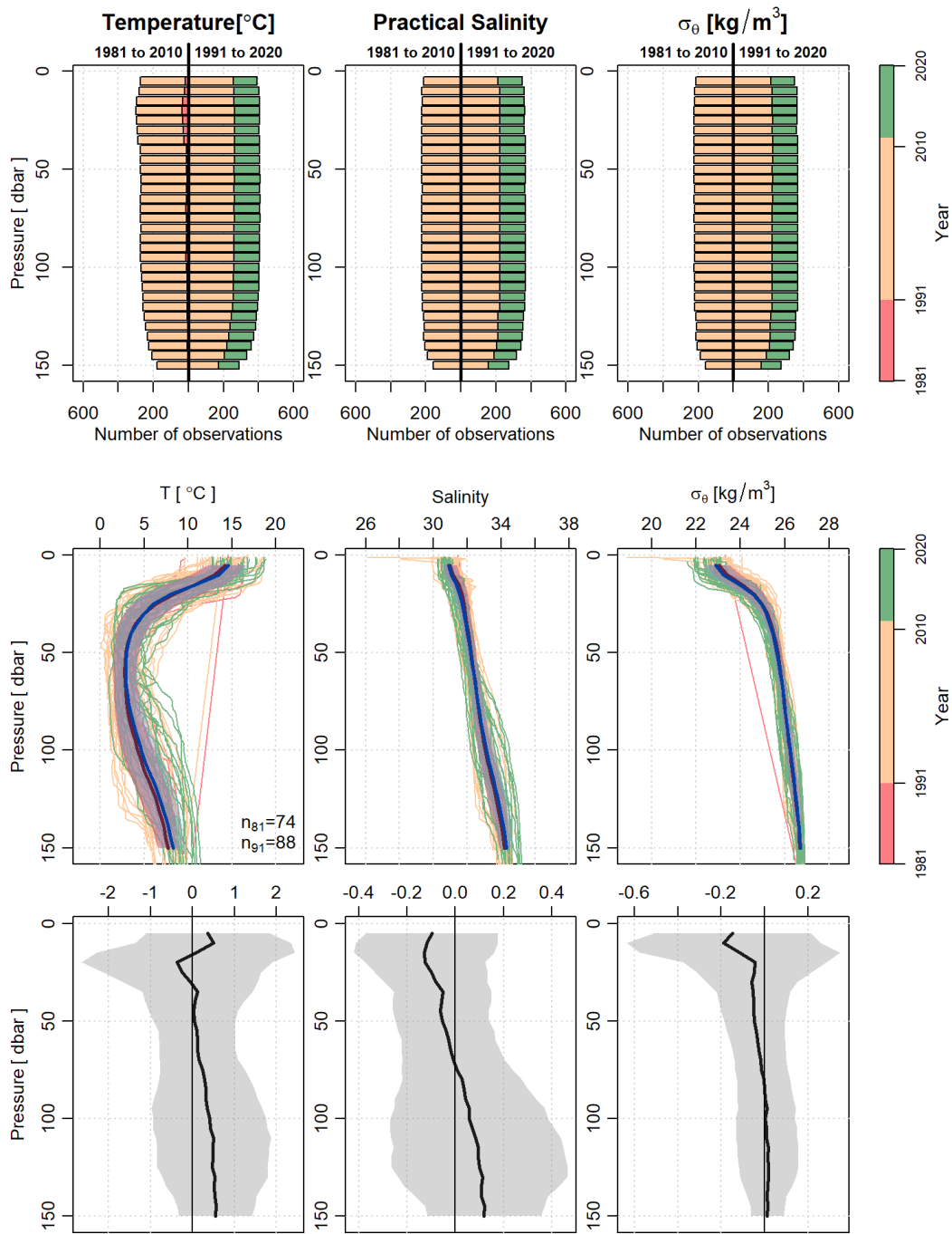
Figure 41. The July number of observations for each climatology reference period, as indicated by the label on the top axis, color coded by year (top row). Mean profiles (thick line) and the \pm 0.5\text{SD} (indicated by shading) for the 1981 to 2010 reference period (red) and 1991 to 2020 reference period (blue) (middle row). Thin lines, color coded by year, are the profile observations that were used in the mean and standard deviation calculations. The difference, 1991 to 2020 minus 1981 to 2010, of the two mean profiles and \pm 0.5\text{SD} for temperature (bottom left), salinity (bottom middle), and density (bottom right). Vertical thin black line denotes a difference of zero.
