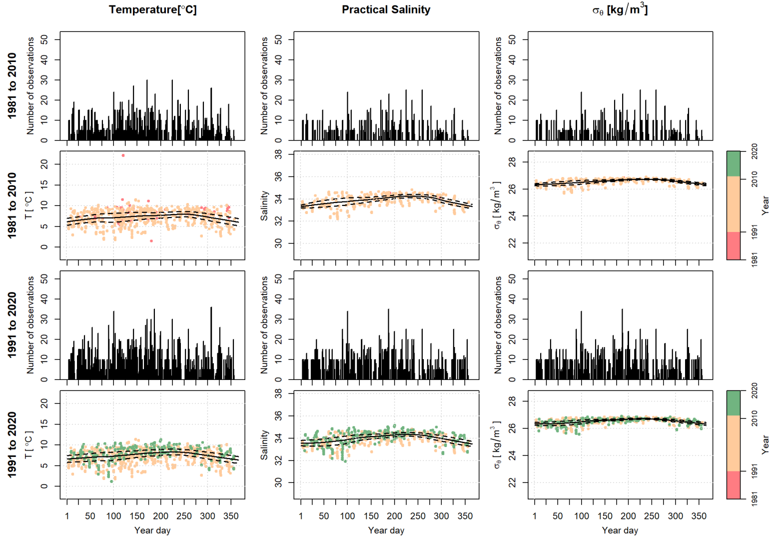
Figure 32. The 147.5m to 152.5m depth bin total number of observations per year day for the 1981 to 2010 (top row) and the 1991 to 2020 (third row) reference period and the scatter plot of data, color coded by year, with the mean (thick black line) and \pm 1 SD (dashed black line) local polynomial regression fits for the 1981 to 2010 (second row) and the 1991 to 2020 (bottom row) reference period for temperature (left column), salinity (middle column), and density (right column).
