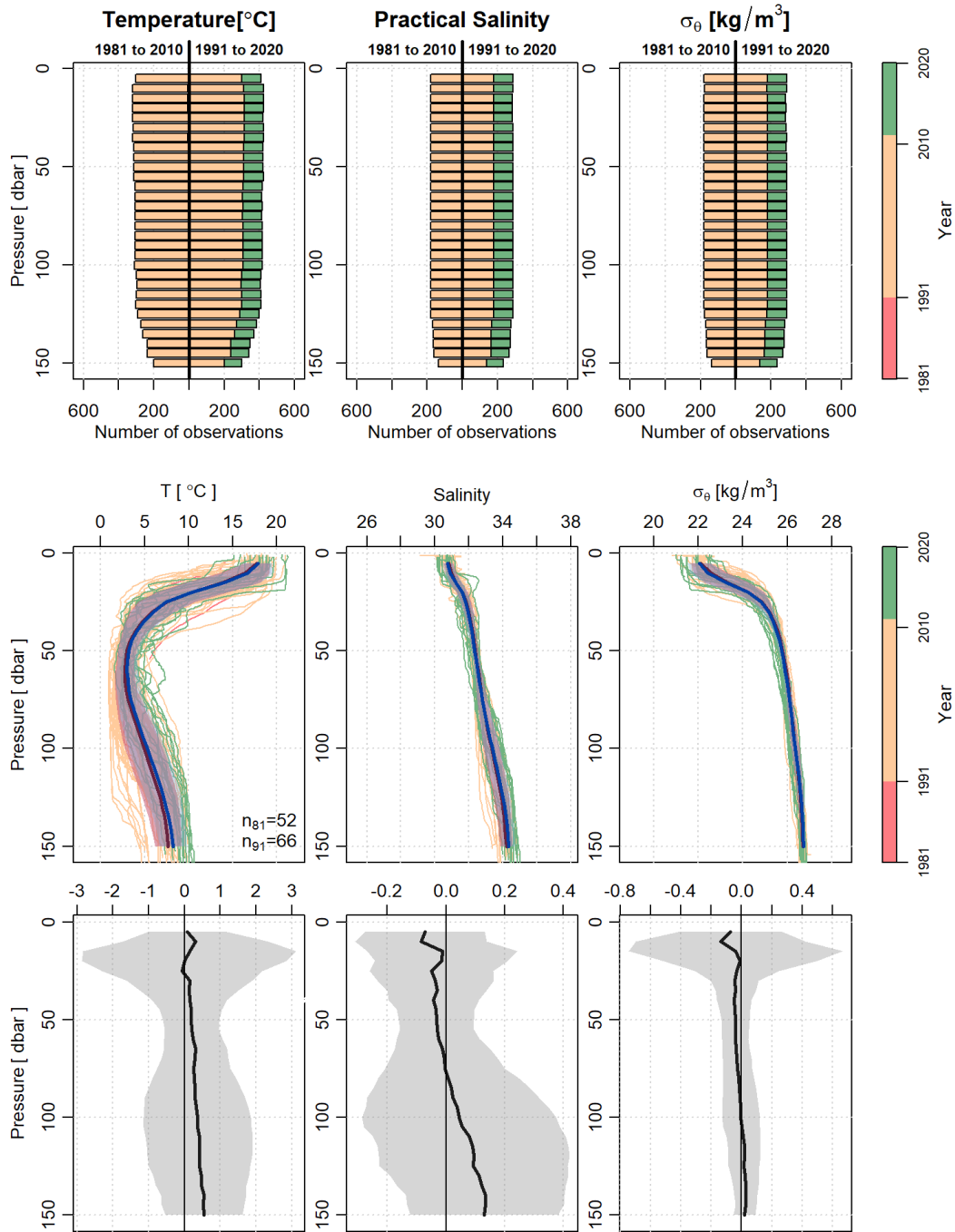
Figure 42. The August number of observations for each climatology reference period, as indicated by the label on the top axis, color coded by year (top row). Mean profiles (thick line) and the \pm 0.5\text{SD} (indicated by shading) for the 1981 to 2010 reference period (red) and 1991 to 2020 reference period (blue) (middle row). Thin lines, color coded by year, are the profile observations that were used in the mean and standard deviation calculations. The difference, 1991 to 2020 minus 1981 to 2010, of the two mean profiles and \pm 0.5\text{SD} for temperature (bottom left), salinity (bottom middle), and density (bottom right). Vertical thin black line denotes a difference of zero.
