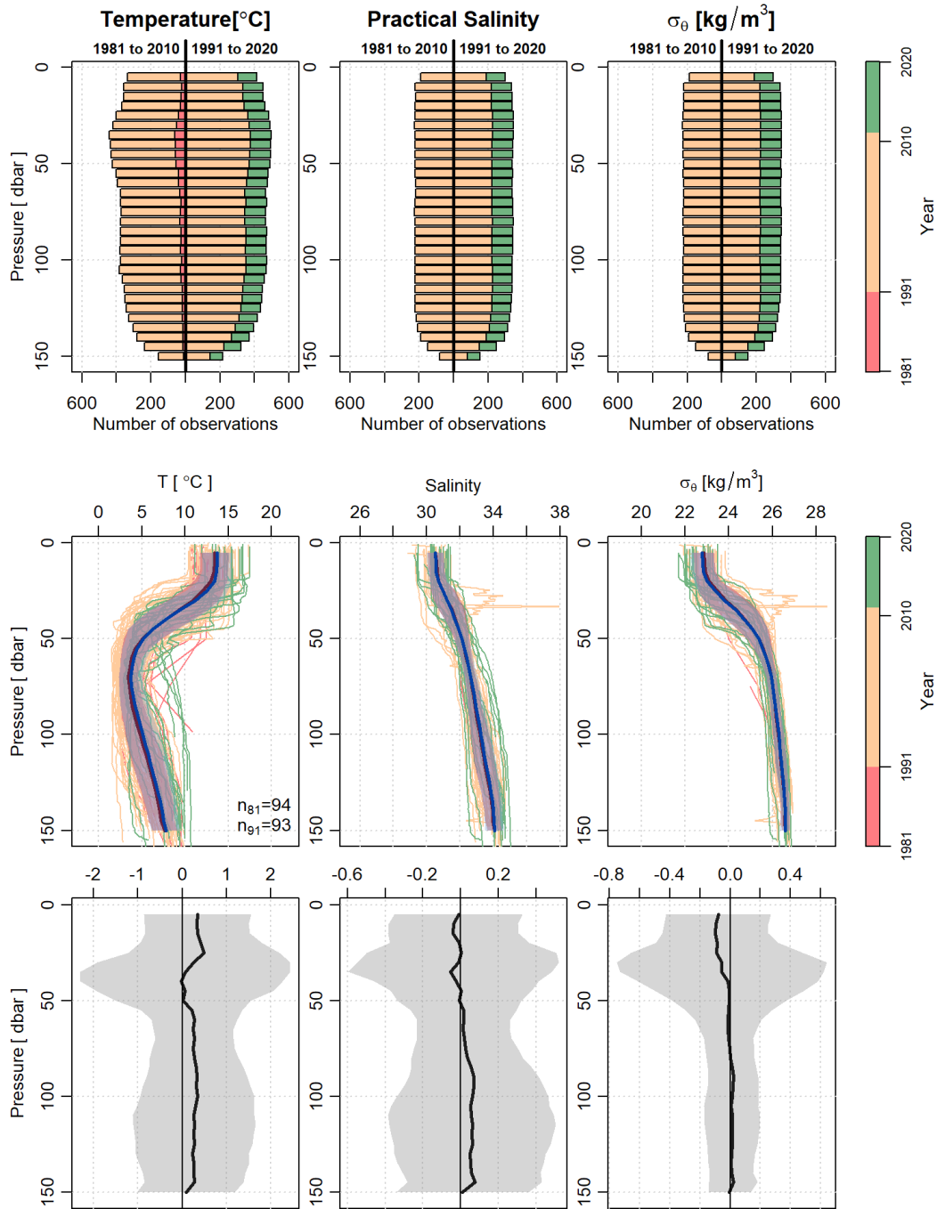
Figure 44. The October number of observations for each climatology reference period, as indicated by the label on the top axis, color coded by year (top row). Mean profiles (thick line) and the \pm 0.5\text{SD} (indicated by shading) for the 1981 to 2010 reference period (red) and 1991 to 2020 reference period (blue) (middle row). Thin lines, color coded by year, are the profile observations that were used in the mean and standard deviation calculations. The difference, 1991 to 2020 minus 1981 to 2010, of the two mean profiles and \pm 0.5\text{SD} for temperature (bottom left), salinity (bottom middle), and density (bottom right). Vertical thin black line denotes a difference of zero.
