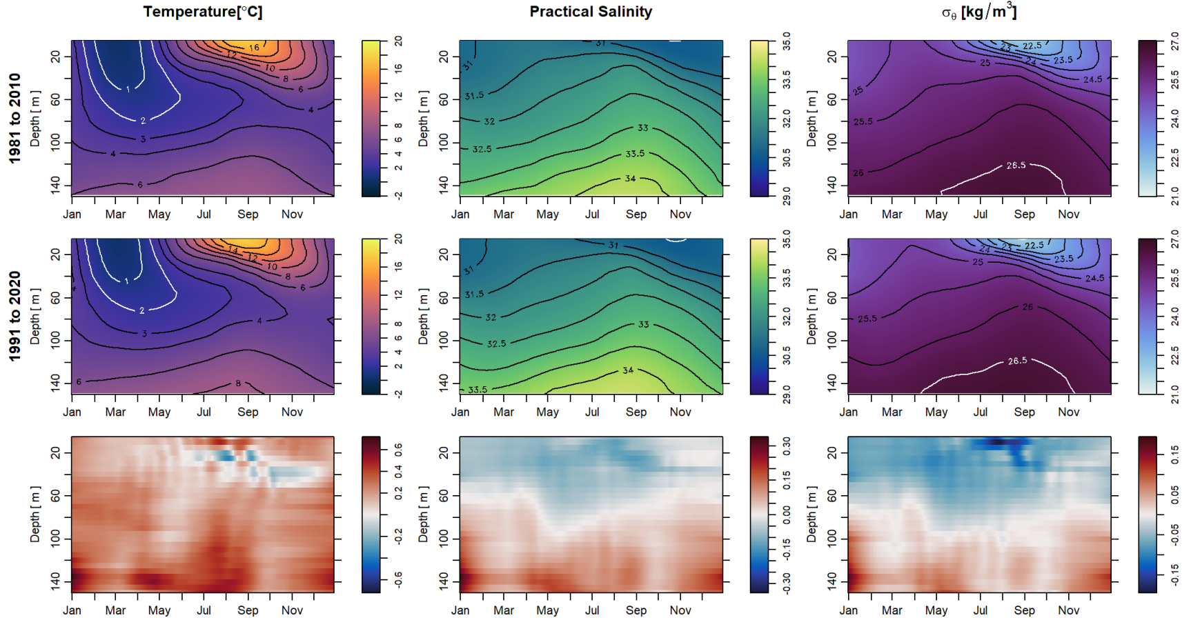
Figure 33. Section plot of the daily temperature (left column), salinity (middle column), and density (right column) climatology for the 1981 to 2010 reference period (top row) and 1991 to 2020 reference period (middle row). The quantized difference between the reference periods, the 1991 to 2020 minus the 1981 to 2010 reference period, of the daily climatology (bottom row).
