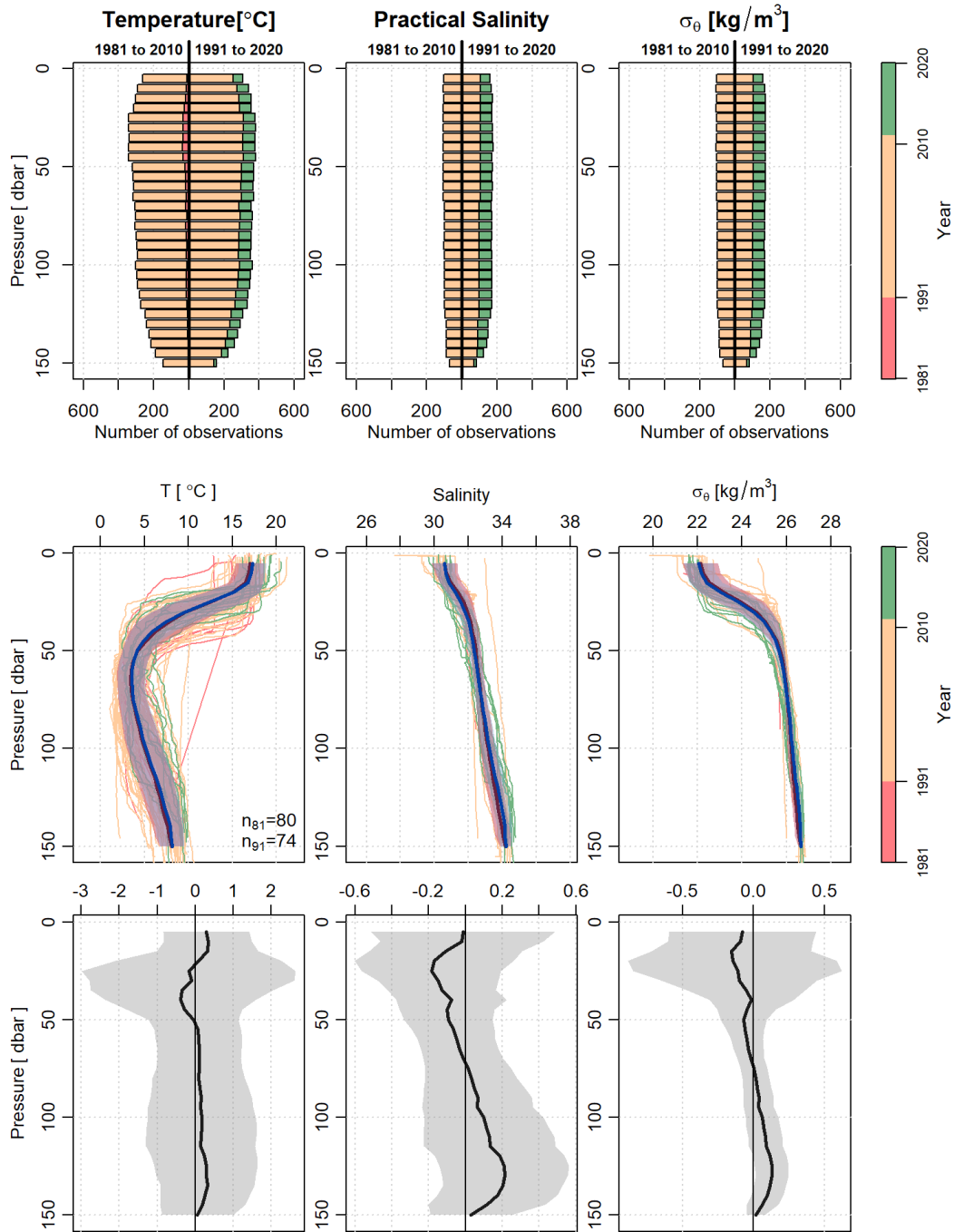
Figure 43. The September number of observations for each climatology reference period, as indicated by the label on the top axis, color coded by year (top row). Mean profiles (thick line) and the \pm 0.5\text{SD} (indicated by shading) for the 1981 to 2010 reference period (red) and 1991 to 2020 reference period (blue) (middle row). Thin lines, color coded by year, are the profile observations that were used in the mean and standard deviation calculations. The difference, 1991 to 2020 minus 1981 to 2010, of the two mean profiles and \pm 0.5\text{SD} for temperature (bottom left), salinity (bottom middle), and density (bottom right). Vertical thin black line denotes a difference of zero.
