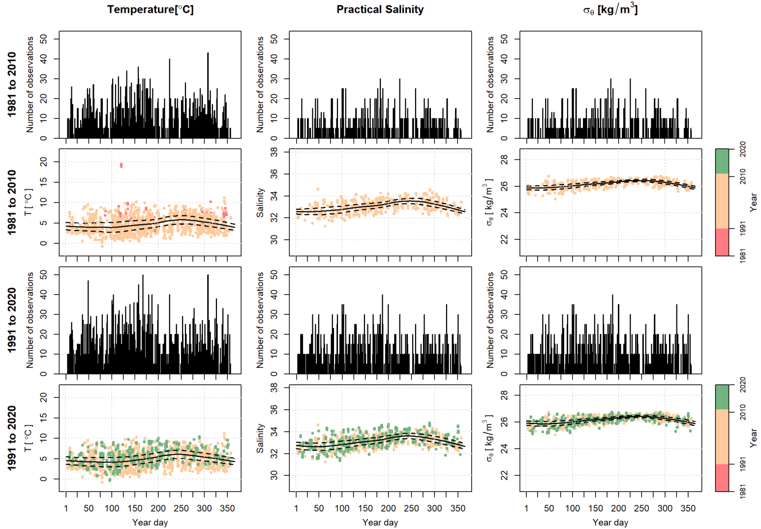
Figure 24. The 107.5m to 112.5m depth bin total number of observations per year day for the 1981 to 2010 (top row) and the 1991 to 2020 (third row) reference period and the scatter plot of data, color coded by year, with the mean (thick black line) and \pm 1 SD (dashed black line) local polynomial regression fits for the 1981 to 2010 (second row) and the 1991 to 2020 (bottom row) reference period for temperature (left column), salinity (middle column), and density (right column).
