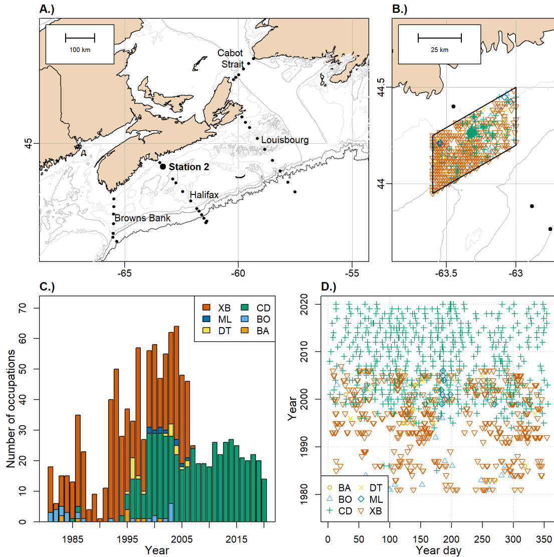
Figure 1. A.) A map of the Maritimes region Atlantic Zone Monitoring Program core transects, as labelled, with Station 2. B.) A close up map of Station 2 with the bounding box used to collate data, with the locations of the collated data which are distinguished by data type. C.) The annual total number of occupations, color coded by data type. D.) The sampling throughout the year, indicated by year day, color coded.
