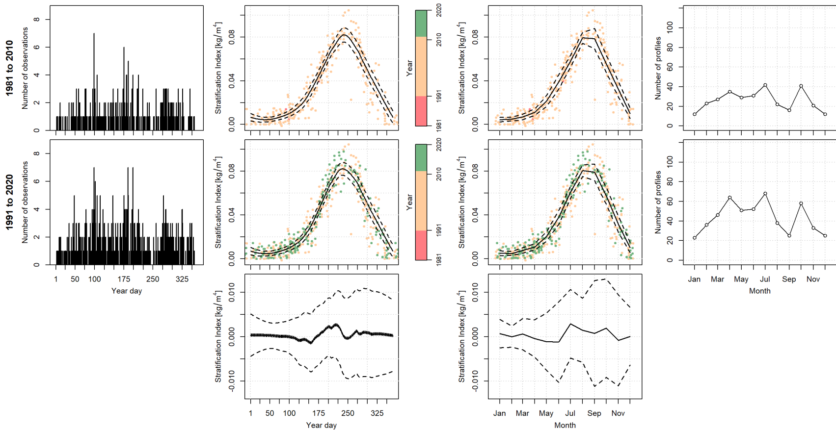
Figure 51. The stratification index calculated between depths 5 to 50m, from left to right, the total number of calculated values per year day, the daily mean local polynomial regression fits (thick black line) and \pm 0.5SD (dashed black lines) with a scatter plot of the calculated values colour coded by year, the monthly mean (thick black line) and \pm 0.5SD (dashed black lines) with a scatter plot of the calculated values colour coded by year, and the total number of observations per month for the 1981 to 2010 (top row) and 1991 to 2020 (middle row) climatology reference periods. The difference (1991 to 2020 minus the 1981 to 2010) of the climatology reference periods mean (thick black line) and the propagated uncertainty (dashed black lines) for the daily and monthly fits (bottom row).
