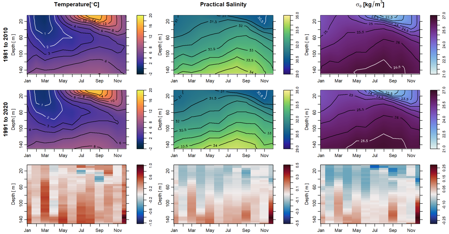
Figure 47. Section plot of the monthly temperature (left column), salinity (middle column), and density (right column) climatology for the 1981 to 2010 reference period (top row) and 1991 to 2020 reference period (middle row). The quantized difference between the reference periods, the 1991 to 2020 minus the 1981 to 2010 reference period, of the monthly climatology (bottom row).
