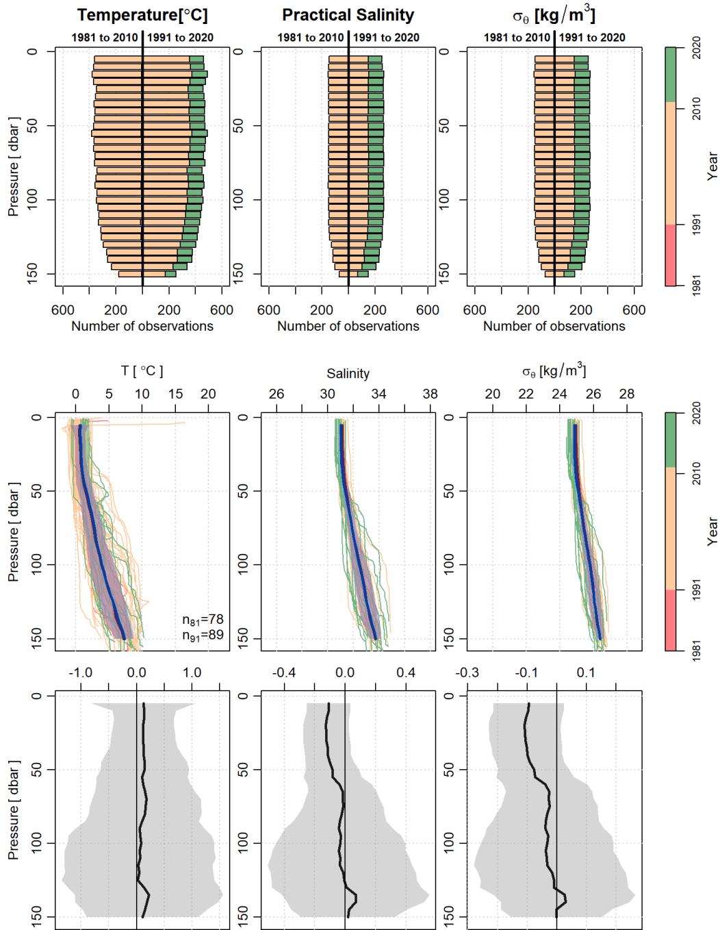
Figure 36. The February number of observations for each climatology reference period, as indicated by the label on the top axis, color coded by year (top row). Mean profiles (thick line) and the \pm 0.5 SD (indicated by shading) for the 1981 to 2010 reference period (red) and 1991 to 2020 reference period (blue) (middle row). Thin lines, color coded by year, are the profile observations that were used in the mean and standard deviation calculations. The difference, 1991 to 2020 minus 1981 to 2010, of the two mean profiles and \pm 0.5 SD for temperature (bottom left), salinity (bottom middle), and density (bottom right). Vertical thin black line denotes a difference of zero.
