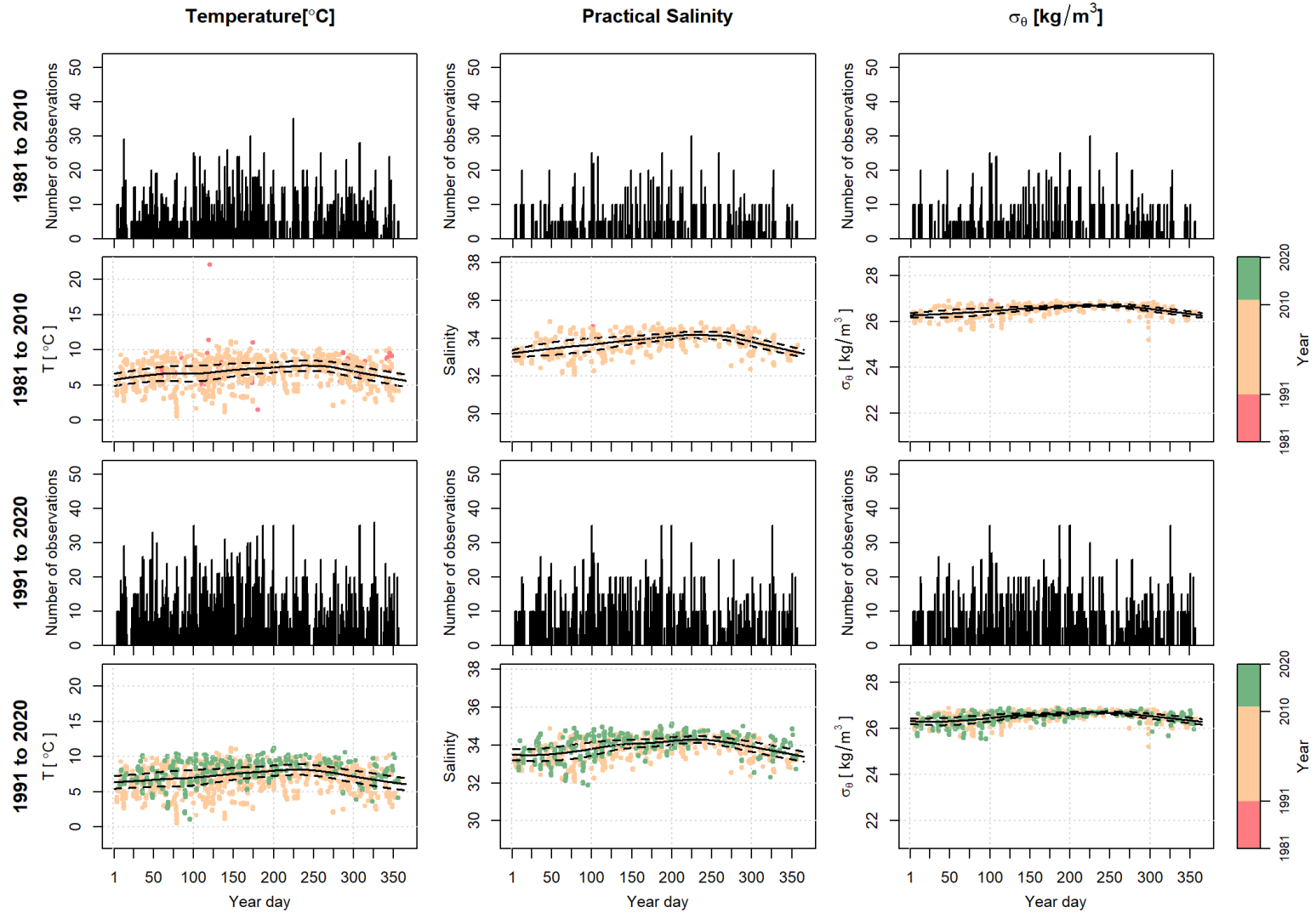
Figure 31. The 142.5m to 147.5m depth bin total number of observations per year day for the 1981 to 2010 (top row) and the 1991 to 2020 (third row) reference period and the scatter plot of data, color coded by year, with the mean (thick black line) and \pm 1 SD (dashed black line) local polynomial regression fits for the 1981 to 2010 (second row) and the 1991 to 2020 (bottom row) reference period for temperature (left column), salinity (middle column), and density (right column).
