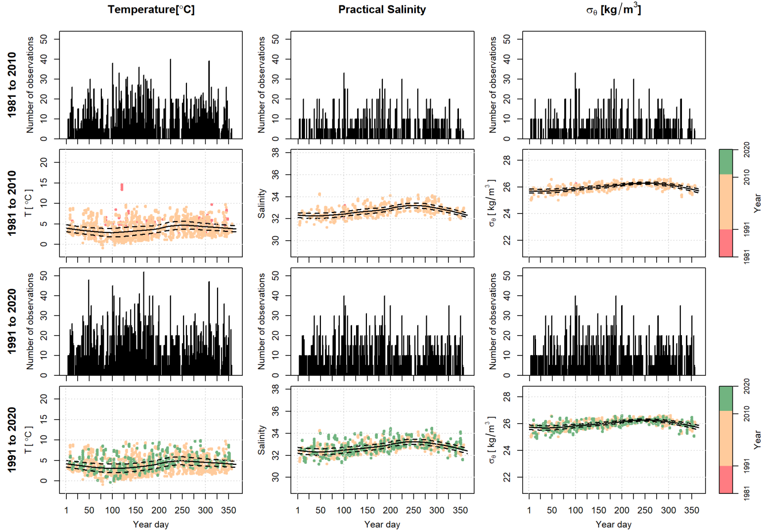
Figure 21. The 92.5m to 97.5m depth bin total number of observations per year day for the 1981 to 2010 (top row) and the 1991 to 2020 (third row) reference period and the scatter plot of data, color coded by year, with the mean (thick black line) and \pm 1 SD (dashed black line) local polynomial regression fits for the 1981 to 2010 (second row) and the 1991 to 2020 (bottom row) reference period for temperature (left column), salinity (middle column), and density (right column).
