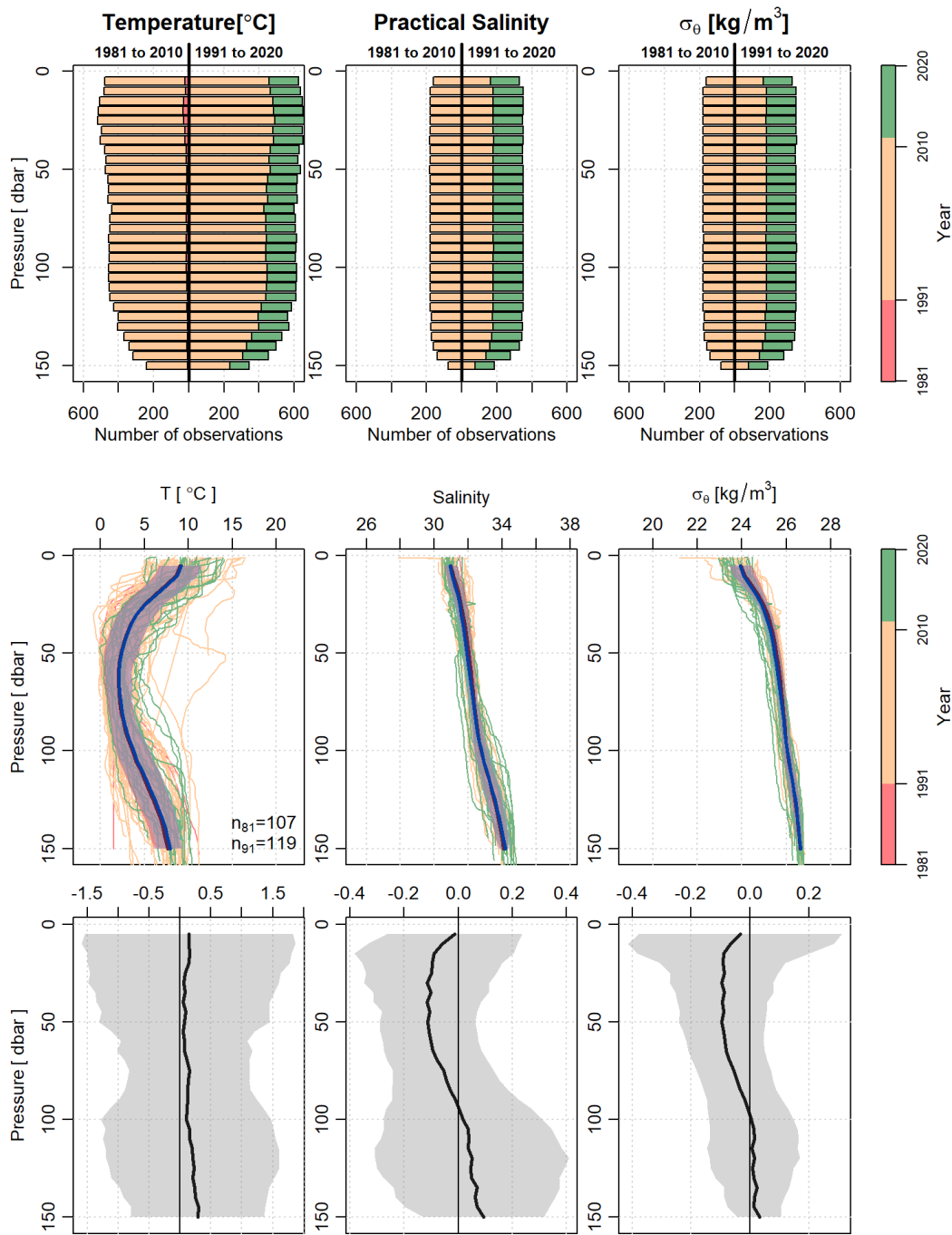
Figure 40. The June number of observations for each climatology reference period, as indicated by the label on the top axis, color coded by year (top row). Mean profiles (thick line) and the \pm 0.5SD (indicated by shading) for the 1981 to 2010 reference period (red) and 1991 to 2020 reference period (blue) (middle row). Thin lines, color coded by year, are the profile observations that were used in the mean and standard deviation calculations. The difference, 1991 to 2020 minus 1981 to 2010, of the two mean profiles and \pm 0.5SD for temperature (bottom left), salinity (bottom middle), and density (bottom right). Vertical thin black line denotes a difference of zero.
