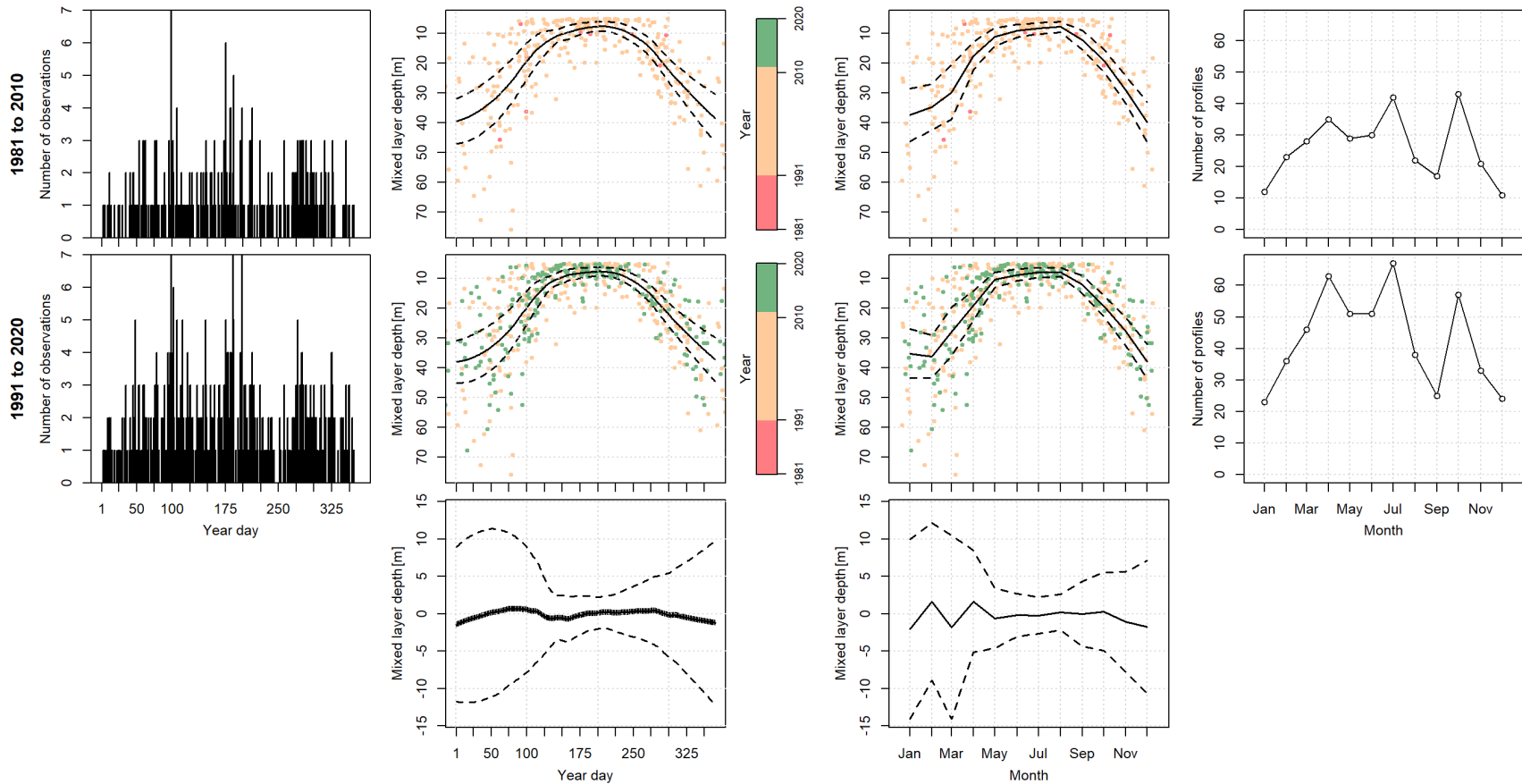
Figure 52. The mixed layer depth, from left to right, total number of calculated values per year day, daily mean local polynomial regression fits (thick black line) and \pm 0.5SD (dashed black lines) with a scatter plot of the calculated values colour coded by year, monthly mean (thick black line) and \pm 0.5SD (dashed black lines) with a scatter plot of the calculated values colour coded by year, and total number of observations per month for the 1981 to 2010 (top row) and 1991 to 2020 (middle row) climatology reference periods. The difference (1991 to 2020 minus the 1981 to 2010) of the climatology reference periods mean (thick black line) and the propagated uncertainty (dashed black lines) for the daily and monthly fits (bottom row).
