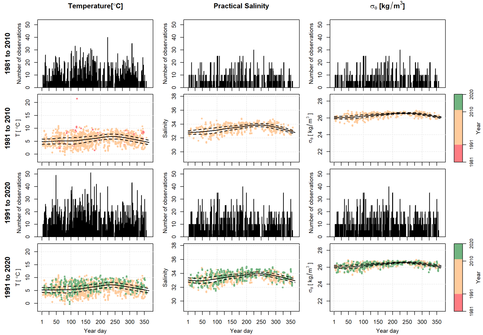
Figure 27. The 122.5m to 127.5m depth bin total number of observations per year day for the 1981 to 2010 (top row) and the 1991 to 2020 (third row) reference period and the scatter plot of data, color coded by year, with the mean (thick black line) and \pm 1 SD (dashed black line) local polynomial regression fits for the 1981 to 2010 (second row) and the 1991 to 2020 (bottom row) reference period for temperature (left column), salinity (middle column), and density (right column).
