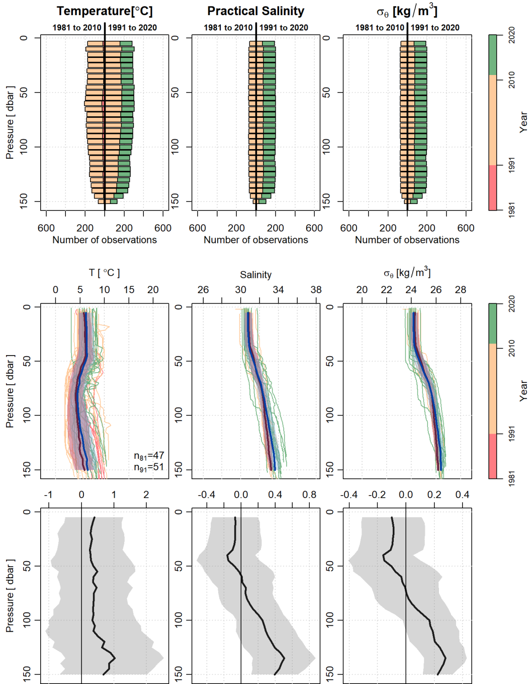
Figure 46. The December number of observations for each climatology reference period, as indicated by the label on the top axis, color coded by year (top row). Mean profiles (thick line) and the \pm 0.5SD (indicated by shading) for the 1981 to 2010 reference period (red) and 1991 to 2020 reference period (blue) (middle row). Thin lines, color coded by year, are the profile observations that were used in the mean and standard deviation calculations. The difference, 1991 to 2020 minus 1981 to 2010, of the two mean profiles and \pm 0.5SD for temperature (bottom left), salinity (bottom middle), and density (bottom right). Vertical thin black line denotes a difference of zero.
