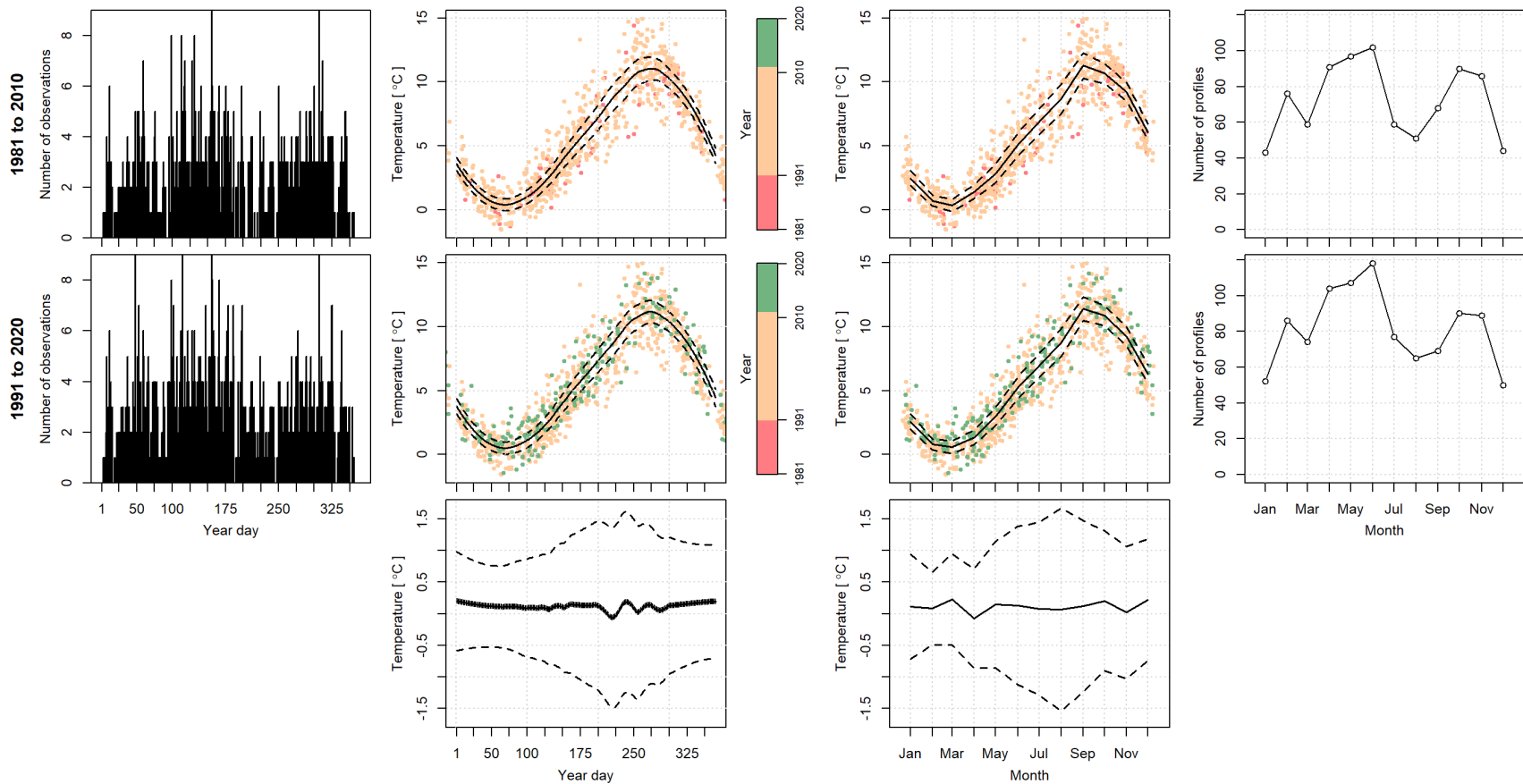
Figure 48. The integrated temperature over depths 5 to 50m, from left to right, the total number of calculated values per year day, the daily mean local polynomial regression fits (thick black line) and \pm 0.5\text{SD} (dashed black lines) with a scatter plot of the calculated values colour coded by year, the monthly mean (thick black line) and \pm 0.5\text{SD} (dashed black lines) with a scatter plot of the calculated values colour coded by year, and the total number of observations per month for the 1981 to 2010 (top row) and 1991 to 2020 (middle row) climatology reference periods. The difference (1991 to 2020 minus the 1981 to 2010) of the climatology reference periods mean (thick black line) and the propagated uncertainty (dashed black lines) for the daily and monthly fits (bottom row).
