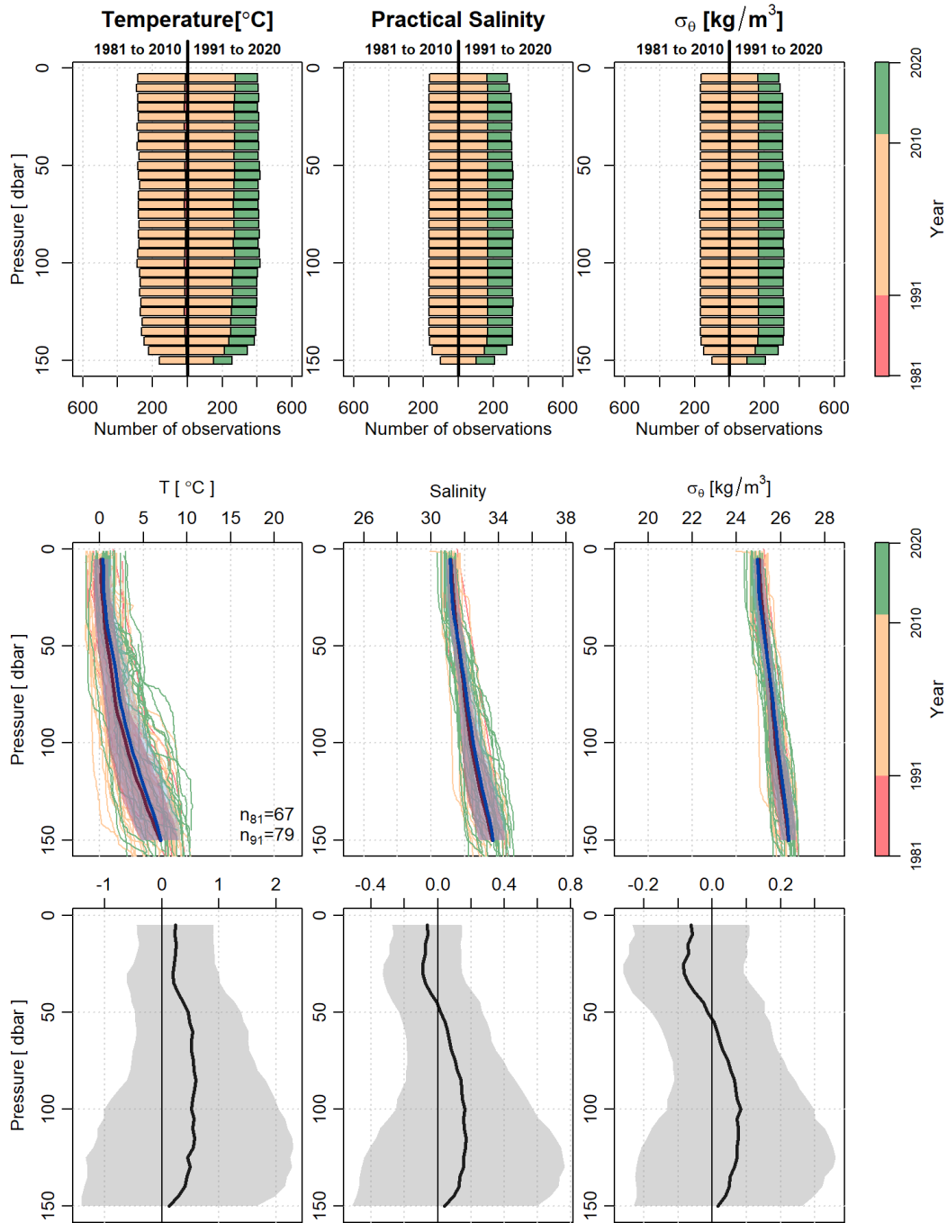
Figure 37. The March number of observations for each climatology reference period, as indicated by the label on the top axis, color coded by year (top row). Mean profiles (thick line) and the \pm 0.5SD (indicated by shading) for the 1981 to 2010 reference period (red) and 1991 to 2020 reference period (blue) (middle row). Thin lines, color coded by year, are the profile observations that were used in the mean and standard deviation calculations. The difference, 1991 to 2020 minus 1981 to 2010, of the two mean profiles and \pm 0.5SD for temperature (bottom left), salinity (bottom middle), and density (bottom right). Vertical thin black line denotes a difference of zero.
