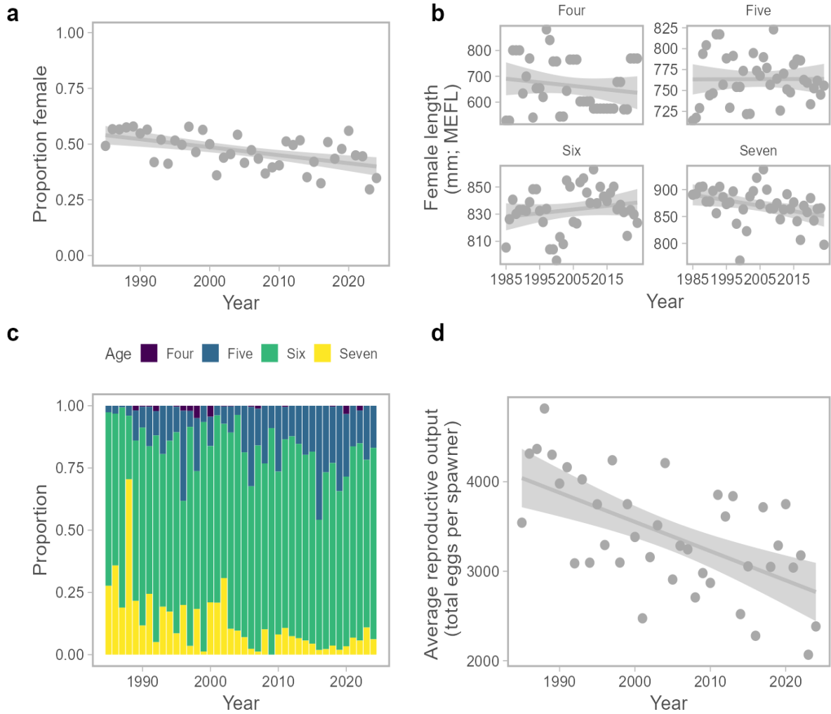
Figure 12. Age, sex, length, and reproductive output trends in Yukon River Chinook salmon over time. a) sex ratio, represented as proportion of spawners that are female, b) body length of female spawners by age (mid eye to tail fork length), c) proportion of returning spawners in each age class over time, d) average reproductive output of female spawners (eggs per female spawner). Data taken from fish sampled at Eagle and White and Sheep rocks.
