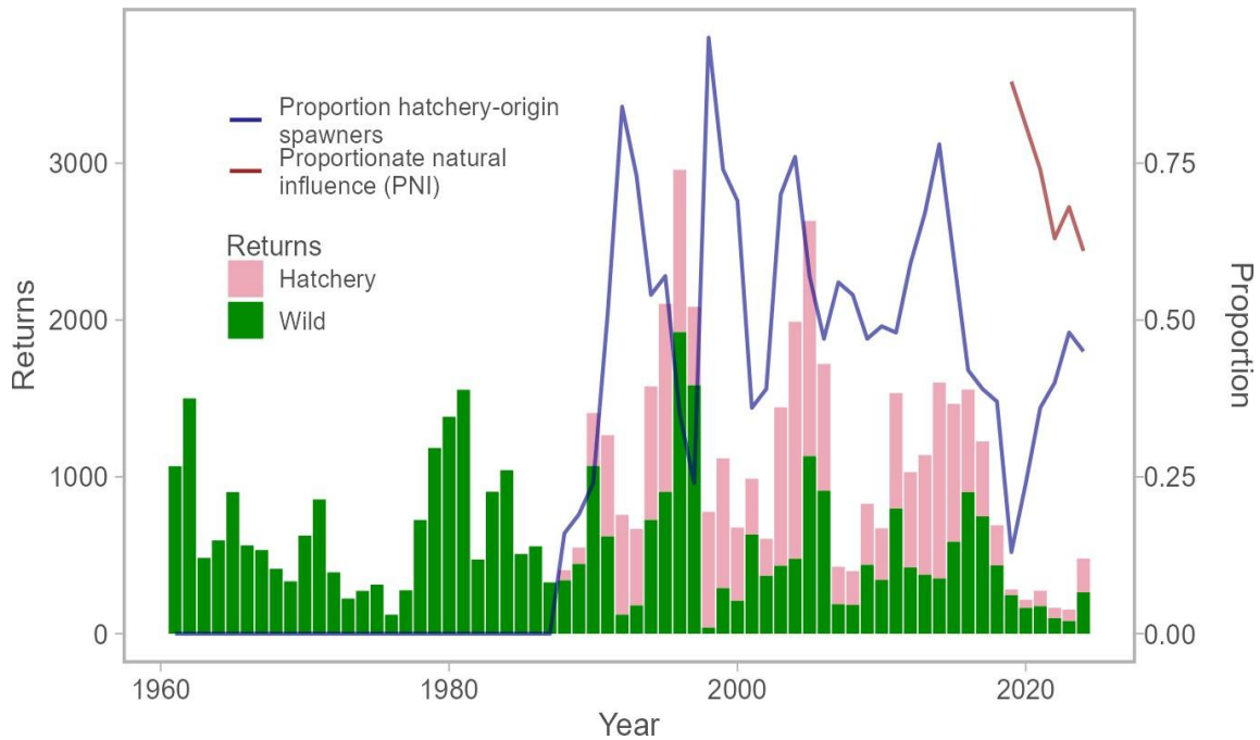
Figure 17. Chinook returns to Whitehorse Rapids fishway (Upper Yukon CU) and proportion hatchery origin spawners (pHOS), based on observed adipose fin clip rates. Proportionate Natural Influence (PNI) for the last six years, calculated from adipose fin clip status and Parentage Based Tagging (PBT) results of broodstock, when available.
