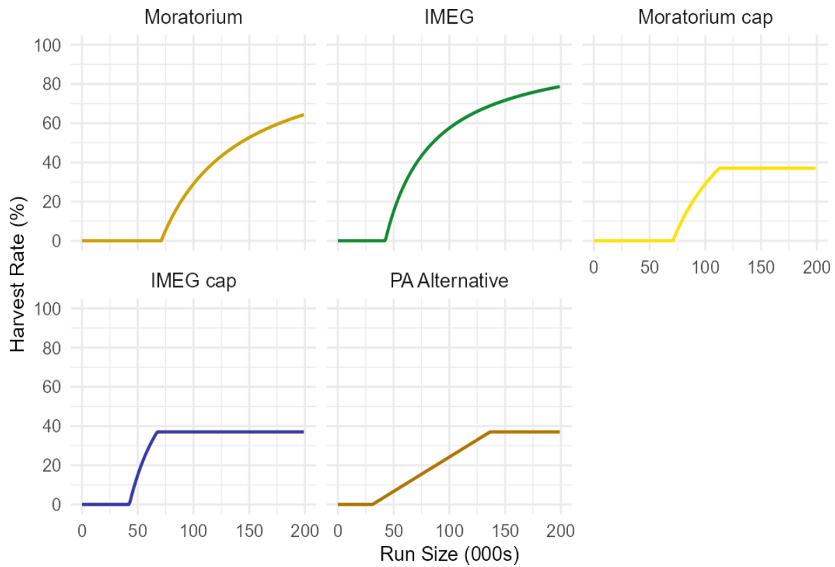
Figure 20. Illustration of the suite of harvest control rules considered in the closed-loop simulations. See Table 9 for description of each harvest control rule. The x-axis range in the plot corresponds approximately to the historical range of Yukon River Chinook salmon run sizes.
