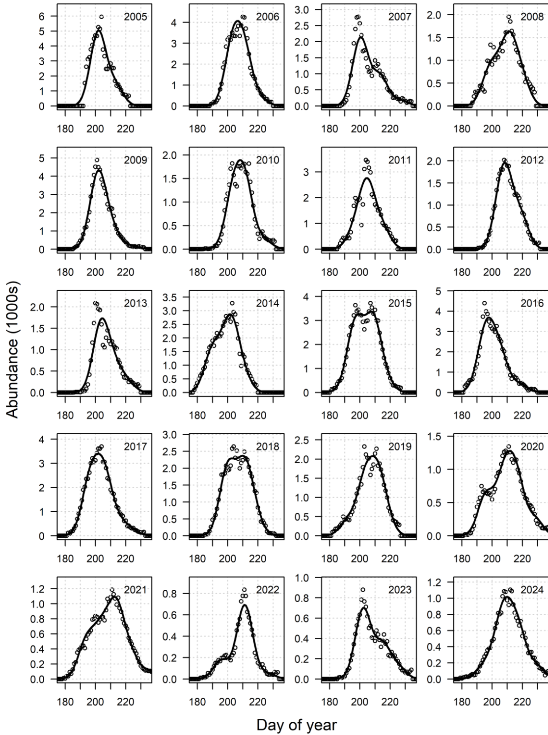
Figure B.2. Fits of the run-reconstruction model (lines) to daily sonar counts (circles) at Eagle, near the U.S.–Canada border.
