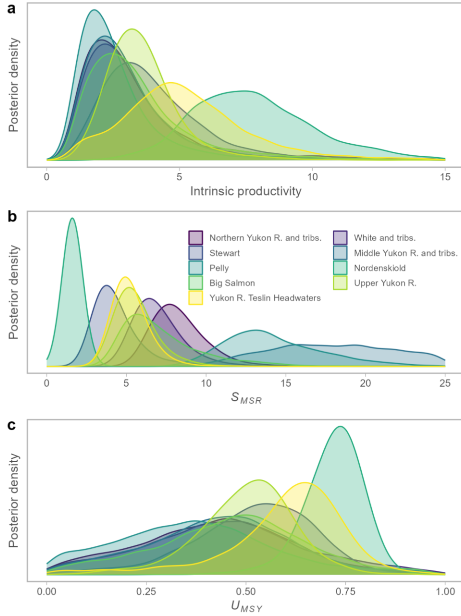
Figure 9. Conservation Unit specific posterior distributions of estimates of intrinsic productivity (a; \alpha in units of recruits-per-spawner), spawner abundance associated with maximum recruitment (b; S_{MSR} ), and exploitation rate associated with maximum sustainable yield (c; U_{MSY} ).
