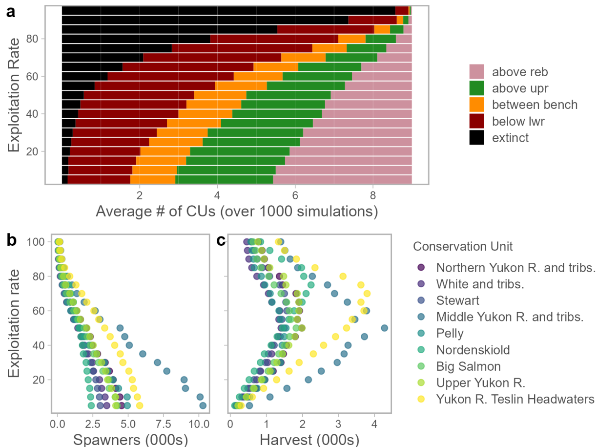
Figure 22. Projected consequences of a range of fixed exploitation rates from the closed loop simulations under the ‘reference’ (base case) operating model scenario. (a) Mean number of Conservation Units that fall above, below, and between their lower and upper biological benchmarks (20% S_{MSR} and 40% S_{MSR} based on analyses that assume stationary productivity) and illustrative rebuilding target ( S_{MSR} based on demographic characteristics from 2019–2024) in the final simulated year (2050), over 1,000 replicate simulations. (b) Mean spawner abundance and (c) mean harvest, by Conservation Units, over all simulation years (2025–2050).
