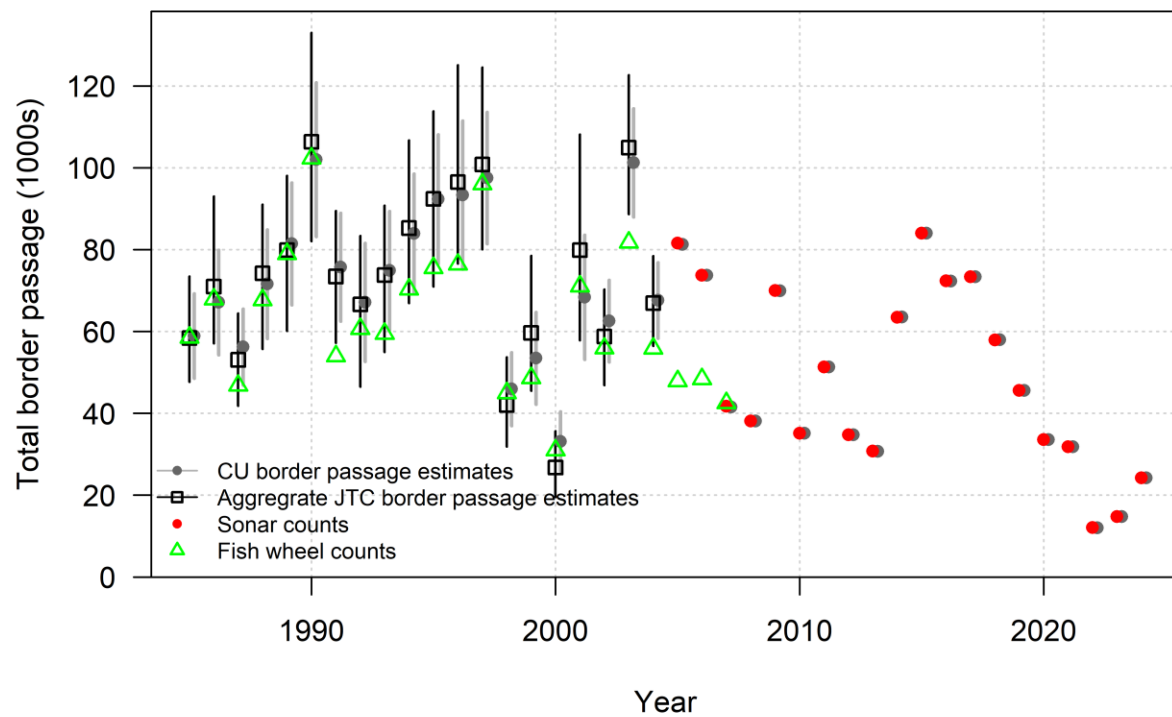
Figure B.4. Total border passage estimates based on the run-reconstruction model (grey circles with bars indicating the central 95% confidence interval), mark-recapture based estimates of run size from fish sampled from fish wheels after accounting for selectivity (open square), annual sum of daily fishwheel counts (scaled by estimated catchability, open green triangle) and the Eagle sonar (red circle).
