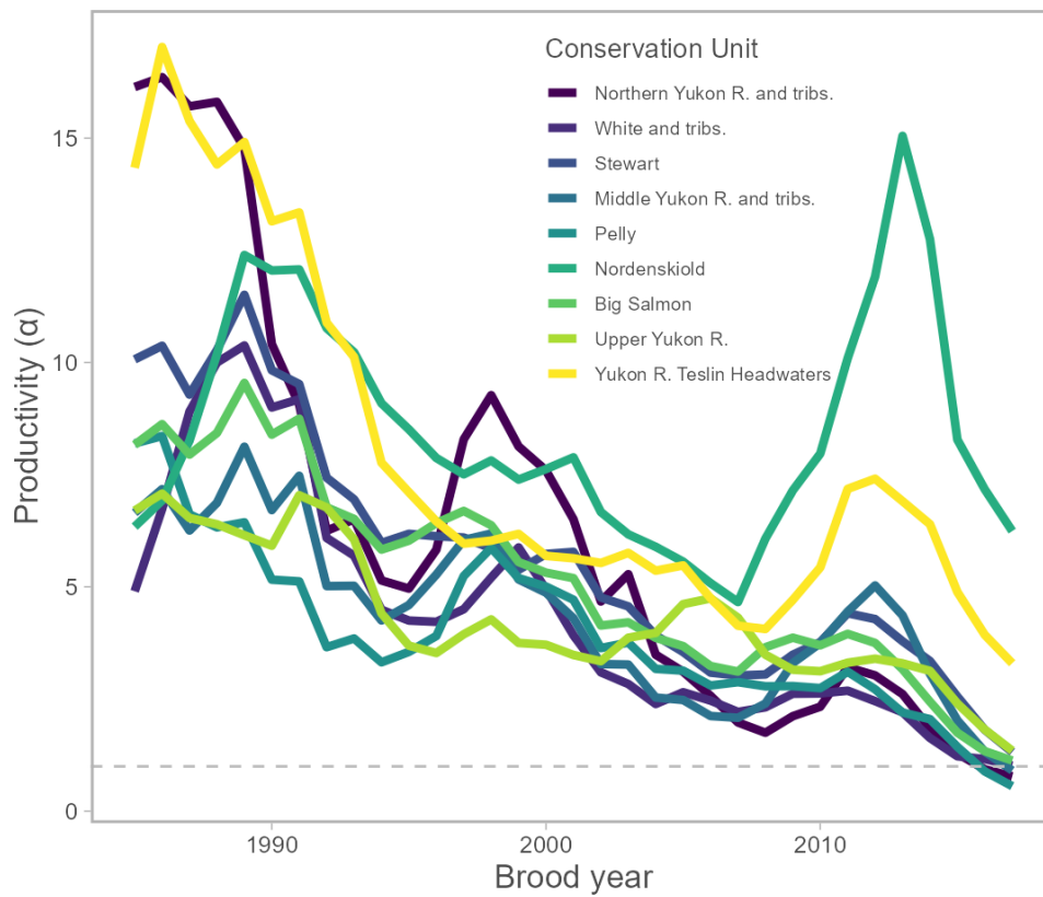
Figure 11. Estimated average intrinsic productivity (Ricker \alpha parameter; maximum recruits per spawner) over time by Conservation Unit in the Yukon Chinook Stock Management Unit. The dashed grey line is replacement (recruits equal spawners).
