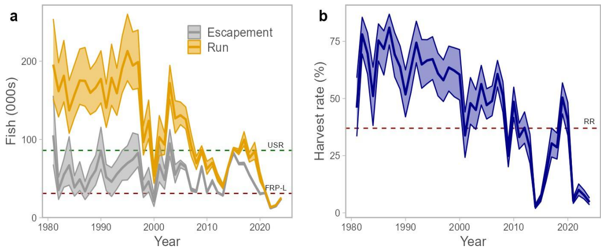
Figure 15. Reconstructed (a) total run size (orange) and spawning escapement (grey), with proposed Upper Stock Reference point (USR; green dashed line) and Lower Fisheries Reference Point (FRP-L; red dashed line), and (b) harvest rates for the Yukon Chinook Stock Management Unit (blue) and Removal Reference point (RR; red dashed line). Thick lines are medians and shaded areas indicate 95% credible intervals. Note that harvest rate in some years (e.g., 2017 and 2019) may be overestimated due to spawning migration mortality that was unaccounted for in the model that was used to estimate them (Connors et al. 2022a).
