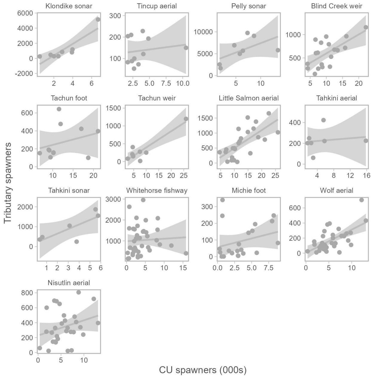
Figure 8. Relationship between estimates of spawner abundance from select tributary scale assessment projects and run-reconstruction based estimates at the Conservation Unit scale. Linear model fit shown in grey. For more details on each assessment project and corresponding Conservation Units see Table 2.
