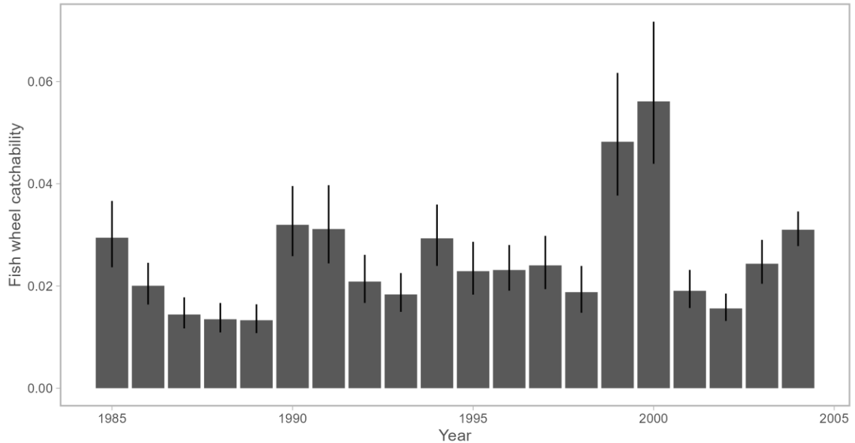
Figure B.1. Estimated fish wheel catchability, by year. Bars are median estimates +/- 95% confidence intervals.
