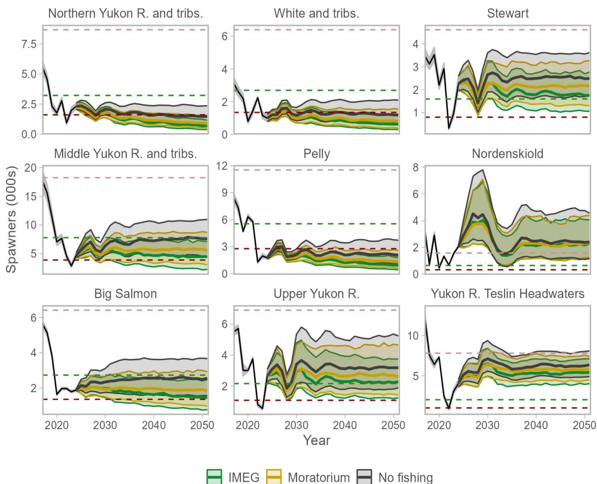
Figure 21. Projected spawner abundance over time (median and 50th percentiles) by Conservation Unit (CU) under three alternative fishery management measures, and the reference (base case) operating model productivity scenario. The last 6 years of observed spawners are shown prior to projections. Red and green dashed lines correspond to proposed lower and upper biological benchmarks for each CU ( 20\%S_{MSR} and 40\%S_{MSR} , respectively) from spawner-recruitment models with stationary productivity. Salmon colored dashed lines are CU rebuilding targets based on analyses that explicitly took demographic characteristics into account ( S_{MSR} based on demographic characteristics from 2019–2024).
