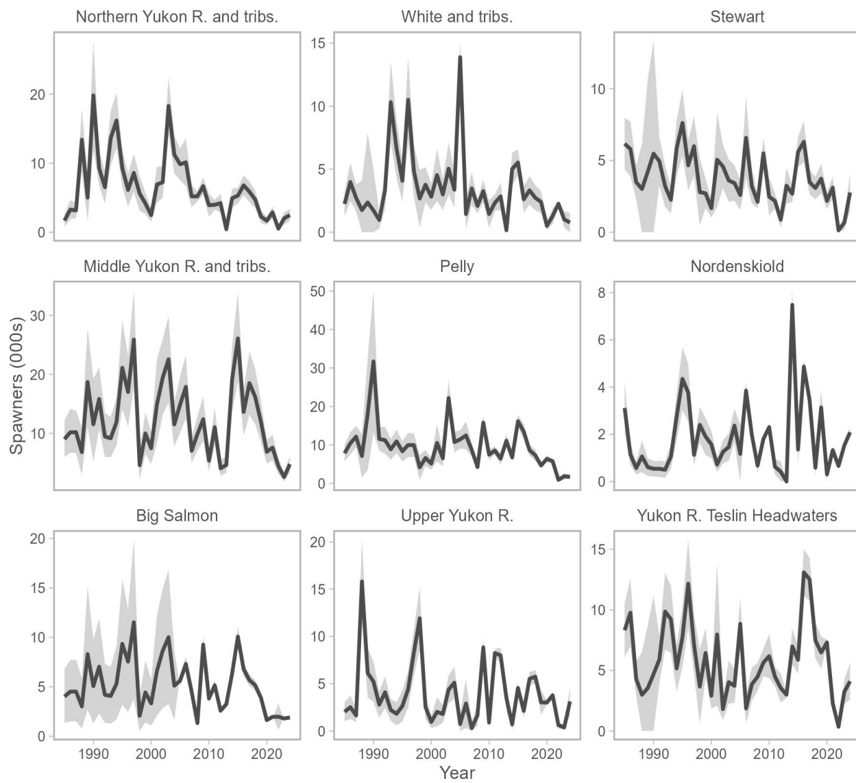
Figure 6. Reconstructed spawner abundance over time by Conservation Unit (median and 95% confidence intervals).
