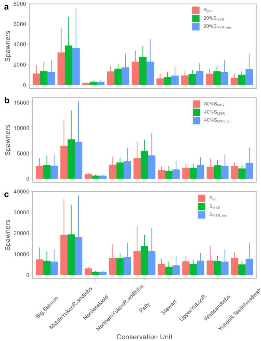
Figure C.1. Comparison of alternative (a) lower and (b) upper biological benchmarks as well as (c) estimates of maximum returns ( S_{MSR} ) or equilibrium population size ( S_{EQ} ) across CUs. The numeric value in legends refers to a percentage of the benchmark and those labelled “egg-mass” are derived from analyses that account for demographic change and are based on demographic characteristics observed over the most recent generation (2019–2024). Bars are medians and whiskers are upper 95th percentiles. Note that in instances where the intrinsic productivity of a CU is less than \sim 2.7 recruits-per-spawner equilibrium population size ( S_{EQ} ) occurs at lower spawner abundances than those associated with maximum recruits ( S_{MSR} ).
