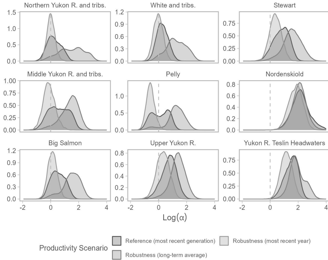
Figure 19. Alternative operating model productivity scenarios considered in the closed-loop simulations including the reference (base case) scenario, the average \alpha of the most recent fully observed generation (2013–2018 brood years), and robustness scenario, the most recent \alpha (2017 brood year).
