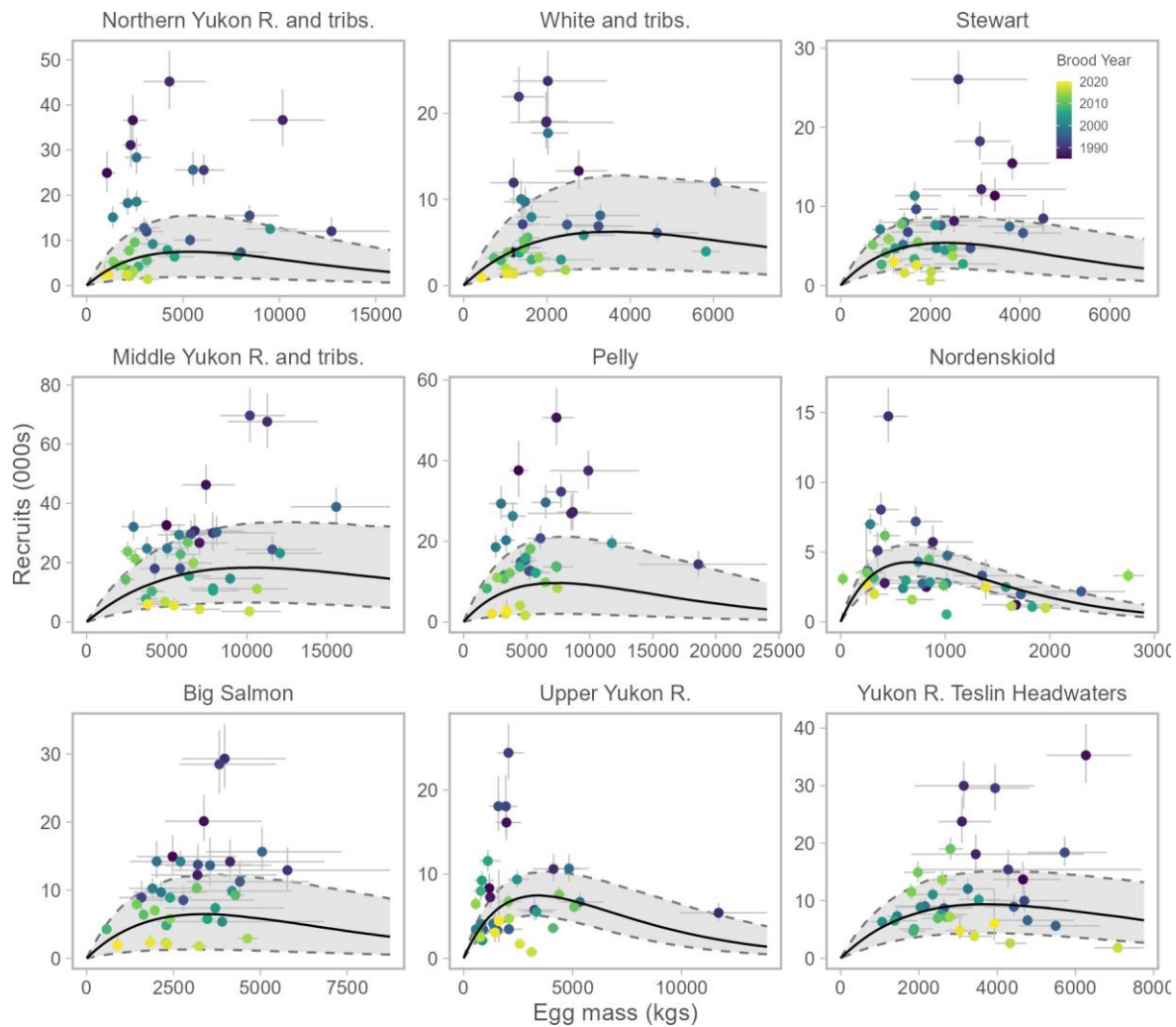
Figure 13. Relationship between total egg mass of spawning females and recruitment by Conservation Units. Individual egg mass-recruitment pairs are color coded according to brood year with 80% credible intervals. The thick black line is the predicted median relationship between egg mass and recruitment along with 80% credible intervals in the shaded region. To aid in visualizing uncertainty we use 80% credible intervals here instead of 95%.
