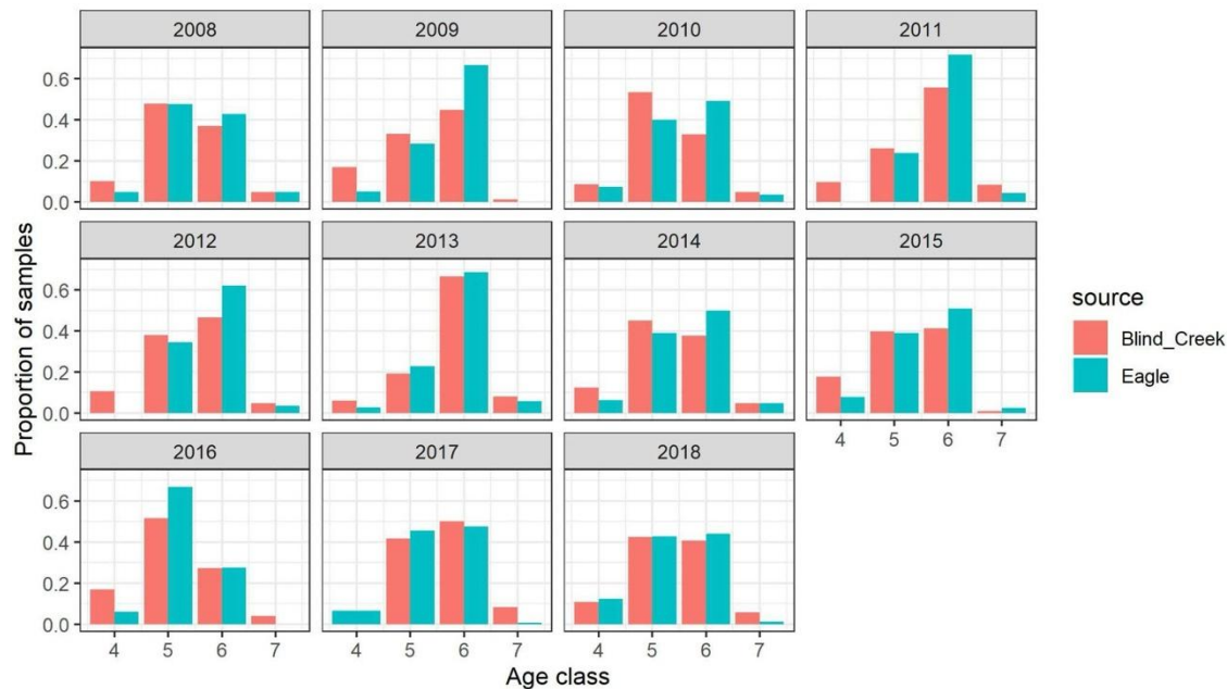
Figure D.2. Age composition of Chinook salmon sampled at the Blind Creek weir (in Pelly CU) and those sampled at the U.S.–Canada border.
