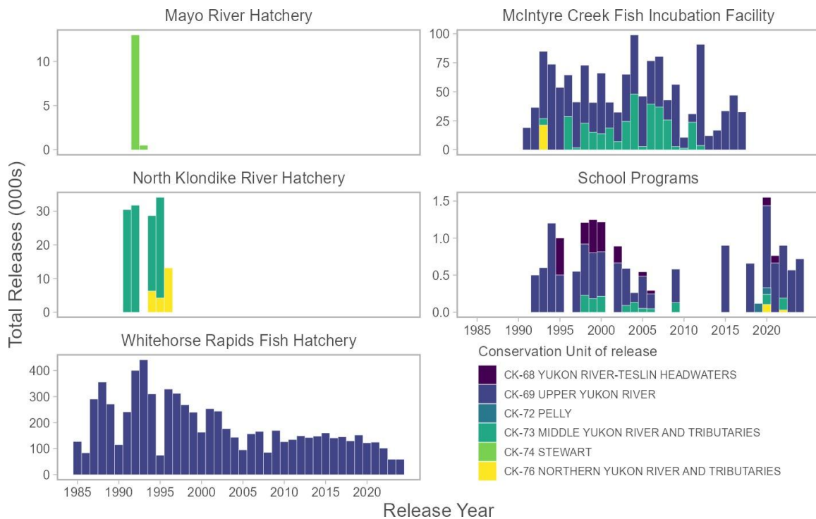
Figure 16. Total Yukon River Chinook salmon releases by facility/type and Conservation Unit. Note: Location of brood collection and release location, by CU, are the same in all cases except for ~250,000 fry from the Upper Yukon that were released in the Tatchun River (Middle Yukon CU) between 2006–2011.
