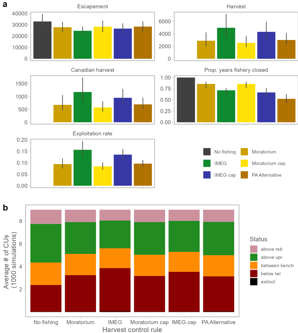
Figure 23. Performance of alternative harvest control rules the reference (base case) operating model productivity scenario. (a) Median (coloured bars) and 50% quantiles (vertical lines) of performance measures calculated over the years 2030–2050 and 1,000 replicate simulations. (b) Mean number of Conservation Units that fall above, below, and between their lower and upper biological benchmarks (20% S_{MSR} and 40% S_{MSR} based on analyses that assume stationary productivity) and illustrative rebuilding target ( S_{MSR} based on demographic characteristics from 2019–2024) in the final simulated year (2050), over 1,000 replicate simulations.
