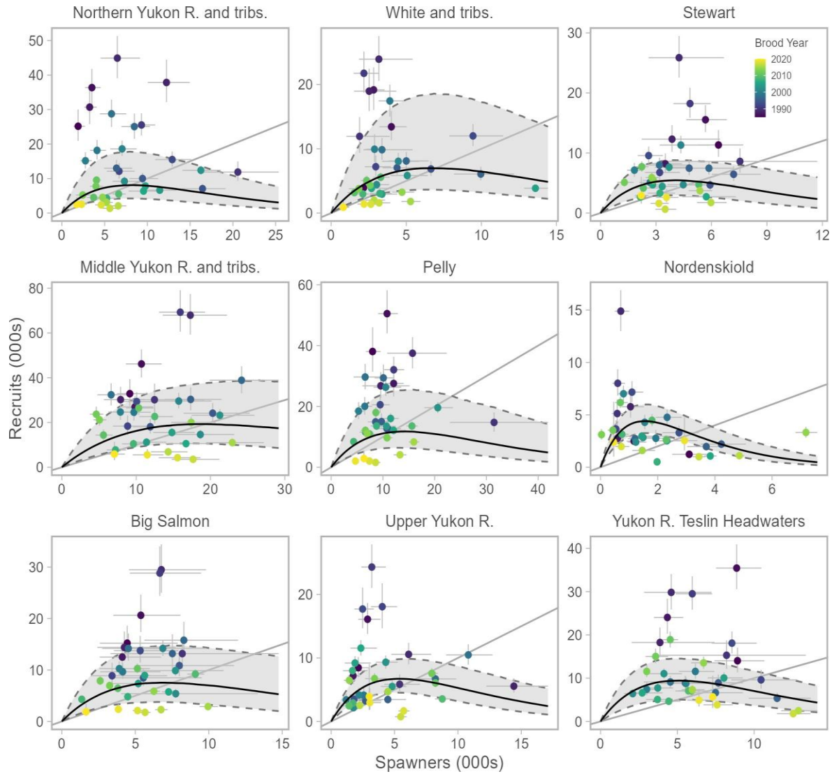
Figure 10. Relationship between spawner abundance and recruitment by Conservation Units. Individual spawner-recruitment pairs are color coded according to brood year with lines representing 80% credible intervals. The thick black line is the predicted median relationship between spawner abundance and recruitment along with 80% credible intervals in the shaded region. The replacement line, where spawners equal recruits, is shown in grey. To aid in visualizing uncertainty we use 80% credible intervals here instead of 95%.
