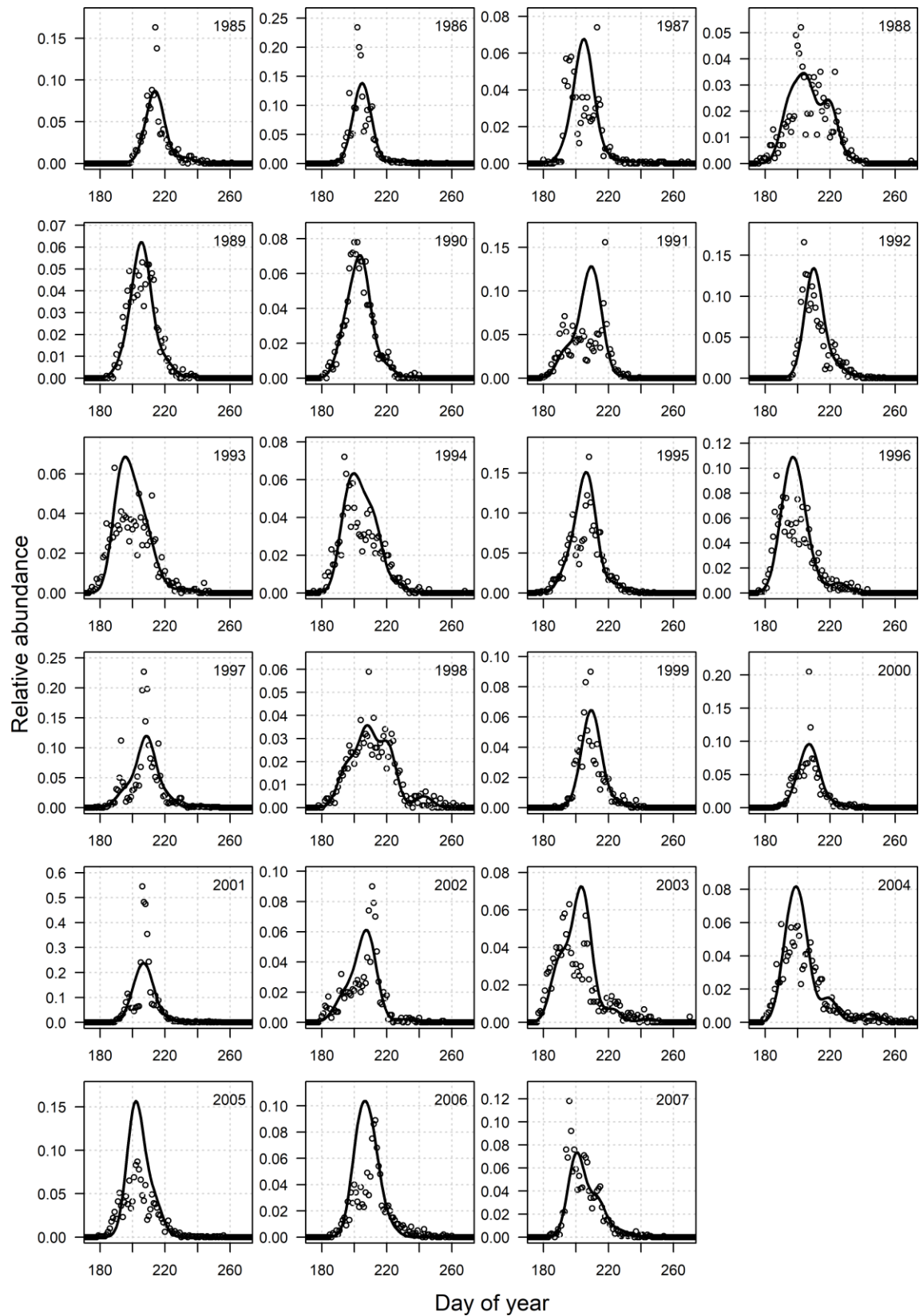
Figure B.3. Fits of the run-reconstruction model (lines) to daily fishwheel counts (circles) at White and Sheep Rocks, near the U.S.–Canada border.
