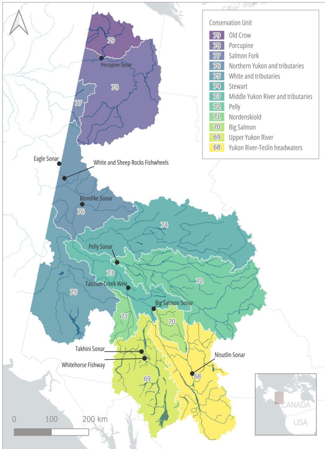
Figure 3. Major assessment projects for adult Chinook salmon in the Canadian portion of the Yukon River watershed. A full list of assessment projects is provided in Table 2.
