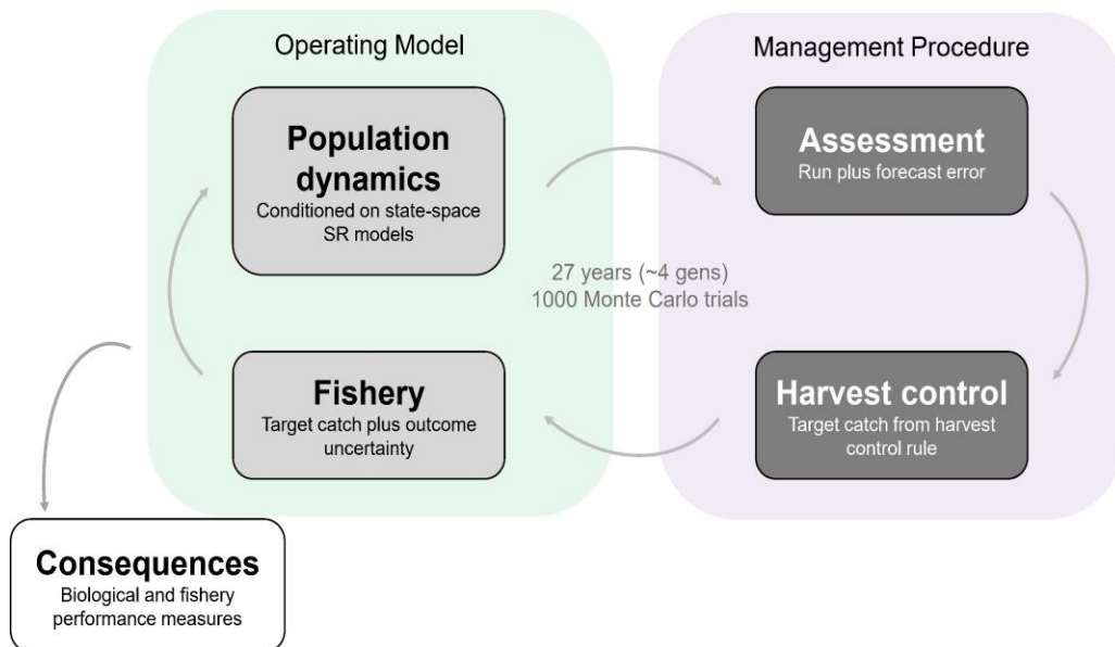
Figure 18. Illustration of steps in the closed loop simulations that were used to quantify future biological and fishery consequences of current and alternative harvest management measures. Run size forecast in forward simulation refers to run size at the U.S.–Canada border.
