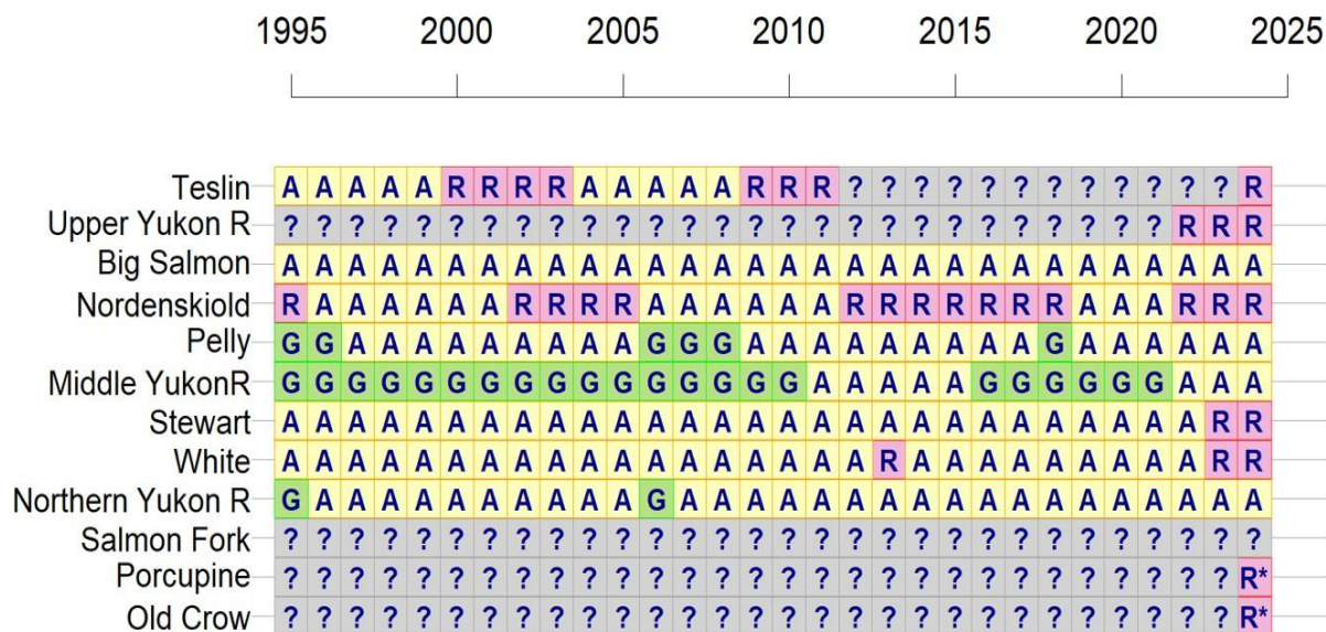
Figure 14. Yukon River Chinook salmon Wild Salmon Policy statuses for years with applicable data. Each row summarizes the statuses available for each Conservation Unit in the Yukon River and Porcupine Stock Management Units. The * for the Porcupine and Old Crow statuses indicates they are based on a combined assessment.
