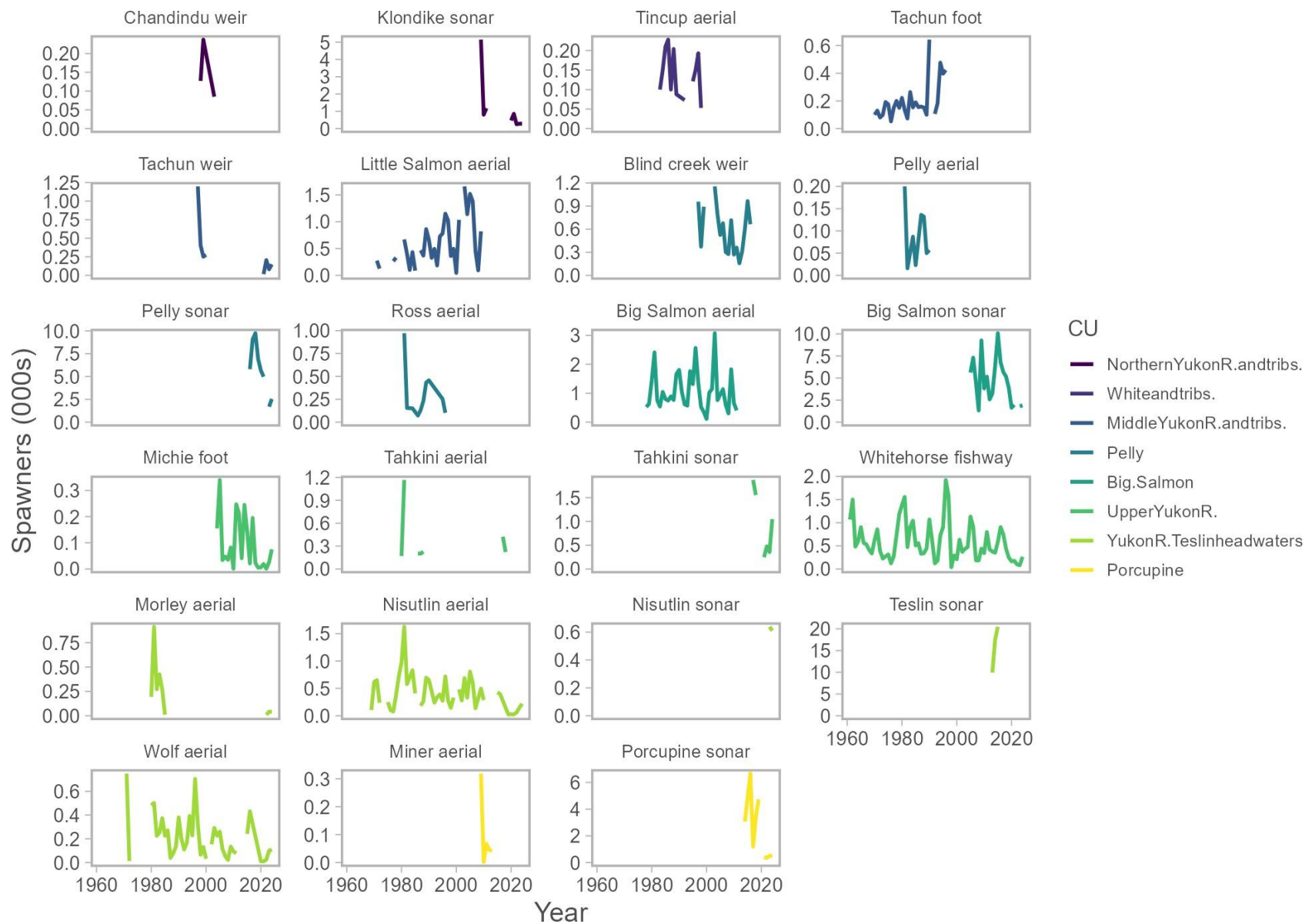
Figure 4. Estimates of spawner abundances over time by tributary assessment project. For more details on each assessment project see Table 2.
