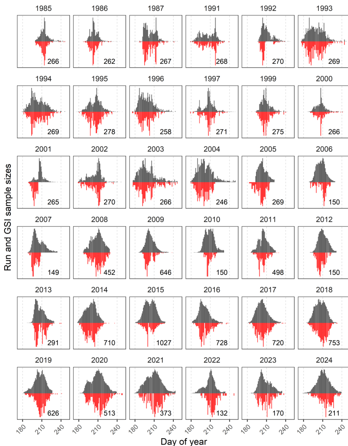
Figure A.1. Daily estimates of Chinook salmon border passage (grey bars) and scales or tissues sampled (red bars) from the run to determine genetic stock identification (GSI). Each bar is relative to the maximum for a given year with GSI samples inverted to allow for visualization of samples relative to border passage. The number of GSI samples in each year is in the bottom right of each panel. Note that scale samples were unavailable for 1988–1990, and 1998. For reference, in a non-leap year 29 June, 29 July and 28 August are equivalent to the 180th, 210th and 240th day of the year, respectively (dashed grey bars).
