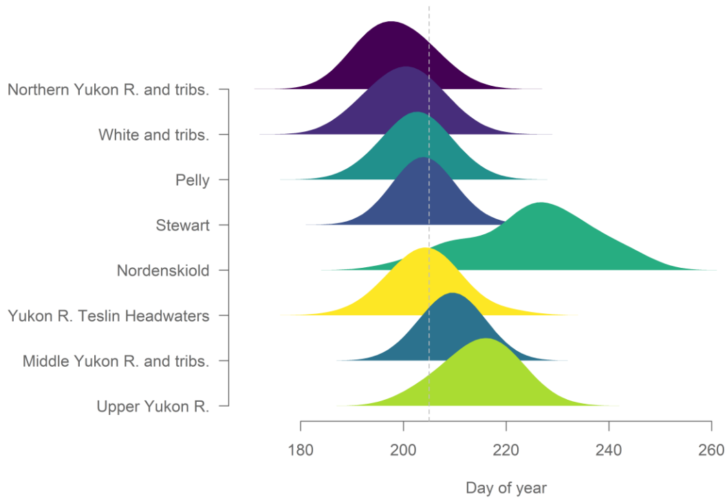
Figure 5. Average annual daily passage (scaled to maximum) from the U.S. into Canada on the mainstem Yukon River for eight Conservation Units. The Big Salmon Conservation Unit is not shown because it cannot be separated out from the Middle Mainstem Conservation Unit based on genetics. For reference, in a non-leap year the 180th, 210th and 240th day of the year correspond to 29 June, 29 July, and 28 August, respectively. The dashed line represents the approximate average peak run-timing for the stock aggregate.
