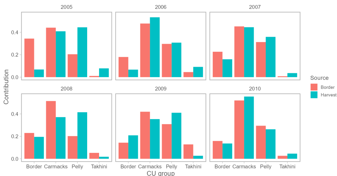
Figure D.3. Conservation Unit group composition of Chinook salmon sampled in commercial and subsistence fisheries in Alaska ("Harvest") and fish sampled in test fisheries at the U.S.–Canada border ("Border"). The "Border" CU grouping includes the Northern Yukon and White and tributaries CUs, the "Pelly" grouping includes the Pelly and Stewart CUs, the "Carmacks" grouping includes the Nordenskiöld, Middle Yukon, Big Salmon and Teslin CUs, and the "Takhini" grouping includes the Upper Yukon CU.
