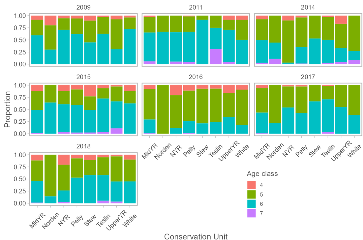
Figure D.1. Age composition in Chinook salmon sampled at the U.S.–Canada border, by Conservation Unit.
