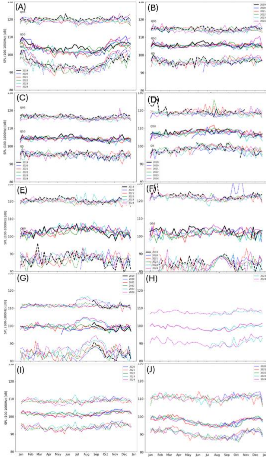
Figure 14: Weekly sound pressure levels (SPL) measured at Q 5 , Q 50 (median) and Q 95 for the 100-1000 Hz frequency range at (A) Swiftsure Bank, (B) Port Renfrew, (C) Jordan River, (D) Sooke, (E) Haro Strait, (F) Boundary Pass, (G) Swanson Channel, (H) Strait of Georgia South-east, (I) Strait of Georgia South, and (J) Strait of Georgia North.
