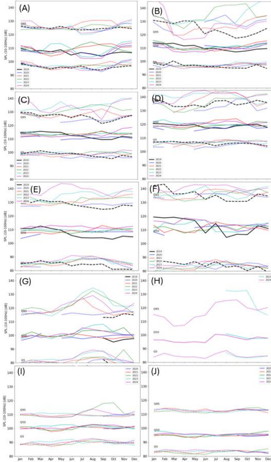
Figure 5: Monthly sound pressure levels (SPL) measured at Q 5 , Q 50 (median) and Q 95 for the 10-100 Hz frequency range at (A) Swiftsure Bank, (B) Port Renfrew, (C) Jordan River, (D) Sooke, (E) Haro Strait, (F) Boundary Pass, (G) Swanson Channel, (H) Strait of Georgia South-east, (I) Strait of Georgia South, and (J) Strait of Georgia North.
