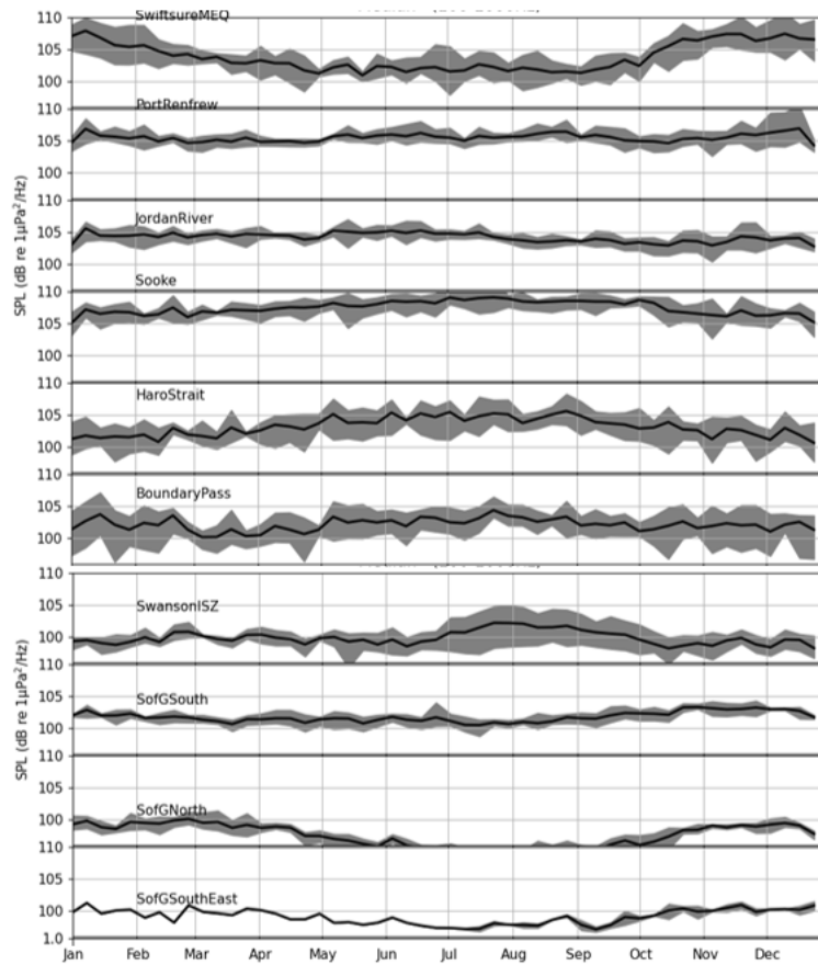
Figure 22: Monthly sound pressure levels (SPL) in the frequency range representing commercial vessel traffic (100-1000 Hz) at each of the mooring locations. The grey shading represents the minimum and maximum observed median levels of all six years (2019-2024), and the black line is the median of all years.
