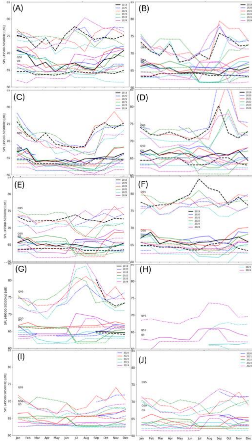
Figure 9: Monthly sound pressure levels (SPL) measured at Q 5 , Q 50 (median) and Q 95 for the 49500-50500 Hz frequency range at (A) Swiftsure Bank, (B) Port Renfrew, (C) Jordan River, (D) Sooke, (E) Haro Strait, (F) Boundary Pass, (G) Swanson Channel, (H) Strait of Georgia South-east, (I) Strait of Georgia South, and (J) Strait of Georgia North.
