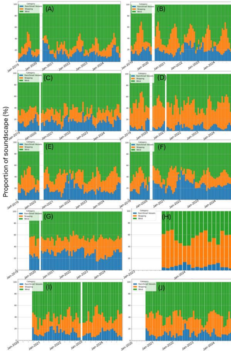
Figure 26: Contributions to the broadband (10-100,000 Hz) soundscape from the commercial vessels (orange), recreational vessels/precipitation (blue) and wind (green) made at (A) Swiftsure Bank, (B) Port Renfrew, (C) Jordan River, (D) Sooke, (E) Haro Strait, (F) Boundary Pass, (G) Swanson Channel, (H) Strait of Georgia South-east, (I) Strait of Georgia South, and (J) Strait of Georgia North, calculated monthly.
