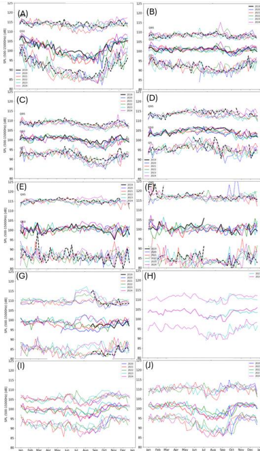
Figure 11: Weekly sound pressure levels (SPL) measured at Q 5 , Q 50 (median) and Q 95 for the southern resident killer whale (SRKW) communication range (500–15000 Hz) at (A) Swiftsure Bank, (B) Port Renfrew, (C) Jordan River, (D) Sooke, (E) Haro Strait, (F) Boundary Pass, (G) Swanson Channel, (H) Strait of Georgia South-east, (I) Strait of Georgia South, and (J) Strait of Georgia North.
