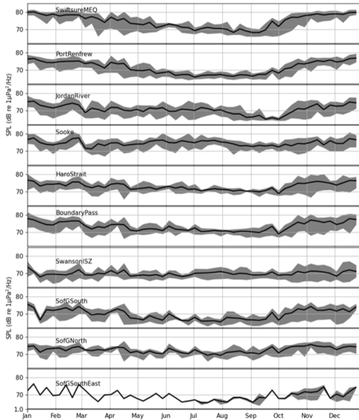
Figure 24: Monthly sound pressure levels (SPL) in the frequency range representing small vessels and precipitation (19500-20500 Hz) at each of the mooring locations. The grey shading represents the minimum and maximum observed median levels of all six years (2019-2024), and the black line is the median of all years.
