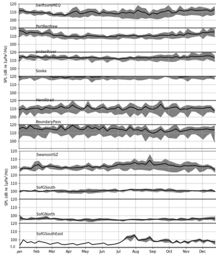
Figure 21: Monthly sound pressure levels (SPL) in the frequency range representing water turbulence (10-100 Hz) at each of the mooring locations. The grey shading represents the minimum and maximum observed median levels of all six years (2019-2024), and the black line is the median of all years.
