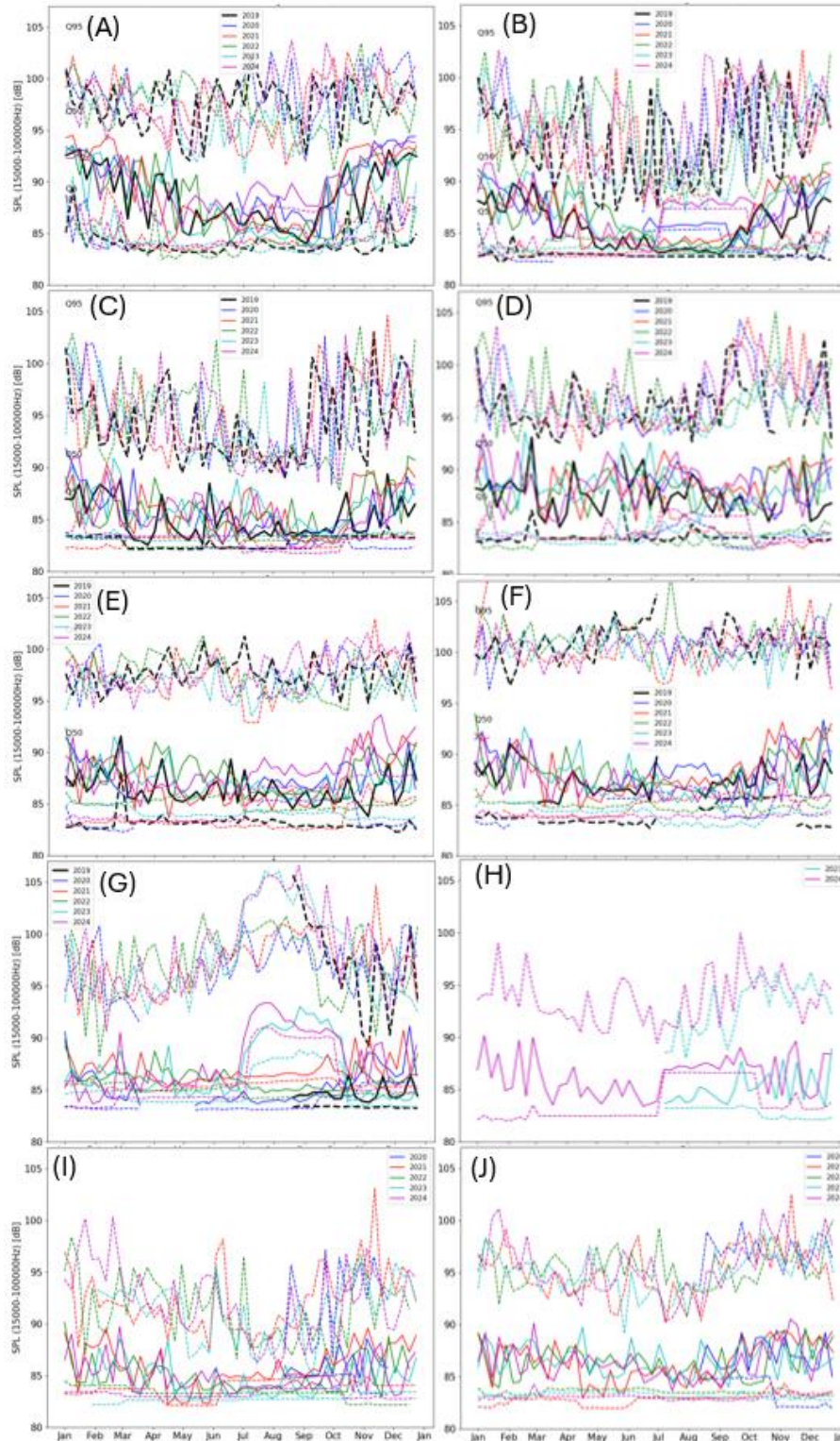
Figure 12: Weekly sound pressure levels (SPL) measured at Q 5 , Q 50 (median) and Q 95 for the southern resident killer whale (SRKW) echolocation range (15000-100000 Hz) at (A) Swiftsure Bank, (B) Port Renfrew, (C) Jordan River, (D) Sooke, (E) Haro Strait, (F) Boundary Pass, (G) Swanson Channel, (H) Strait of Georgia South-east, (I) Strait of Georgia South, and (J) Strait of Georgia North.
