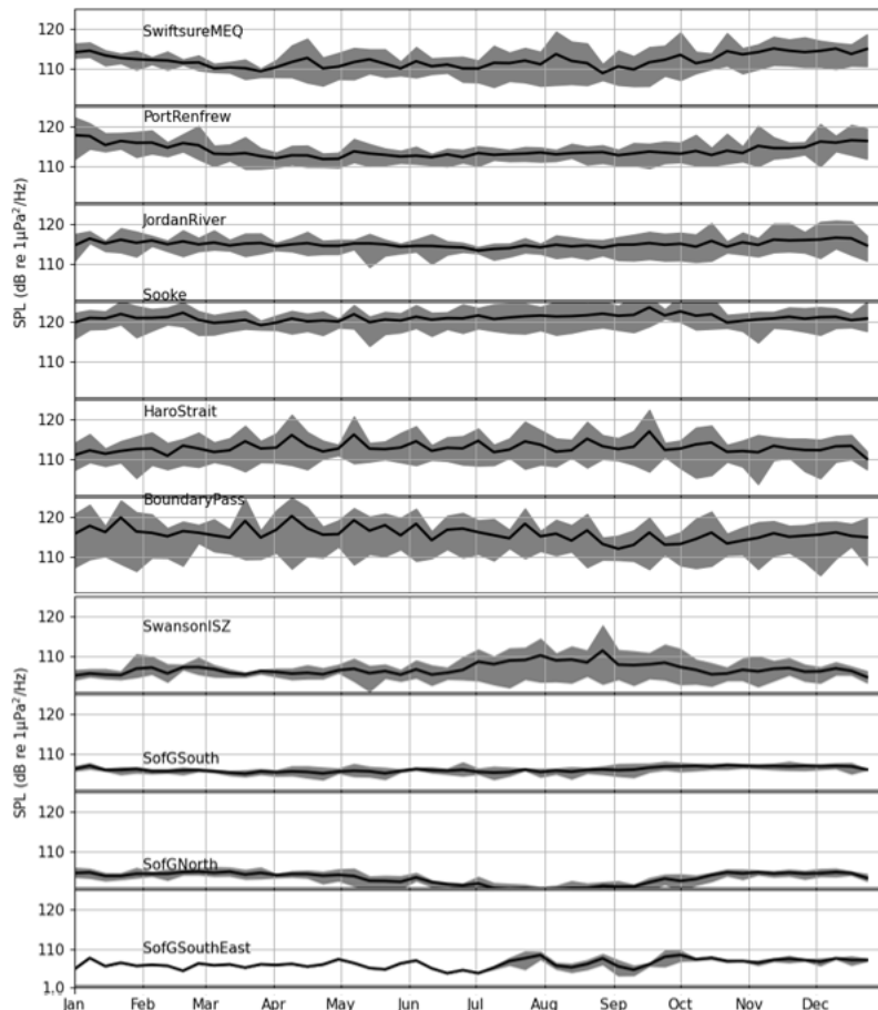
Figure 18: Monthly broadband (10-100,000 Hz) median sound pressure levels (SPL) at each of the mooring locations. The grey shading represents the minimum and maximum observed median levels of all six years (2019-2024), and the black line is the median of all years.
