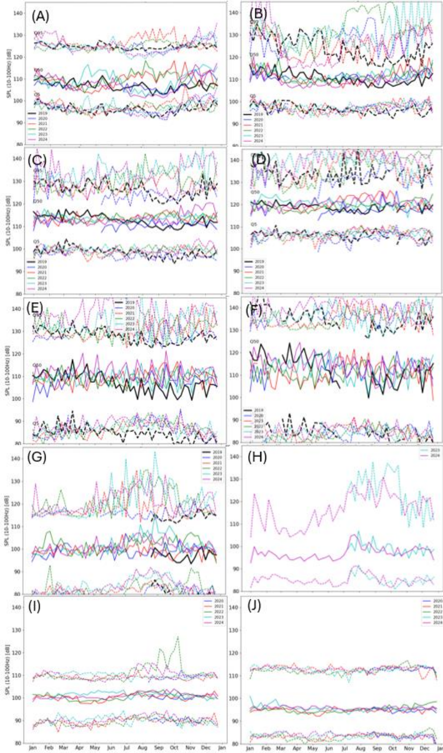
Figure 13: Weekly sound pressure levels (SPL) measured at Q 5 , Q 50 (median) and Q 95 for the 10-100 Hz frequency range at (A) Swiftsure Bank, (B) Port Renfrew, (C) Jordan River, (D) Sooke, (E) Haro Strait, (F) Boundary Pass, (G) Swanson Channel, (H) Strait of Georgia South-east, (I) Strait of Georgia South, and (J) Strait of Georgia North.
