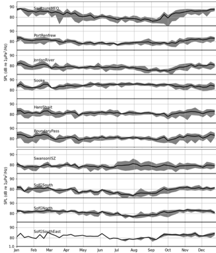
Figure 23: Monthly sound pressure levels (SPL) in the frequency range representing wind (7500-8500 Hz) at each of the mooring locations. The grey shading represents the minimum and maximum observed median levels of all six years (2019-2024), and the black line is the median of all years.
