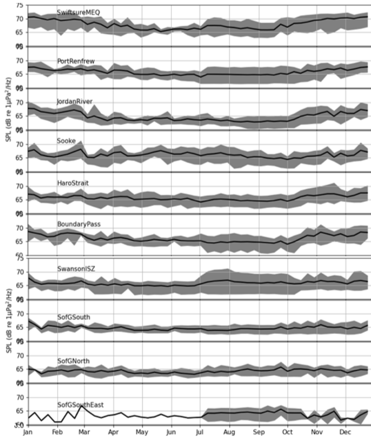
Figure 25: Monthly sound pressure levels (SPL) in the frequency range representing echosounders and recreational vessels (49500-50500 Hz) at each of the mooring locations. The grey shading represents the minimum and maximum observed median levels of all six years (2019-2024), and the black line is the median of all years.
