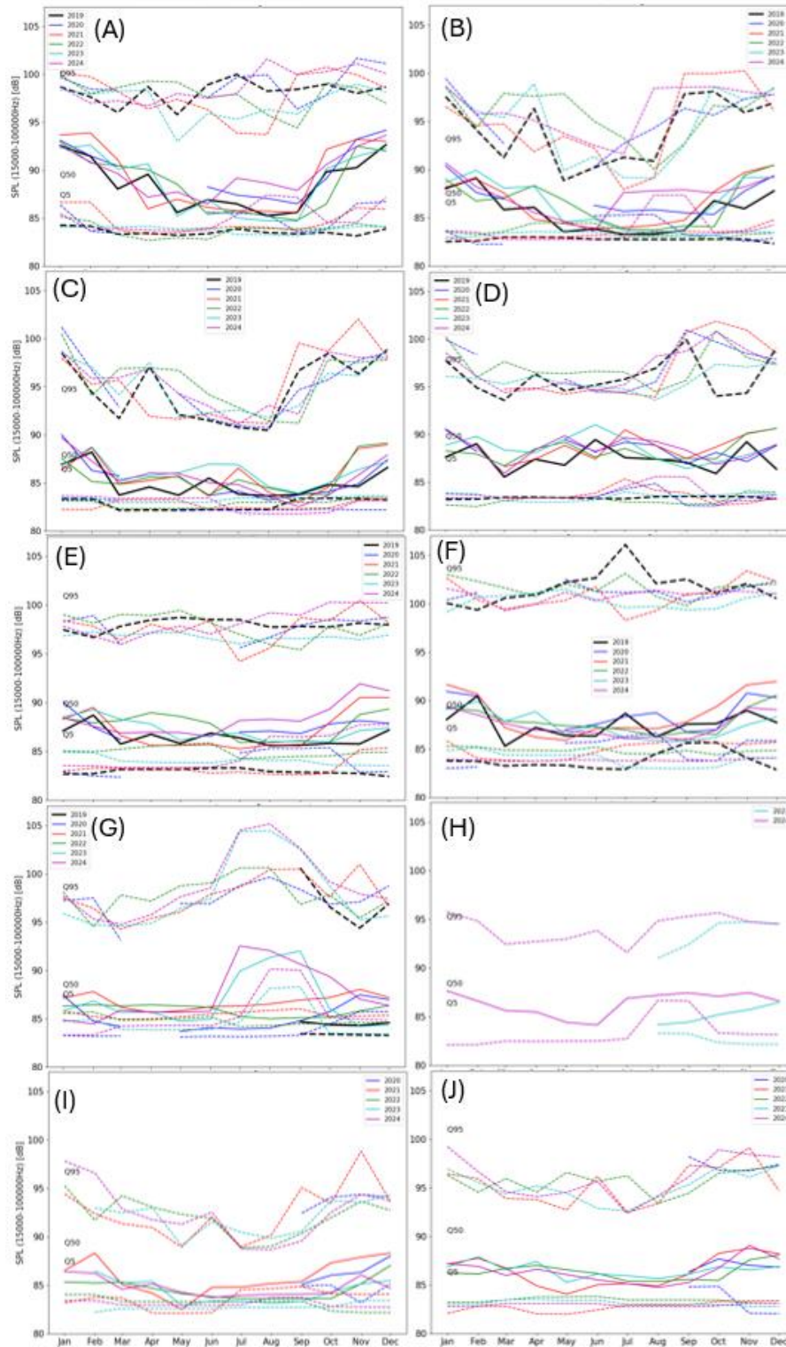
Figure 4: Monthly sound pressure levels (SPL) measured at Q 5 , Q 50 (median) and Q 95 for the southern resident killer whale (SRKW) echolocation range (15000-100000 Hz) at (A) Swiftsure Bank, (B) Port Renfrew, (C) Jordan River, (D) Sooke, (E) Haro Strait, (F) Boundary Pass, (G) Swanson Channel, (H) Strait of Georgia South-east, (I) Strait of Georgia South, and (J) Strait of Georgia North.
