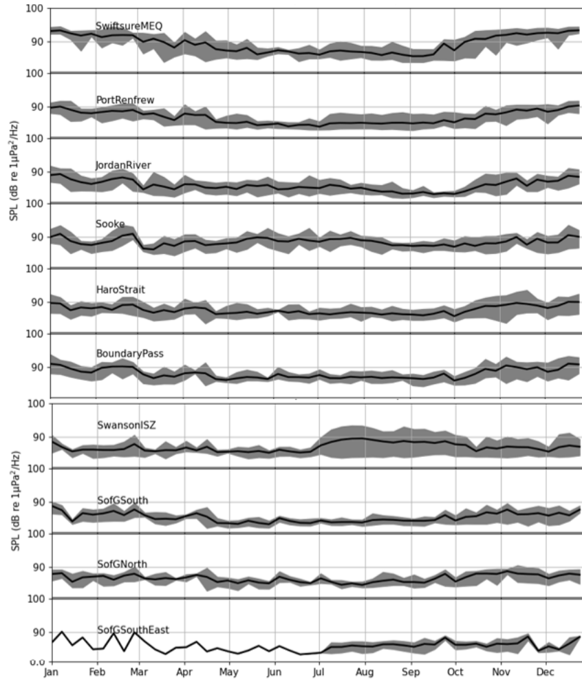
Figure 20: Monthly SRKW echolocation (15-100 kHz) sound pressure levels (SPL) at each of the mooring locations. The grey shading represents the minimum and maximum observed median levels of all six years (2019-2024), and the black line is the median of all years.
