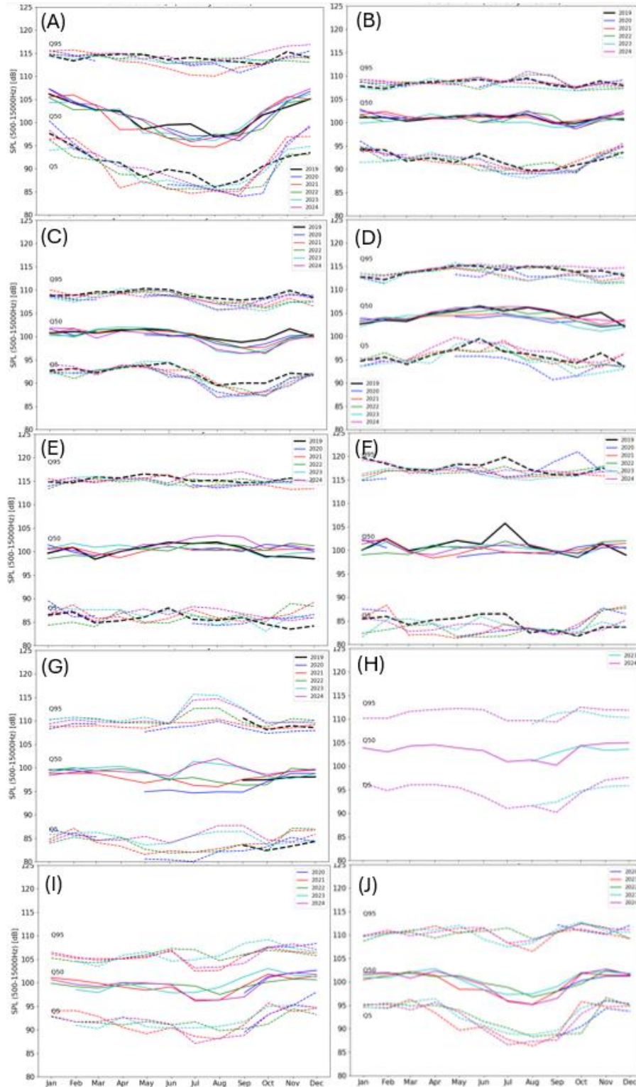
Figure 3: Monthly sound pressure levels (SPL) measured at Q 5 , Q 50 (median) and Q 95 for the southern resident killer whale (SRKW) communication range (500-15000 Hz) at (A) Swiftsure Bank, (B) Port Renfrew, (C) Jordan River, (D) Sooke, (E) Haro Strait, (F) Boundary Pass, (G) Swanson Channel, (H) Strait of Georgia South-east, (I) Strait of Georgia South, and (J) Strait of Georgia North.
