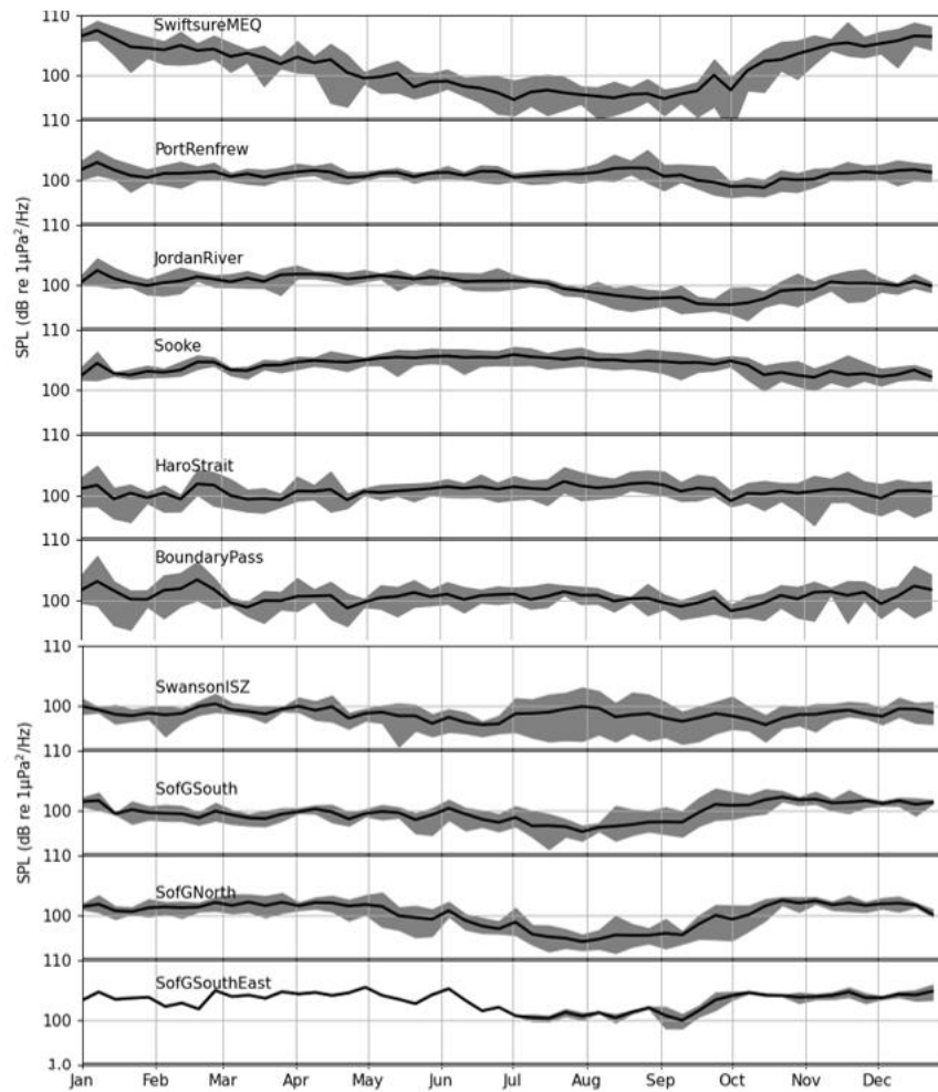
Figure 19: Monthly SRKW communication (500-15000 Hz) sound pressure levels (SPL) at each of the mooring locations. The grey shading represents the minimum and maximum observed median levels of all six years (2019-2024), and the black line is the median of all years.
