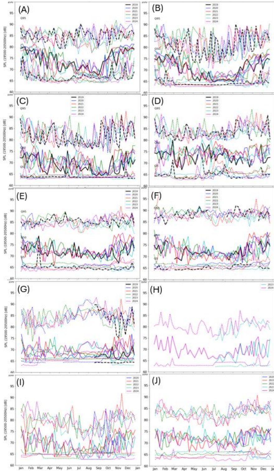
Figure 16: Weekly sound pressure levels (SPL) measured at Q 5 , Q 50 (median) and Q 95 for the 19500-20500 Hz frequency range at (A) Swiftsure Bank, (B) Port Renfrew, (C) Jordan River, (D) Sooke, (E) Haro Strait, (F) Boundary Pass, (G) Swanson Channel, (H) Strait of Georgia South-east, (I) Strait of Georgia South, and (J) Strait of Georgia North.
