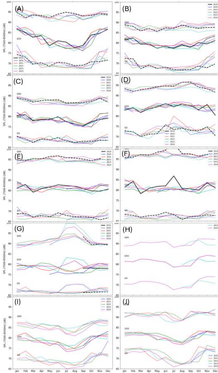
Figure 7: Monthly sound pressure levels (SPL) measured at Q 5 , Q 50 (median) and Q 95 for the 7500-8500 Hz frequency range at (A) Swiftsure Bank, (B) Port Renfrew, (C) Jordan River, (D) Sooke, (E) Haro Strait, (F) Boundary Pass, (G) Swanson Channel, (H) Strait of Georgia South-east, (I) Strait of Georgia South, and (J) Strait of Georgia North.
