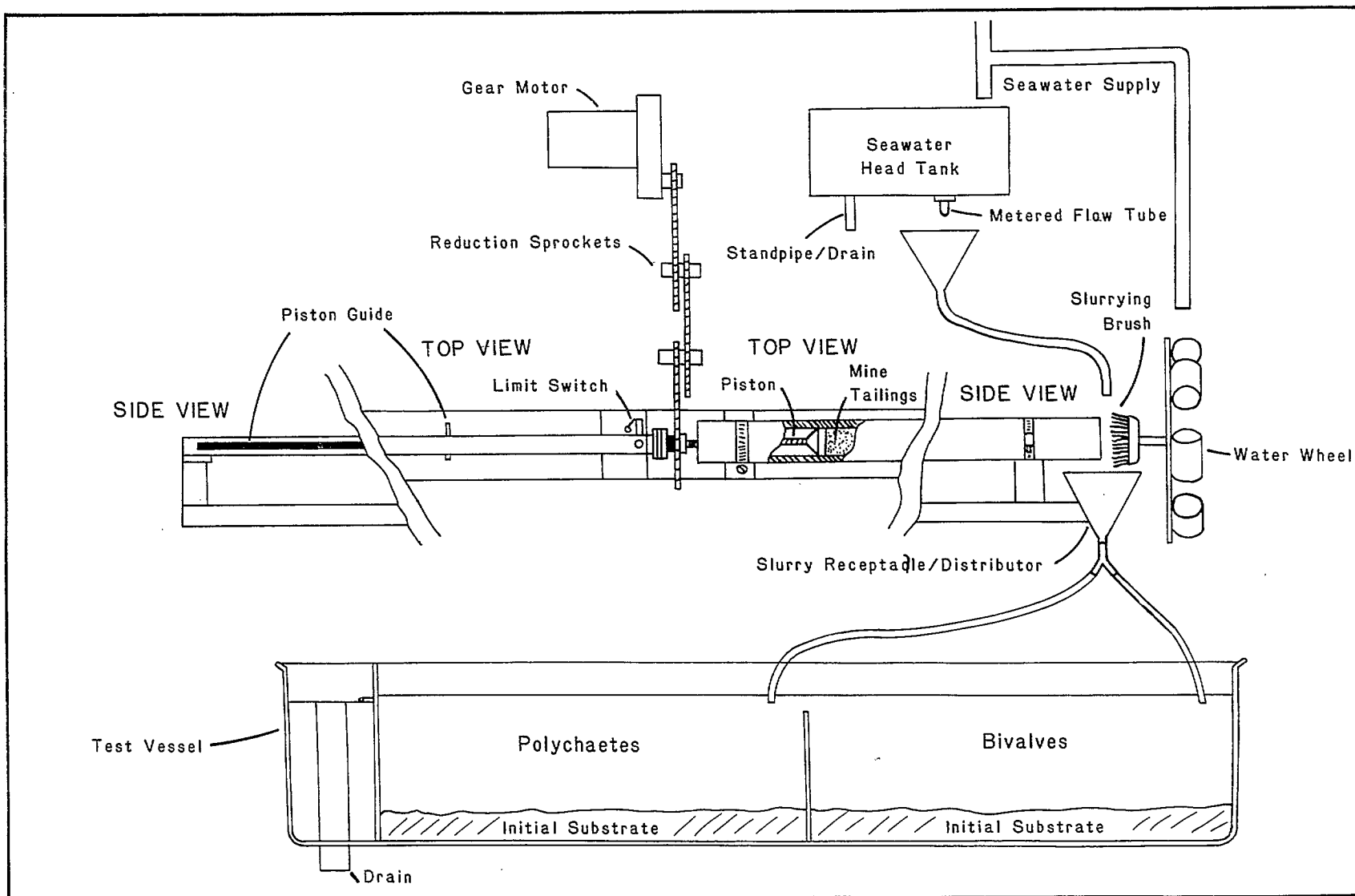
FIGURE 2. Schematic representation of continuous deposition apparatus. (Note: The substrate and polychaete/bivalve partition were removed for the 11 day study)
