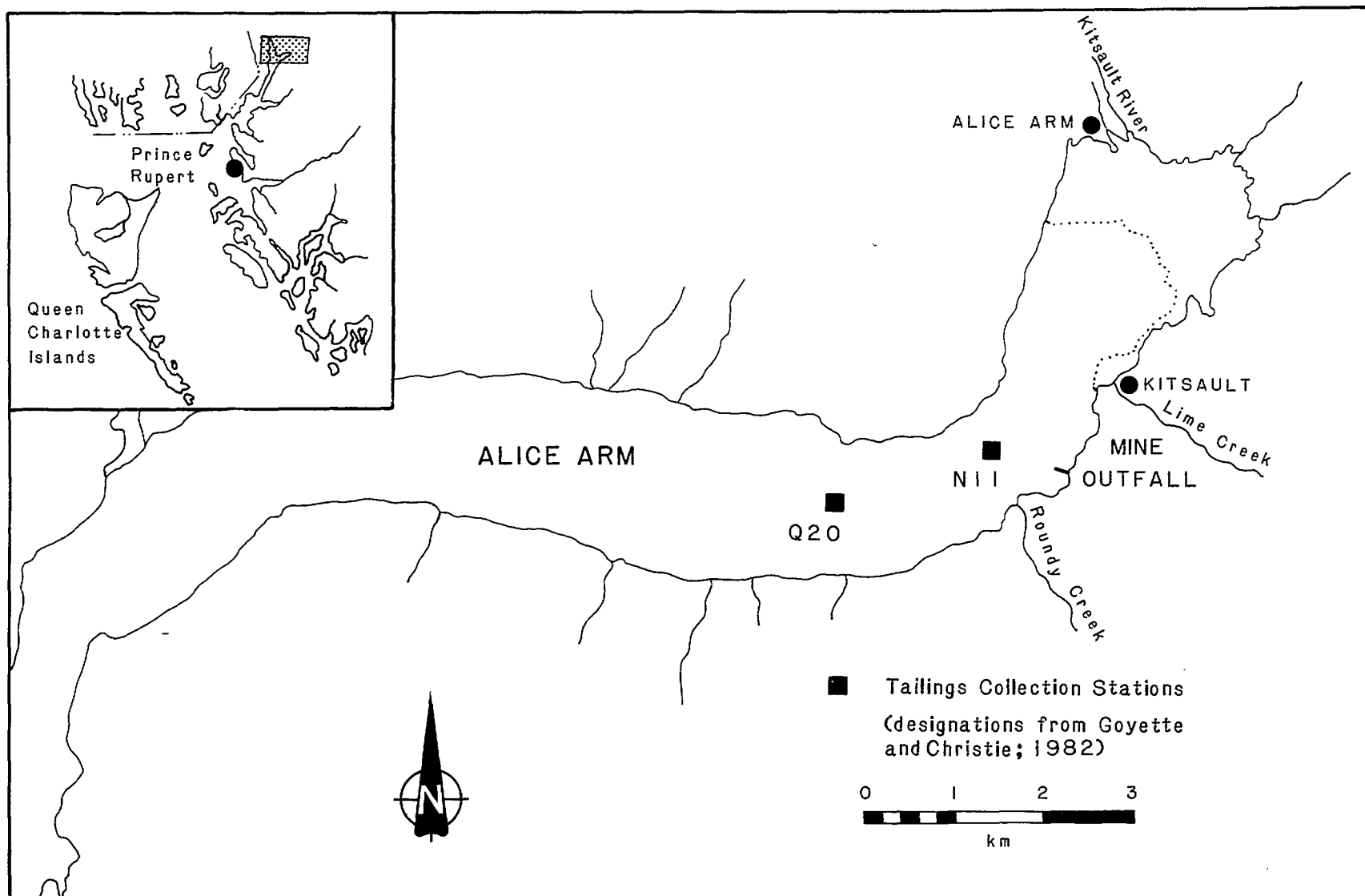
FIGURE 1. Collection site for Amax/Kitsault mine tailings.
