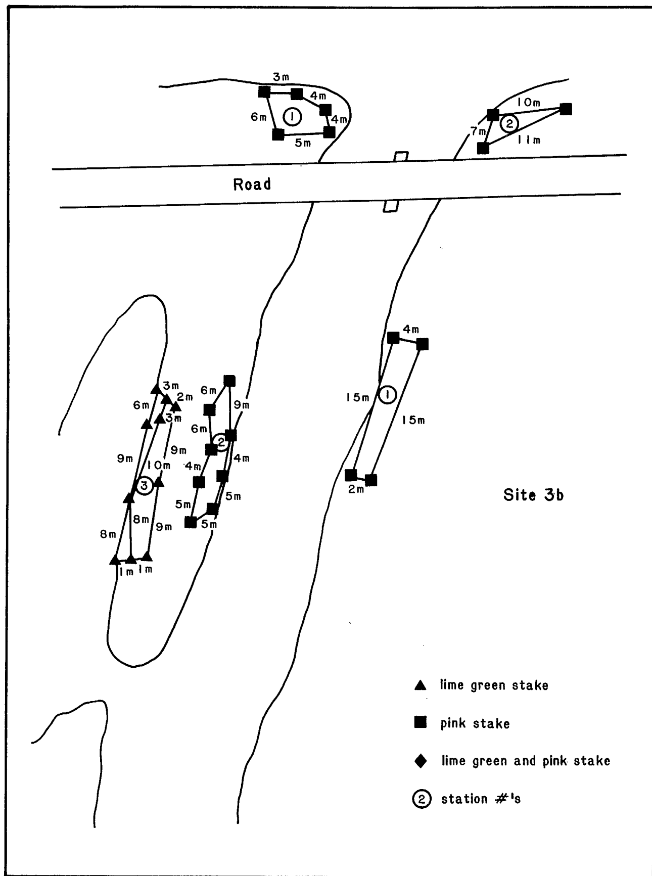
Fig. 4 Survey Map of Sites 3a and 3b
