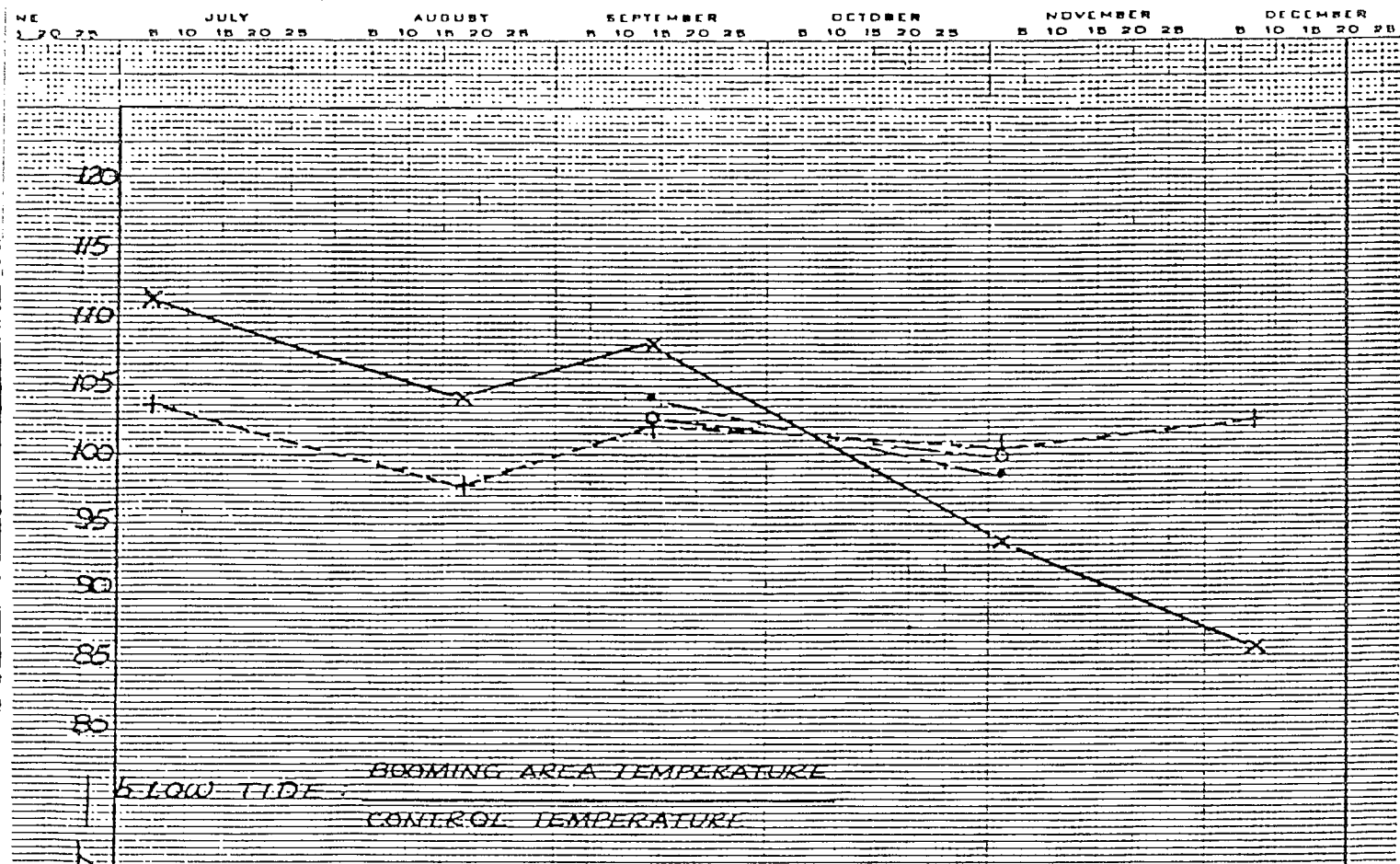
FIG. 2. BOOMING AREA WATER TEMPERATURE / CONTROL WATER TEMPERATURE BY DEPTH AND TIME
