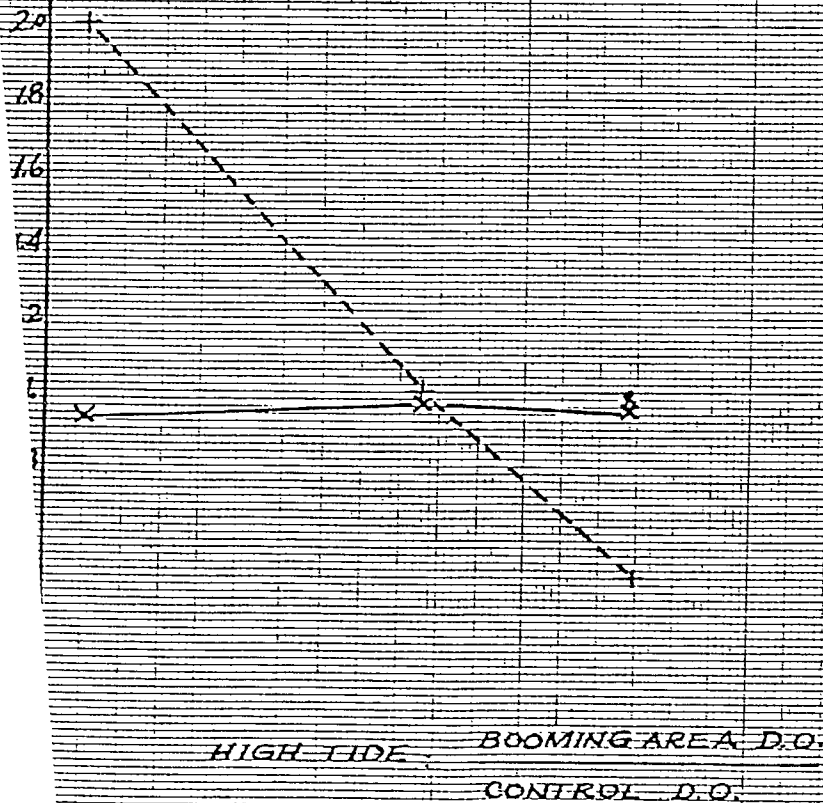
FIGURE 7: BOOMING AREA DISSOLVED OXYGEN / CONTROL DISSOLVED OXYGEN BY DEPTH, TIDE AND TIME
