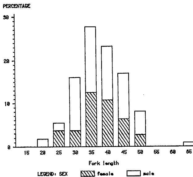
Fig. 2b. Length-frequency distribution for yelloweye rockfish. Fork length (cm) is the midpoint of the size interval.
