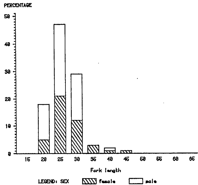
Fig. 2a. Length-frequency distribution of copper rockfish. Fork length (cm) is the midpoint of the size interval.
