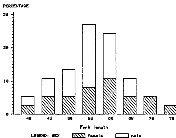
Fig. 4b. Length-frequency distribution for lingcod caught in the recreational fishery. Fork length (cm) is the midpoint of the size interval.
