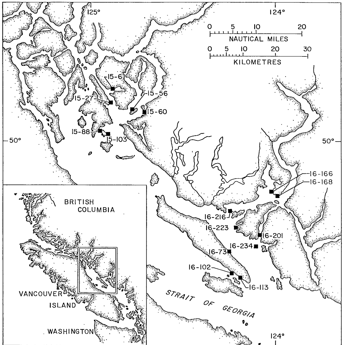
Fig. 1. Locations of study sites.
