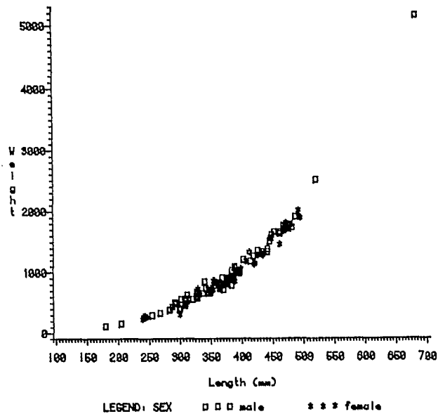
Fig. 5d. The relationship between weight (g) and fork length (mm) for yelloweye rockfish.
