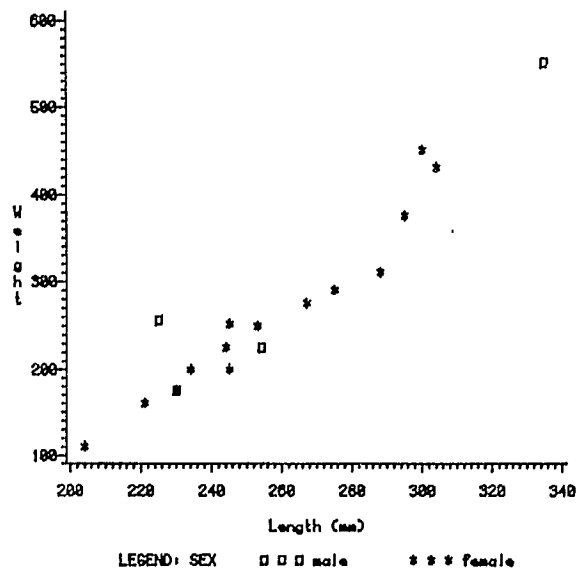
Fig. 5b. The relationship between weight (g) and fork length (mm) for greenstriped rockfish.
