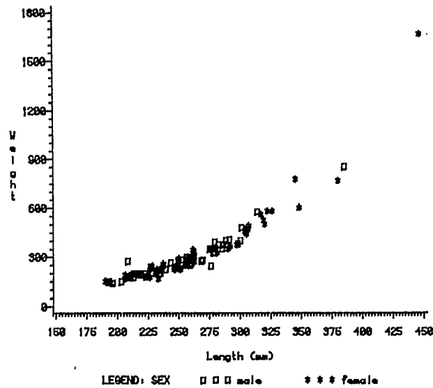
Fig. 5a. The relationship between weight (g) and fork length (mm) for copper rockfish.
