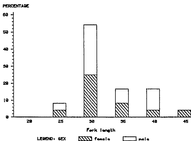
Fig. 4a. Length-frequency distribution for quillback rockfish caught in the recreational fishery. Fork length (cm) is the midpoint of the size interval.
