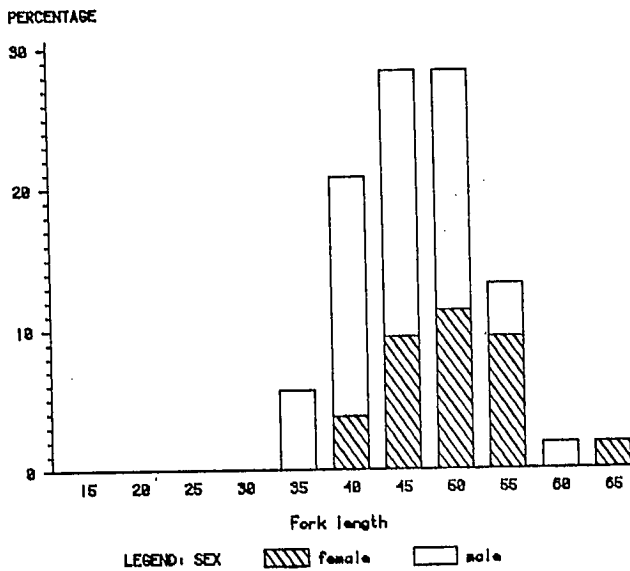
Fig. 2c. Length-frequency distribution for lingcod. Fork length (cm) is the midpoint of the size interval.
