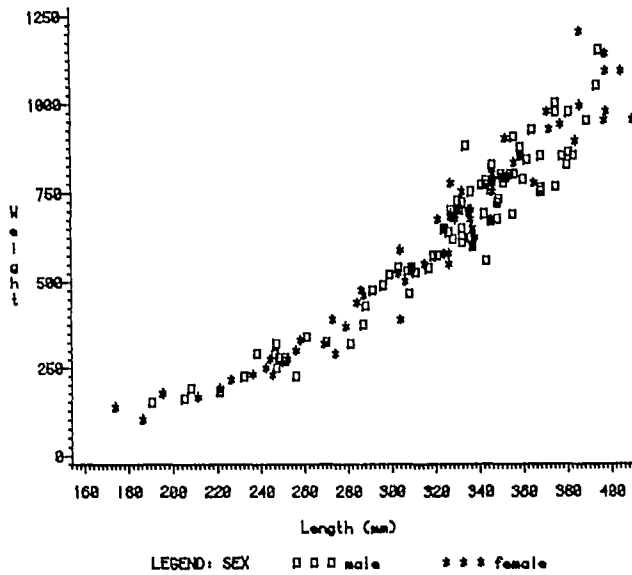
Fig. 5c. The relationship between weight (g) and fork length (mm) for quillback rockfish.
