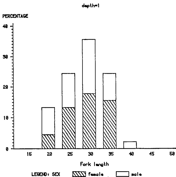
Fig. 3. Length-frequency distribution for quillback rockfish. Fork length (cm) is the midpoint of the size interval. Depths are 5-40 m (1), 41-70 m (2), 71-100 m (3).
