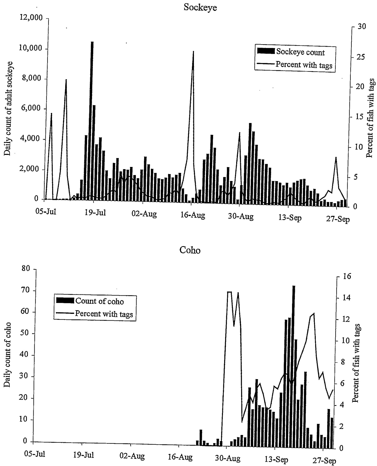
Figure 11. Daily counts and percent of fish with tags for sockeye and coho salmon passing through the Meziadin fishway, 1997. A running 5-day average was used for the percent of coho salmon with tags.
