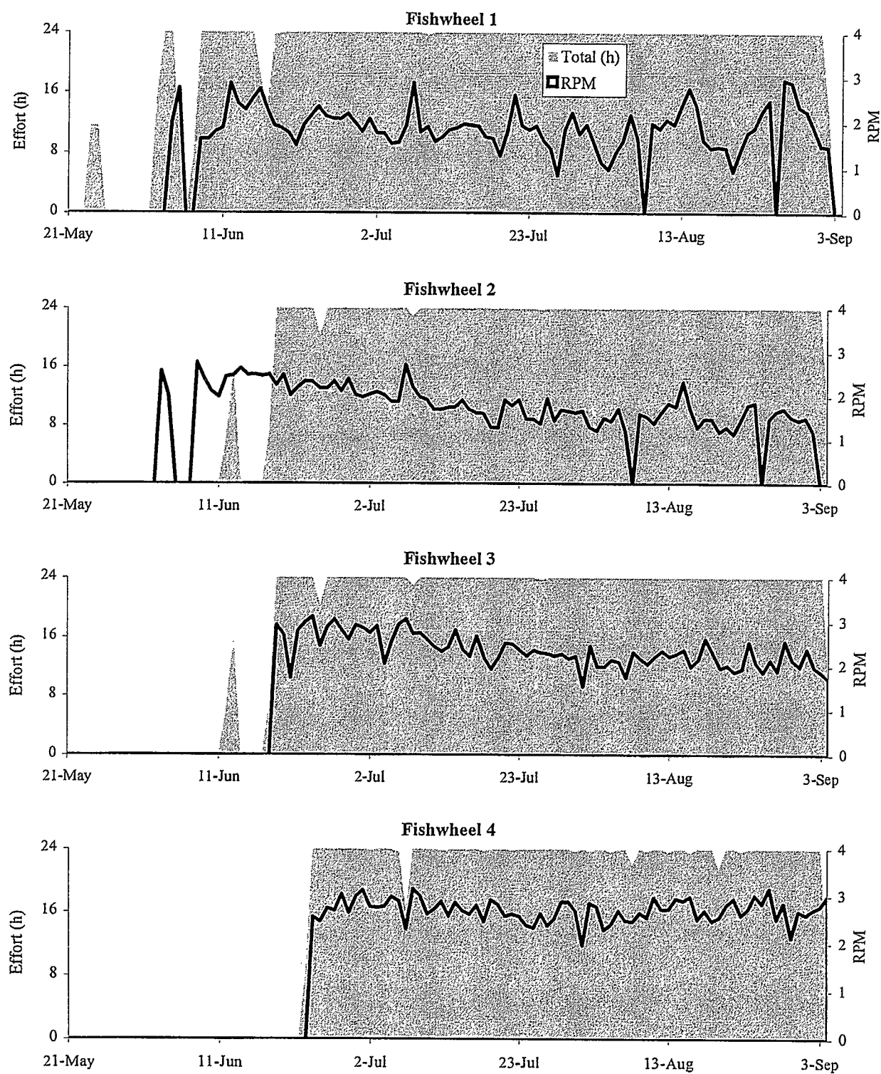
Figure 2. Fishwheel effort (hours) and speed (RPM) for four fishwheels on the Nass River, 1997.
