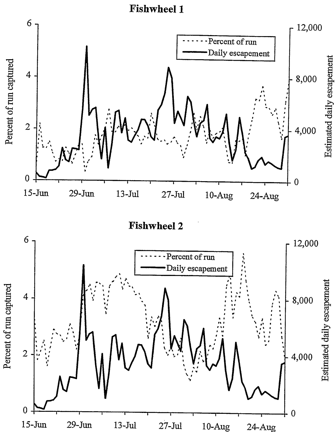
Figure 13. Percent of the sockeye salmon run captured by fishwheels 1 and 2 versus estimated daily escapement, 1997.
