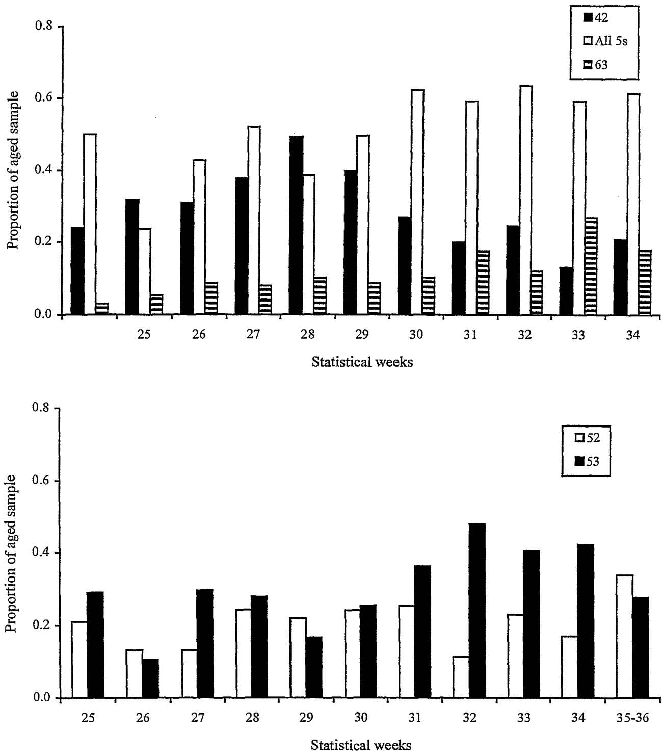
Figure 15. Weekly age composition of successfully aged sockeye salmon sampled from the Nass River fishwheel catch, 1997 (most common ages only, top: the aged-five fish were pooled for clarity).
