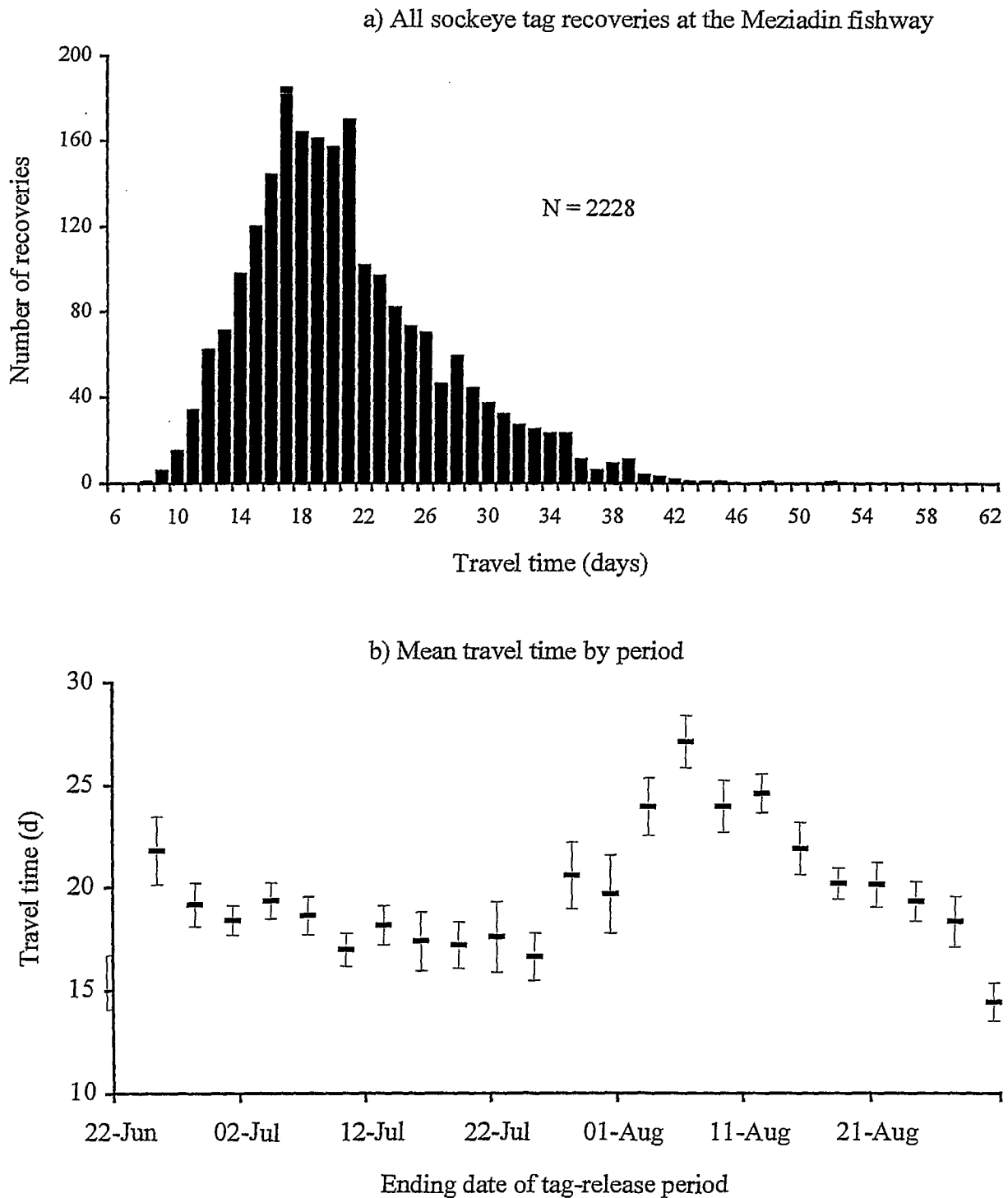
Figure 12. a) The distribution of travel times (days) to the Meziadin fishway for sockeye salmon tagged at the Nass River fishwheels and recovered at the Meziadin fishway, 1997. b) Mean travel time (with 95% confidence intervals) for 3-day release periods.
