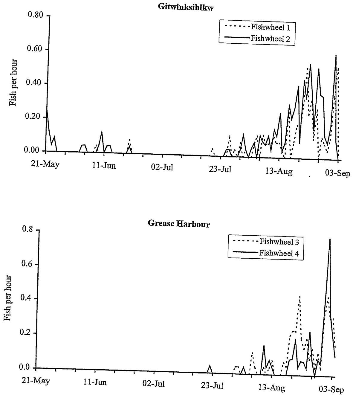
Figure 6. Fishwheel CPUE (catch per wheel hour) for adult steelhead captured with four fishwheels on the Nass River, 1997.
