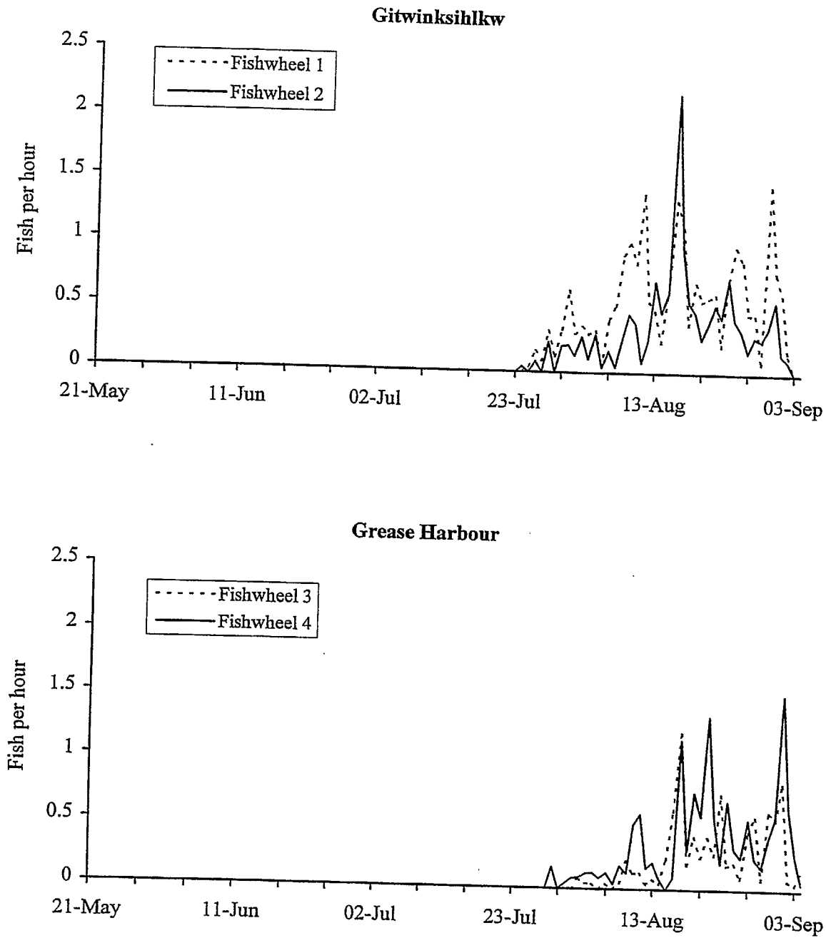
Figure 5. Fishwheel CPUE (catch per wheel hour) for adult coho salmon captured with four fishwheels on the Nass River, 1997.
