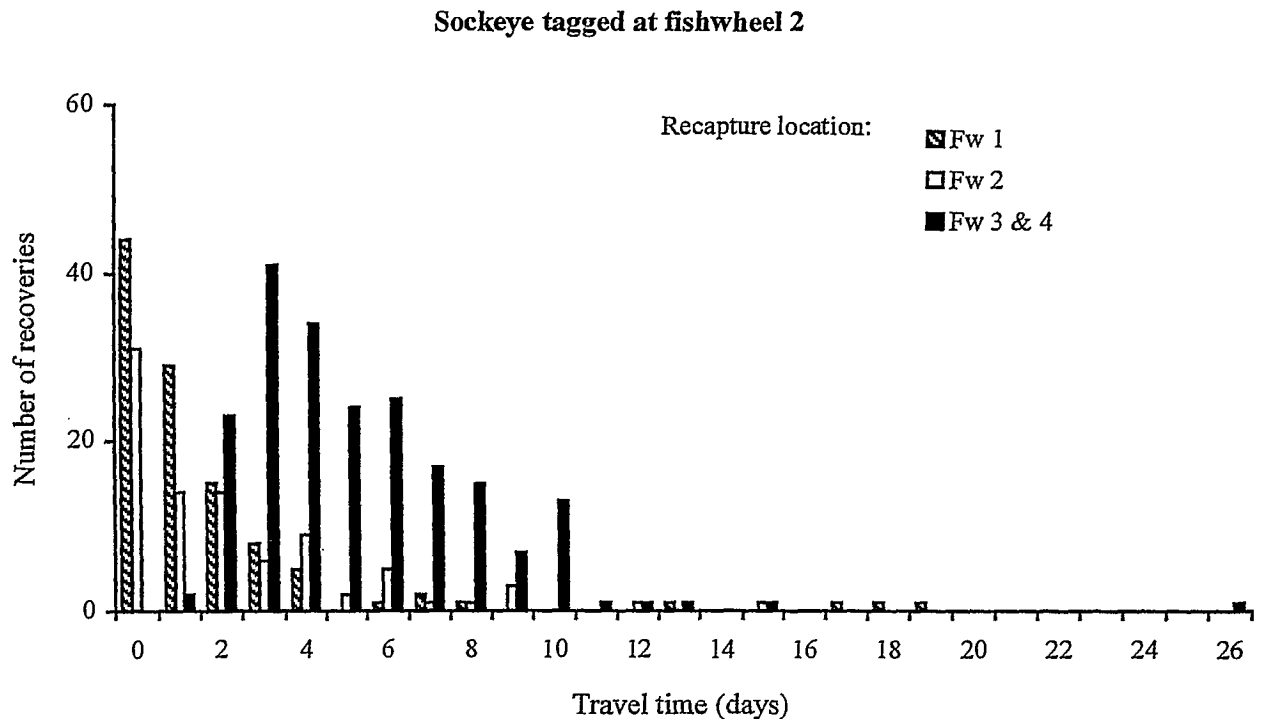
Figure 10. Time between release and recapture for sockeye salmon tagged at fishwheels 1 and 2 and subsequently recaptured in each of the four fishwheels, 1997. Fishwheel 3 and 4 were pooled for clarity.
