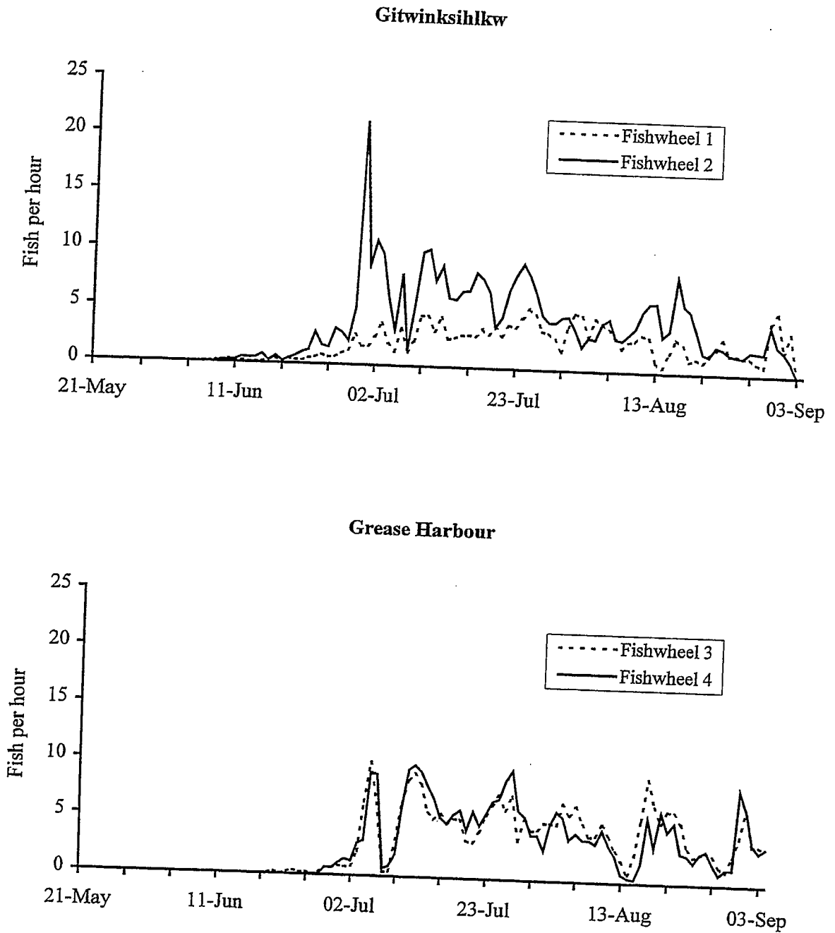
Figure 4. Fishwheel CPUE (catch per wheel hour) for adult sockeye salmon captured with four fishwheels on the Nass River, 1997.
