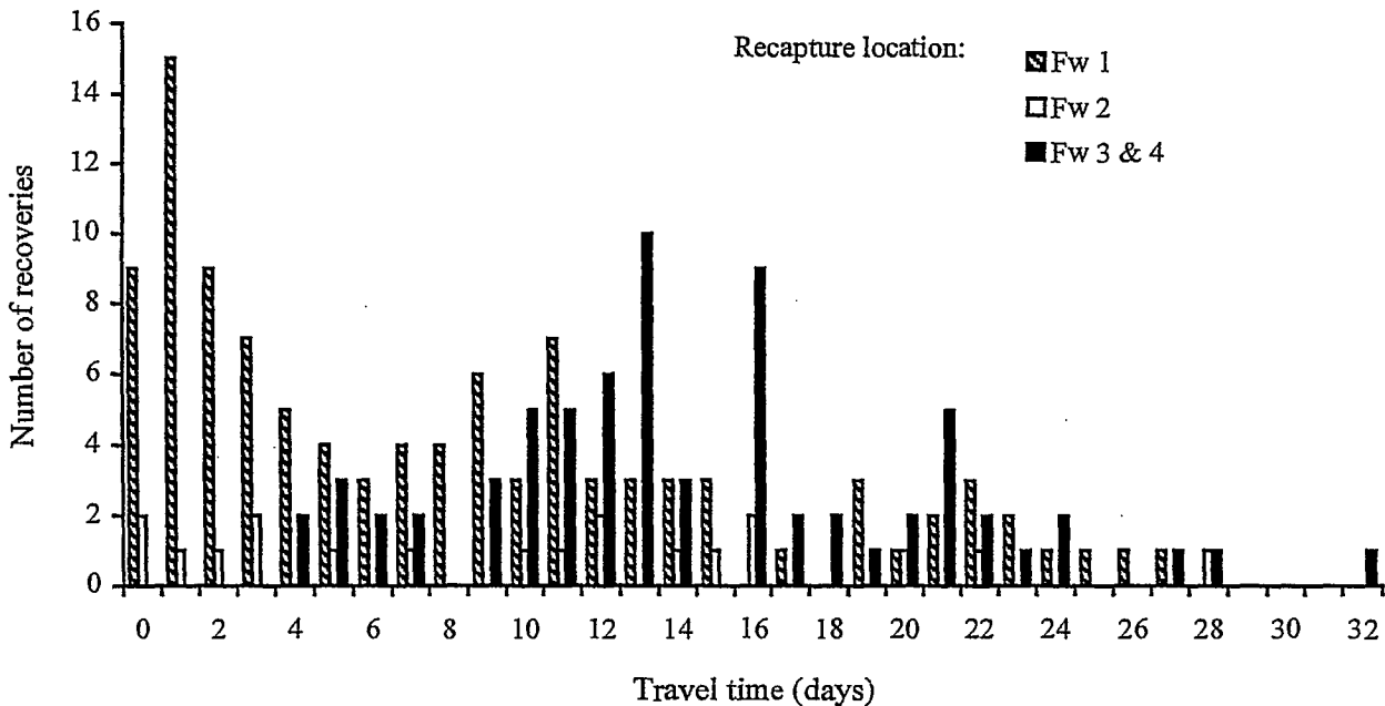
Figure 9. Time between release and recapture for chinook salmon tagged at fishwheels 1 and 2 and subsequently recaptured in each of the four fishwheels, 1997. Fishwheel 3 and 4 were pooled for clarity.
