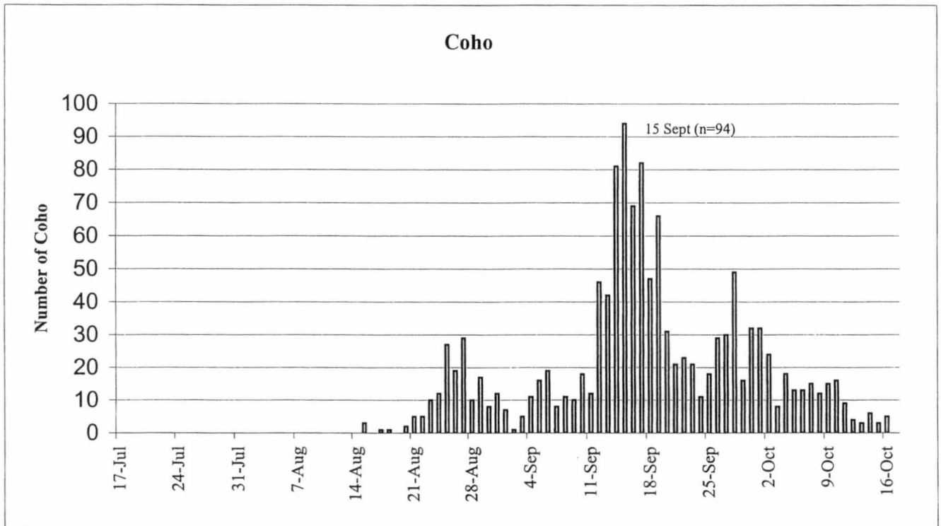
Figure 7. Daily net upstream counts of adult coho through Kwinageese River counting fence, 2002.
