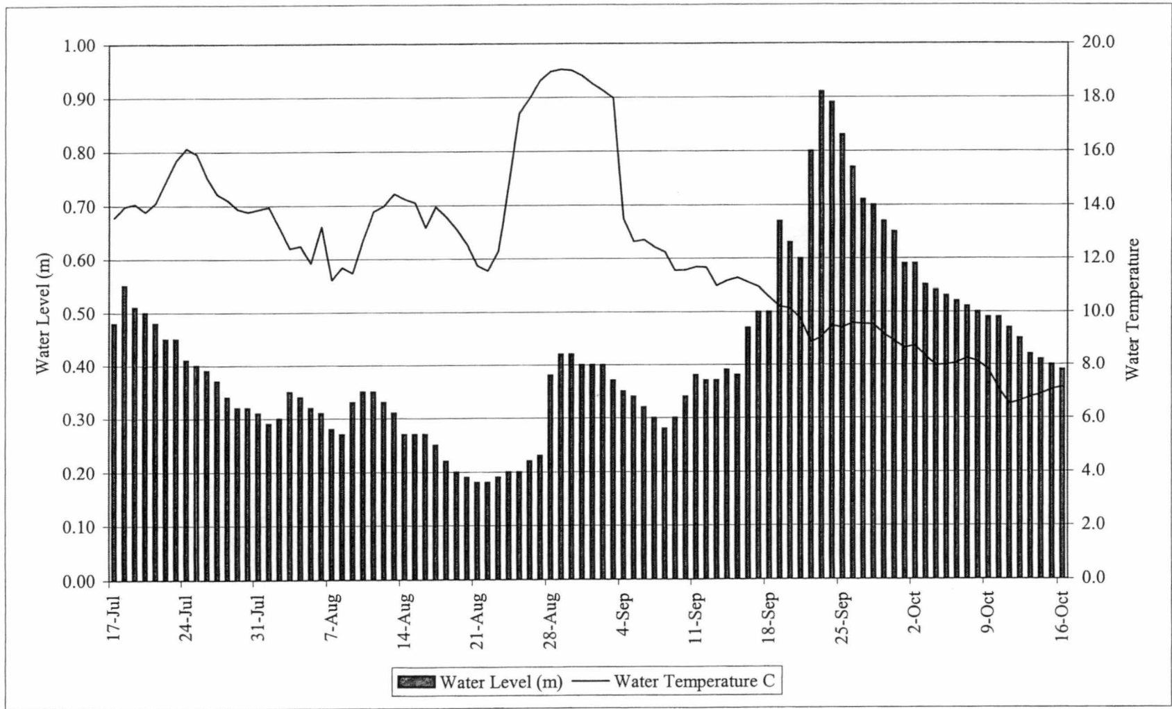
Figure 4. Water level and temperature at Kwinageese River, 2002
