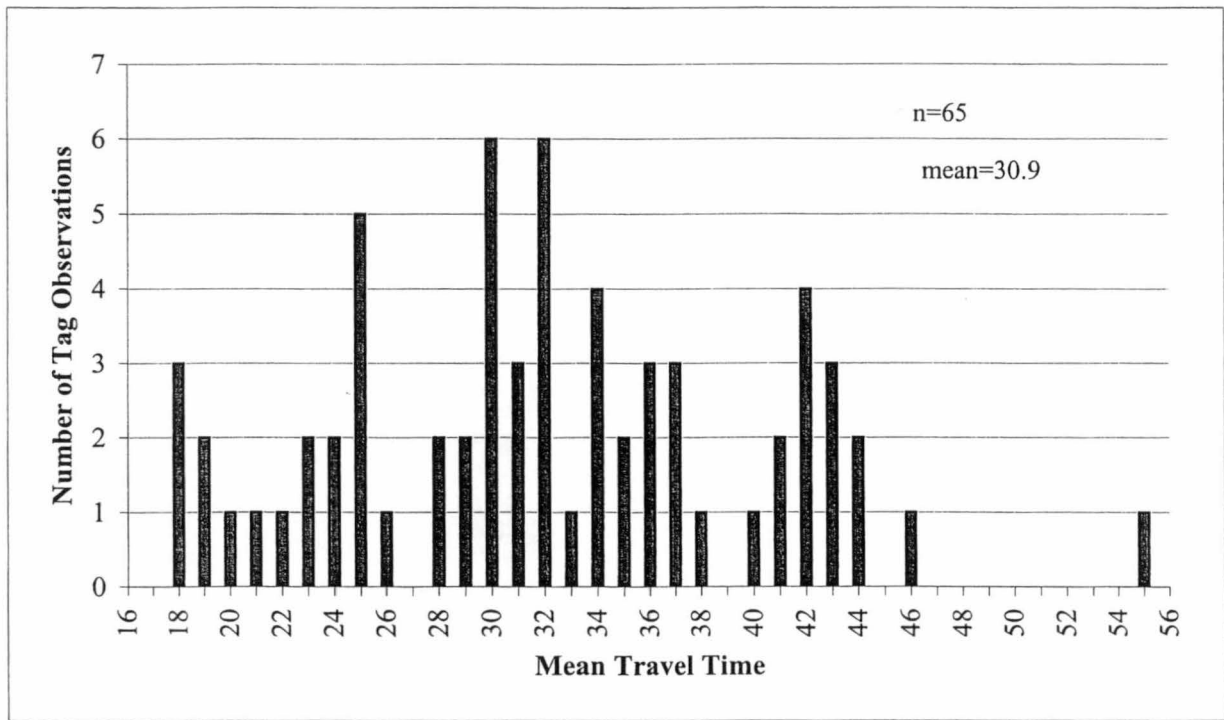
Figure 12. The distribution of mean travel times (days) to the Kwinageese River counting site for sockeye salmon tagged at the Nass River fishwheels, 2002
