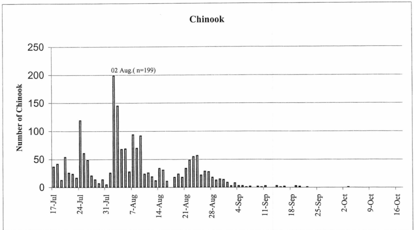
Figure 5. Daily net upstream counts of adult chinook through Kwinageese River counting fence, 2002.
