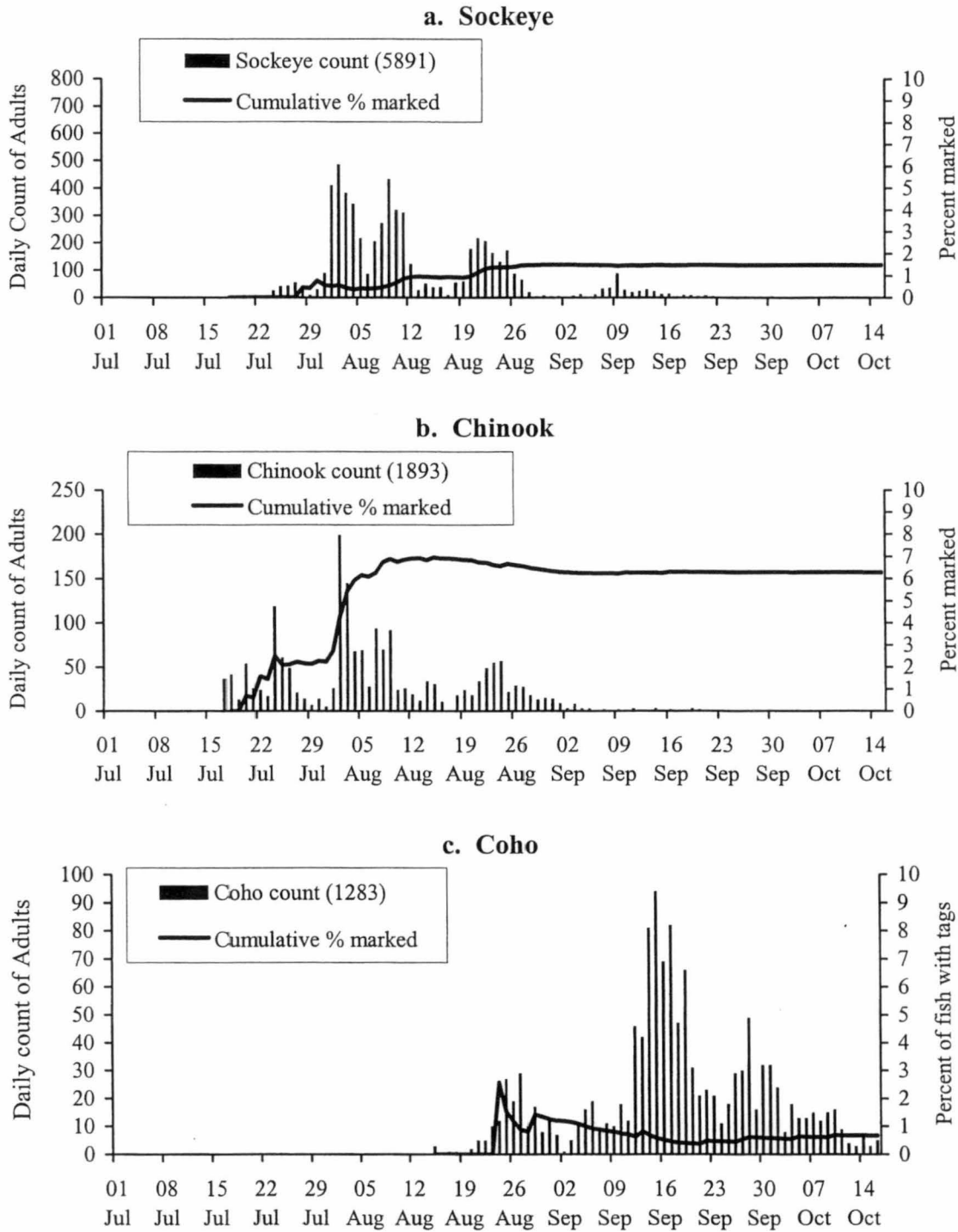
Figure 10. Daily counts and mark rate for sockeye, chinook and coho salmon passing through the Kwinageese weir, 17 July to 17 October 2002.
