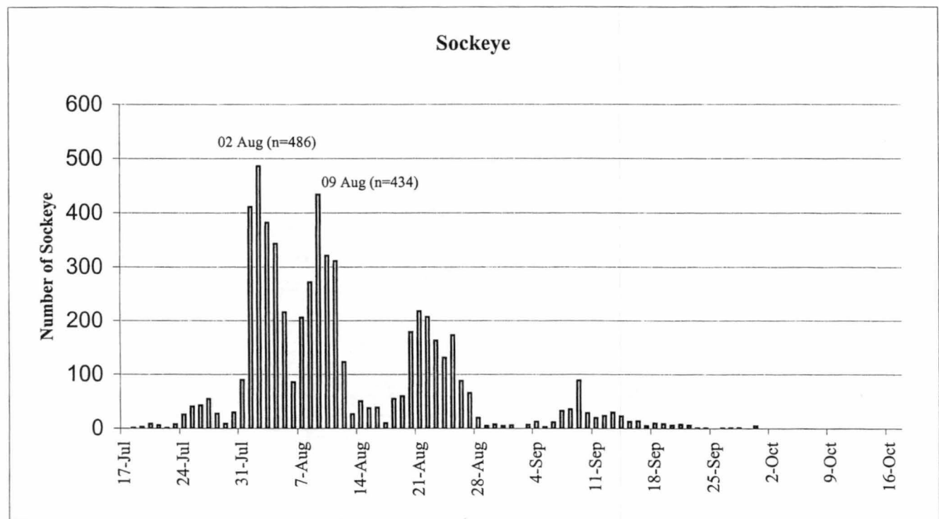
Figure 6. Daily net upstream counts of adult sockeye through Kwinageese River counting fence, 2002.
