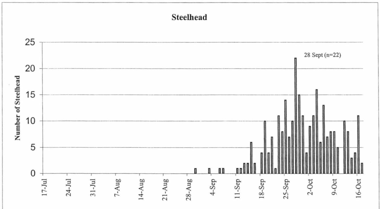
Figure 8. Daily net upstream counts of adult steelhead through Kwinageese River counting fence, 2002.
