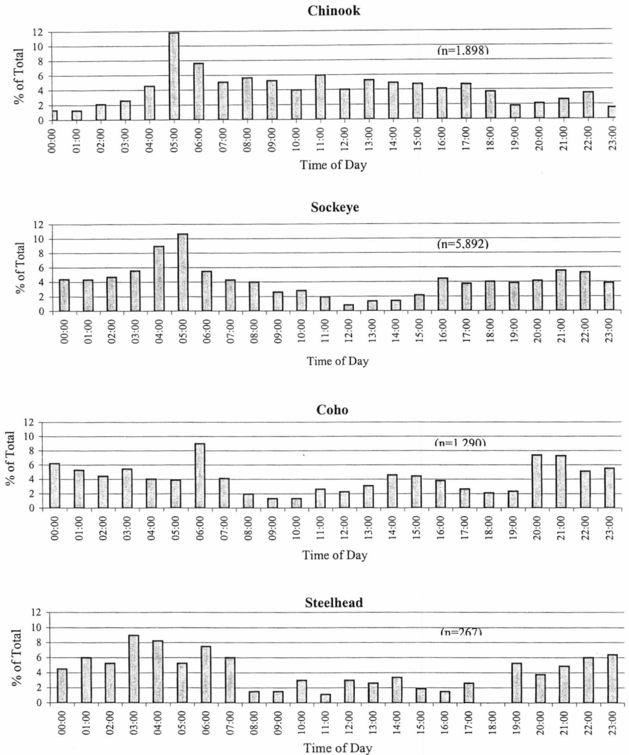
Figure 9. Diel timing of chinook, sockeye, coho and steelhead migration through the Kwinageese River video counting weir in 2002.
