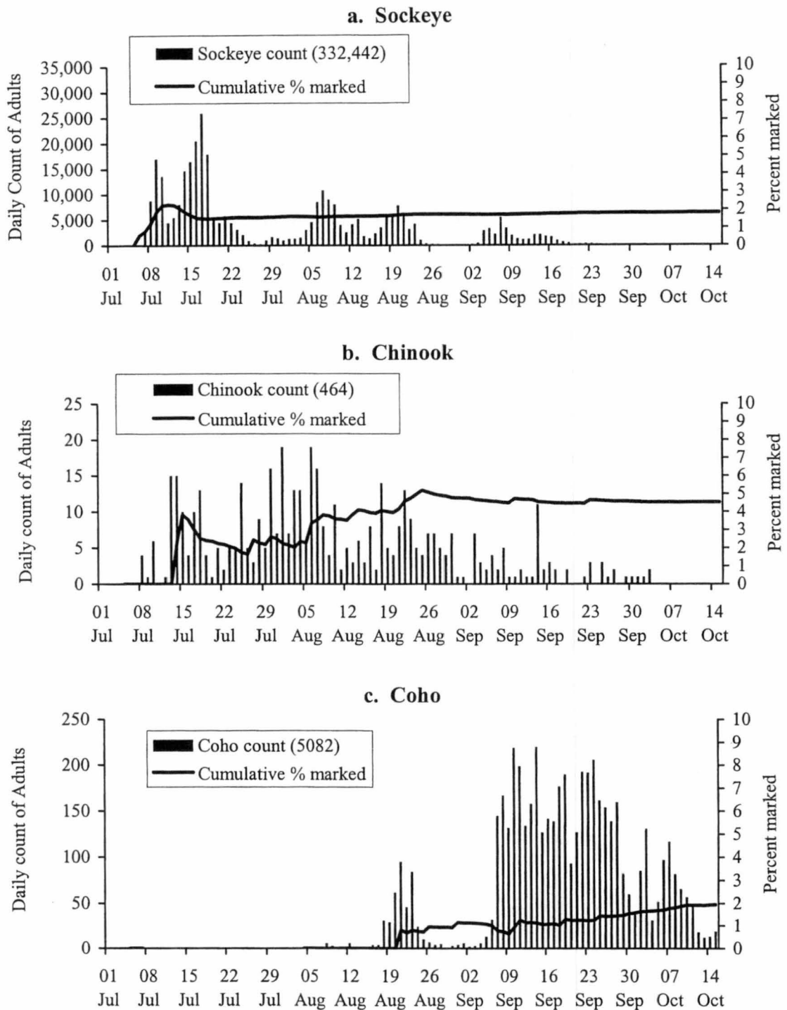
Figure 11. Daily counts and mark rate for sockeye, chinook and coho salmon passing through the Meziadin fishway, 1 July to 15 October 2002. Data from Alexander and Bocking, In Prep.
