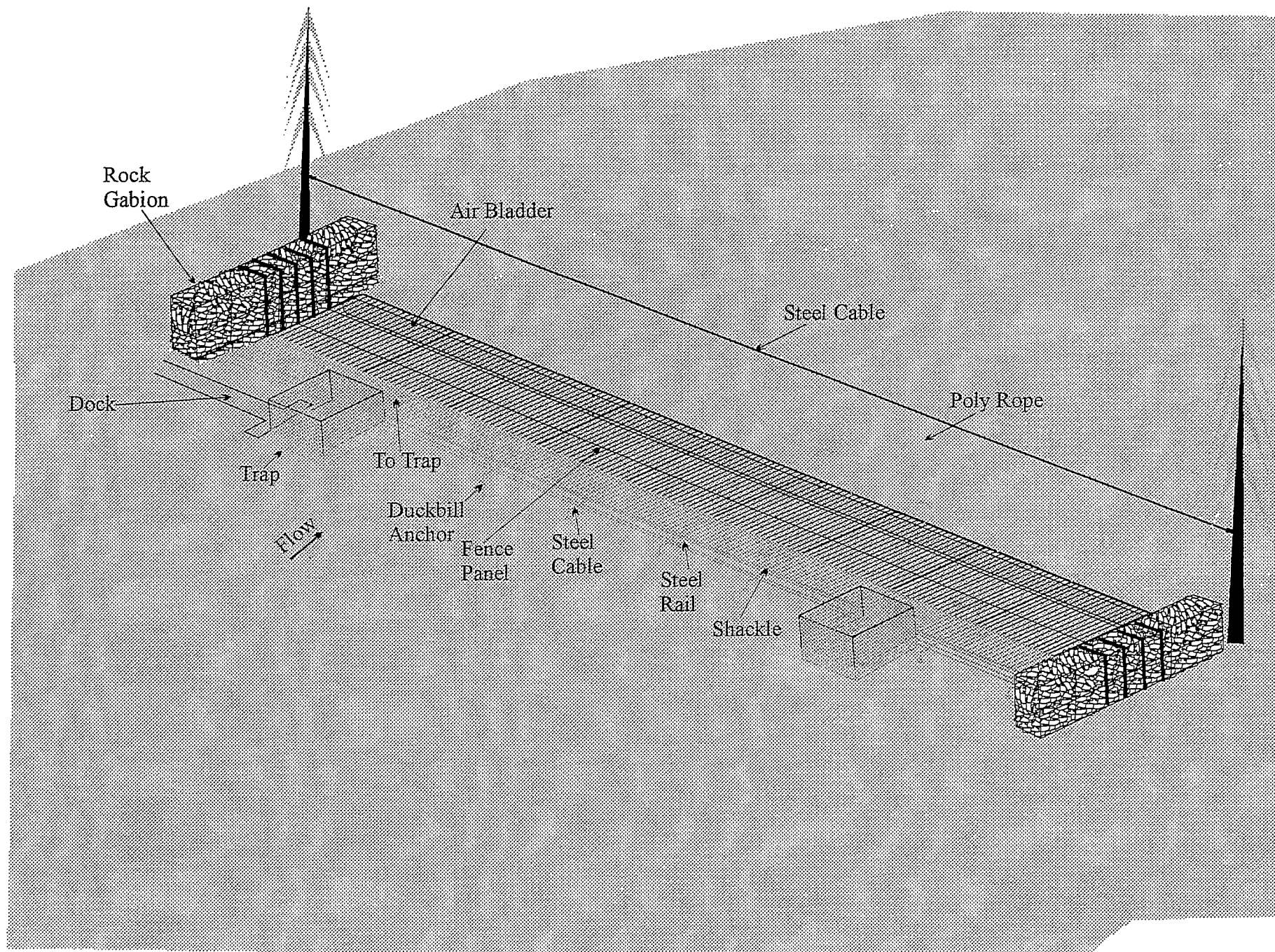
Figure D-1. Floating fence used at Zolzap Creek in 2004. (Schematic not to scale)
