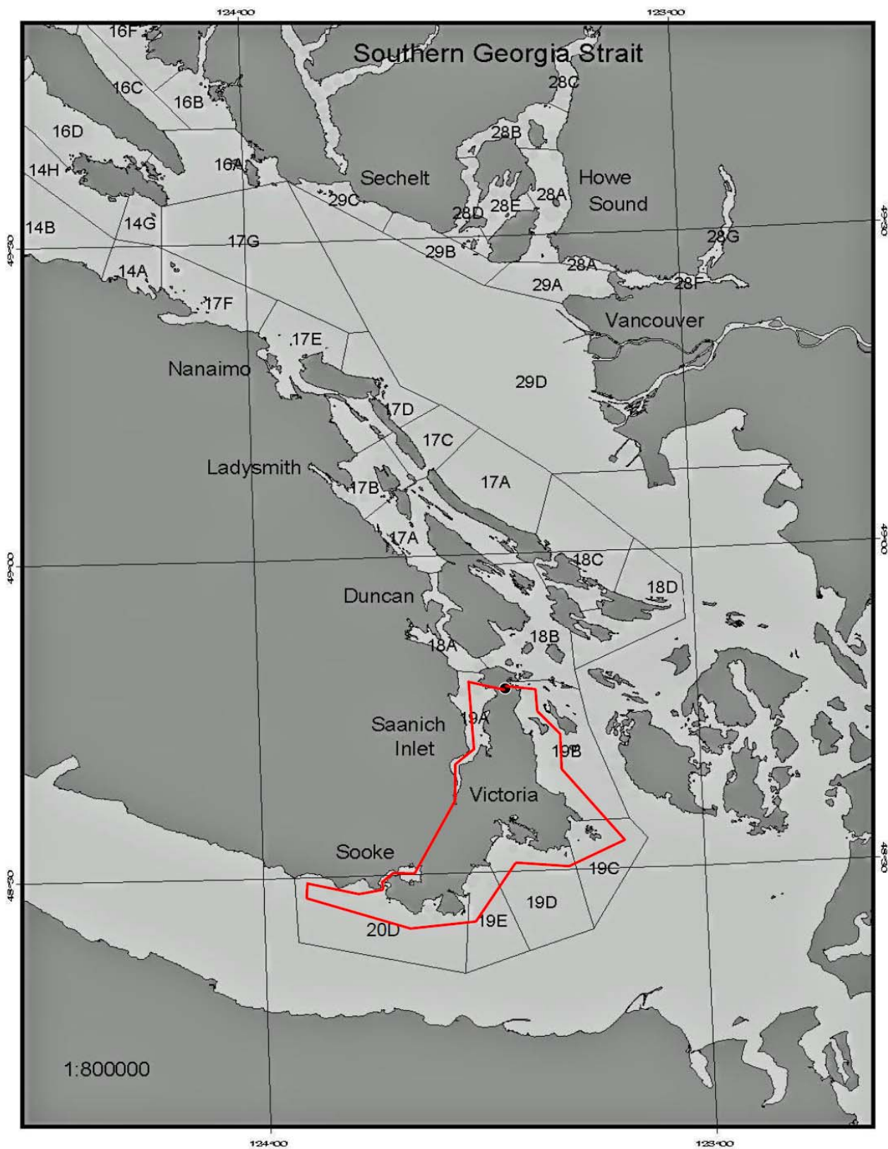
Figure 3c. SG creel survey southern aerial survey winter route, 2010.
