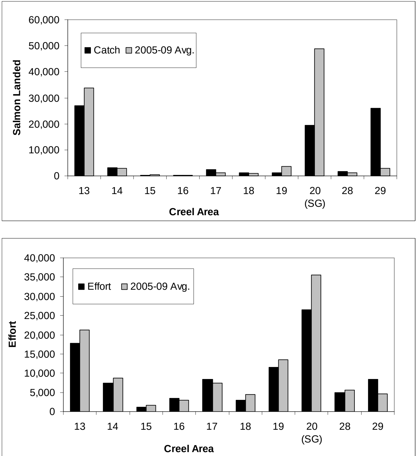
Figure 15. Total salmon landed and total fishing effort by creel area 1 in the SG during 2010 and the five-year average for 2005 to 2009.
