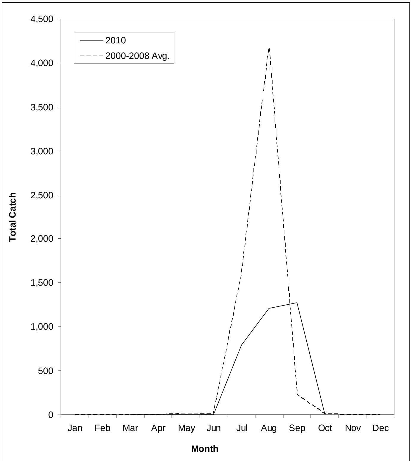
Figure 13. Monthly 1 estimated even year pink kept catches in the SG during 2010 and the five-cycle average for 2000 to 2008.
