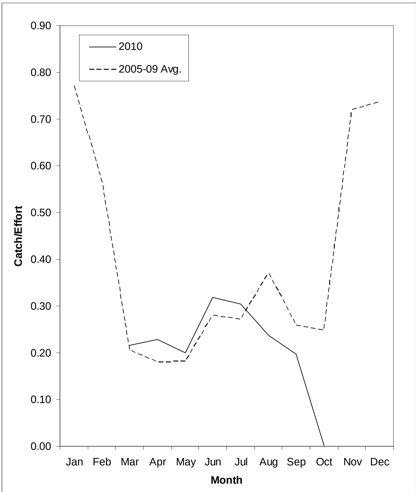
Figure 8. Monthly 1 chinook kept catch per boat trip in the SG during 2010 and the five-year average for 2005 to 2009.
