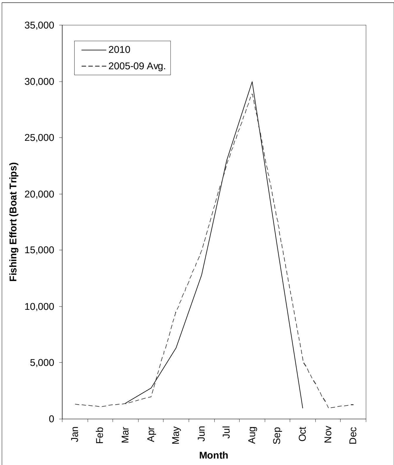
Figure 6. Monthly 1 fishing effort estimates (boat trips) in the SG during 2010 and the five-year average for 2005 to 2009.
