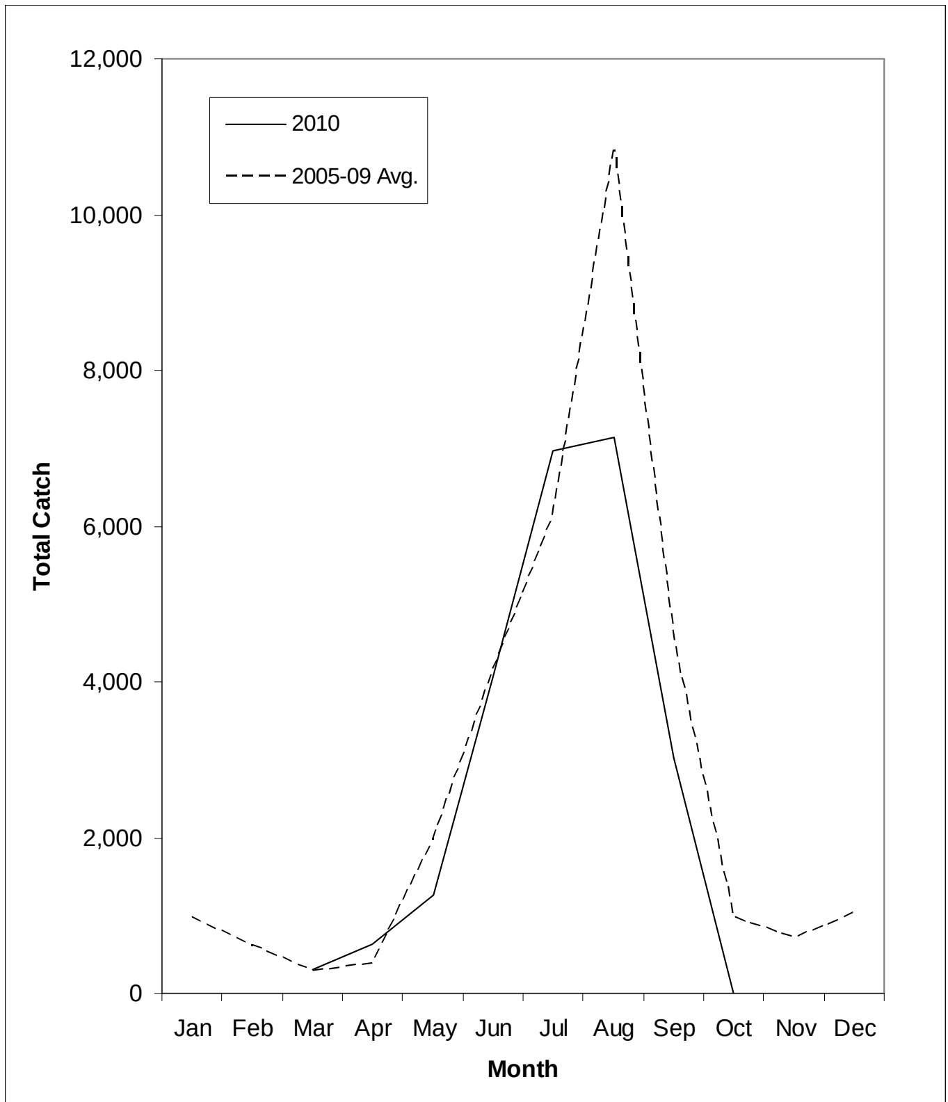
Figure 7. Monthly 1 chinook kept catches in the SG during 2010 and the five-year average for 2005 to 2009.
