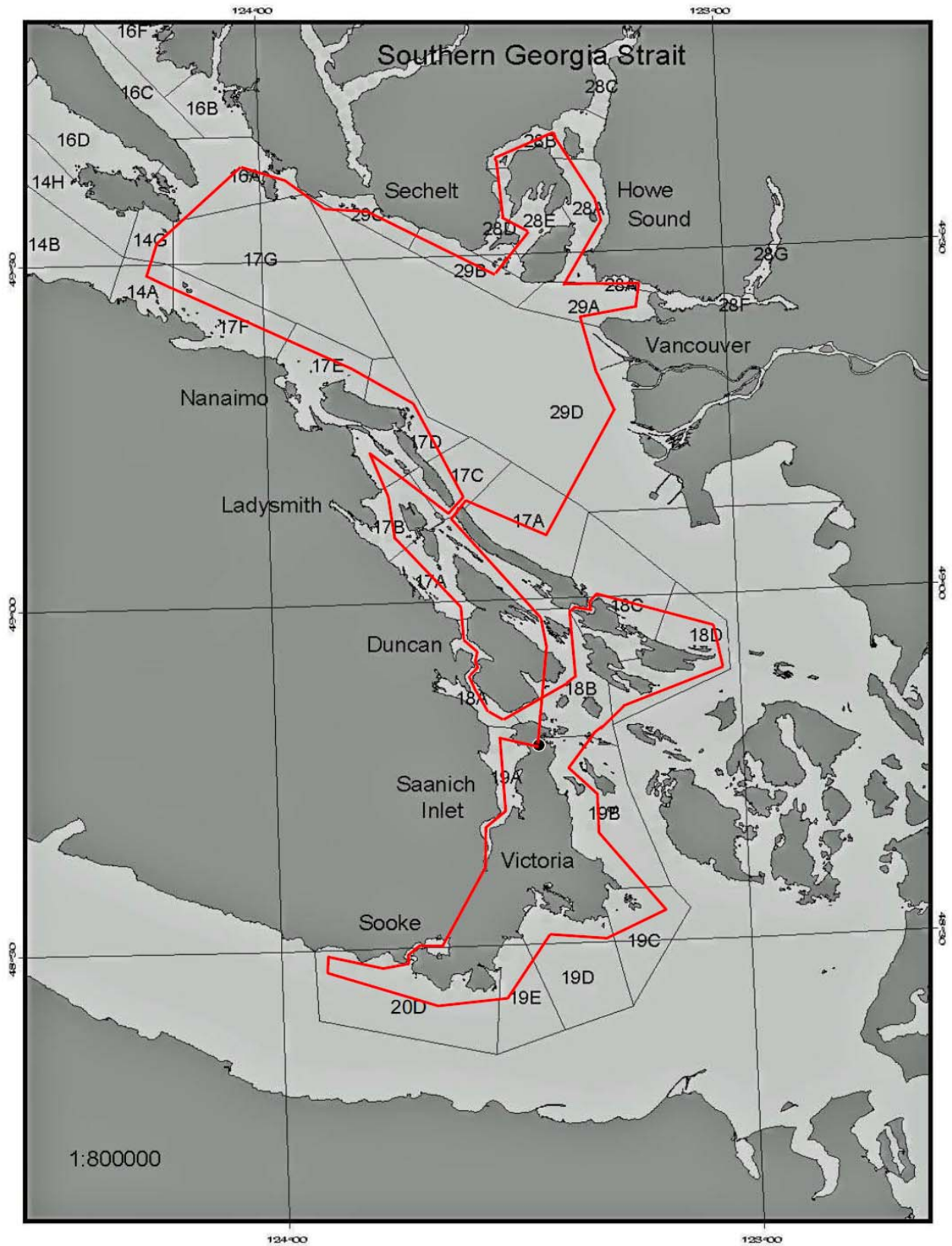
Figure 3b. SG creel survey southern aerial survey route, 2010.
