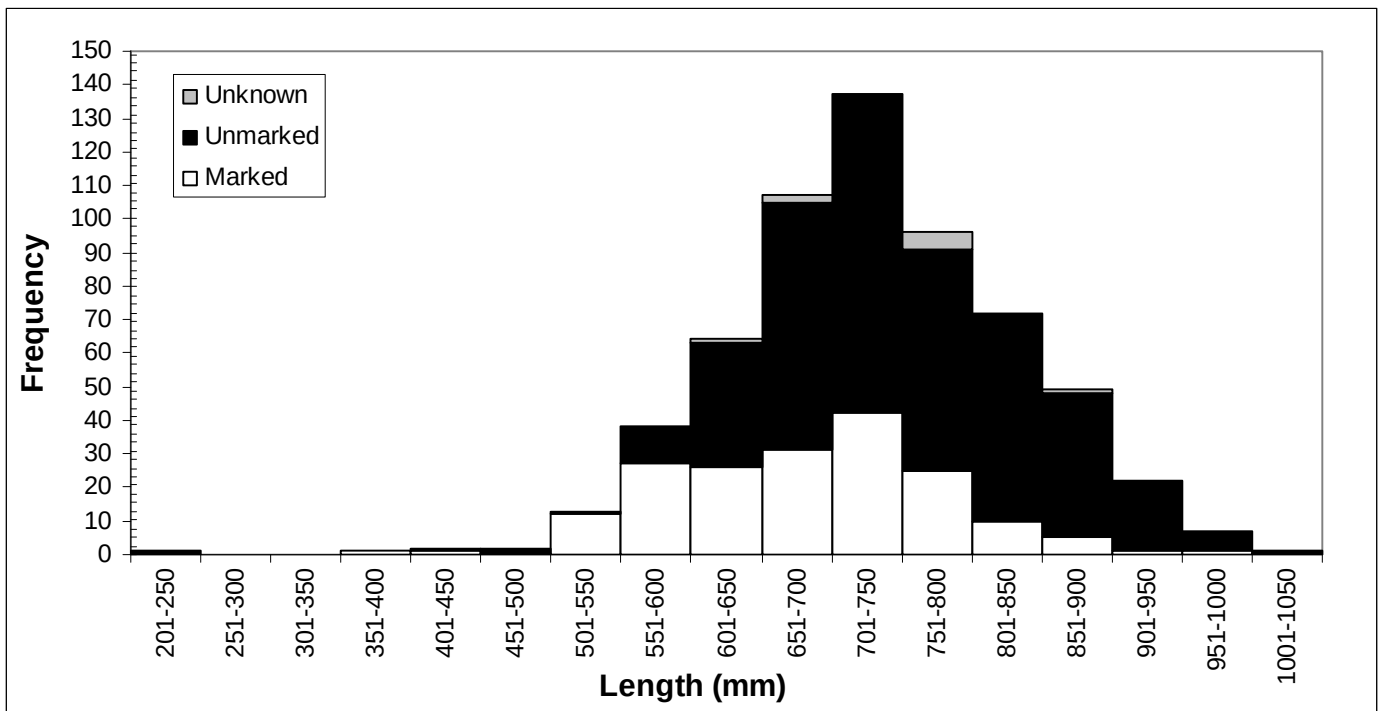
Figure 19. Length frequency distribution of chinook salmon sampled in the SG creel survey, 2010.
