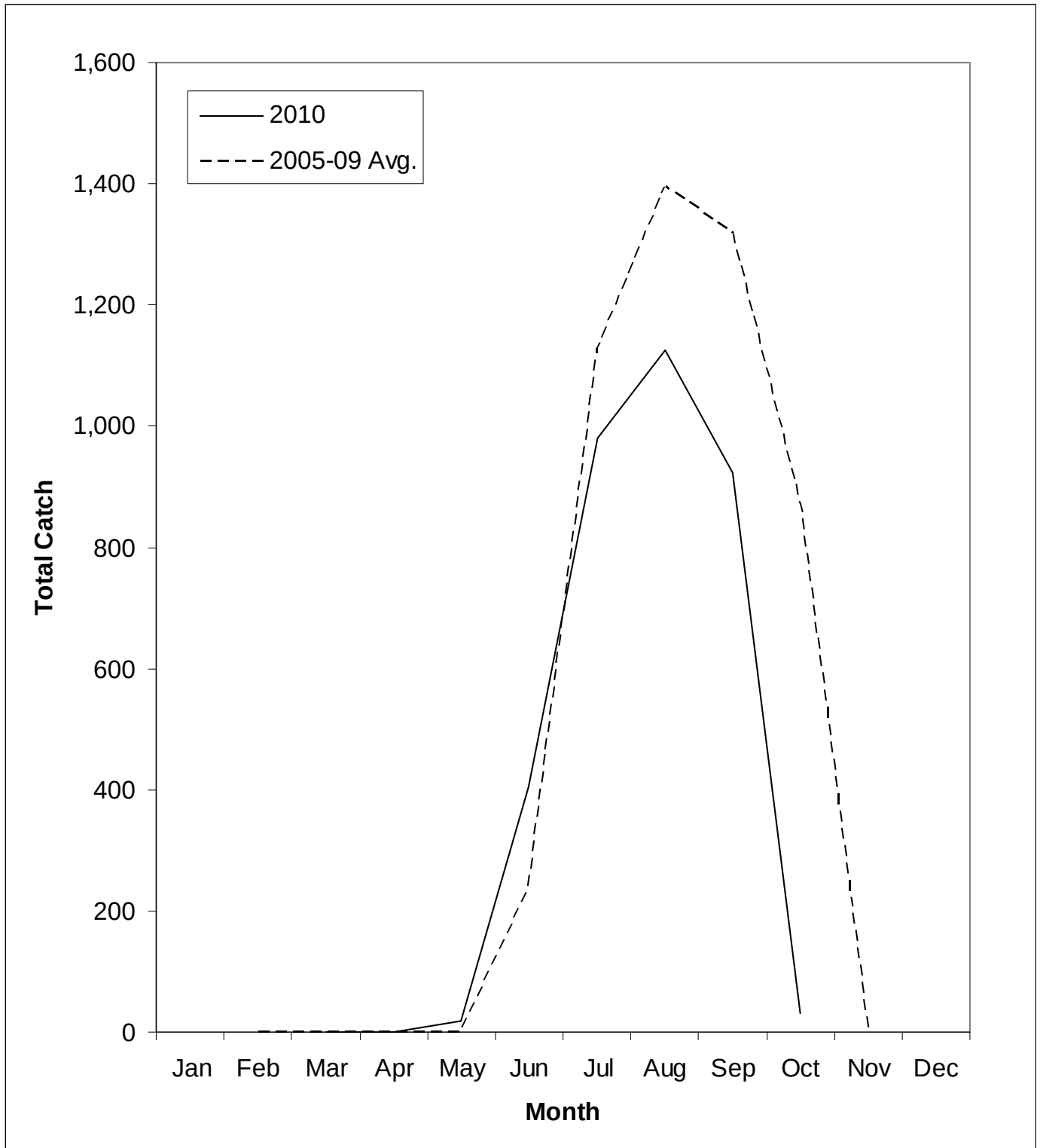
Figure 10. Monthly 1 estimated coho kept catches in the SG during 2010 and the five-year average for 2005 to 2009.
