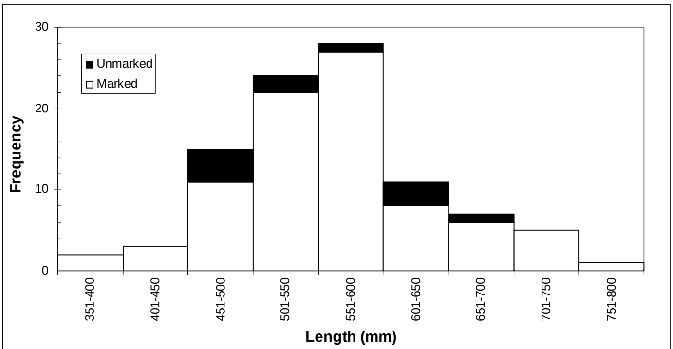
Figure 20. Length frequency distribution of coho salmon sampled in the SG creel survey, 2010.
