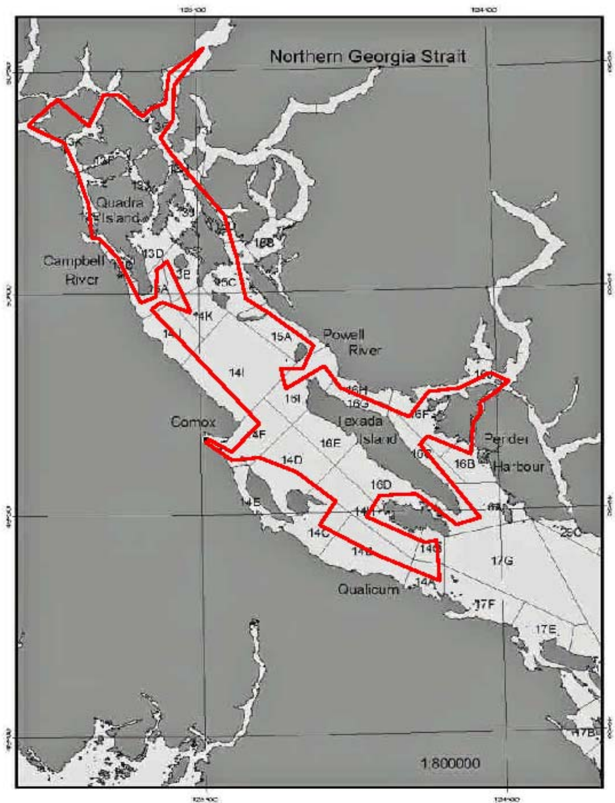
Figure 3a. SG creel survey northern aerial survey route, 2010.
