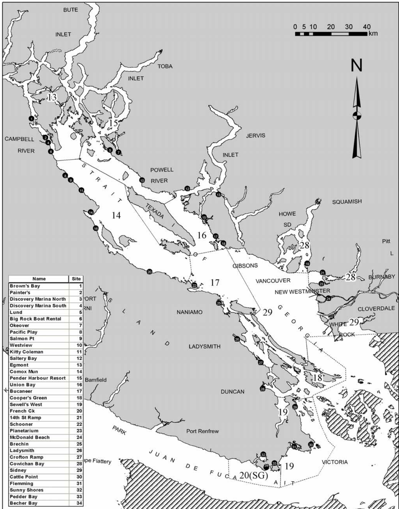
Figure 1. SG creel survey study area and landing site locations, 2010.
