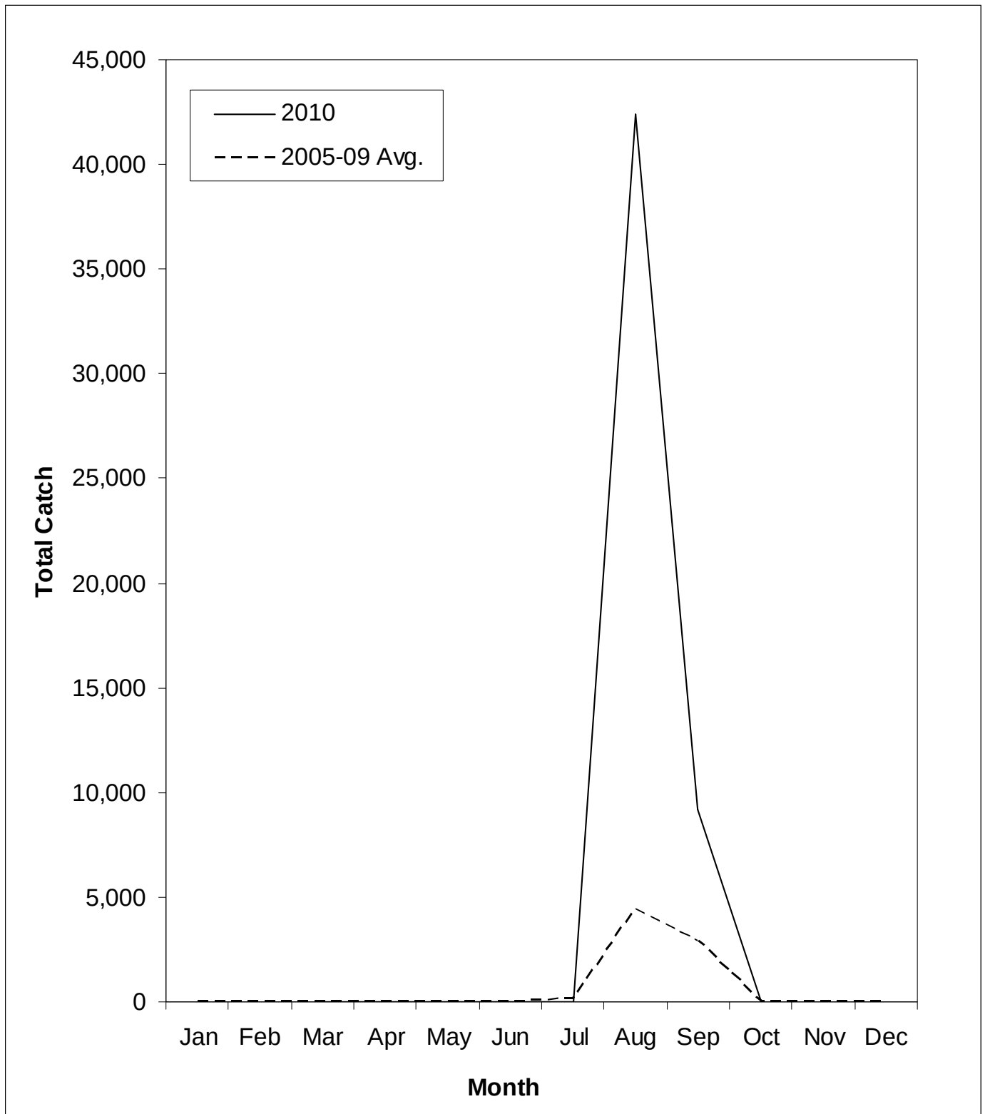
Figure 12. Monthly 1 estimated sockeye kept catches in the SG during 2010 and the five-year average for 2005 to 2009.
