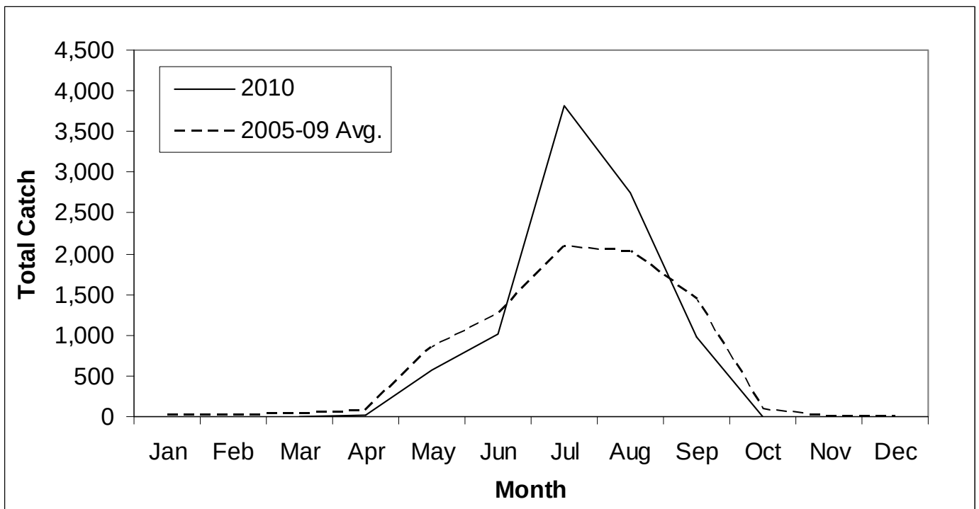
Figure 16. Monthly 1 estimated rockfish (all species) kept catches in the SG during 2010 and the five-year average for 2005 to 2009.
