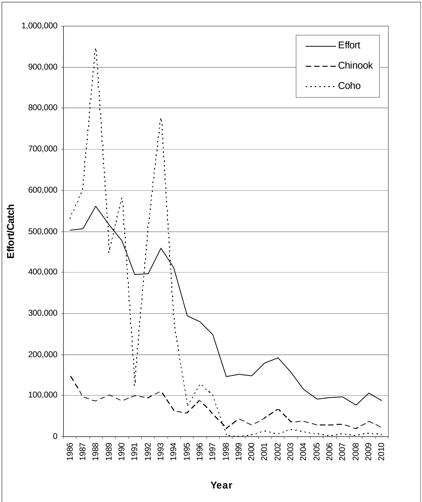
Figure 5. Effort (boat trips) statistics and estimated kept catches 1 of chinook and coho salmon in the SG, 1986 to 2010.
