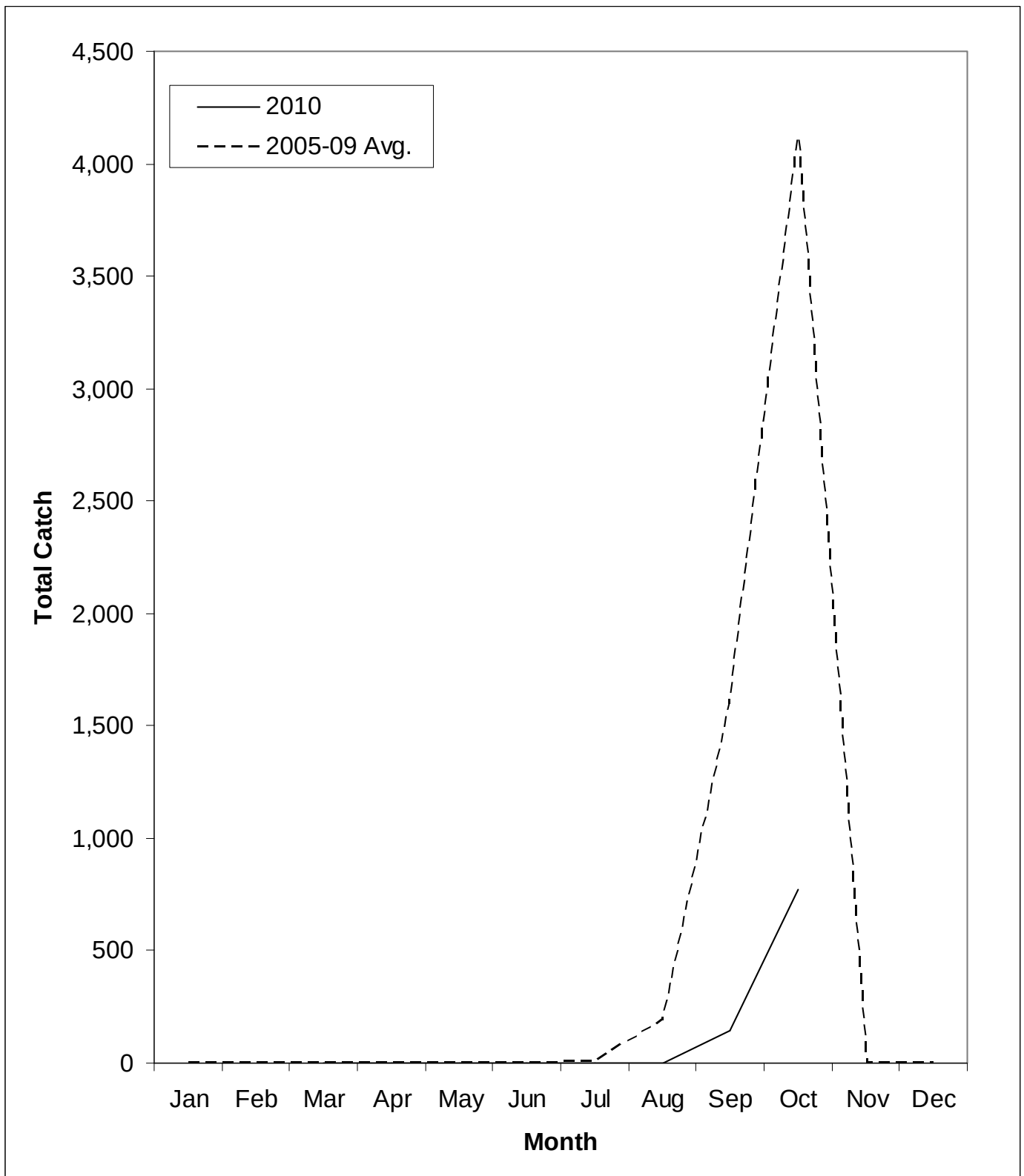
Figure 14. Monthly 1 estimated chum kept catches in the SG during 2010 and the five-year average for 2005 to 2009.
