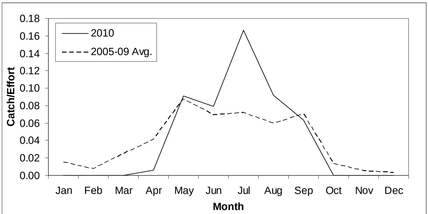
Figure 17. Monthly 1 estimated rockfish (all species) kept catch per boat trip in the SG during 2010 and the five-year average for 2005 to 2009.
