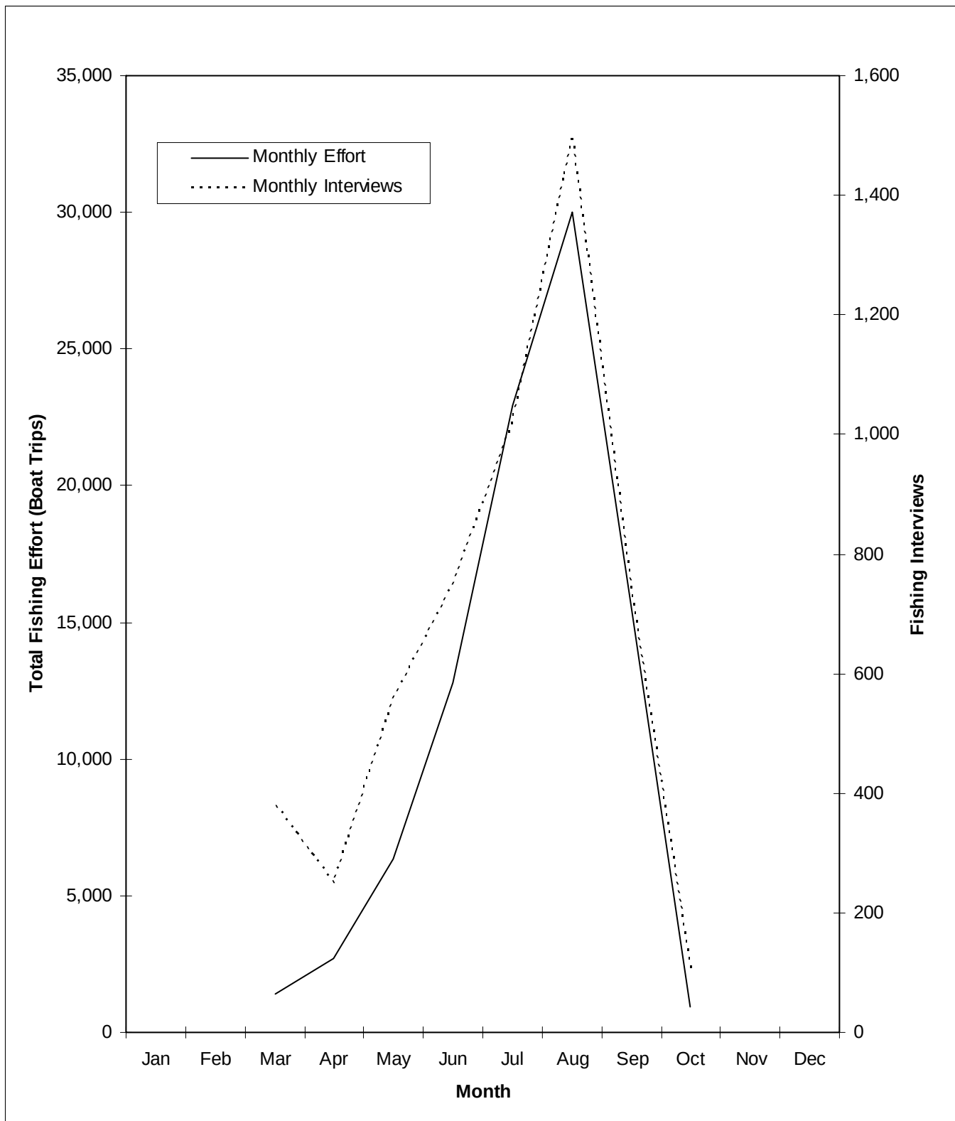
Figure 4. Comparison of monthly 1 total fishing effort in the SG and monthly 1 interviews in the SG creel survey, 2010.
