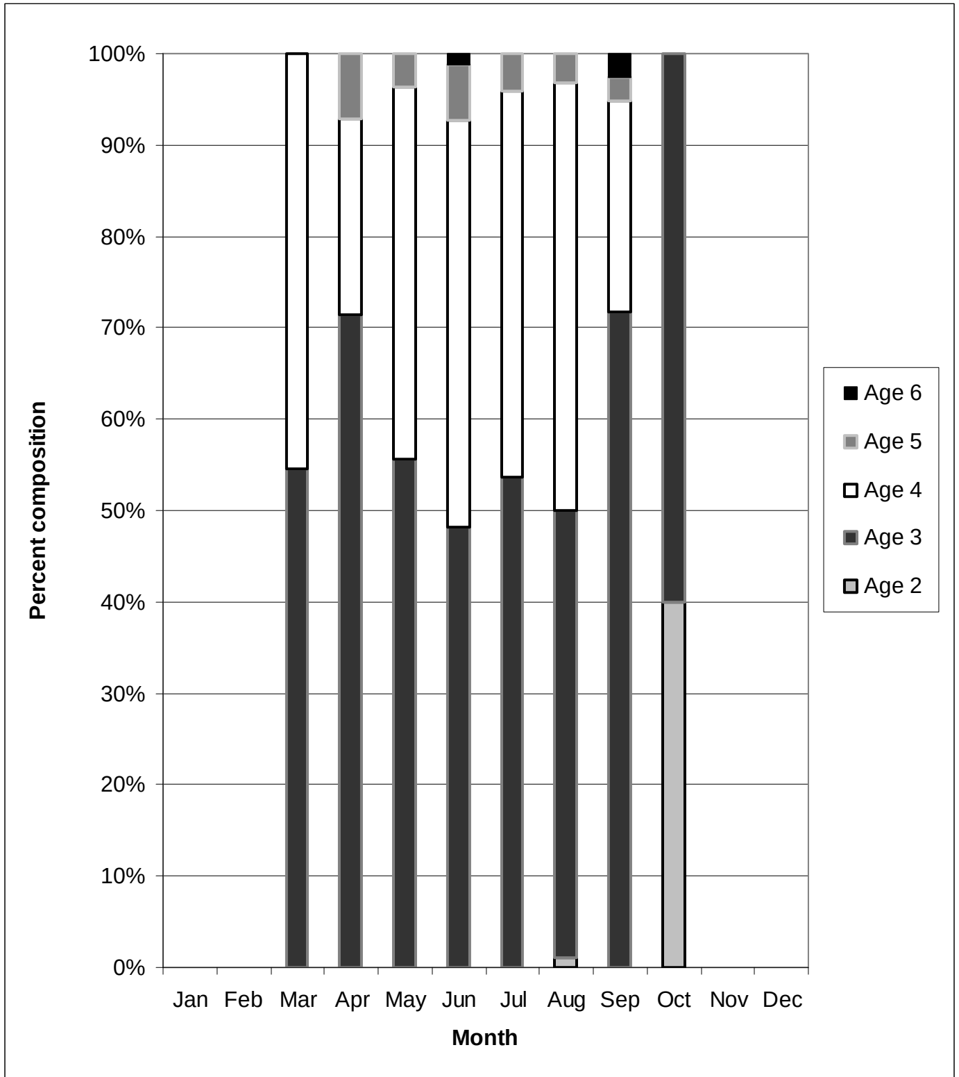
Figure 18. Monthly 1 percent age composition of chinook salmon sampled in the SG creel survey, 2010.
