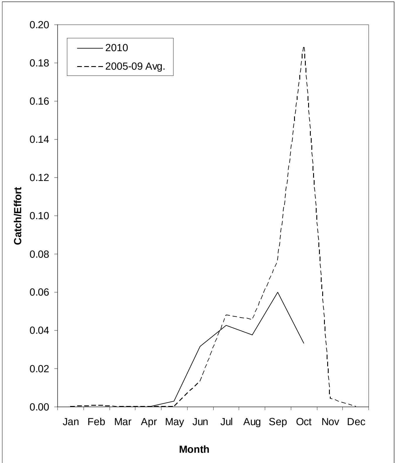
Figure 11. Monthly 1 estimated coho kept catch per boat trip in the SG during 2010 and the five-year average for 2005 to 2009.
