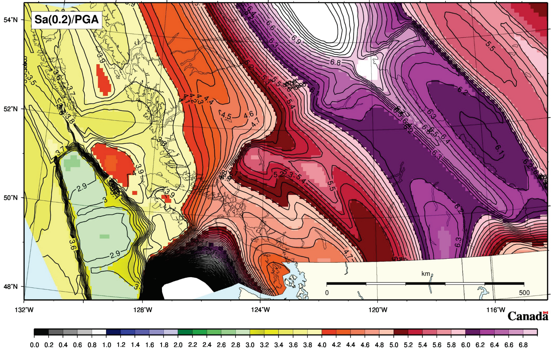
Figure A3-9. Ratio of 2%/50 year Sa(0.2) /10%/50 year PGA for southwestern Canada
