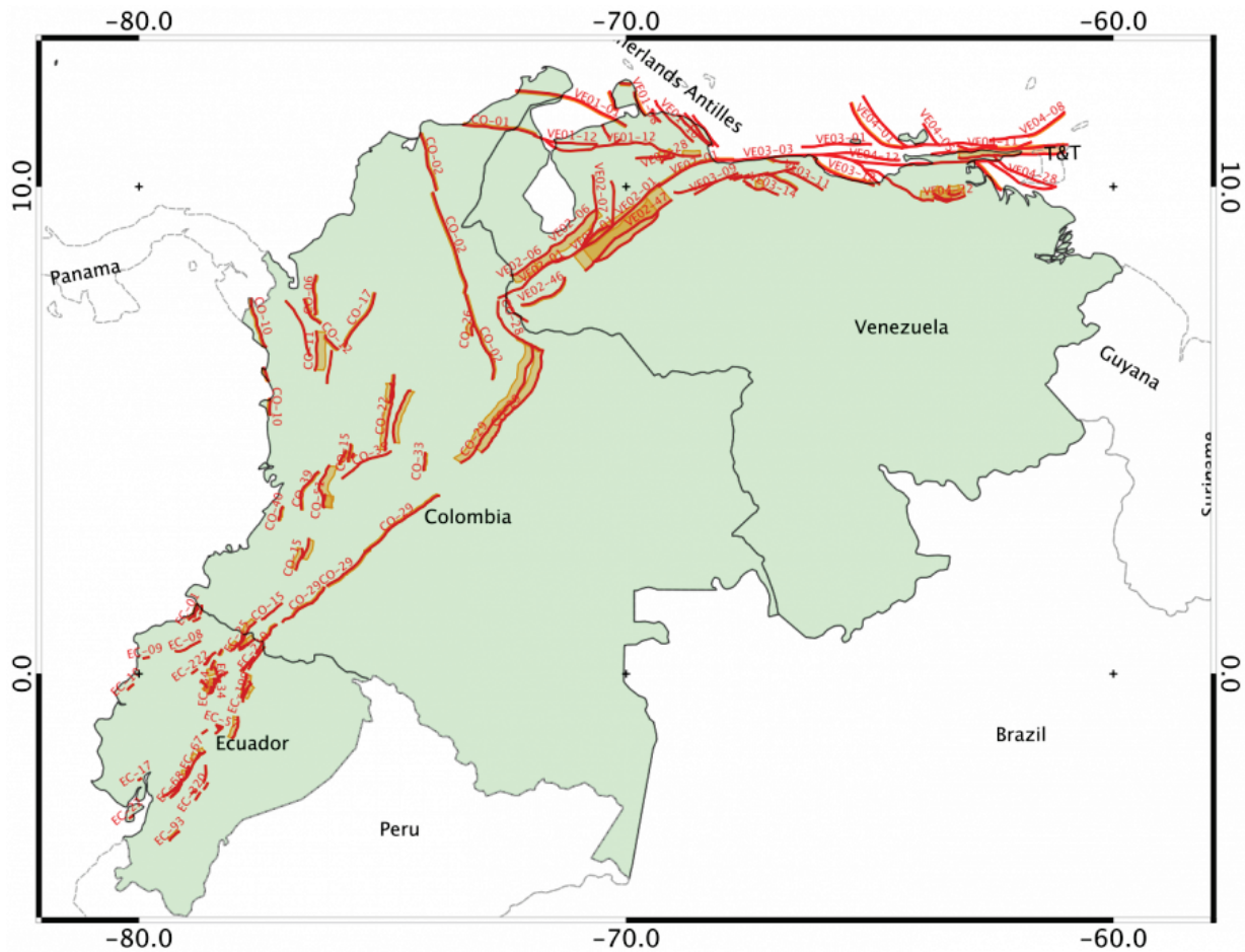
Figure 3. Map of northwestern South America showing the active faults considered in the model. Downloaded from https://sara.openquake.org/hazard_rt2 on 2019-05-03.
