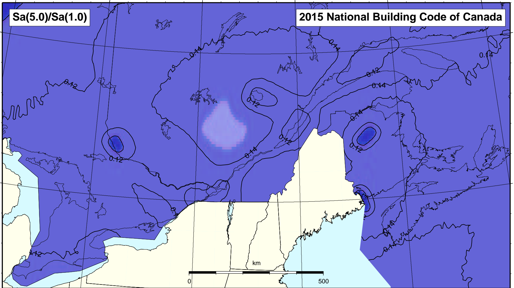
80°W 75°W 70°W 65°W Ratio 2%/50 Sa(5.0)/2%/50 Sa(1.0) for Canada
