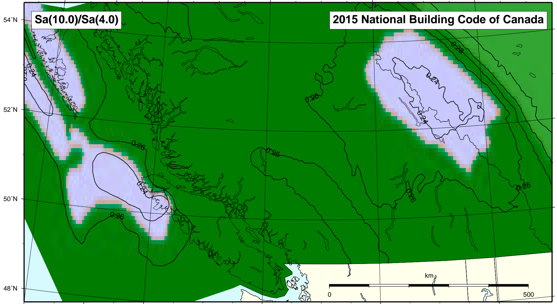
Ratio 2%/50 Sa(10.0)/2%/50 Sa(4.0) (via interpolation) for Canada
