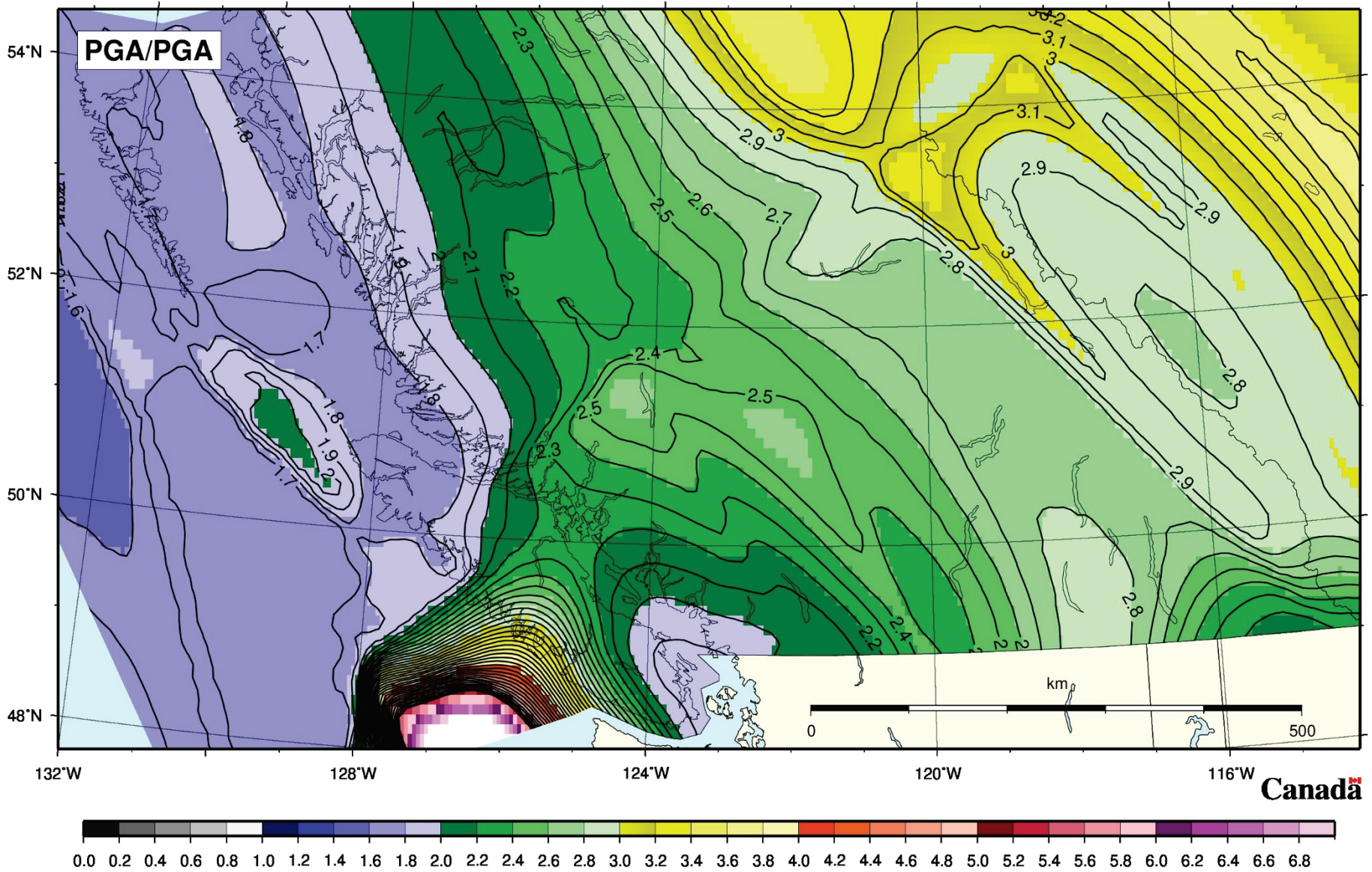
Figure A3-8. Ratio of 2%/50 year PGA /10%/50 year PGA for southwestern Canada
