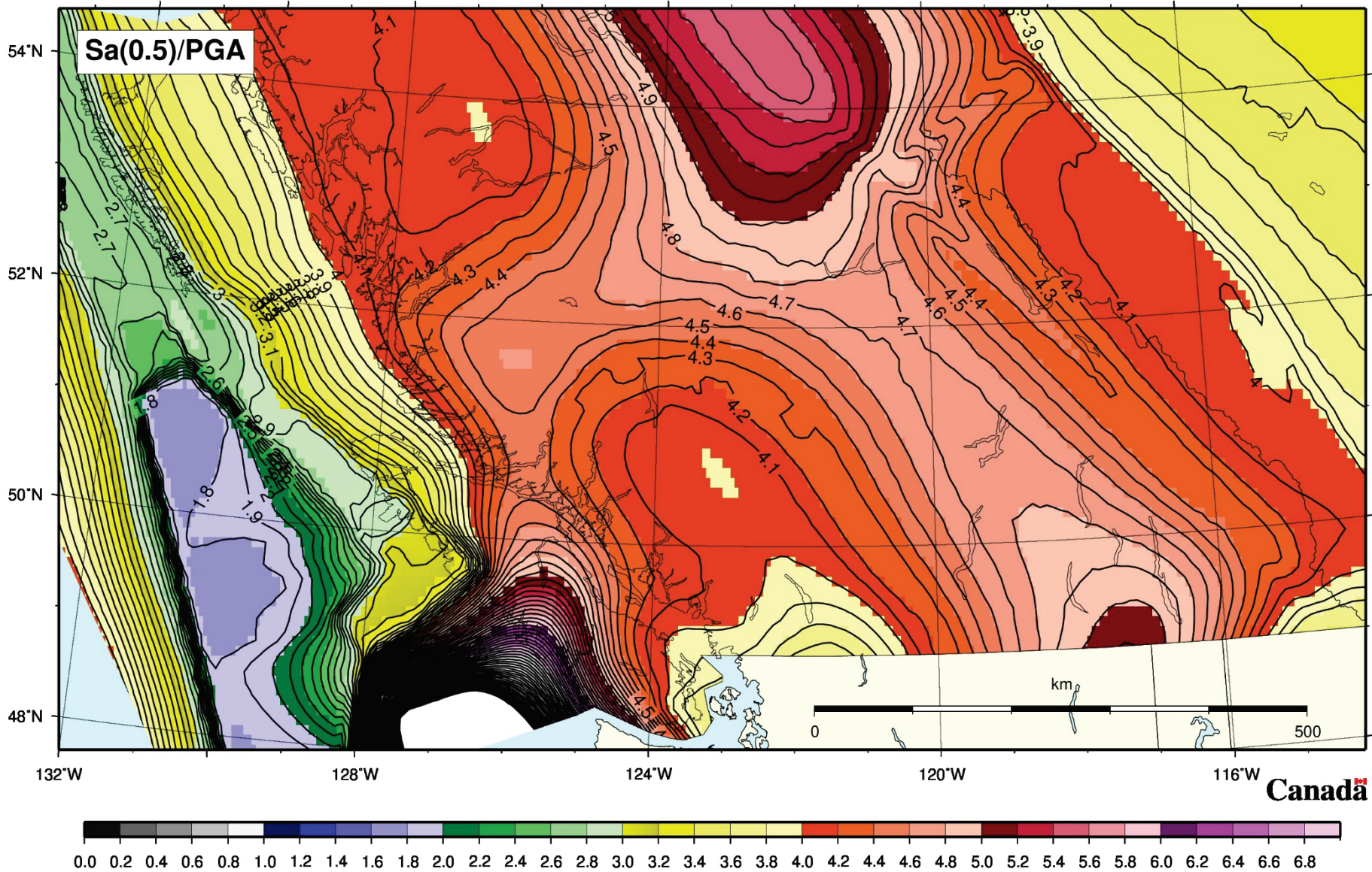
Figure A3-10. Ratio of 2%/50 year Sa(0.5) /10%/50 year PGA for southwestern Canada
