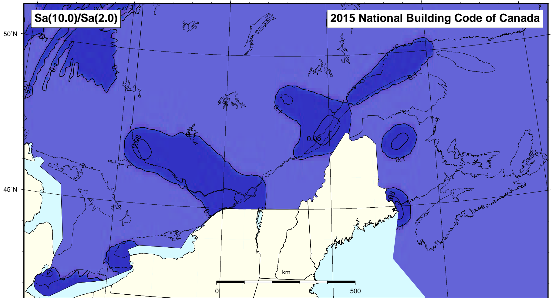
Ratio 2%/50 Sa(10.0)/2%/50 Sa(2.0) for Canada
