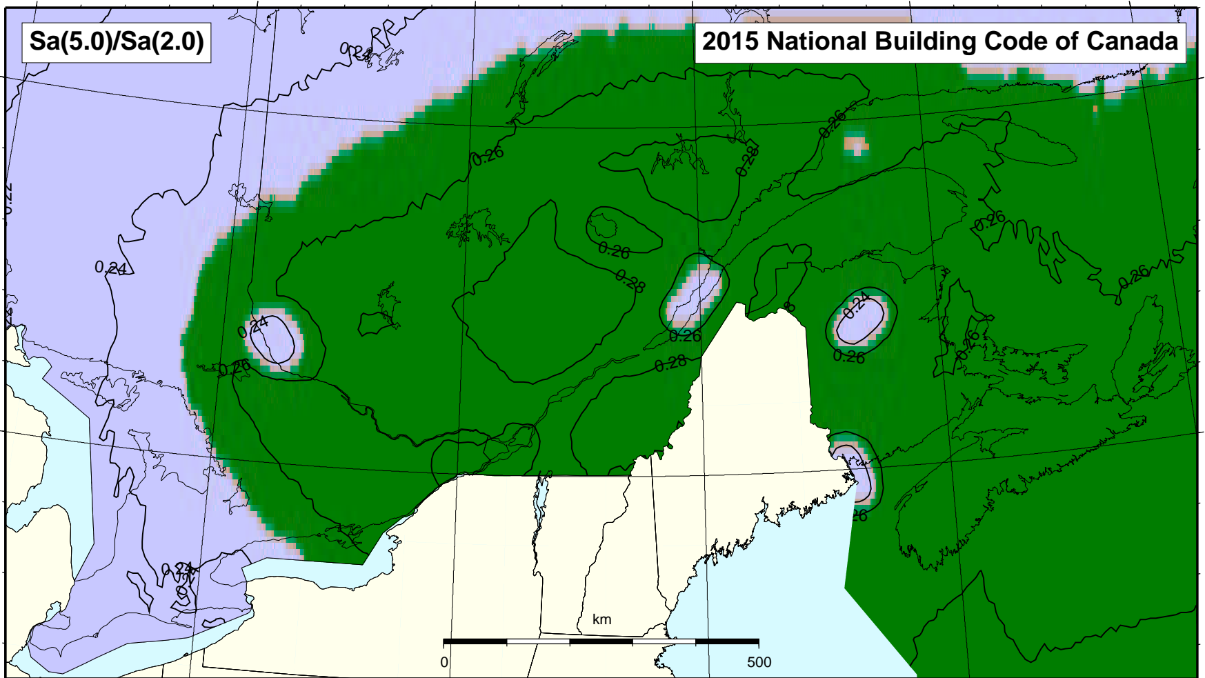
80°W 75°W 70°W 65°W Ratio 2%/50 S_a(5.0)/2\%/50 S_a(2.0) for Canada
