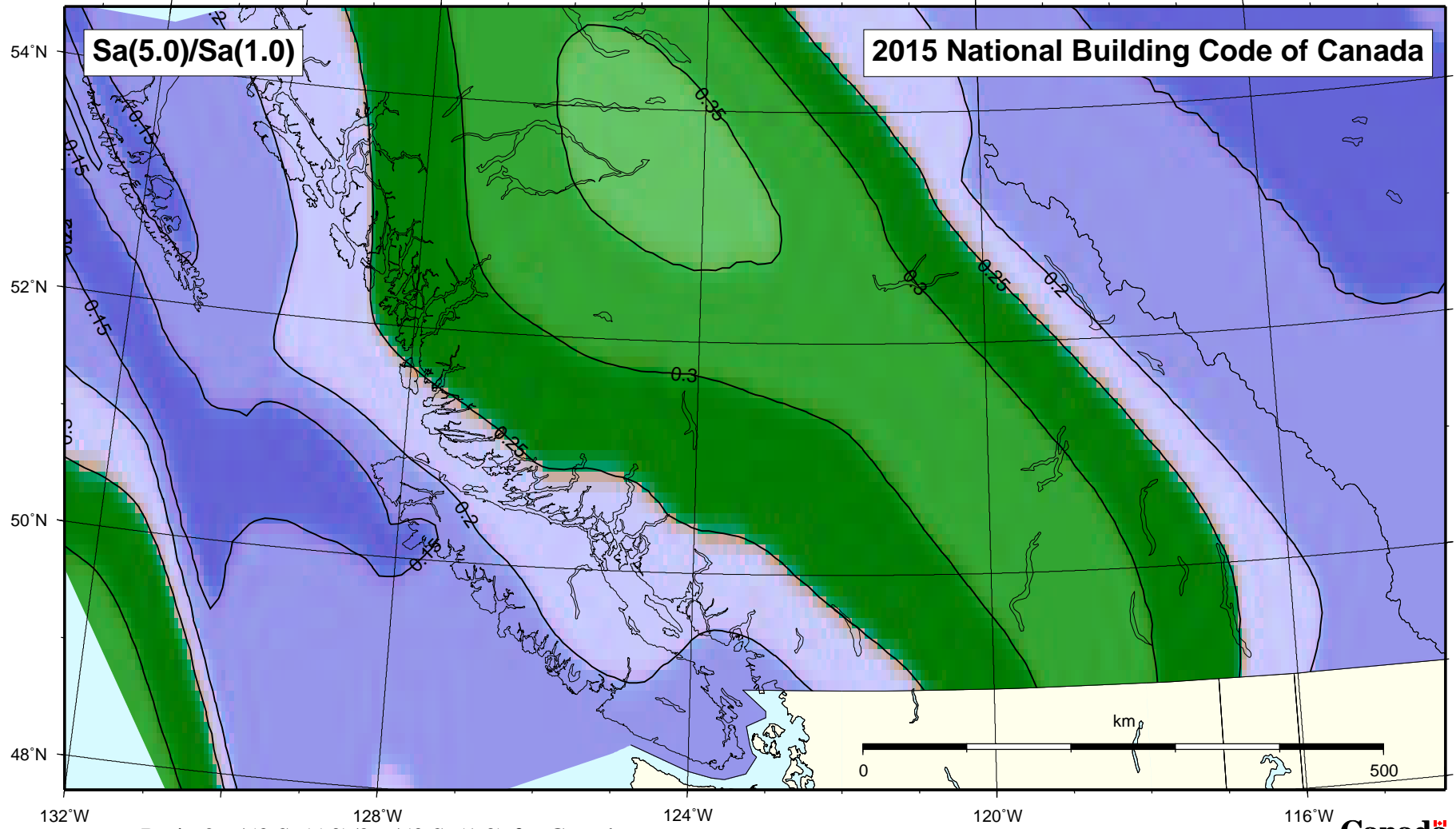
Ratio 2%/50 Sa(5.0)/2%/50 Sa(1.0) for Canada
