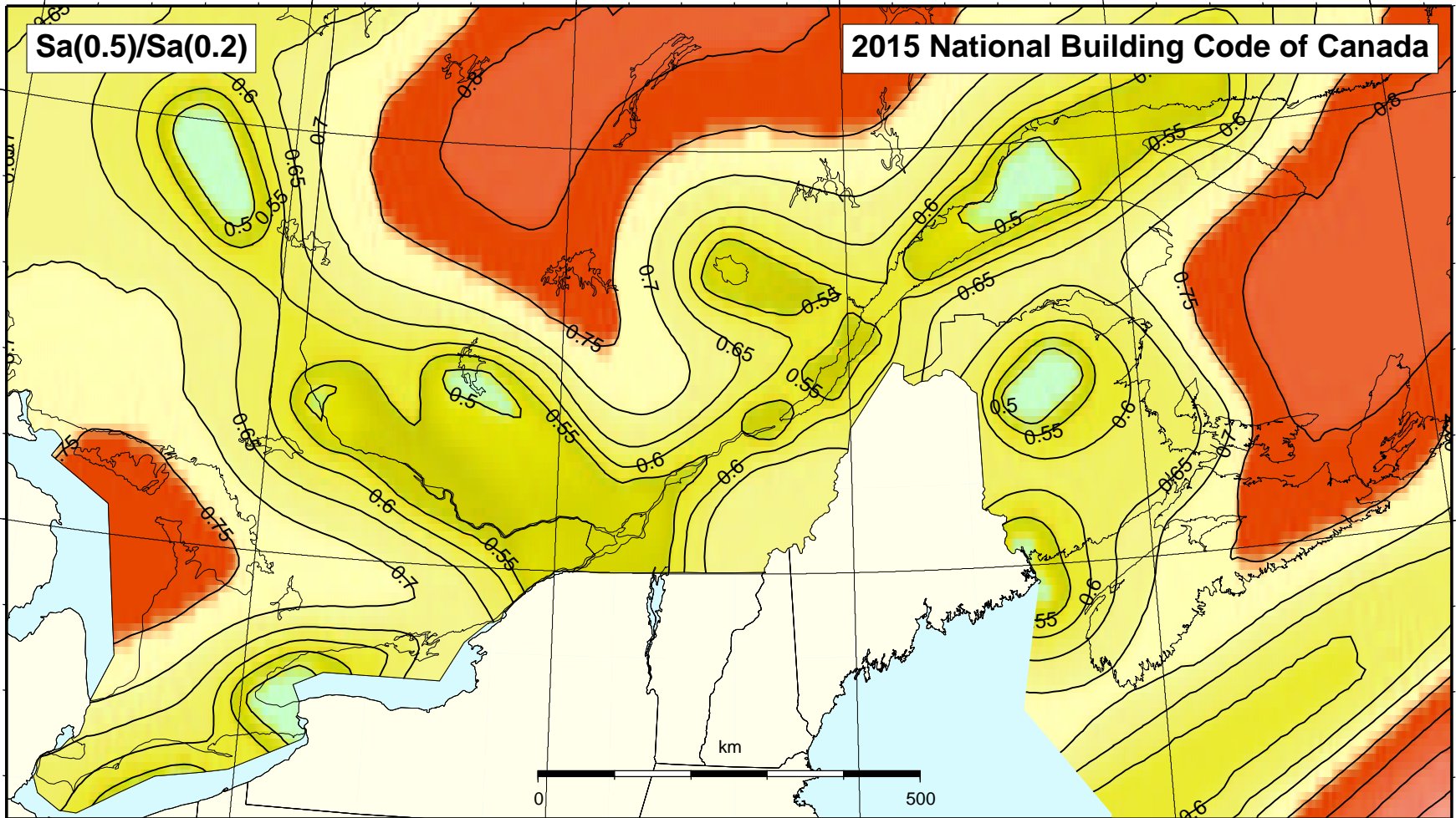
80°W 75°W 70°W 65°W Ratio 2%/50 Sa(0.5)/2%/50 Sa(0.2) for Canada
