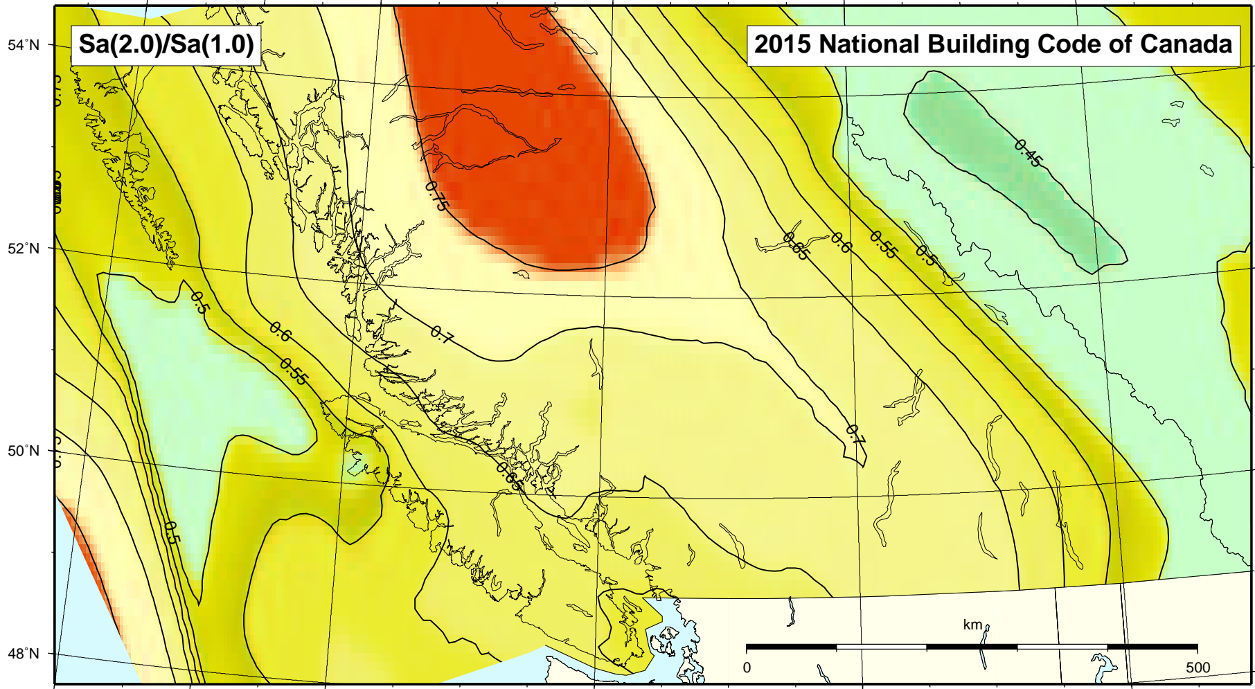
Ratio 2%/50 Sa(2.0)/2%/50 Sa(1.0) for Canada
