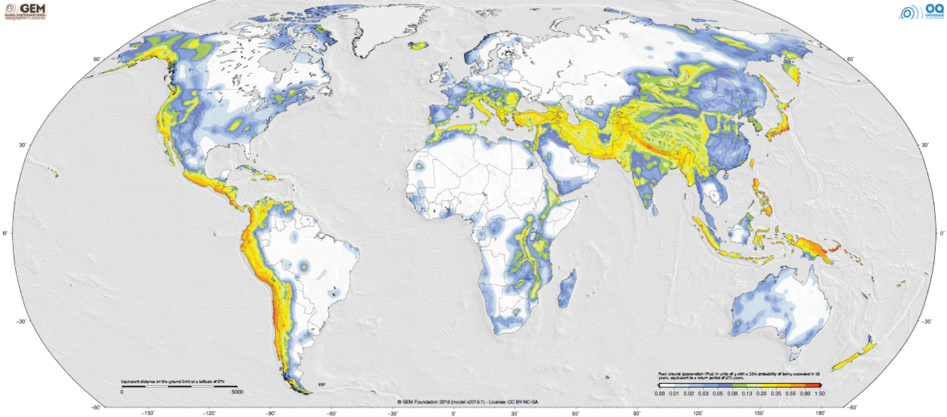
Figure 4. The GEM Global Seismic Hazard Map, v. 2018.1. This map shows PGA with a 10% probability of being exceeded in 50 years, on the reference soil conditions ( V_{s30}=760\text{-}800\text{m/s} ). This is a low-resolution version of a 52 MB file at https://hazard.openquake.org/gem/images/home/gem_global_seismic_hazard_map_v2018.1.pdf accessed on 2019-05-01.
