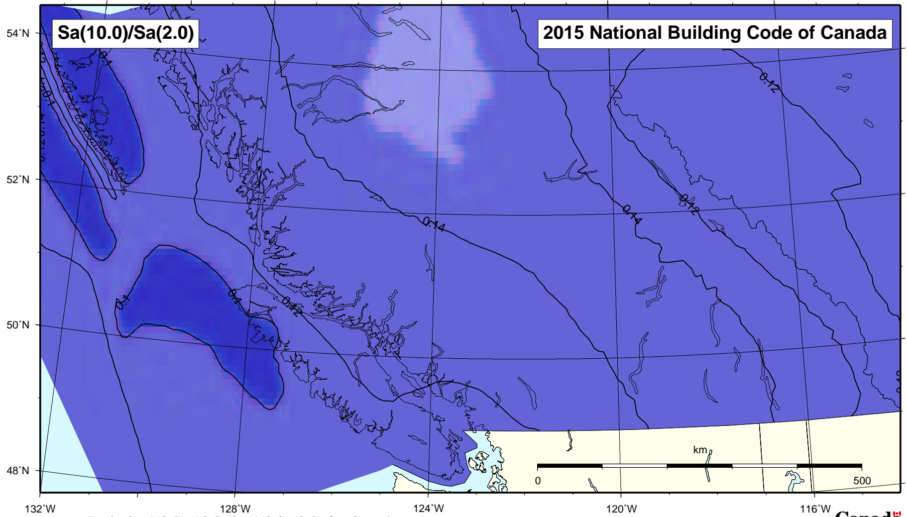
Ratio 2%/50 Sa(10.0)/2%/50 Sa(2.0) for Canada
