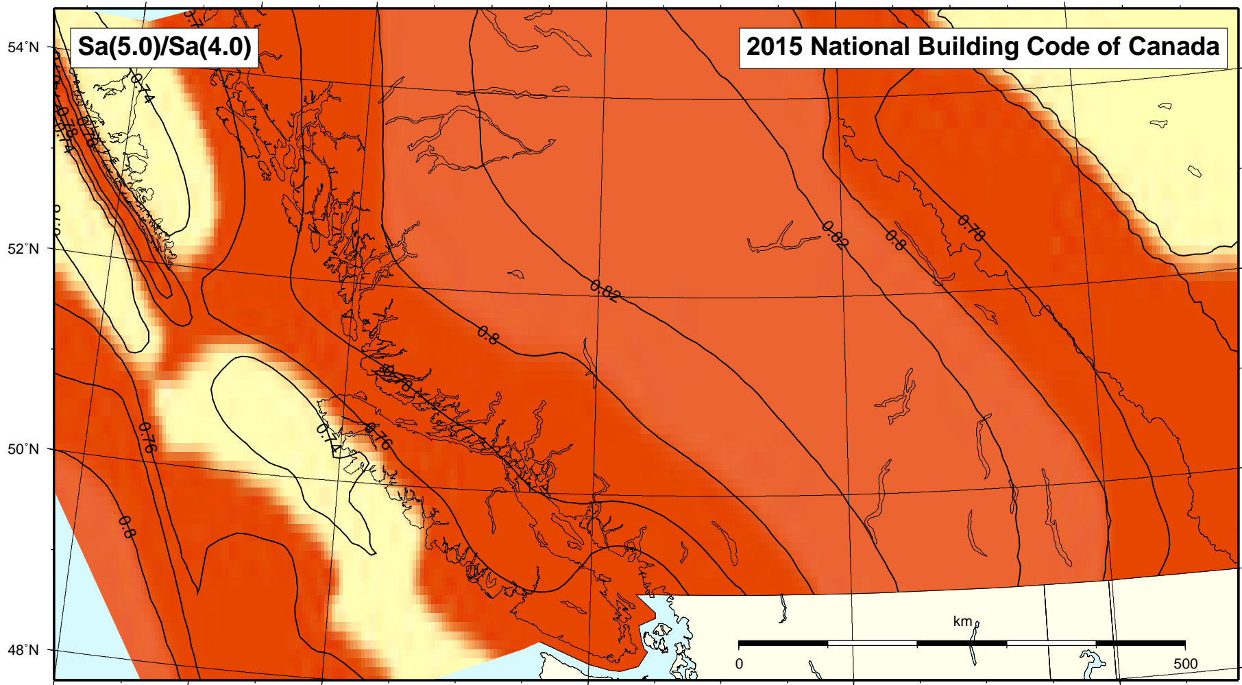
Ratio 2%/50 Sa(5.0)/2%/50 Sa(4.0) (via interpolation) for Canada
