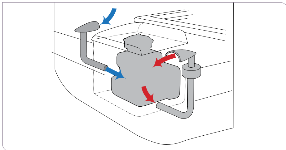
Typical propane installation with ventilation
