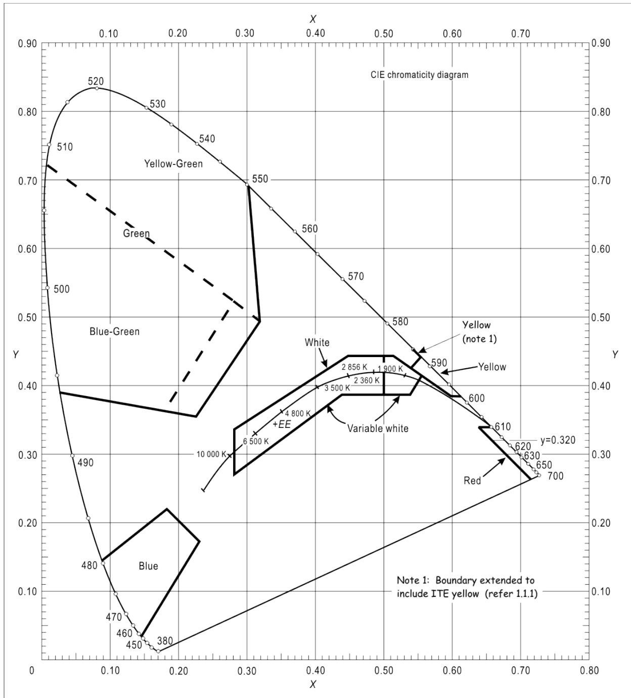
Figure A-1(a): Colours for aeronautical ground light (filament type lamps)
