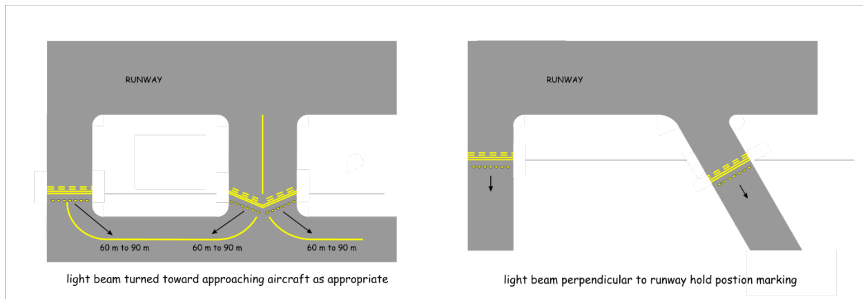
Figure 5-57: Inset runway guard light orientation
