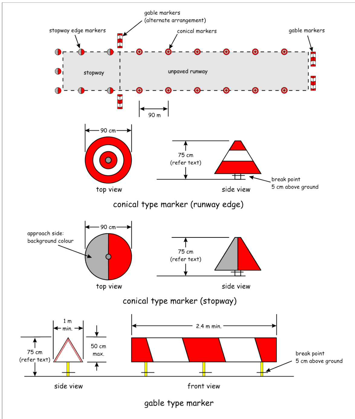
Figure 5-71(a): Example of conical and gable markers
