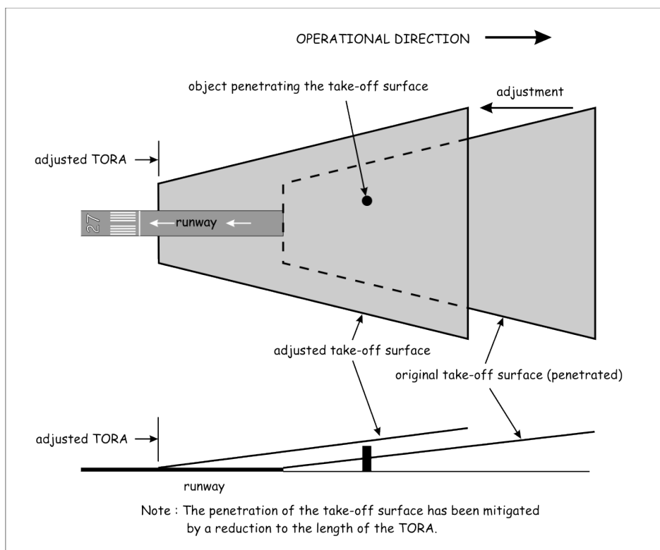
Figure 4-4: Mitigation for penetration of take-off surface
