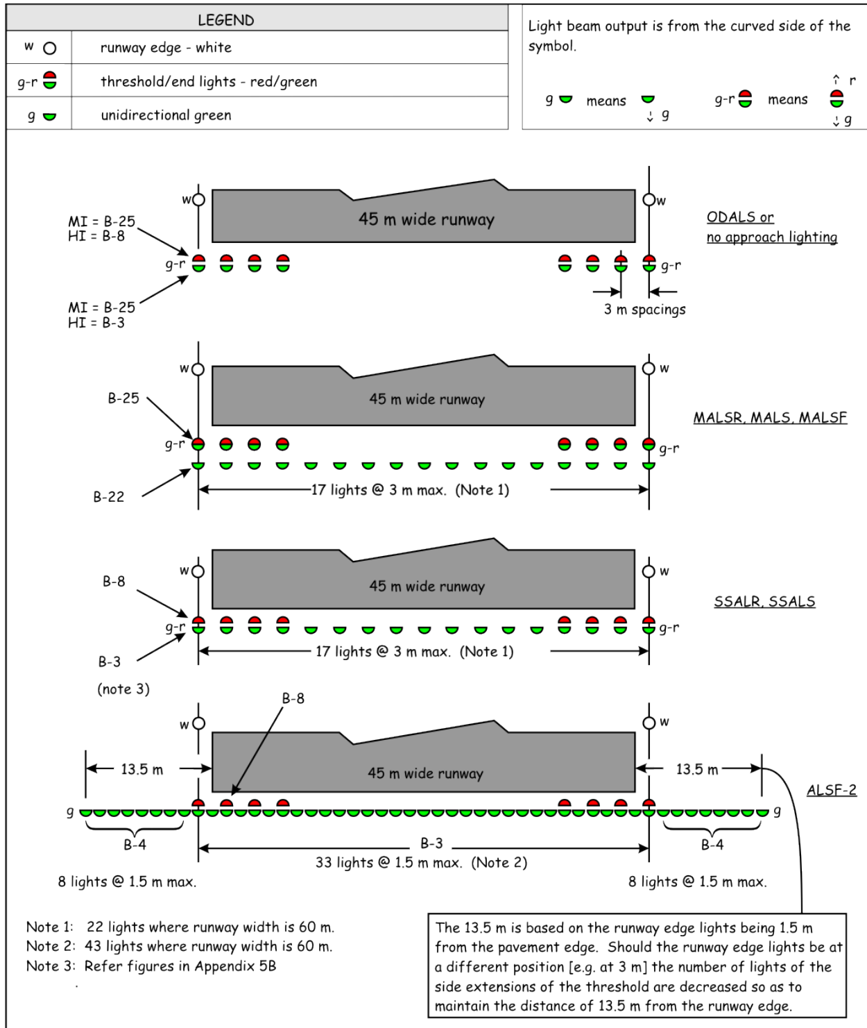
Figure 5-33: Approach threshold, runway threshold and runway end light configurations
