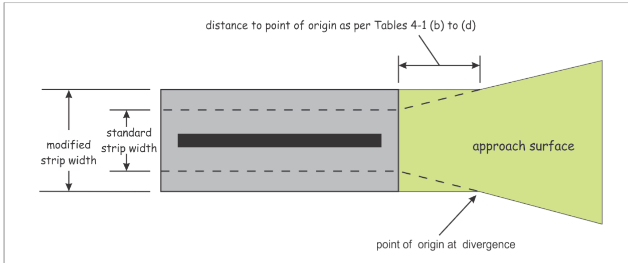
Figure 4-2(a): Modified obstacle limitation surface
