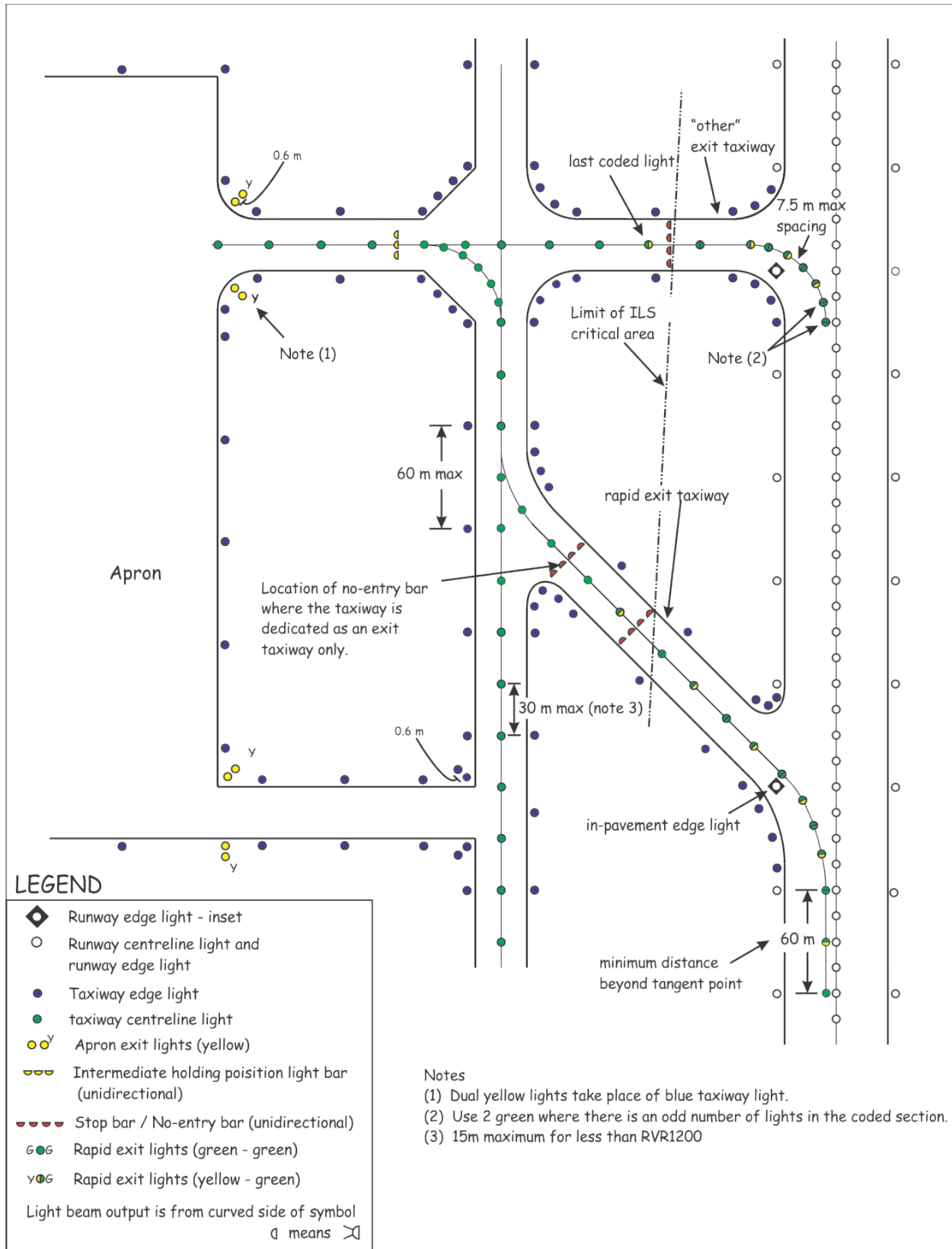
Figure 5-49: Taxiway lighting
