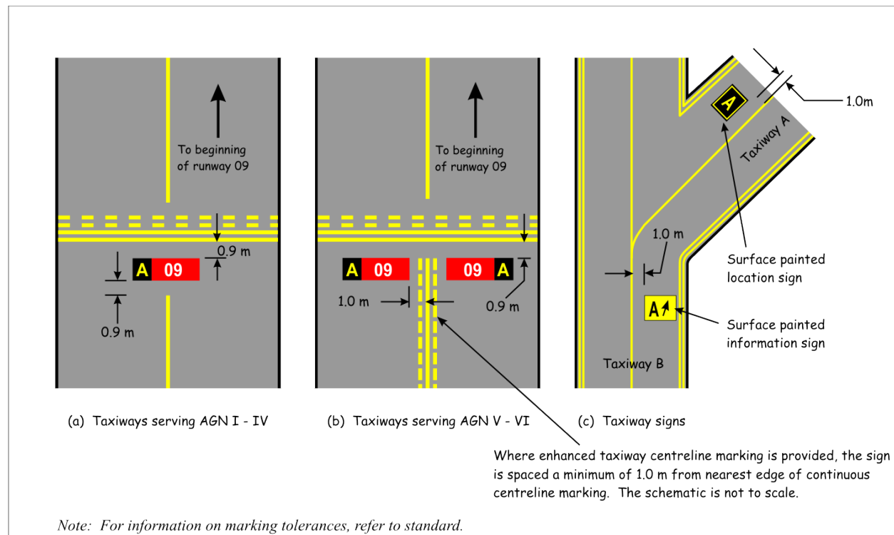
Figure 5-18: Painted sign markings
