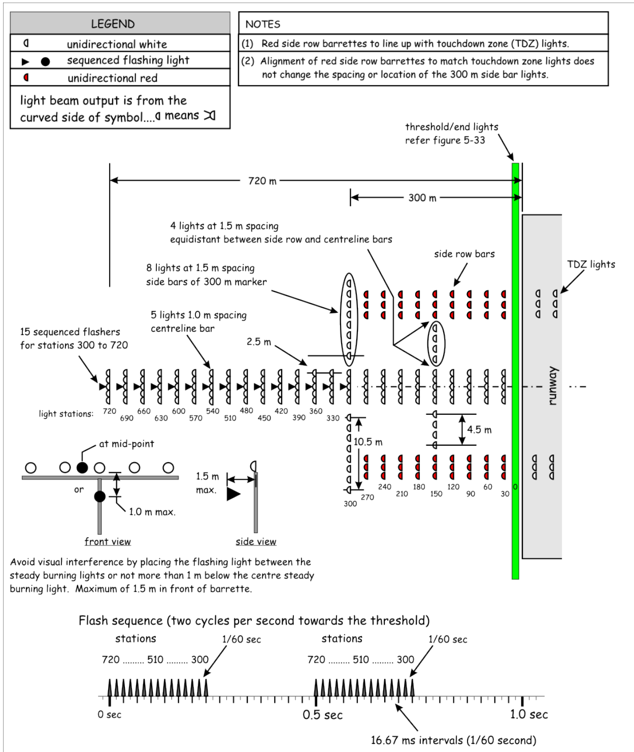
Figure 5-31: ALSF-2 configuration
