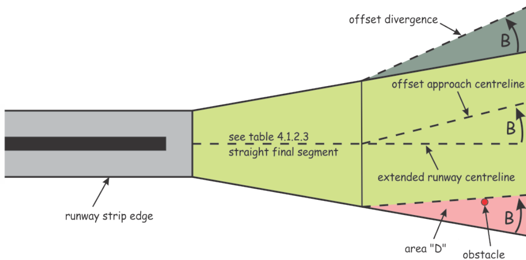
Figure 4-3(b): Offset approach surface (Non-instrument runways)
