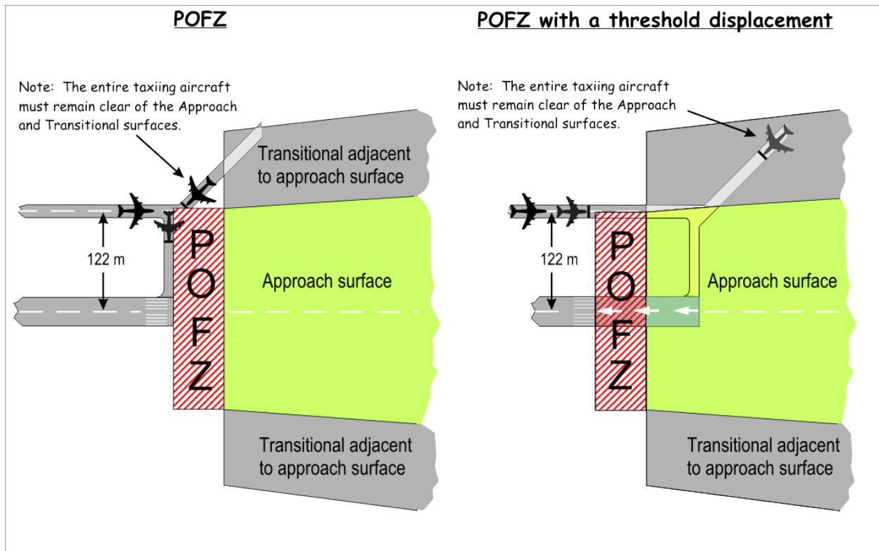
Figure 4-7: Precision Obstacle Free Zone
