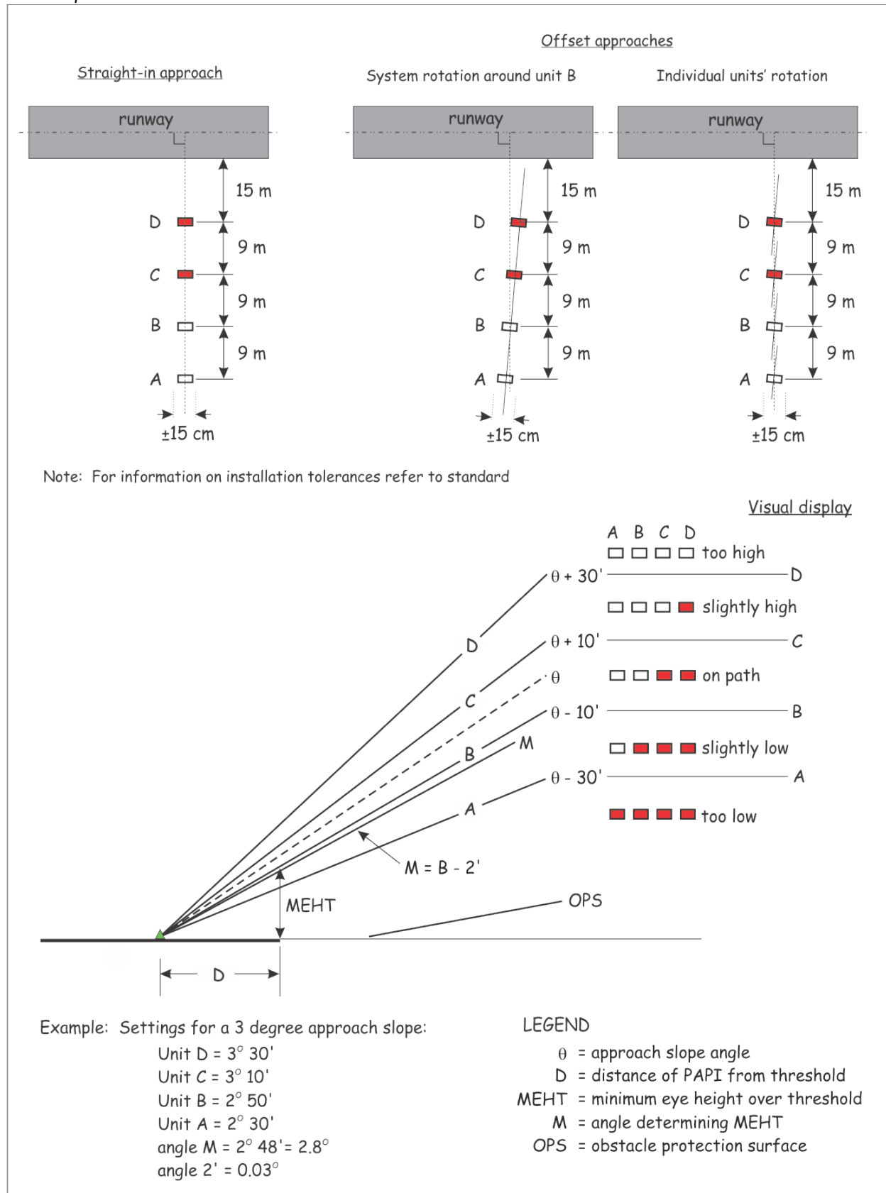
Figure 5-41: PAPI general arrangement
