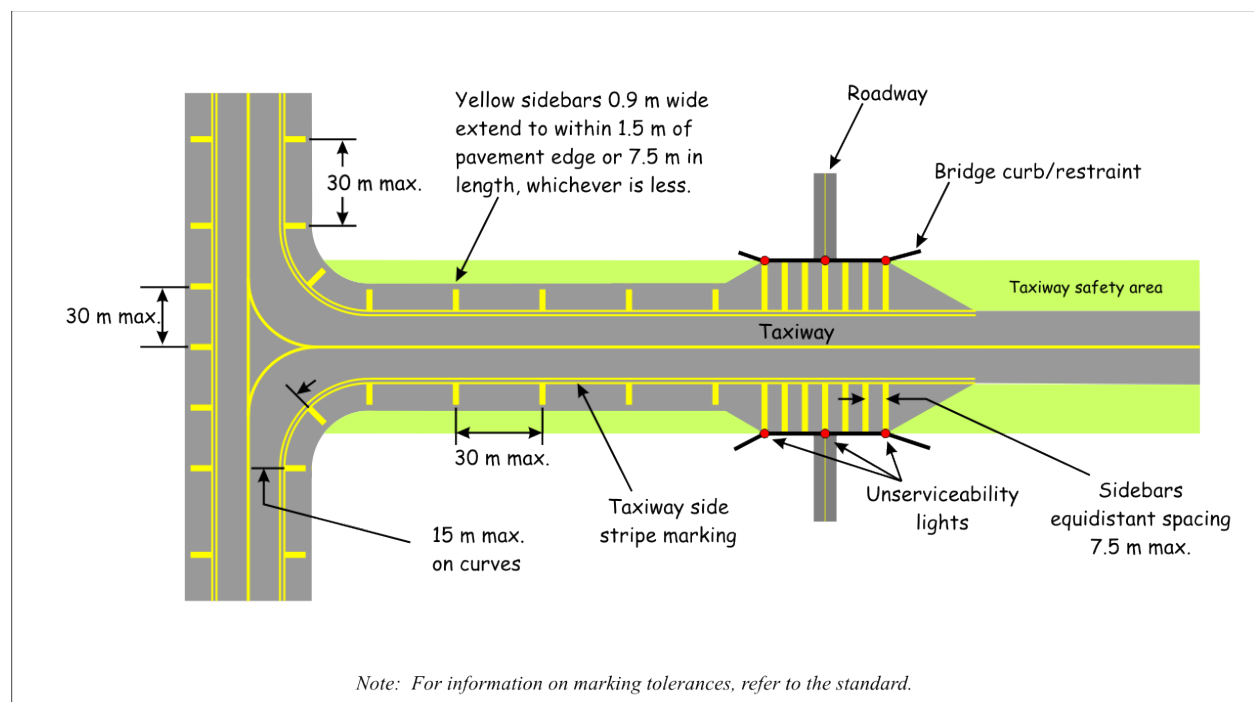
Figure 5-11: Taxiway safety area marking
