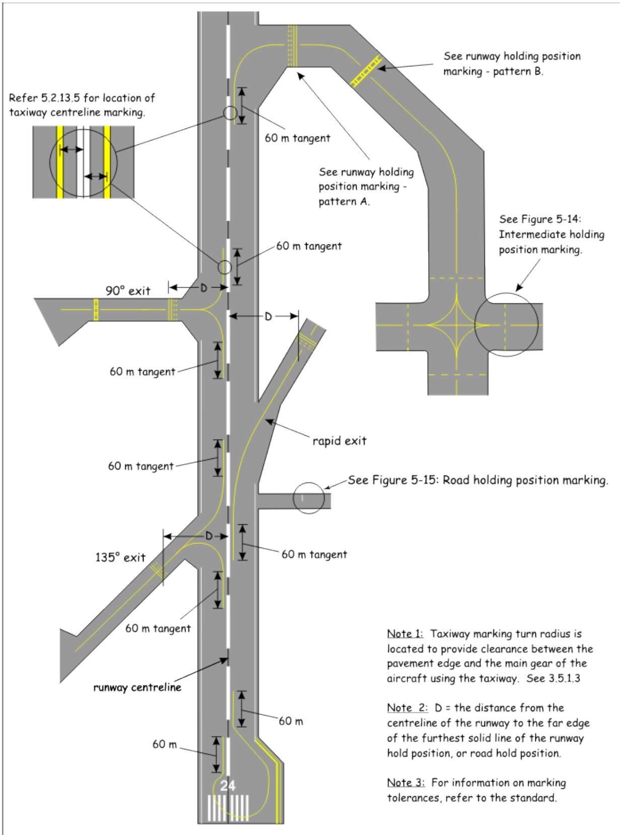
Figure 5-8: Taxiway markings
