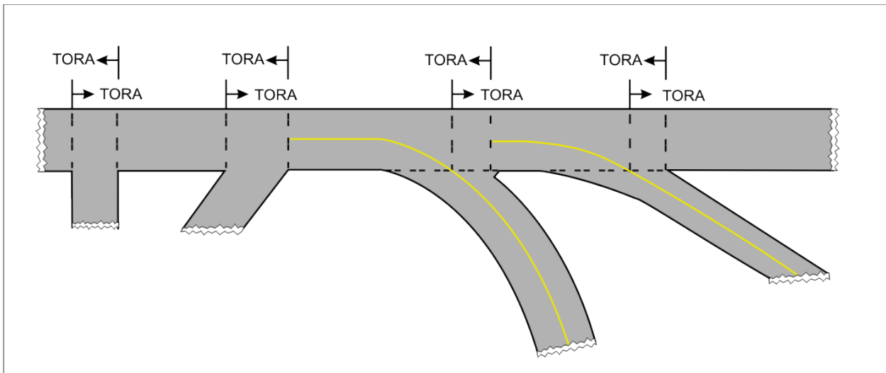
Figure 2-3: Illustration of intersection take-off run distances
