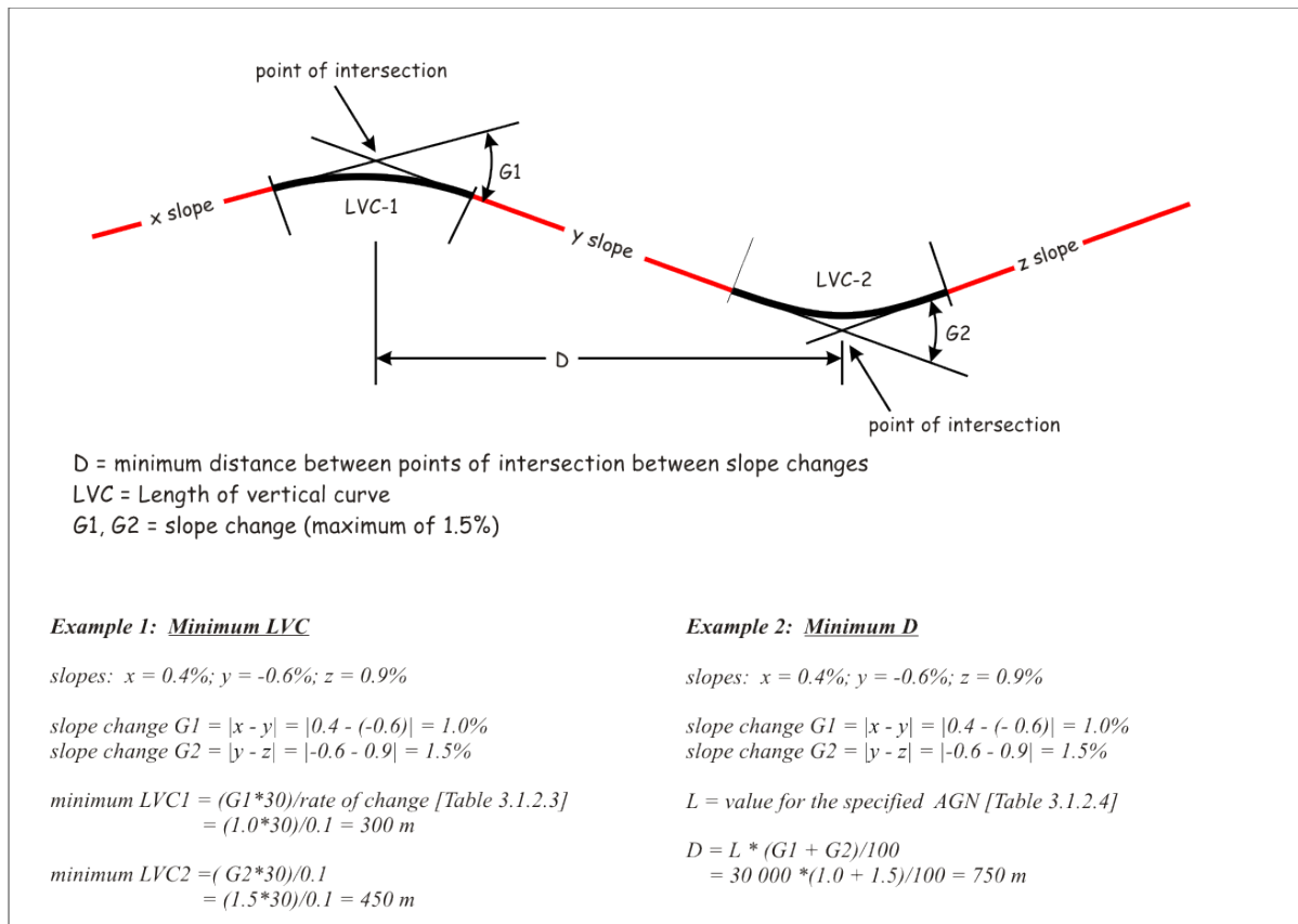
Figure 3-1: Runway longitudinal slope limitations
