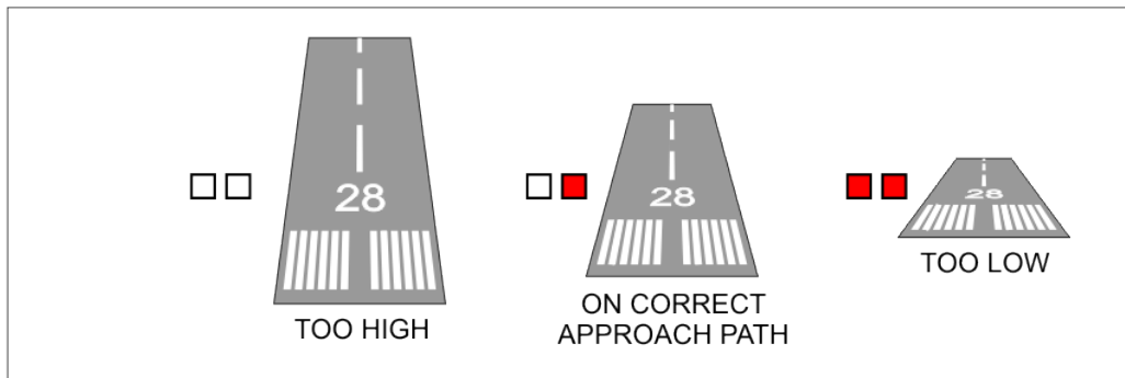
Figure 5-40: APAPI approach slope presentation
