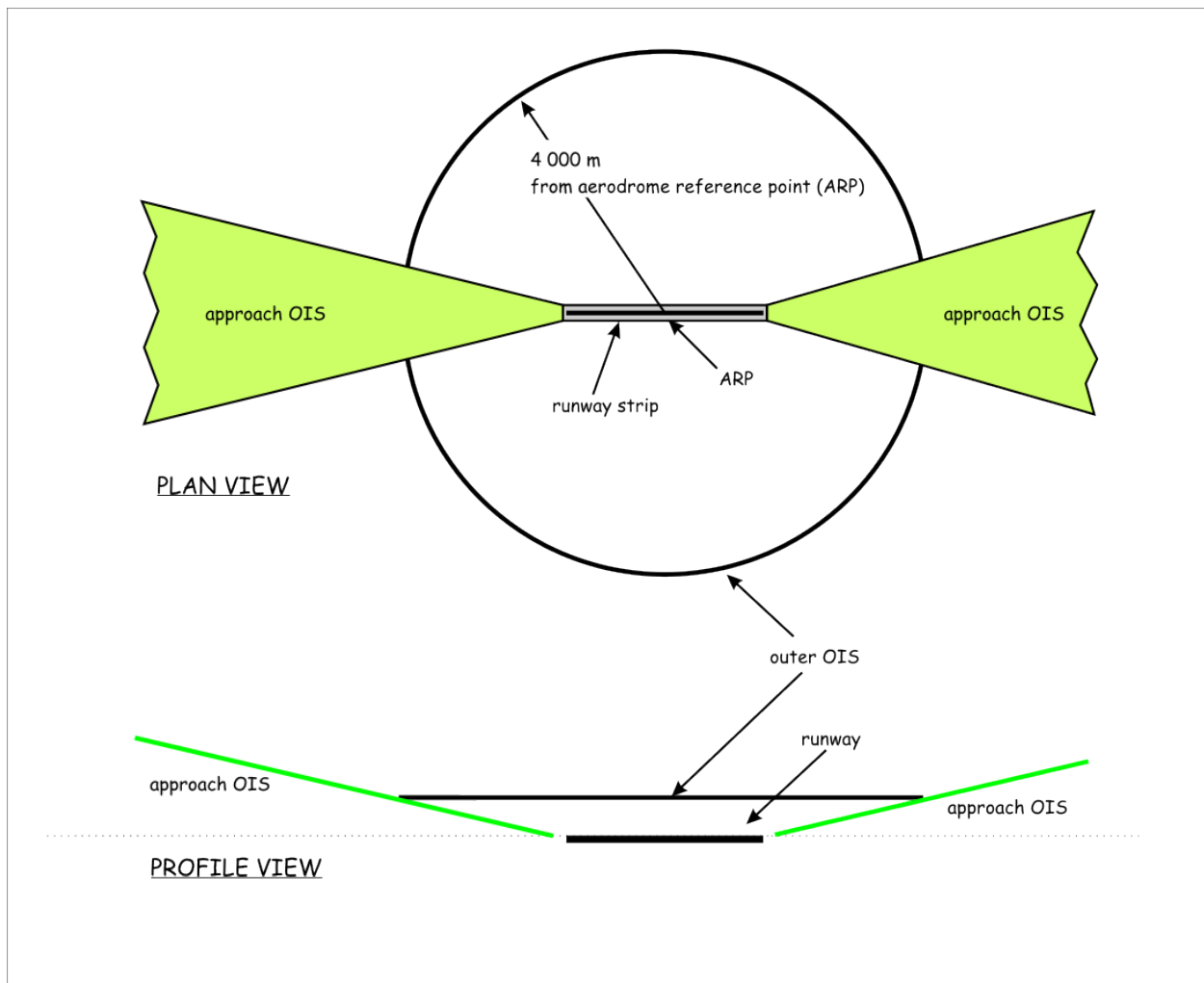
Figure 4-8: Obstacle identification surfaces (OIS)
