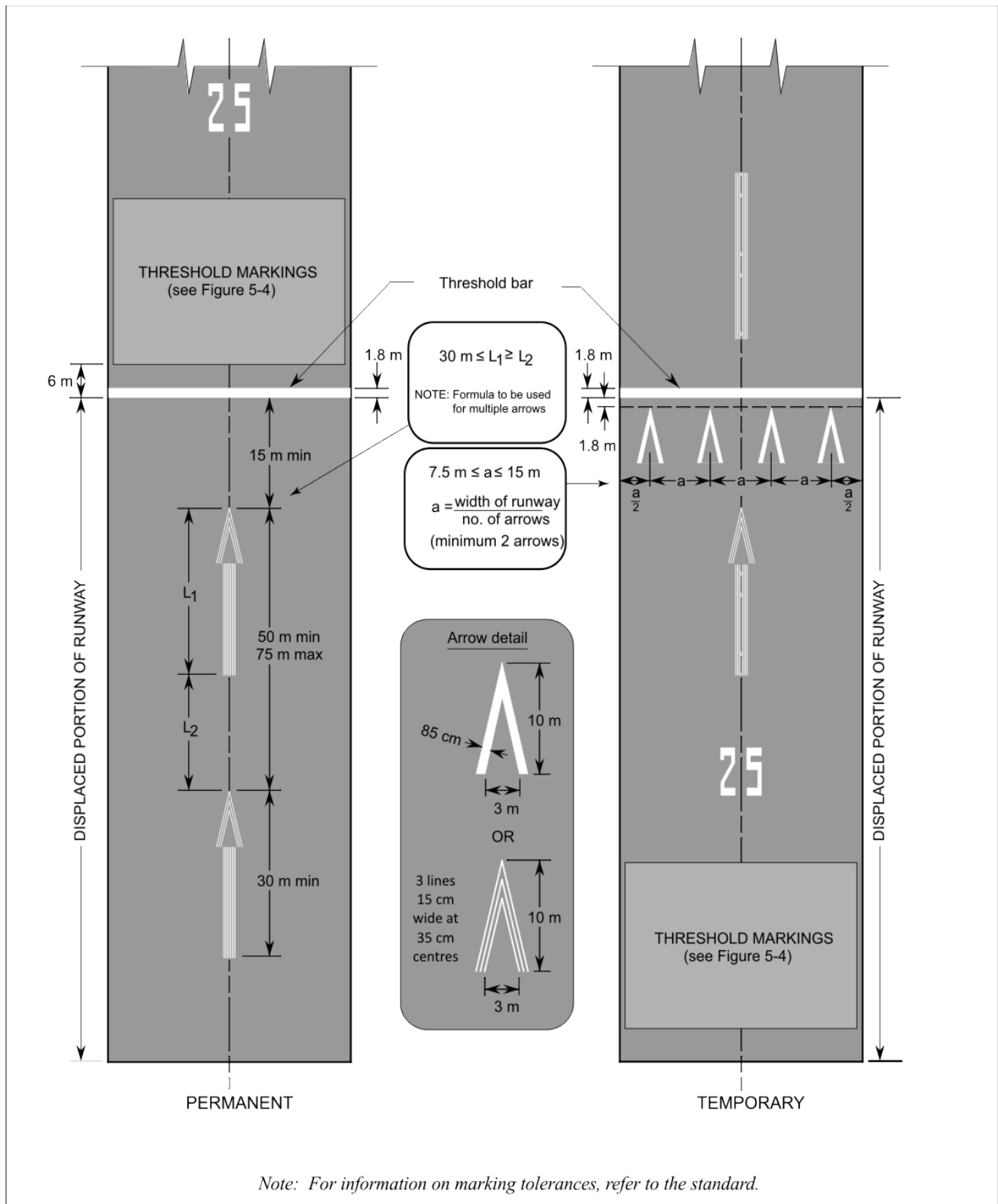
Figure 5-6(a): Arrow markings
