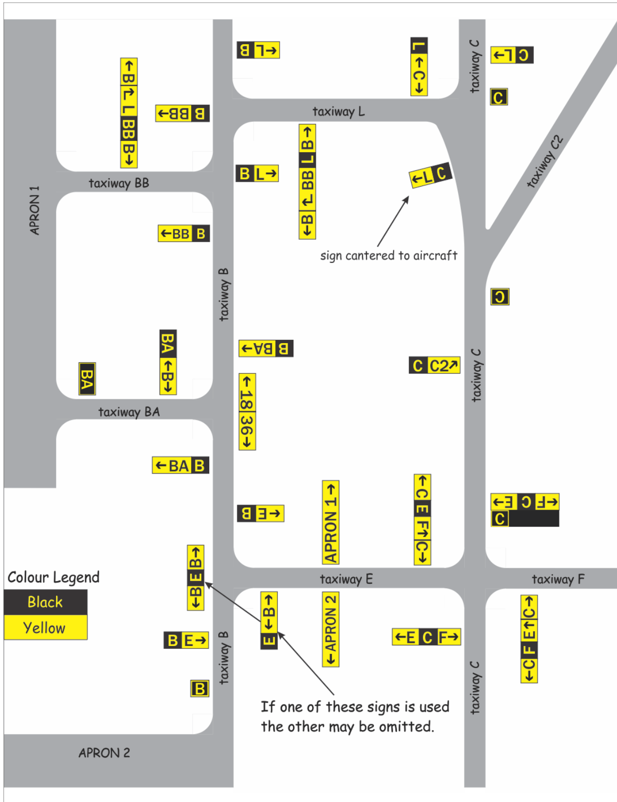
Figure 5-62: Examples of locating information signs
