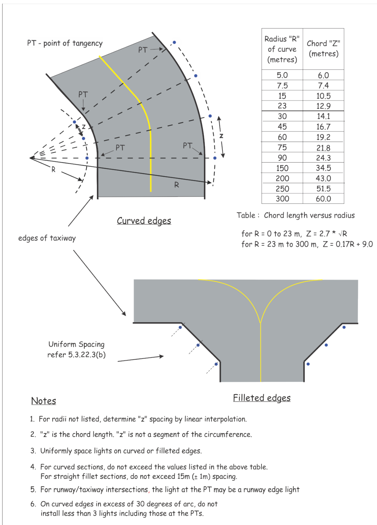
Figure 5-53: Spacing of lights on curved taxiway edges
