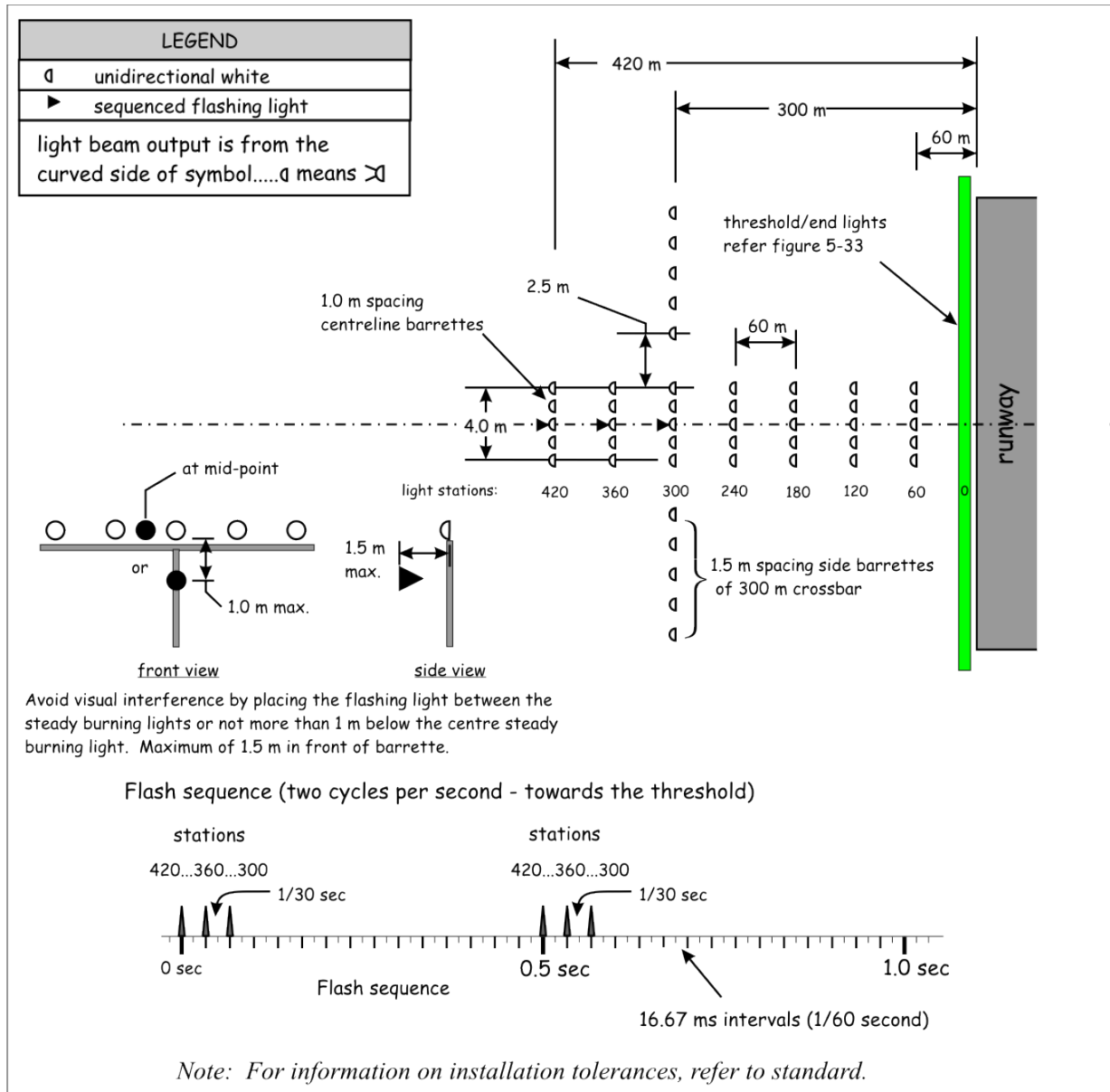
Figure 5-30: MALSF configuration
