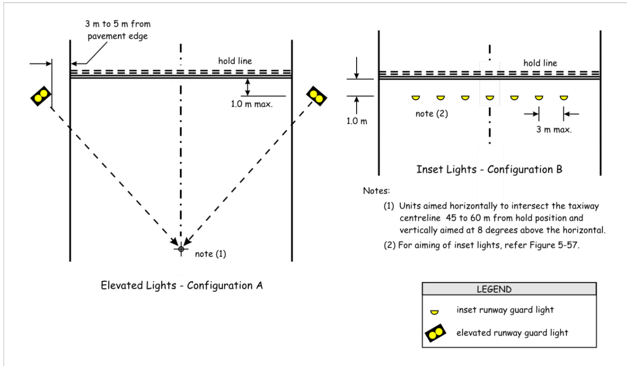
Figure 5-56: Runway guard light configuration
