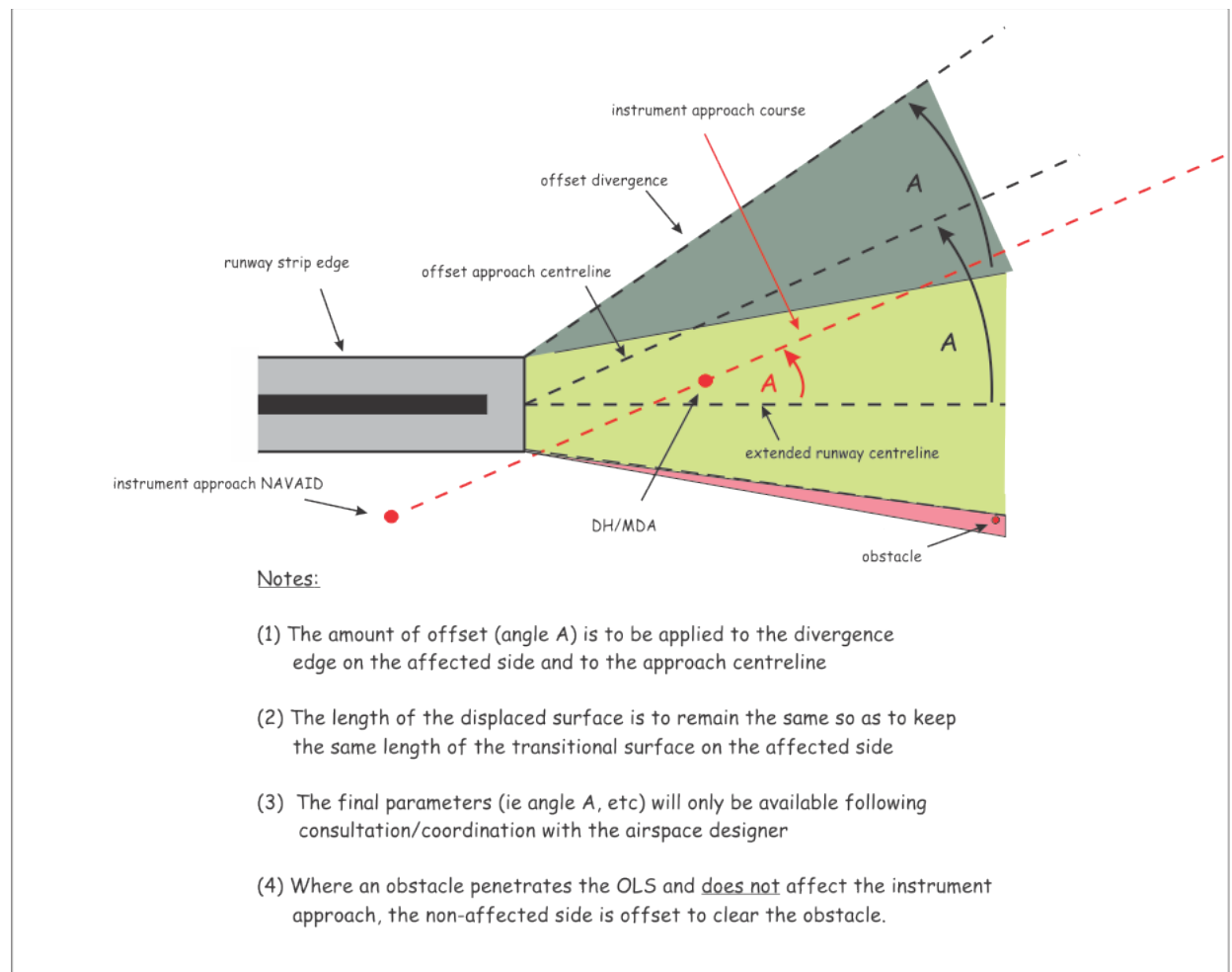
Figure 4-3(a): Offset approach surface (Precision or Non-Precision runways)
