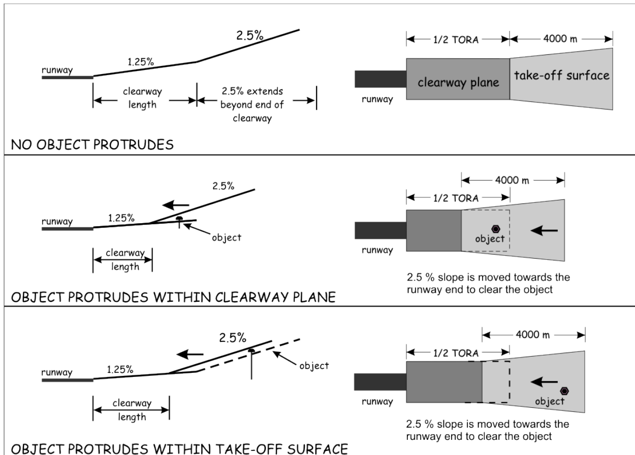
Figure 4-9: Clearway plane
