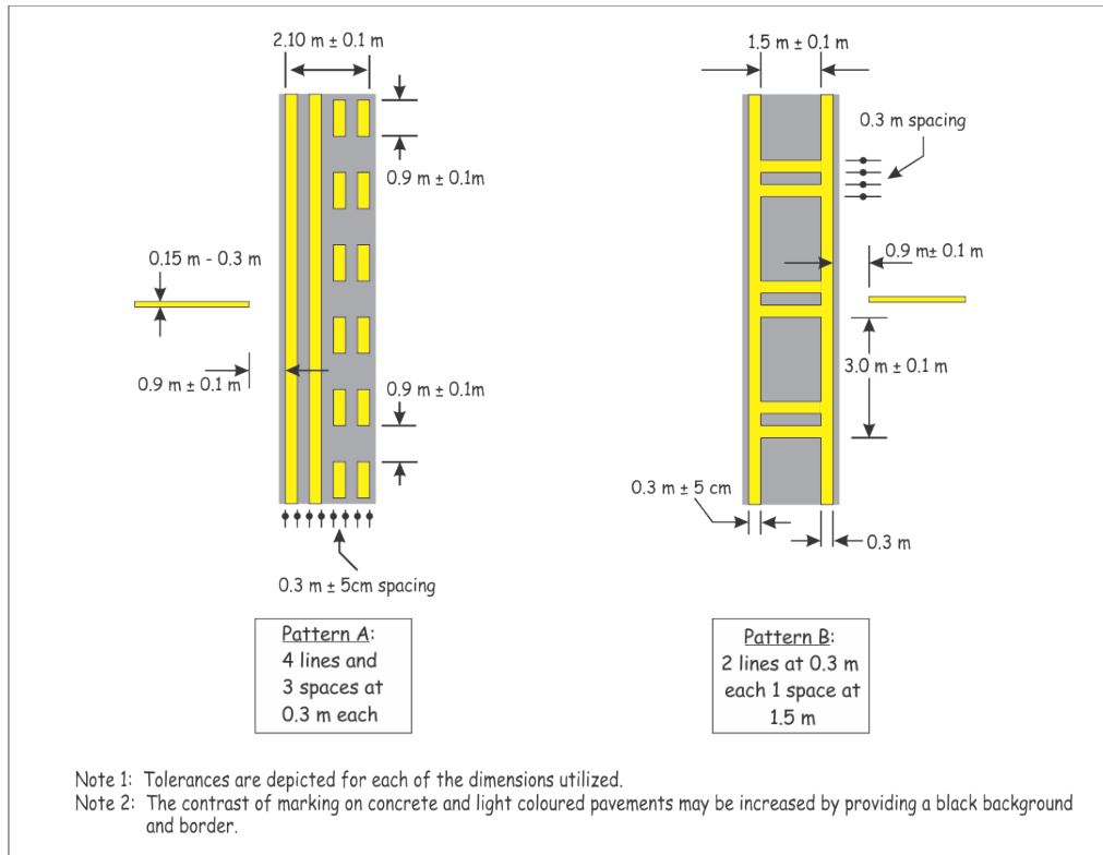
Figure 5-12: Runway-holding position markings
