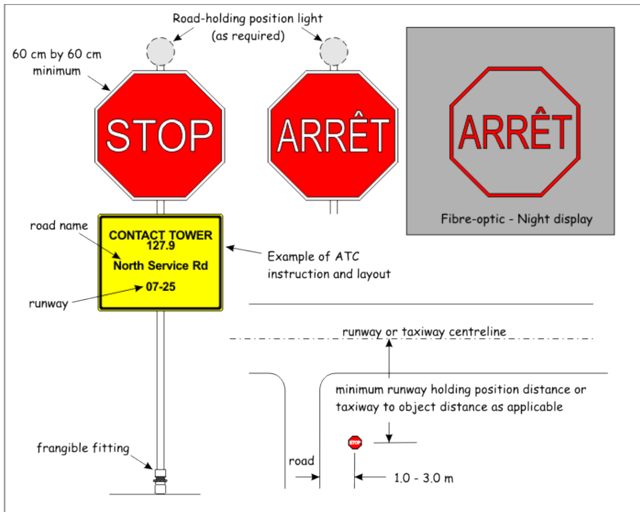
Figure 5-66: Road-holding position sign
