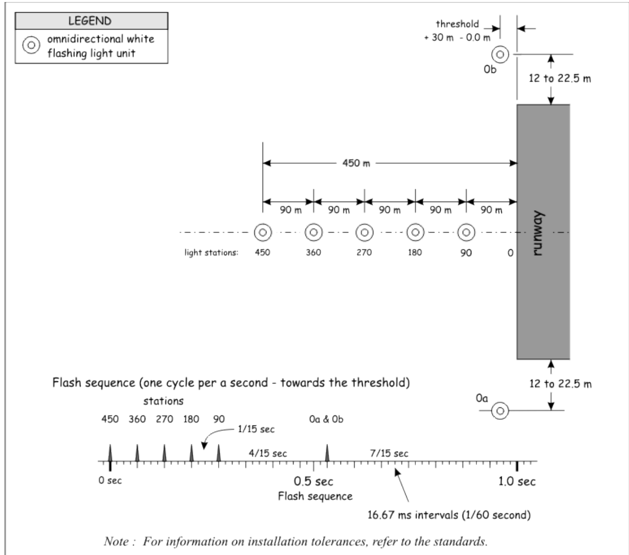
Figure 5-24: ODALS configuration
