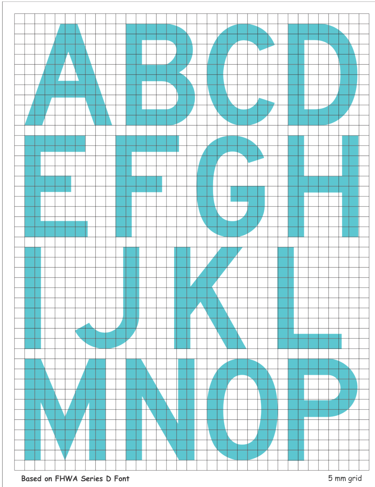
Figure 5-69 (a): Forms of characters (signs)
