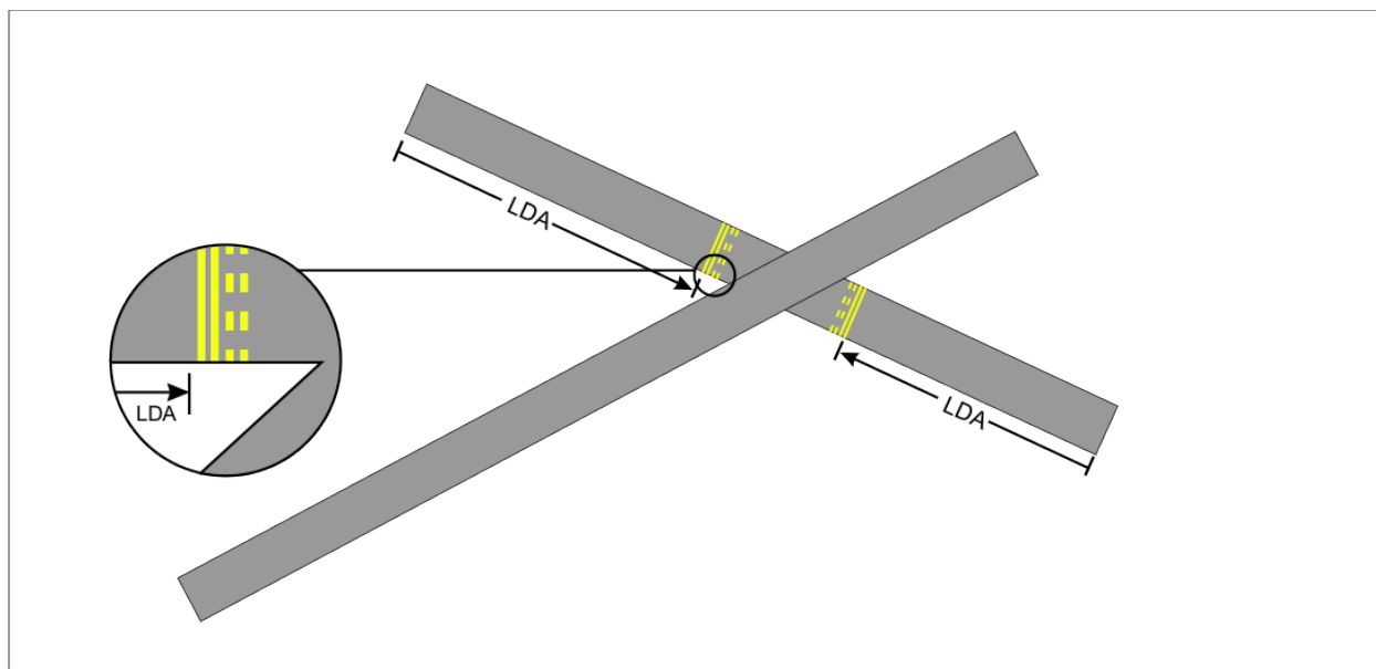
Figure 2-2 : Illustration des distances LAHSO
