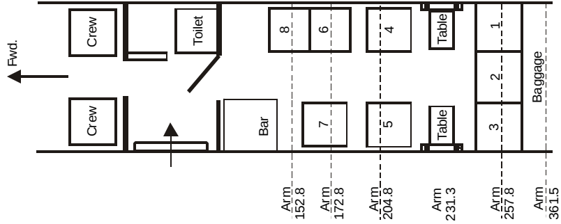
Aircraft Seating Diagram
